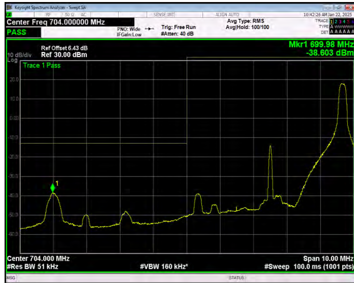
Band17 QPSK BW=5MHz Channel=23755 RB Size=25 Position=#0 Extended
