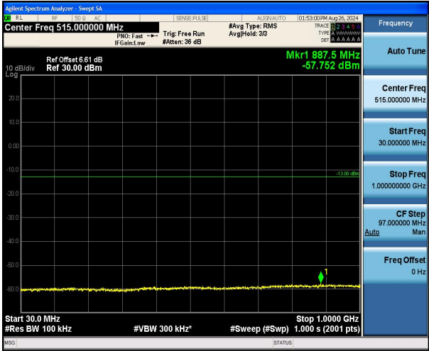
Band4_15MHz_QPSK_20325_1RB#0_30~1000_30~1000
