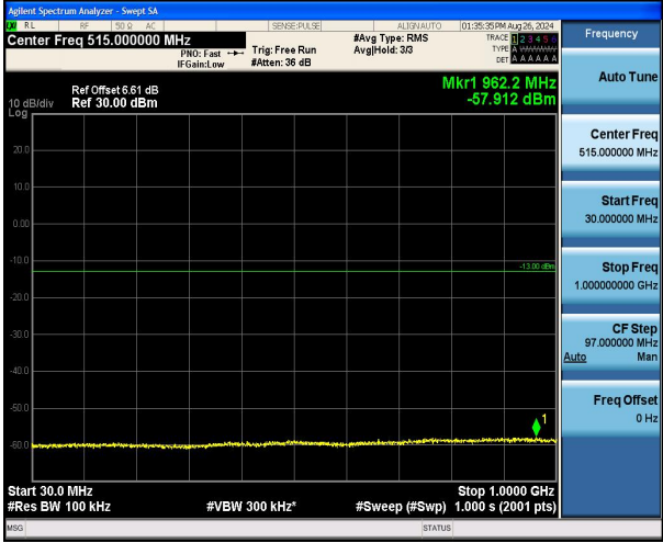
Band4_10MHz_16QAM_20000_1RB#0_30~1000_30~1000
