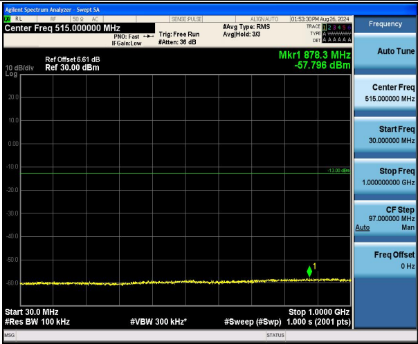
Band4_15MHz_16QAM_20325_1RB#0_30~1000_30~1000
