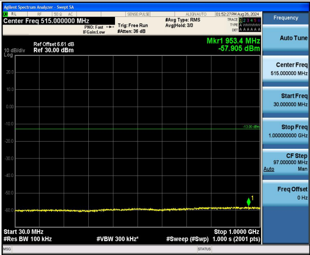
Band4_15MHz_16QAM_20175_1RB#0_30~1000_30~1000
