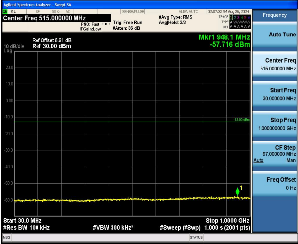
Band4_20MHz_16QAM_20050_1RB#0_30~1000_30~1000
