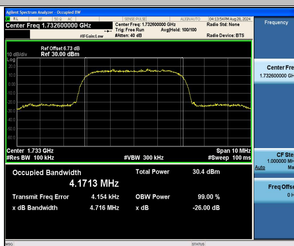
Band4-1413-PASS
