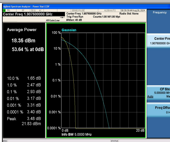
Band2-9538-PASS
