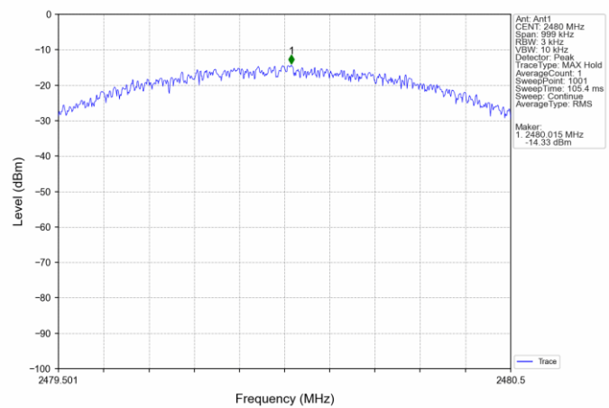
1M_HCH_2480MHz_Ant1_NTNV
