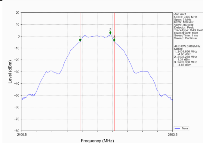
1M_LCH_2402MHz_Ant1_NTNV
