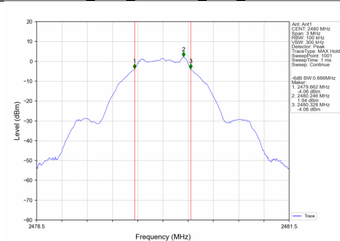
1M_HCH_2480MHz_Ant1_NTNV
