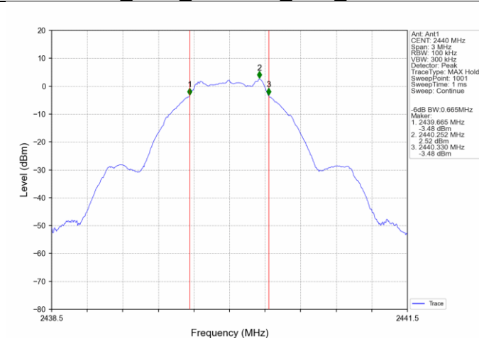
1M_MCH_2440MHz_Ant1_NTNV
