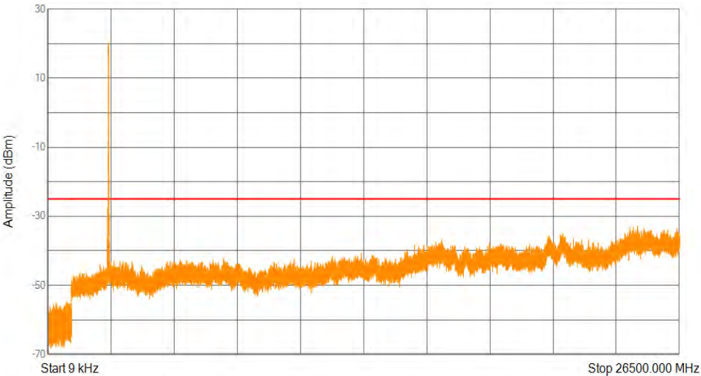
Band41(2555-2655) QPSK BW=10MHz Channel=40290 RB Size=50 Position=#0
