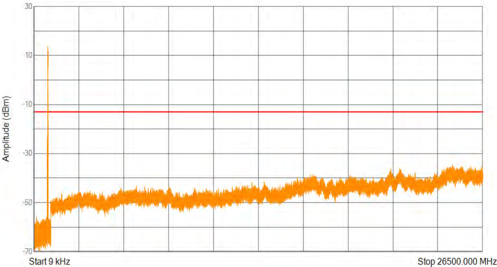
Band26(824-849) QPSK BW=10MHz Channel=26840 RB Size=50 Position=#0
