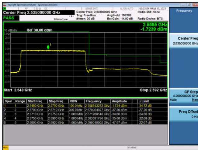
FDD7-20MHz-QPSK-HCH-100RB#0
