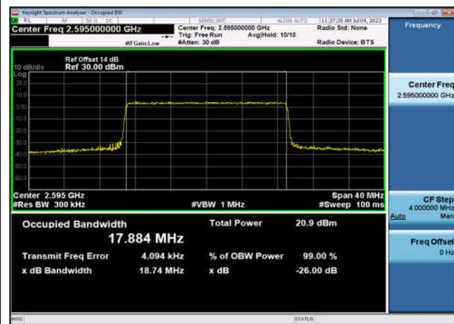
TDD41_MidRange_20_2595_QPSK
