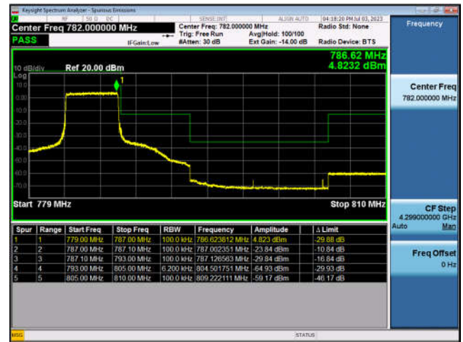
FDD13-10MHz-16QAM-MCH-1RB#0
