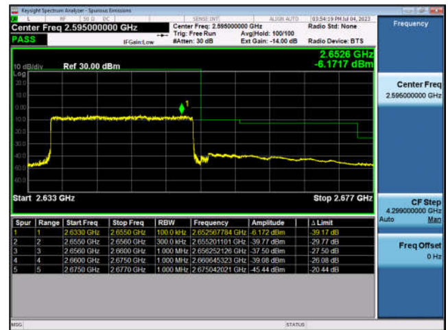
FDD7-20MHz-16QAM-HCH-100RB#0
