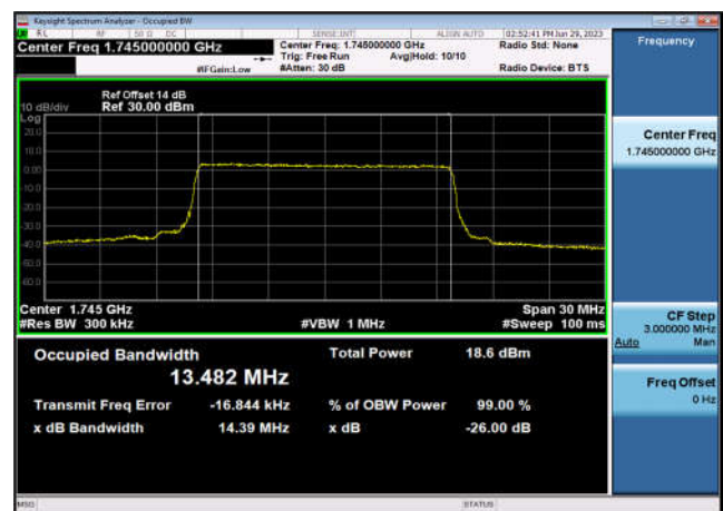
FDD66_MidRange_15_1745_Q16
