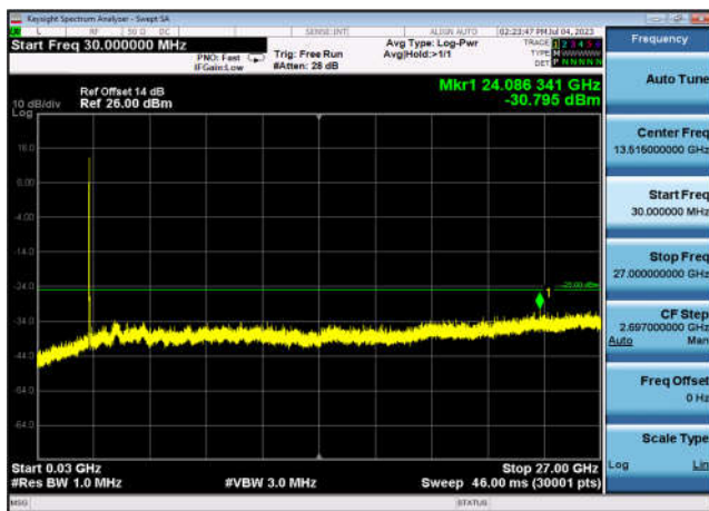
TDD41_MidRange_20MHz_30MHz~27GHz
