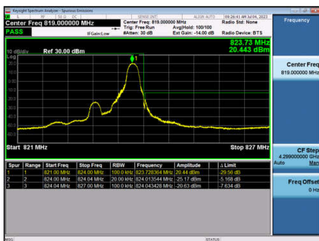
FDD26-Part 90-1.4MHz-QPSK-HCH-1RB#5
