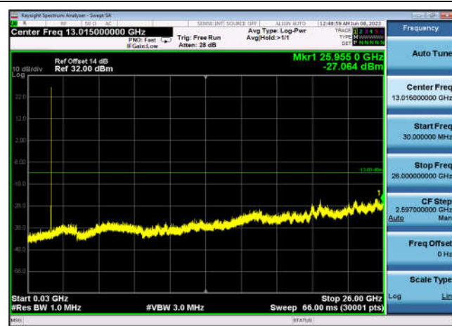
FDD04_MidRange_10MHz_30MHz~26GHz
