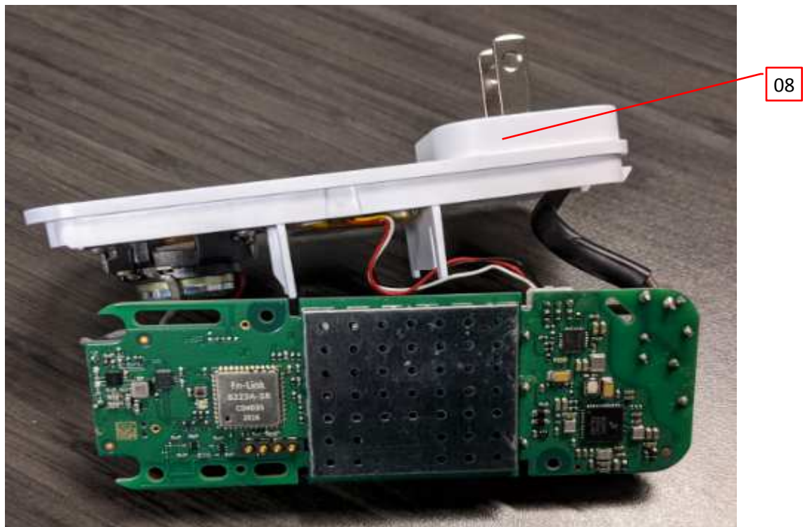
Photo 6 - Internal Top view of the HUB PCB and components
