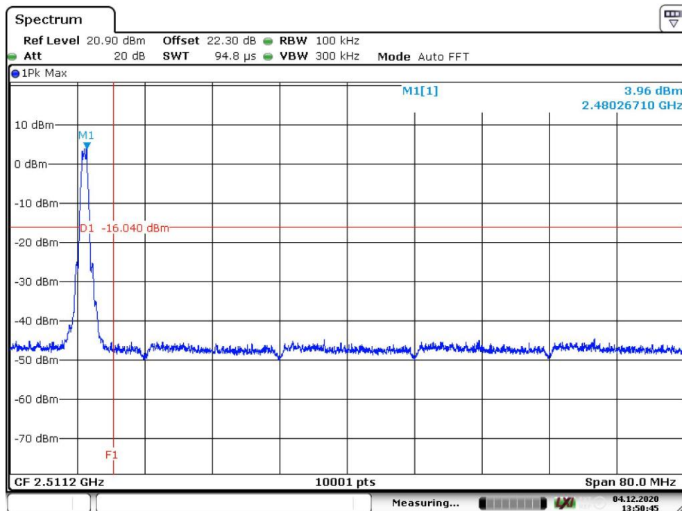
Screenshot: Upper band edge sweep, Bluetooth Low Energy 1 Mbit
