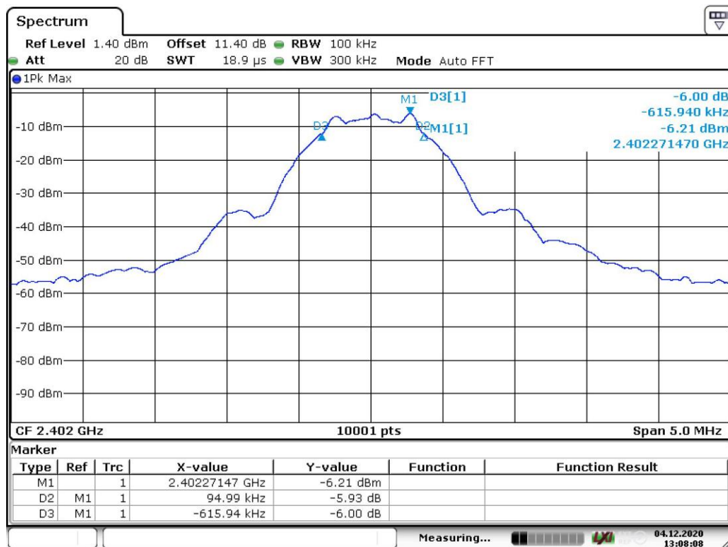
Screenshot: Occupied 6 dB bandwidth, low channel, Bluetooth Low Energy 1 Mbit
