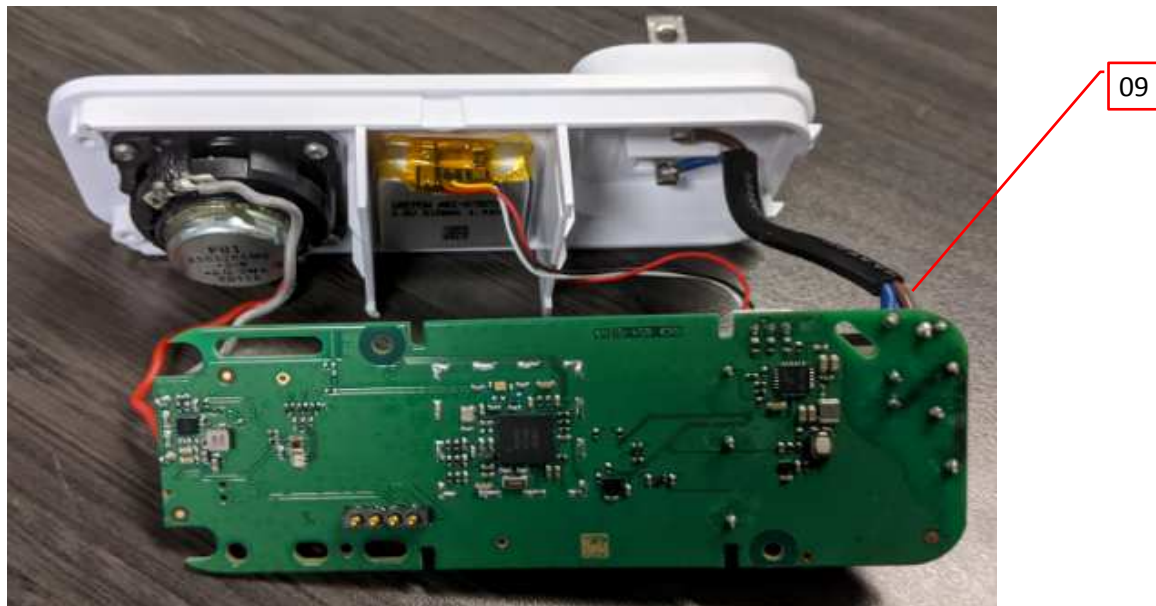
Photo 4 - Internal Bottom view of the SATELLITE PCB and components
