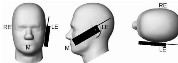
Figure 5: "Cheek" position of DUT
