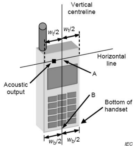
Figure 4: DUT's basic scheme
