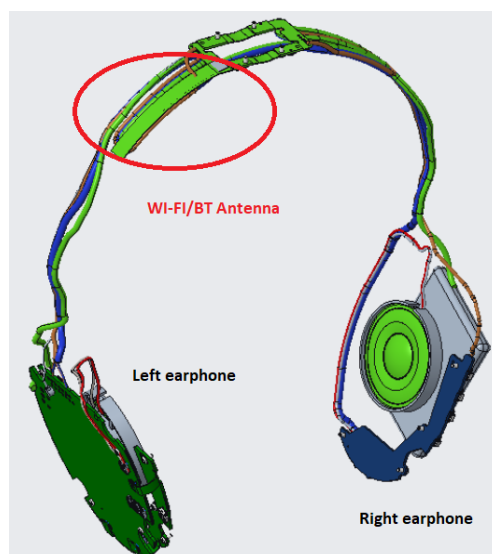
Figure 7: Antenna location.
