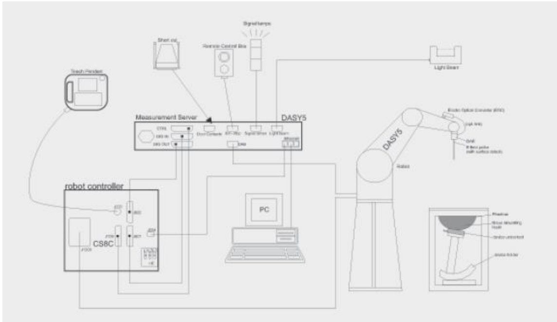
Figure 3: SAR Measurement system
