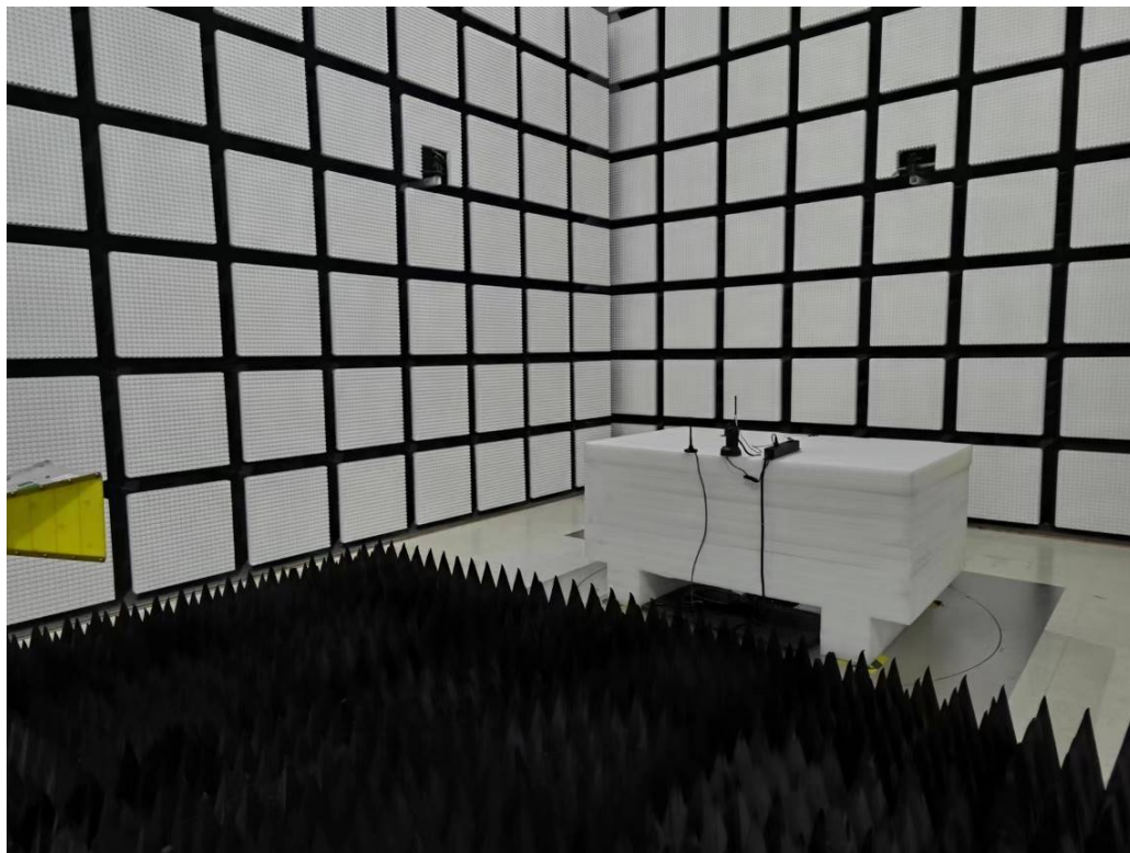
Radiated Emission Above 1GHz Rear View M3
