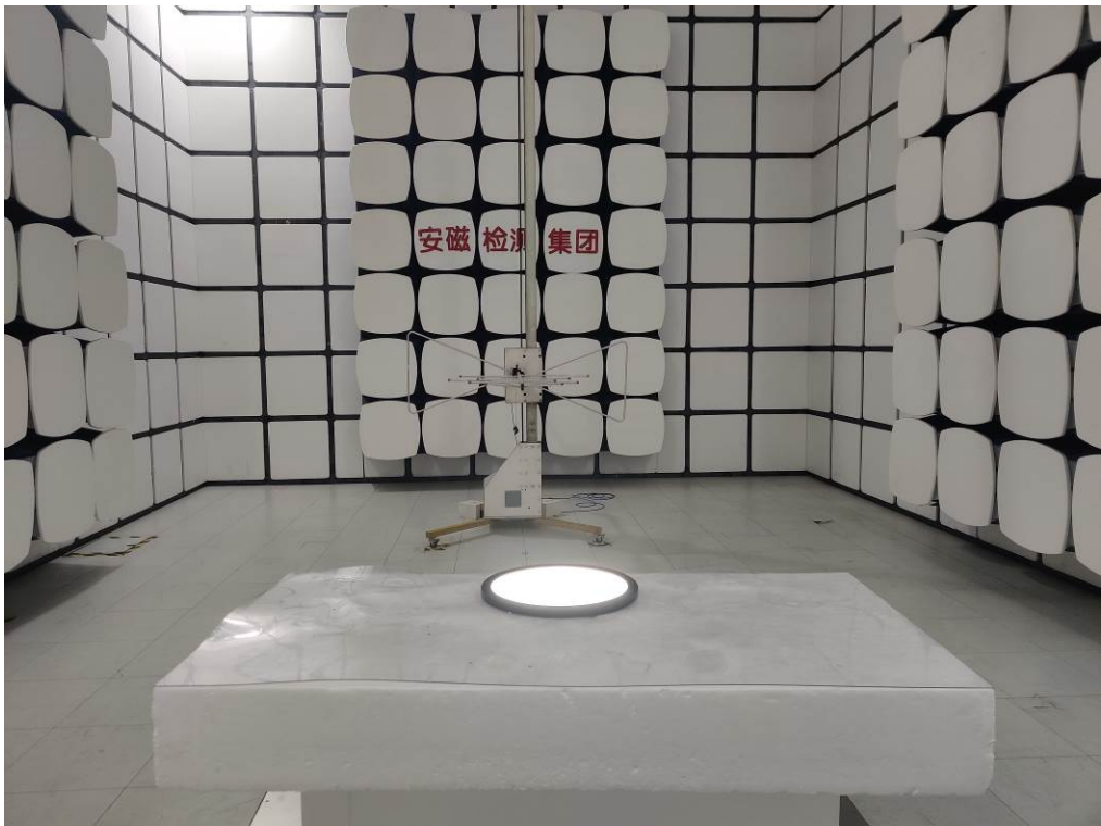
Photos of Radiation Emission Measurement
