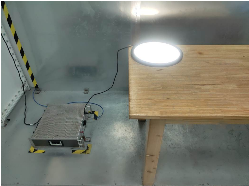
Photos of Conducted Emission Measurement
