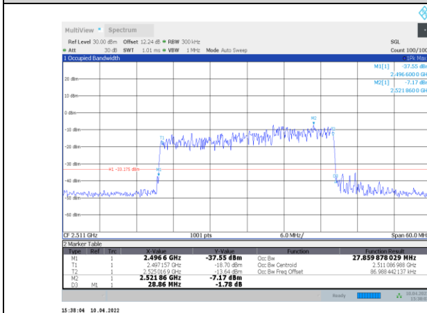
1-N41-PC3-30-30-L-4-DFT-64QAM-Outter_Full-75@0-Ant 1-27.86-28.860-≤30-PASS
