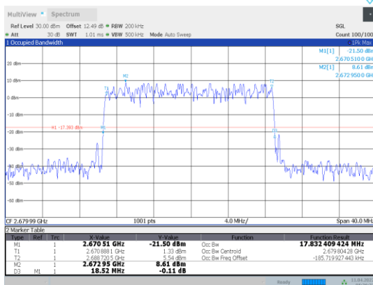
1-N41-PC3-30-20-H-9-DFT-256QAM-Outer_Full-50@0-Ant 1-17.832-18.520-≤20-PASS
