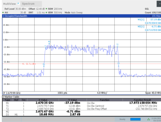
1-N41-PC3-30-20-H-7-CP-64QAM-Outer_Full-51@0-Ant 1-17.973-18.680-≤20-PASS
