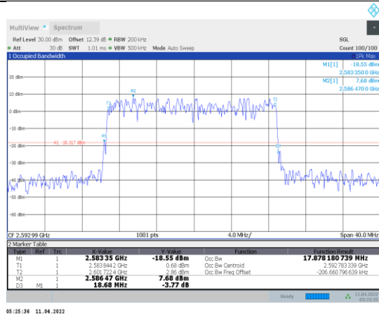
1-N41-PC3-30-20-M-9-DFT-256QAM-Outer_Full-50@0-Ant1-17.878-18.680-≤20-PASS
