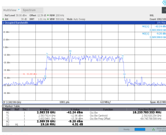
1-N41-PC3-30-20-M-2-DFT-PI2BPSK-Outer_Full-51@0-Ant 1-18.256-19.160-≤20-PASS
