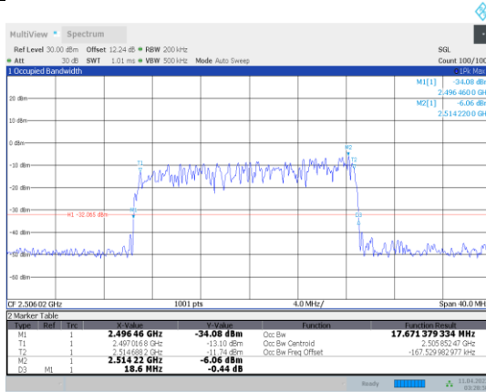
1-N41-PC3-30-20-L-7-CP-64QAM-Outer_Full-51@0-Ant 1-17.671-18.600-≤20-PASS
