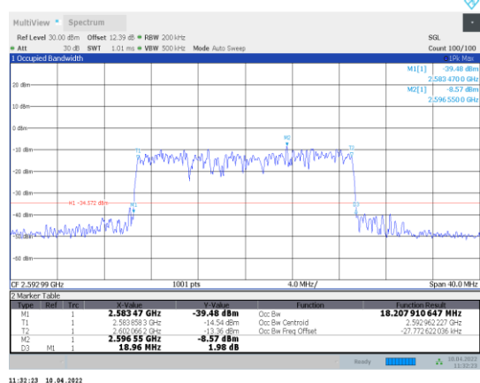
1-N41-PC3-30-20-M-1-DFT-QPSK-Outer_Full-50@0-Ant 1-18.208-18.960-≤20-PASS
