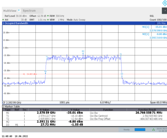
1-N41-PC3-30-30-M-1-DFT-QPSK-Outer_Full-75@0-A nt1-26.767-27.720-≤30-PASS
