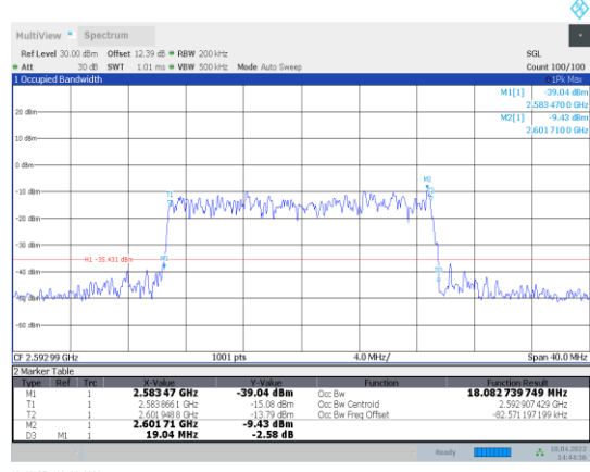
1-N41-PC3-30-20-M-3-DFT-16QAM-Outer_Full-50@0-Ant 1-18.083-19.040-≤20-PASS
