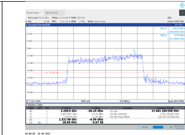
1-N41-PC3-30-30-L-3-DFT-16QAM-Outter_Full-75@0-Ant 1-27.681-28.980-≤30-PASS
