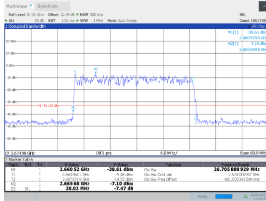
1-N41-PC3-30-30-H-6-CP-16QAM-Outer_Full-78@0-A Ant1-26.706-28.020-≤30-PASS
