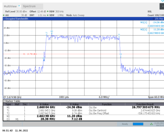
1-N41-PC3-30-30-H-8-CP-256QAM-Outer_Full-78@0- Ant1-26.797-28.380-≤30-PASS
