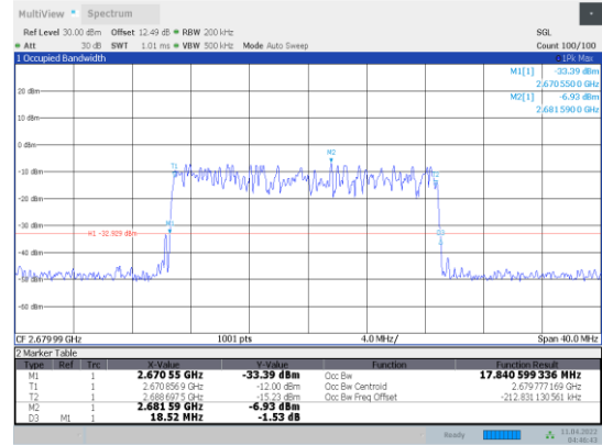
1-N41-PC3-30-20-H-8-CP-256QAM-Outer_Full-51@0-Ant 1-17.841-18.520-≤20-PASS
