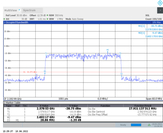
1-N41-PC3-30-30-M-4-DFT-64QAM-Outer_Full-75@0-A nt1-27.921-28.860-≤30-PASS
