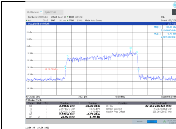
1-N41-PC3-30-30-L-1-DFT-QPSK-Outter_Full-75@0-Ant 1-27.51-28.920-≤30-PASS
