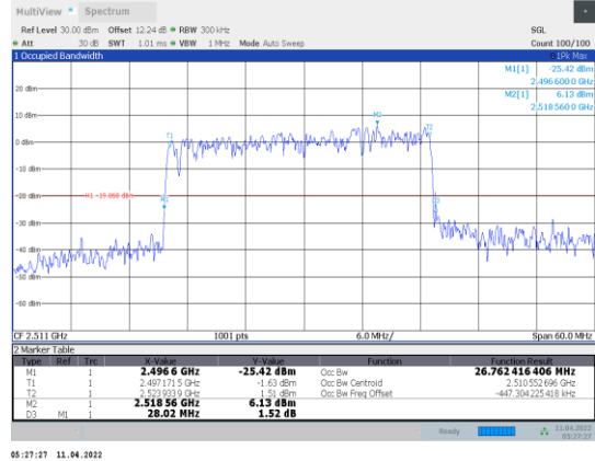
1-N41-PC3-30-30-L-9-DFT-256QAM-Outer_Full-75@0-A nt1-26.762-28.020-≤30-PASS
