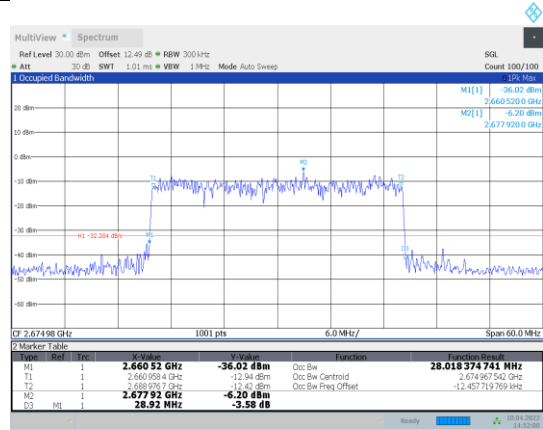
1-N41-PC3-30-30-H-3-DFT-16QAM-Outer_Full-75@0-Ant1-28.031-28.920-≤30-PASS
