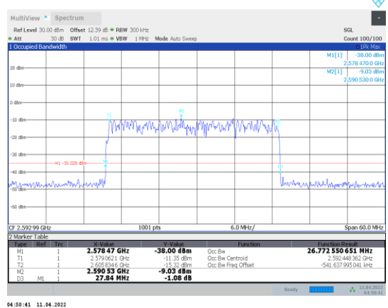
1-N41-PC3-30-30-M-8-CP-256QAM-Outer_Full-78@0-A nt1-26.773-27.840-≤30-PASS
