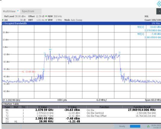
1-N41-PC3-30-30-M-3-DFT-16QAM-Outer_Full-75@0-A nt1-27.975-28.980-≤30-PASS
