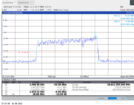
1-N41-PC3-30-30-L-6-CP-16QAM-Outer_Full-78@0-A nt1-26.611-28.080-≤30-PASS
