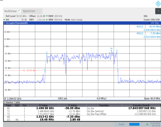
1-N41-PC3-30-20-L-8-CP-256QAM-Outer_Full-51@0-Ant 1-17.845-18.480-≤20-PASS
