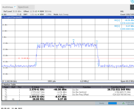
1-N41-PC3-30-30-M-7-CP-64QAM-Outer_Full-78@0-A nt1-26.721-28.080-≤30-PASS
