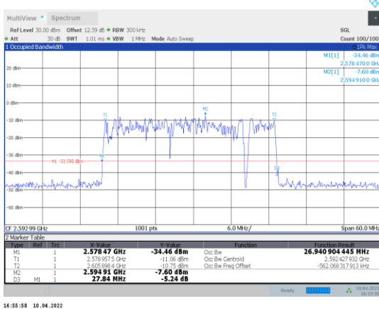
1-N41-PC3-30-30-M-5-CP-QPSK-Outer_Full-78@0-Ant 1-26.941-27.840-≤30-PASS
