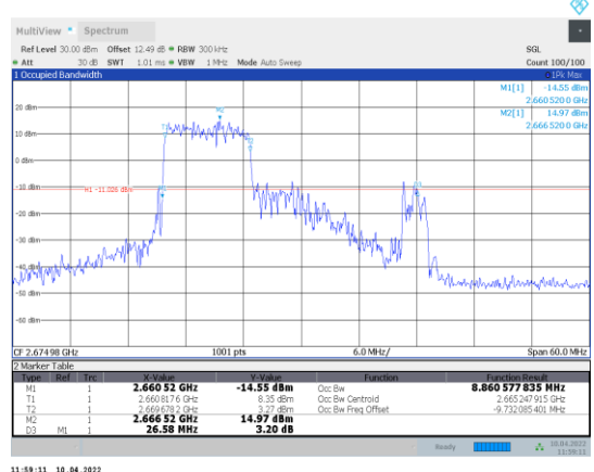
1-N41-PC3-30-30-H-1-DFT-QPSK-Outer_Full-75@0-An t1-8.865-26.580-≤30-PASS
