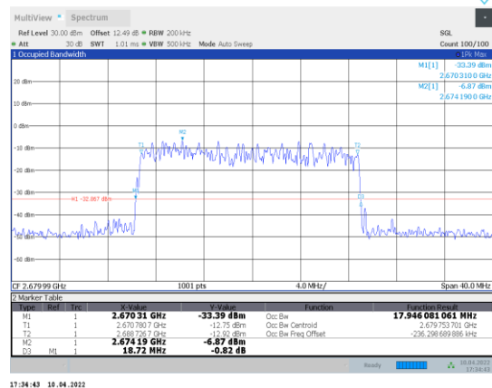
1-N41-PC3-30-20-H-6-CP-16QAM-Outet_Full-51@0-A nt1-17.946-18.720-≤20-PASS
