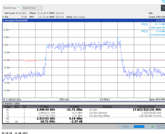
1-N41-PC3-30-20-L-9-DFT-256QAM-Outer_Full-50@0-Ant 1-17.823-18.720-≤20-PASS
