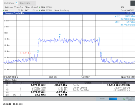
1-N41-PC3-30-20-H-2-DFT-PI2BPSK-Outet_Full-51@0-A nt1-18.319-19.200-≤20-PASS
