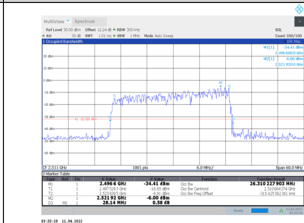
1-N41-PC3-30-30-L-7-CP-64QAM-Outter_Full-78@0-Ant 1-26.31-28.140-≤30-PASS
