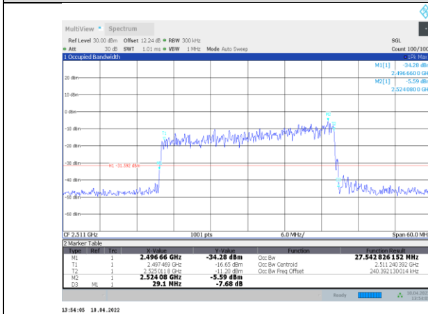
1-N41-PC3-30-30-L-2-DFT-PI2BPSK-Outter_Full-78@0-Ant 1-27.543-29.100-≤30-PASS
