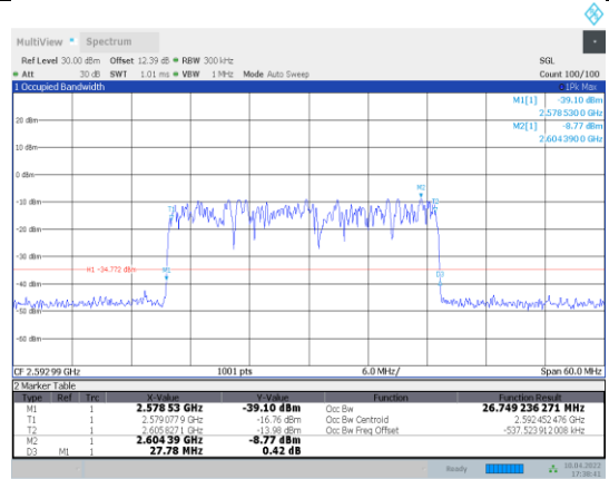
1-N41-PC3-30-30-M-6-CP-16QAM-Outer_Full-78@0-An t1-26.749-27.780-≤30-PASS
