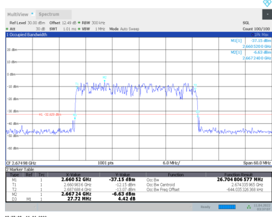
1-N41-PC3-30-30-H-7-CP-64QAM-Outer_Full-78@0-Ant1-26.705-27.720-≤30-PASS
