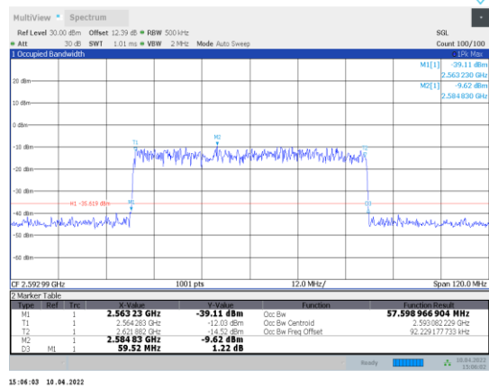
1-N41-PC3-30-60-M-3-DFT-16QAM-Outer_Full-162@0-A Ant1-57.599-59.520-≤60-PASS
