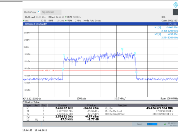
1-N41-PC3-30-50-L-5-CP-QPSK-Outter_Full-133@0-A nt1-45.425-47.300-≤50-PASS
