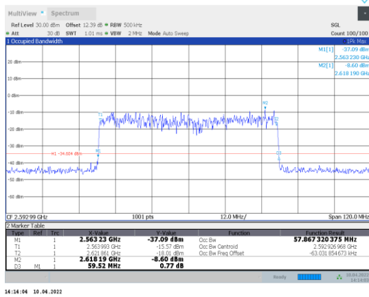
1-N41-PC3-30-60-M-2-DFT-PI2BPSK-Outer_Full-162@0-A Ant1-57.867-59.520-≤60-PASS
