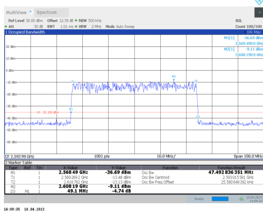
1-N41-PC3-30-50-M-2-DFT-PI2BPSK-Outer_Full-133@0- Ant1-47.493-49.100-≤50-PASS
