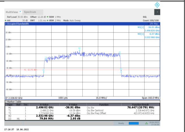
1-N41-PC3-30-80-L-5-CP-QPSK-Outer_Full-217@0-A nt1-76.447-79.840-≤80-PASS
