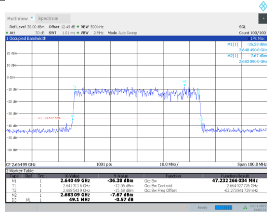
1-N41-PC3-30-50-H-3-DFT-16QAM-Outer_Full-128@0-Ant1-47.232-49.100-≤50-PASS
