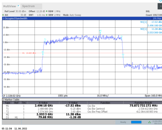
1-N41-PC3-30-80-L-8-CP-256QAM-Outer_Full-217@0- Ant1-75.873-79.680-≤80-PASS
