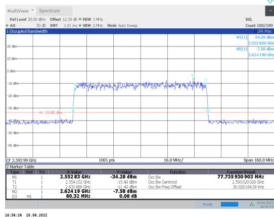
1-N41-PC3-30-80-M-4-DFT-64QAM-Outer_Full-216@0- Ant1-77.736-80.320-≤80-PASS
