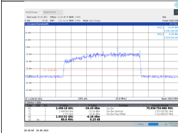
1-N41-PC3-30-80-L-2-DFT-PI2BPSK-Outer_Full-217@0-A nt1-75.937-80.000-≤80-PASS
