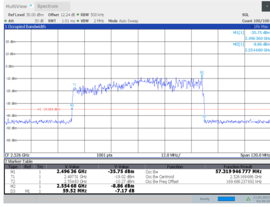
1-N41-PC3-30-60-L-7-CP-64QAM-Outer_Full-162@0-A nt1-57.32-59.520-≤60-PASS
