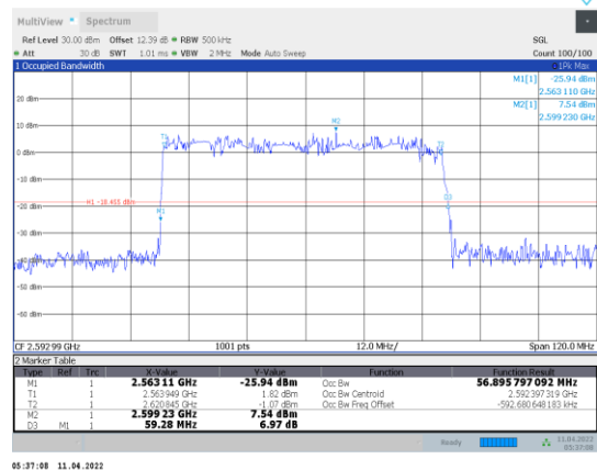
1-N41-PC3-30-60-M-9-DFT-256QAM-Outer_Full-162@0-Ant1-56.896-59.280-≤60-PASS
