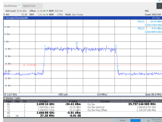
1-N41-PC3-30-40-H-6-CP-16QAM-Out_ Full-106@0-Ant1-35.788-37.280-≤40-PASS
