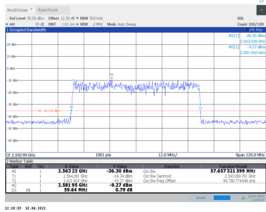
1-N41-PC3-30-60-M-1-DFT-QPSK-Outer_Full-162@0-A Ant1-57.657-59.640-≤60-PASS
