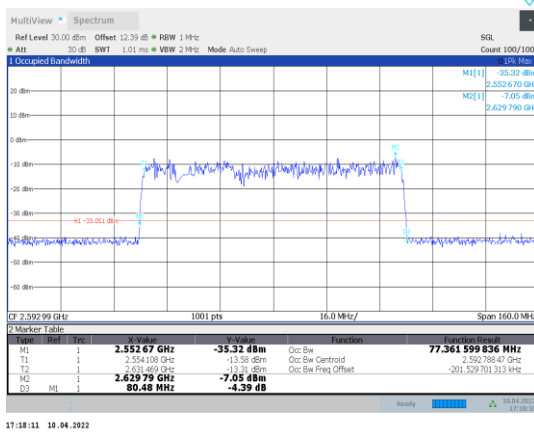
1-N41-PC3-30-80-M-5-CP-QPSK-Outer_Full-217@0-Ant1-77.362-80.480-≤80-PASS
