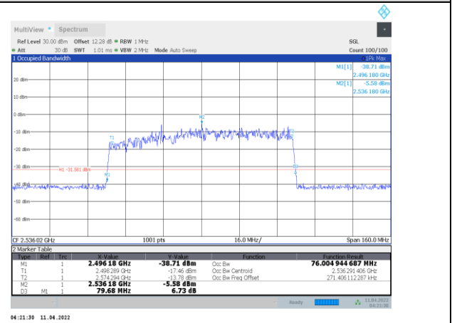
1-N41-PC3-30-80-L-7-CP-64QAM-Outer_Full-217@0-A nt1-76.005-79.680-≤80-PASS
