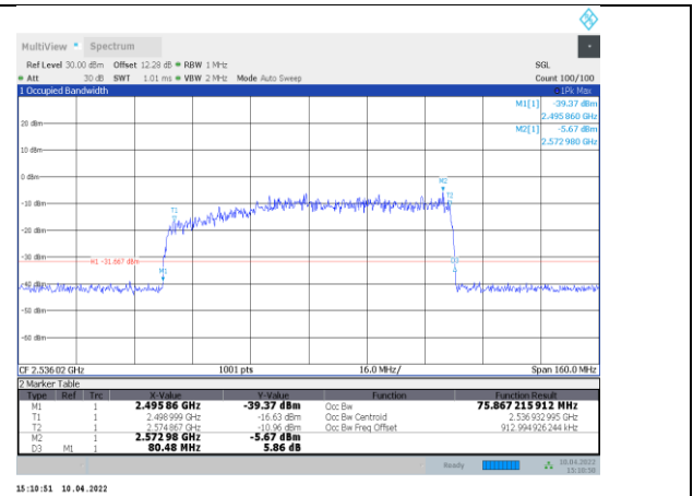
1-N41-PC3-30-80-L-3-DFT-16QAM-Outer_Full-216@0-A nt1-75.867-80.480-≤80-PASS
