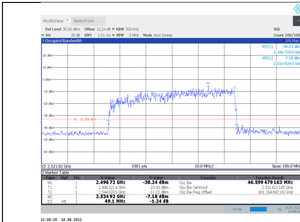
1-N41-PC3-30-50-L-1-DFT-QPSK-Outter_Full-128@0-A nt1-46.599-49.100-≤50-PASS
