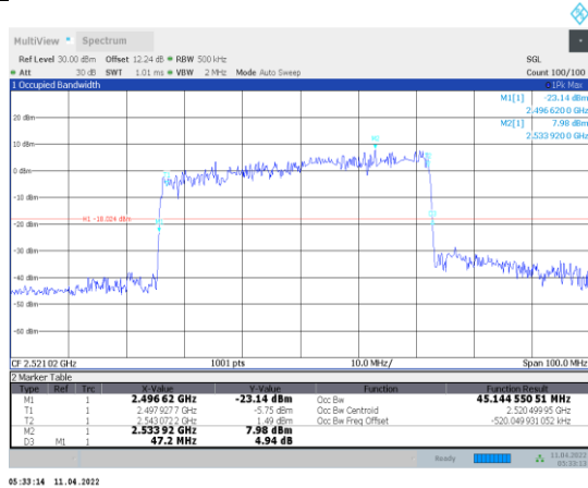
1-N41-PC3-30-50-L-9-DFT-256QAM-Outer_Full-128@0- Ant1-45.145-47.200-≤50-PASS
