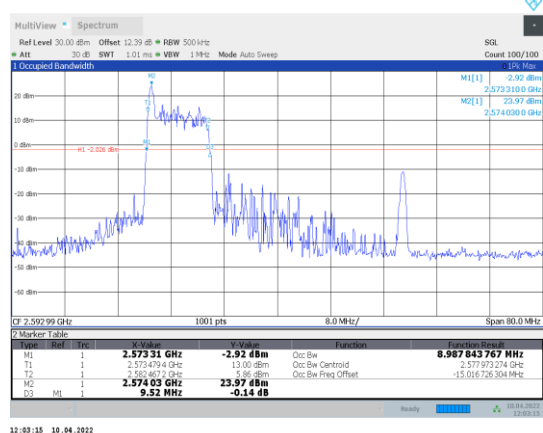
1-N41-PC3-30-40-M-1-DFT-QPSK-Outer_Full-100@0-A Ant1-8.988-9.520-≤40-PASS
