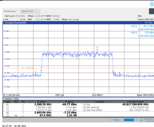
1-N41-PC3-30-50-M-4-DFT-64QAM-Outer_Full-128@0- Ant1-45.817-47.400-≤50-PASS
