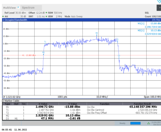
1-N41-PC3-30-50-L-8-CP-256QAM-Outer_Full-133@0- Ant1-45.148-47.100-≤50-PASS
