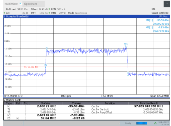
1-N41-PC3-30-60-H-2-DFT-PI2BPSK-Outter_Full-162@0-Ant1-57.86-59.640-≤60-PASS
