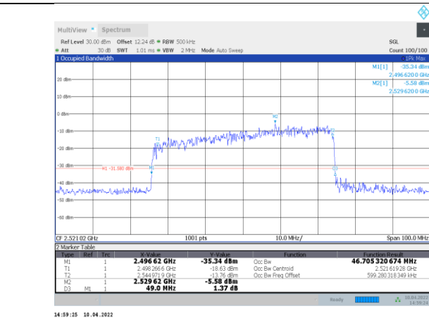
1-N41-PC3-30-50-L-3-DFT-16QAM-Outter_Full-128@0-A Ant1-46.705-49.000-≤50-PASS
