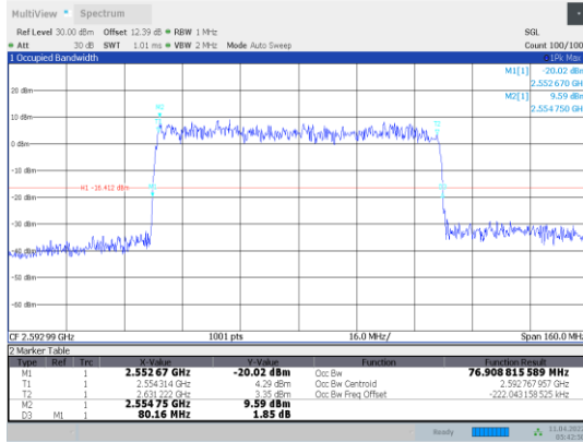
1-N41-PC3-30-80-M-9-DFT-256QAM-Outer_Full-216@0-Ant1-76.909-80.160-≤80-PASS
