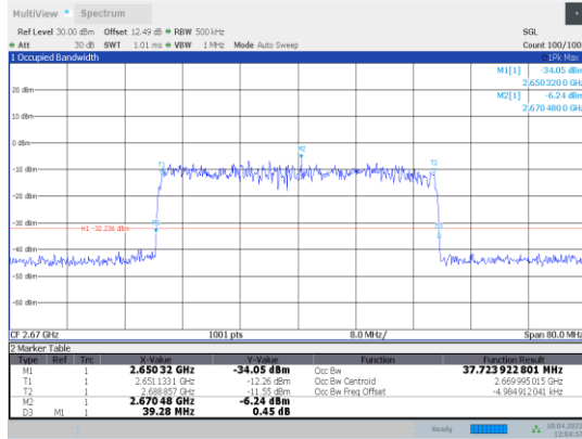
1-N41-PC3-30-40-H-1-DFT-QPSK-Out_ Full-100@0-Ant1-37.711-39.280-≤40-PASS
