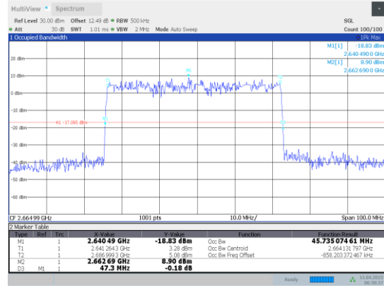
1-N41-PC3-30-50-H-9-DFT-256QAM-Outer_Full-128@0-Ant1-45.735-47.300-≤50-PASS
