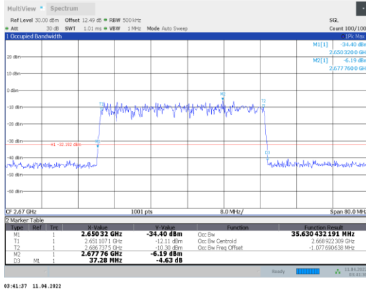
1-N41-PC3-30-40-H-7-CP-64QAM-Outer_Full-106@0-A nt1-35.63-37.280-≤40-PASS
