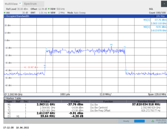
1-N41-PC3-30-60-M-5-CP-QPSK-Outer_Full-162@0-An t1-57.82-59.640-≤60-PASS
