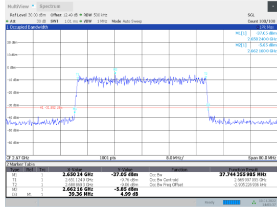
1-N41-PC3-30-40-H-2-DFT-PI2BPSK-Out_ Full-106@0-Ant1-37.772-39.360-≤40-PASS
