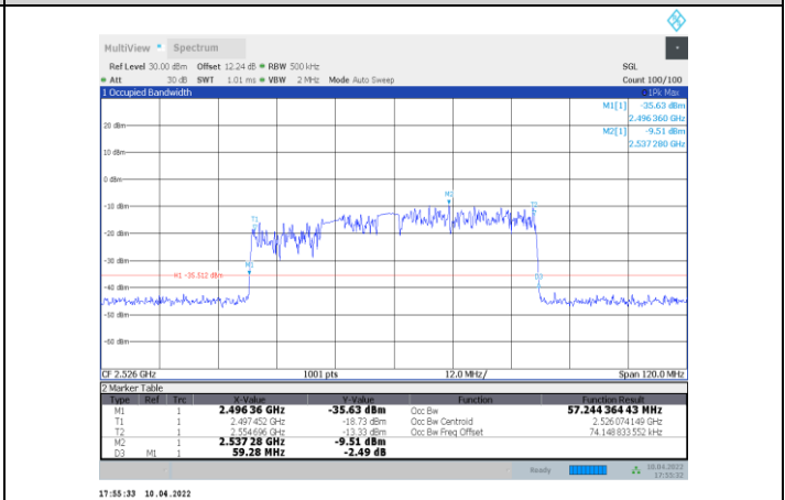
1-N41-PC3-30-60-L-6-CP-16QAM-Outter_Full-162@0-Ant1-57.244-59.280-≤60-PASS
