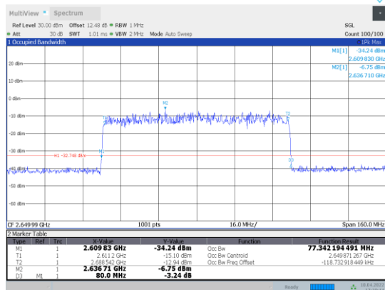
1-N41-PC3-30-80-H-5-CP-QPSK-Outer_Full-217@0-Ant1-77.342-80.000-≤80-PASS
