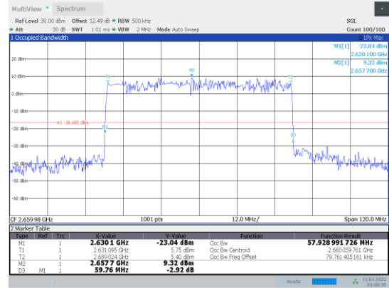
1-N41-PC3-30-60-H-8-CP-256QAM-Outer_Full-162@0- Ant1-57.929-59.760-≤60-PASS
