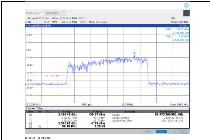
1-N41-PC3-30-60-L-1-DFT-QPSK-Outter_Full-162@0-Ant1-56.973-59.280-≤60-PASS
