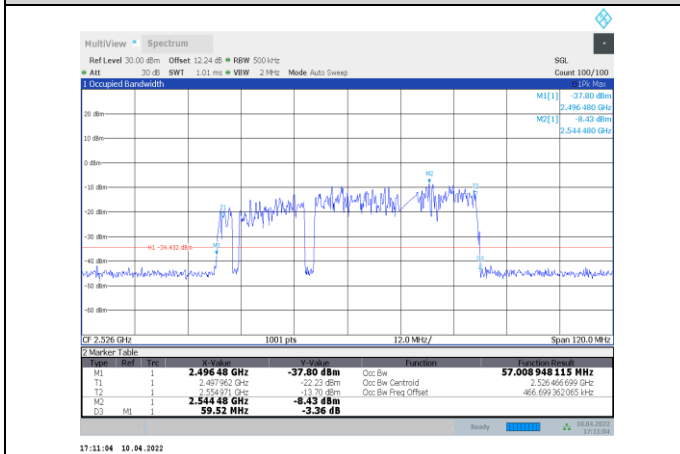
1-N41-PC3-30-60-L-5-CP-QPSK-Outter_Full-162@0-Ant1-57.009-59.520-≤60-PASS
