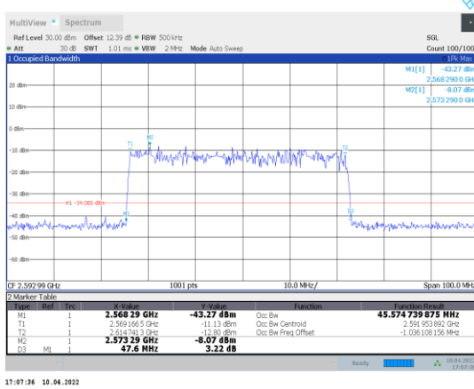
1-N41-PC3-30-50-M-5-CP-QPSK-Outer_Full-133@0-Ant1-45.575-47.600-≤50-PASS
