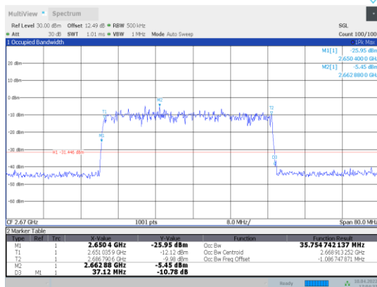
1-N41-PC3-30-40-H-5-CP-QPSK-Out_ Full-106@0-Ant1-35.701-37.120-≤40-PASS
