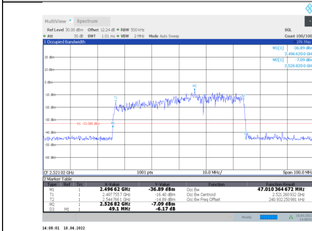
1-N41-PC3-30-50-L-2-DFT-PI2BPSK-Outter_Full-133@0-A Ant1-47.01-49.100-≤50-PASS
