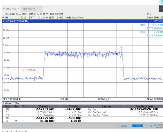
1-N41-PC3-30-40-M-2-DFT-PI2BPSK-Outer_Full-106@0-A Ant1-37.854-39.280-≤40-PASS
