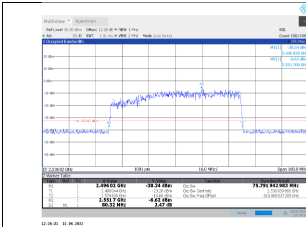
1-N41-PC3-30-80-L-1-DFT-QPSK-Outer_Full-216@0-A nt1-75.792-80.320-≤80-PASS
