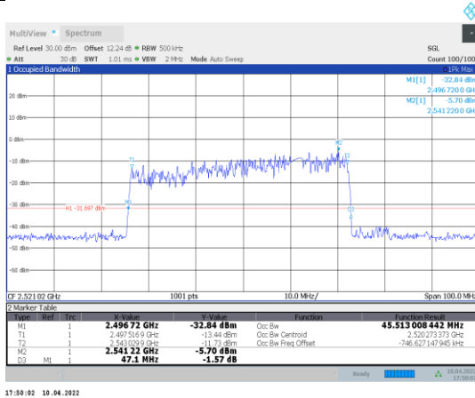
1-N41-PC3-30-50-L-6-CP-16QAM-Outer_Full-133@0-A Ant1-45.513-47.100-≤50-PASS
