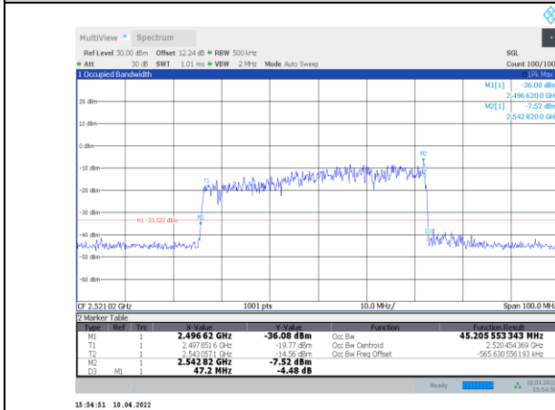
1-N41-PC3-30-50-L-4-DFT-64QAM-Outter_Full-128@0-A Ant1-45.206-47.200-≤50-PASS
