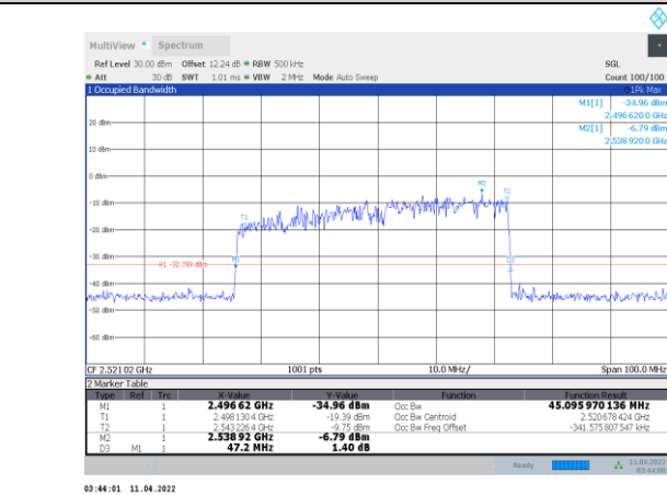
1-N41-PC3-30-50-L-7-CP-64QAM-Outter_Full-133@0-A nt1-45.096-47.200-≤50-PASS
