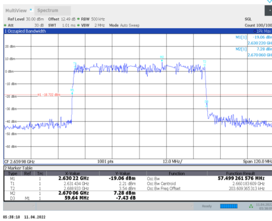
1-N41-PC3-30-60-H-9-DFT-256QAM-Outer_Full-162@0 -Ant1-57.499-59.640-≤60-PASS
