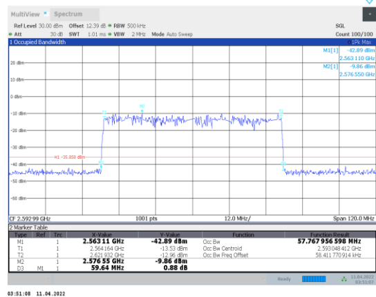
1-N41-PC3-30-60-M-7-CP-64QAM-Outer_Full-162@0-A nt1-57.768-59.640-≤60-PASS
