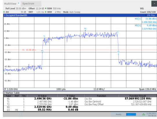
1-N41-PC3-30-60-L-8-CP-256QAM-Outer_Full-162@0-A Ant1-57.07-59.520-≤60-PASS
