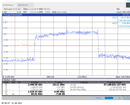
1-N41-PC3-30-60-L-9-DFT-256QAM-Outer_Full-162@0-A Ant1-57.189-59.520-≤60-PASS
