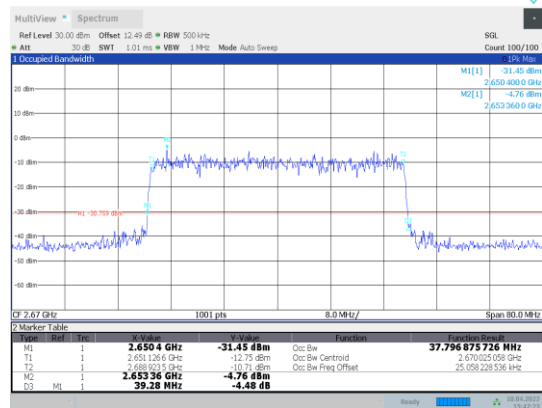
1-N41-PC3-30-40-H-4-DFT-64QAM-Out_ Full-100@0-Ant1-37.829-39.280-≤40-PASS
