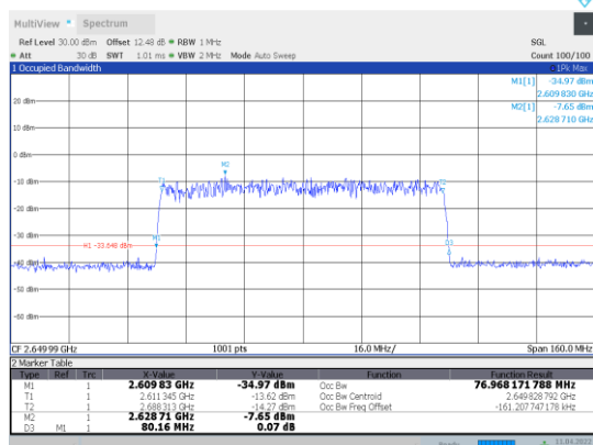
1-N41-PC3-30-80-H-7-CP-64QAM-Outer_Full-217@0-Ant1-76.968-80.160-≤80-PASS
