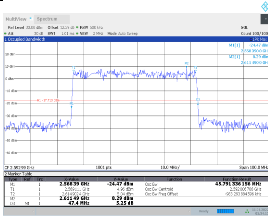
1-N41-PC3-30-50-M-9-DFT-256QAM-Outer_Full-128@0-Ant1-45.791-47.400-≤50-PASS
