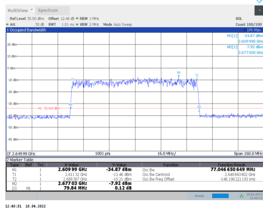
1-N41-PC3-30-80-H-1-DFT-QPSK-Outer_Full-216@0-Ant1-77.047-79.840-≤80-PASS
