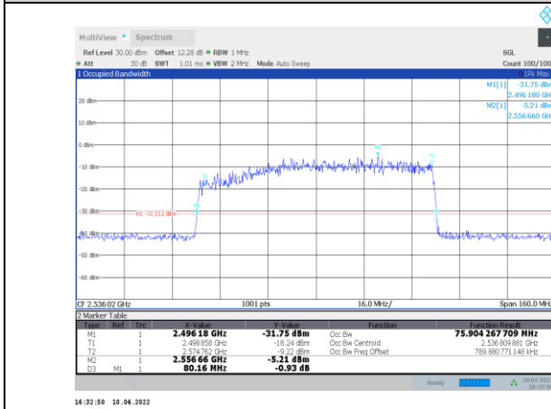
1-N41-PC3-30-80-L-4-DFT-64QAM-Outer_Full-216@0-A nt1-75.904-80.160-≤80-PASS
