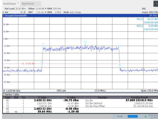
1-N41-PC3-30-60-H-1-DFT-QPSK-Outter_Full-162@0-A nt1-57.889-59.640-≤60-PASS
