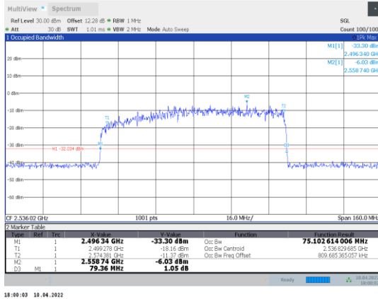
1-N41-PC3-30-80-L-6-CP-16QAM-Outer_Full-217@0-A Ant1-75.103-79.360-≤80-PASS
