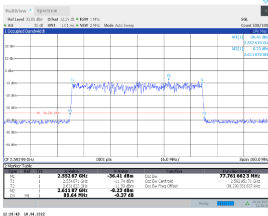
1-N41-PC3-30-80-M-1-DFT-QPSK-Outer_Full-216@0- Ant1-77.762-80.640-≤80-PASS
