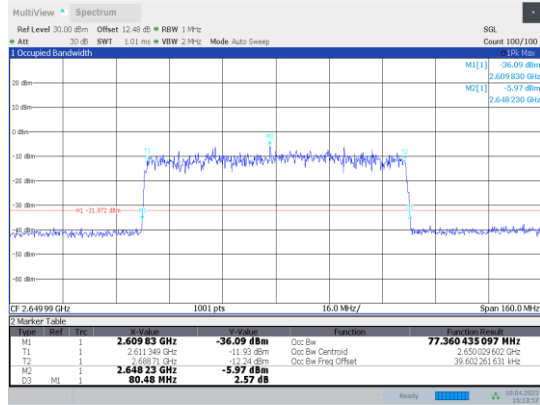
1-N41-PC3-30-80-H-3-DFT-16QAM-Outer_Full-216@0-Ant1-77.36-80.480-≤80-PASS
