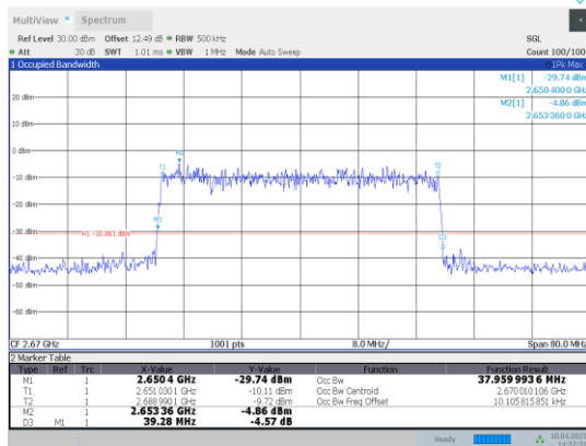
1-N41-PC3-30-40-H-3-DFT-16QAM-Out_ Full-100@0-Ant1-37.946-39.280-≤40-PASS
