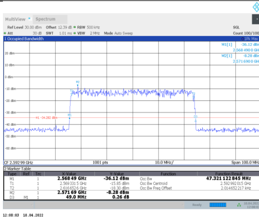
1-N41-PC3-30-50-M-1-DFT-QPSK-Outer_Full-128@0- Ant1-47.321-49.000-≤50-PASS
