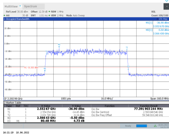
1-N41-PC3-30-80-M-2-DFT-PI2BPSK-Outer_Full-217@0- Ant1-77.392-80.480-≤80-PASS
