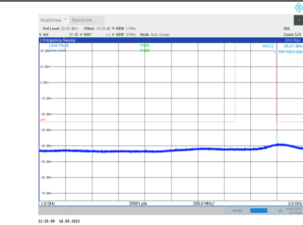
1-N41-PC3-30-100-H-1-CP-OFDM QPSK-Edge_1RB_Left-1 @0-1000-3000-Ant1--38.27--25-PASS
