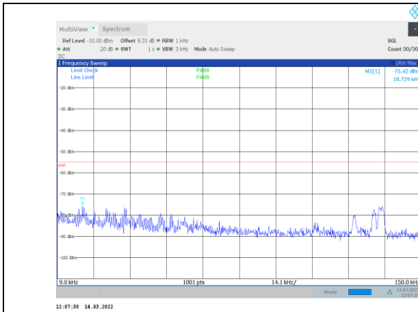
1-N41-PC3-30-100-L-1-CP-OFDM QPSK-Edge_1RB_Left-1 @0-0.009-0.15-Ant1--75.42--55-PASS
