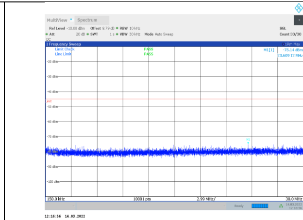
1-N41-PC3-30-100-M-1-CP-OFDM QPSK-Edge_1RB_Left-1 @0.15-30-Ant1--75.14--45-PASS
