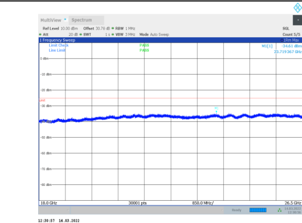
1-N41-PC3-30-100-H-3-CP-OFDM QPSK-Outter_Full-273 @0-18000-26500-Ant1--34.61--25-PASS
