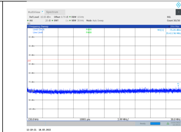
1-N41-PC3-30-100-M-2-CP-OFDM QPSK-Edge_1RB_Right-1 @272-0.15-30-Ant1--75.26--45-PASS
