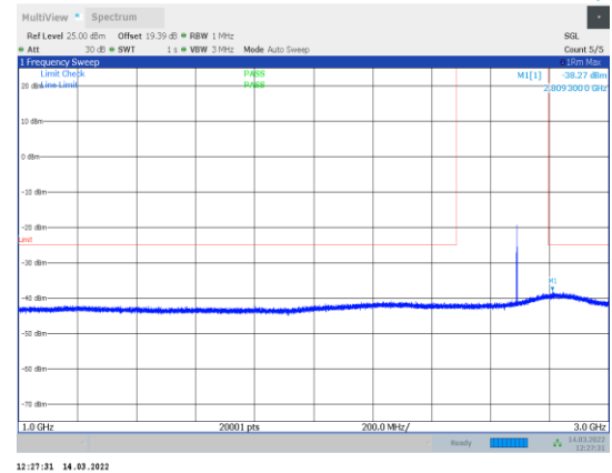
1-N41-PC3-30-100-H-2-CP-OFDM QPSK-Edge_1RB_Right-1 @272-1000-3000-Ant1--38.27--25-PASS
