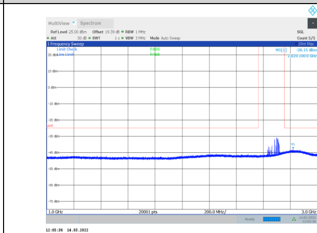
1-N41-PC3-30-60-H-3-CP-OFDM QPSK-Outer_Full-162 @0-1000-3000-Ant1--38.15--25-PASS
