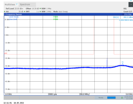
1-N41-PC3-30-100-L-2-CP-OFDM QPSK-Edge_1RB_Right-1 @272-1000-3000-Ant1--38.11--25-PASS
