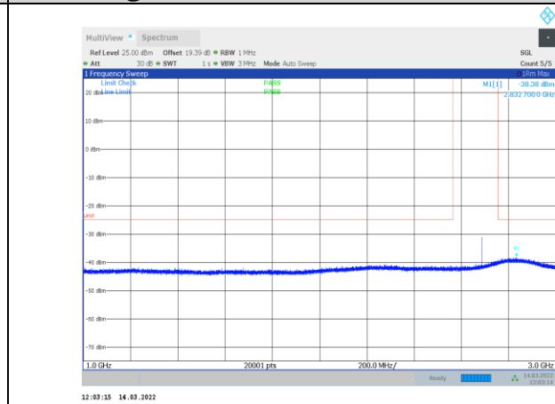
1-N41-PC3-30-60-H-2-CP-OFDM QPSK-Edge_1RB_Right-1 @161-1000-3000-Ant1--38.38--25-PASS
