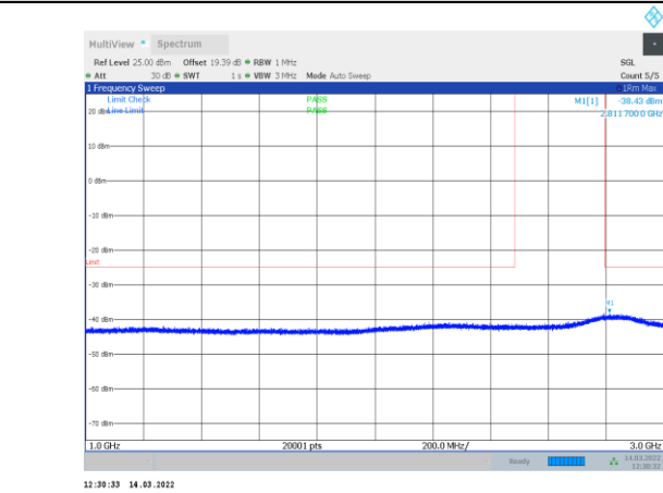
1-N41-PC3-30-100-H-3-CP-OFDM QPSK-Outter_Full-273 @0-1000-3000-Ant1--38.43--25-PASS
