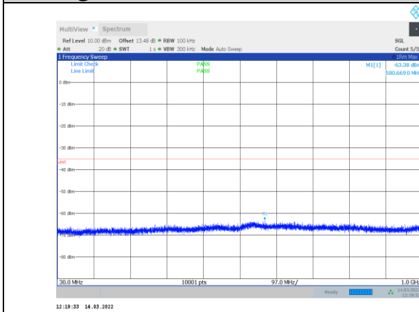
1-N41-PC3-30-100-M-2-CP-OFDM QPSK-Edge_1RB_Right-1 @272-30-1000-Ant1--63.38--35-PASS
