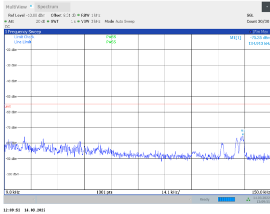
1-N41-PC3-30-100-L-2-CP-OFDM QPSK-Edge_1RB_Right-1 @272-0.009-0.15-Ant1--75.35--55-PASS
