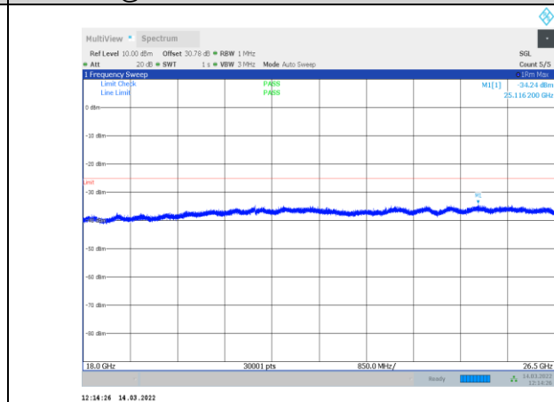
1-N41-PC3-30-100-L-3-CP-OFDM QPSK-Outter_Full-273 @0-18000-26500-Ant1--34.24--25-PASS
