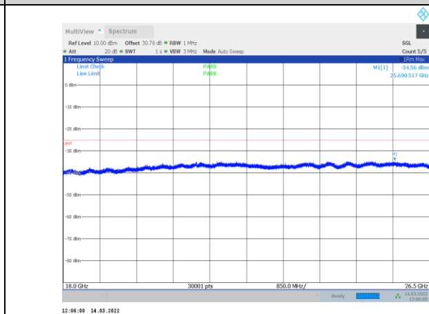
1-N41-PC3-30-60-H-3-CP-OFDM QPSK-Outer_Full-162 @0-18000-26500-Ant1--34.56--25-PASS
