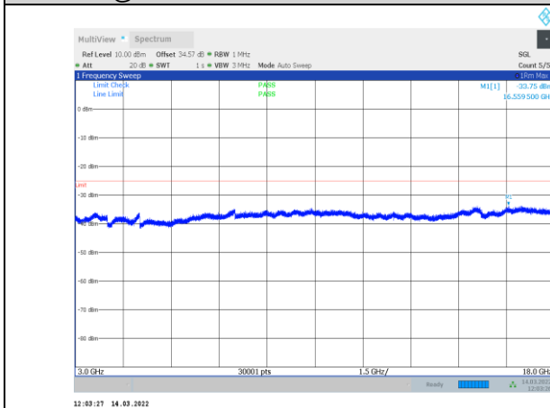
1-N41-PC3-30-60-H-2-CP-OFDM QPSK-Edge_1RB_Right-1 @161-3000-18000-Ant1--33.75--25-PASS
