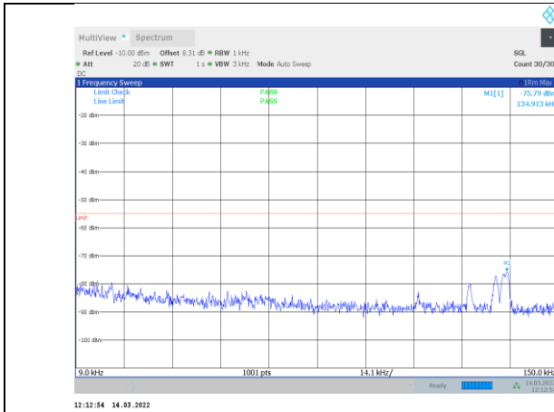
1-N41-PC3-30-100-L-3-CP-OFDM QPSK-Outter_Full-273 @0-0.009-0.15-Ant1--75.79--55-PASS
