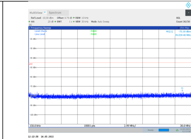
1-N41-PC3-30-100-L-3-CP-OFDM QPSK-Outter_Full-273 @0-0.15-30-Ant1--75.18--45-PASS
