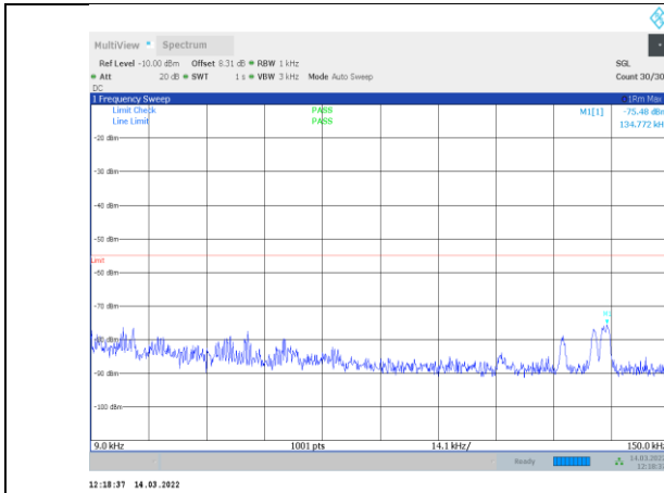
1-N41-PC3-30-100-M-2-CP-OFDM QPSK-Edge_1RB_Right-1 @272-0.009-0.15-Ant1--75.48--55-PASS
