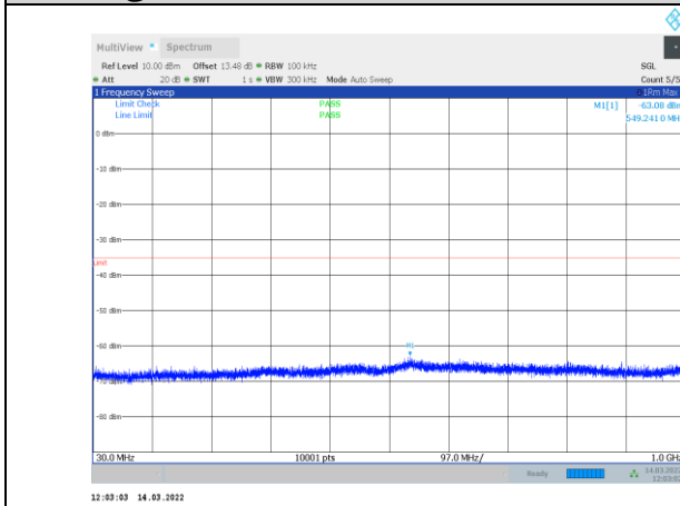
1-N41-PC3-30-60-H-2-CP-OFDM QPSK-Edge_1RB_Right-1 @161-30-1000-Ant1--63.08--35-PASS
