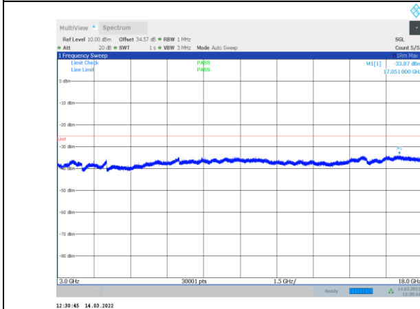
1-N41-PC3-30-100-H-3-CP-OFDM QPSK-Outter_Full-273 @0-3000-18000-Ant1--33.87--25-PASS
