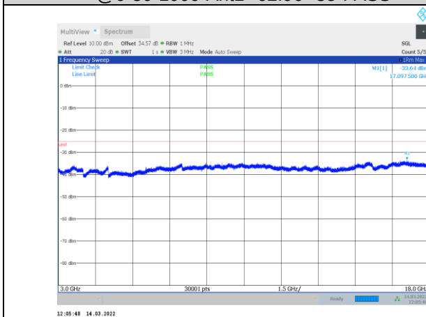
1-N41-PC3-30-60-H-3-CP-OFDM QPSK-Outer_Full-162 @0-3000-18000-Ant1--33.64--25-PASS
