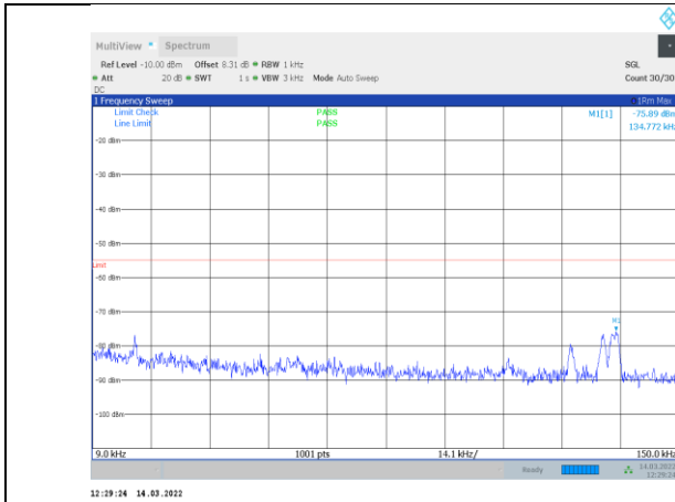
1-N41-PC3-30-100-H-3-CP-OFDM QPSK-Outter_Full-273 @0-0.009-0.15-Ant1--75.89--55-PASS
