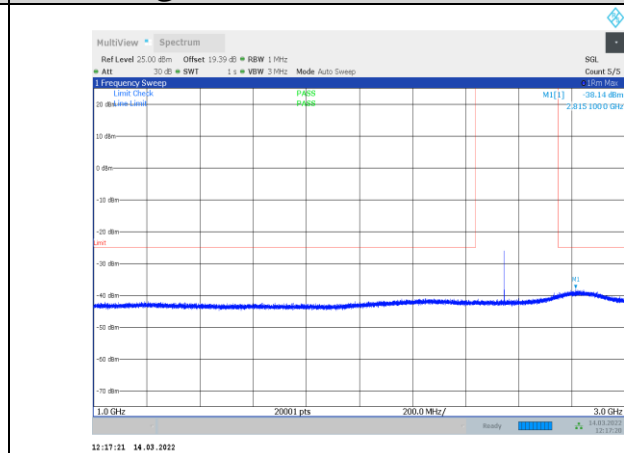
1-N41-PC3-30-100-M-1-CP-OFDM QPSK-Edge_1RB_Left-1 @0-1000-3000-Ant1--38.14--25-PASS
