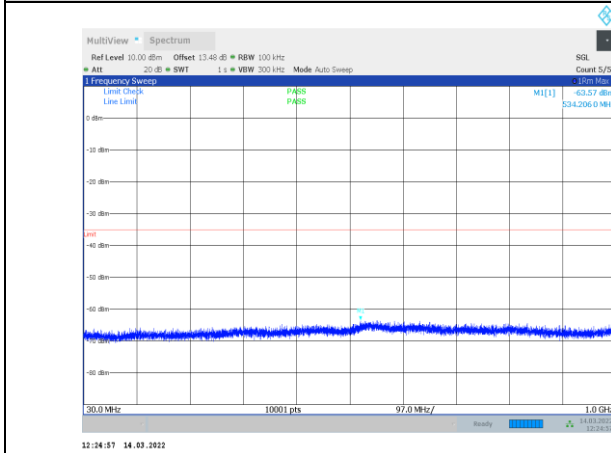
1-N41-PC3-30-100-H-1-CP-OFDM QPSK-Edge_1RB_Left-1 @0-30-1000-Ant1--63.57--35-PASS
