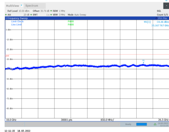
1-N41-PC3-30-100-L-2-CP-OFDM QPSK-Edge_1RB_Right-1 @272-18000-26500-Ant1--34.46--25-PASS
