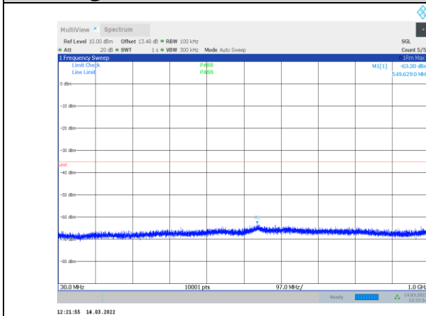
1-N41-PC3-30-100-M-3-CP-OFDM QPSK-Outter_Full-273 @0-30-1000-Ant1--63.30--35-PASS
