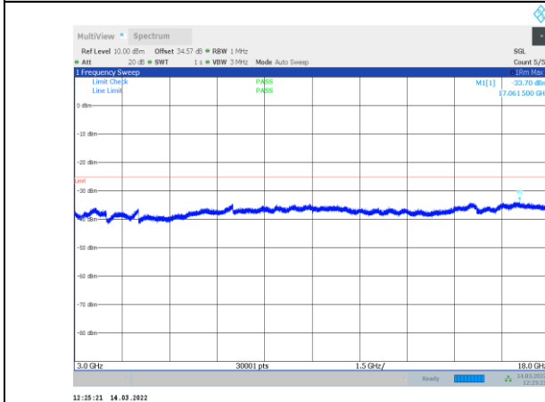
1-N41-PC3-30-100-H-1-CP-OFDM QPSK-Edge_1RB_Left-1 @0-3000-18000-Ant1--33.70--25-PASS
