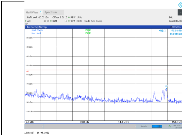
1-N41-PC3-30-60-H-2-CP-OFDM QPSK-Edge_1RB_Right-1 @161-0.009-0.15-Ant1--75.90--55-PASS
