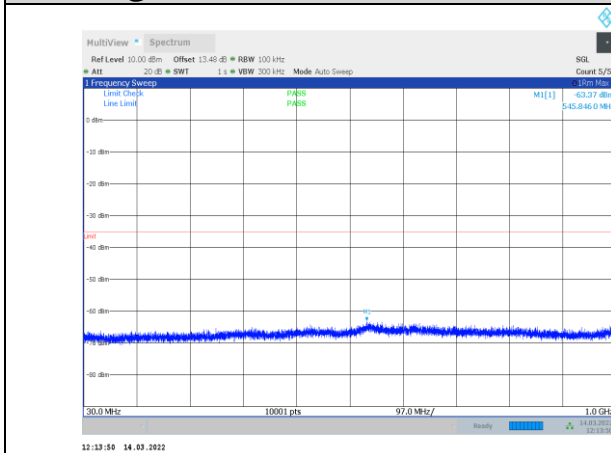
1-N41-PC3-30-100-L-3-CP-OFDM QPSK-Outter_Full-273 @0-30-1000-Ant1--63.37--35-PASS
