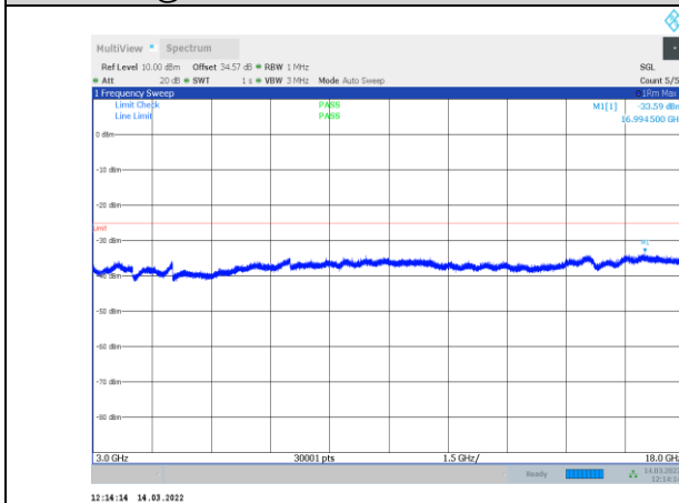
1-N41-PC3-30-100-L-3-CP-OFDM QPSK-Outter_Full-273 @0-3000-18000-Ant1--33.59--25-PASS
