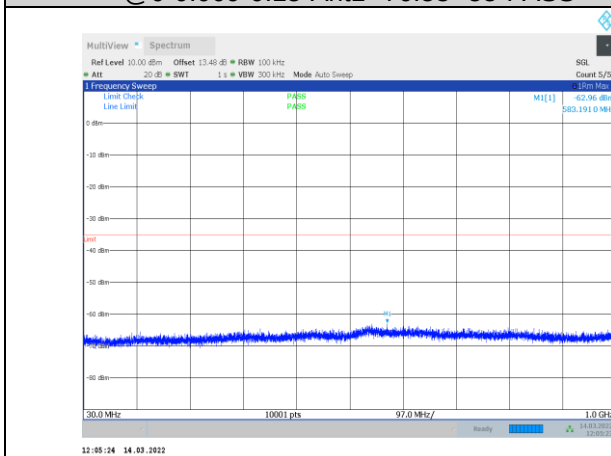
1-N41-PC3-30-60-H-3-CP-OFDM QPSK-Outer_Full-162 @0-30-1000-Ant1--62.96--35-PASS
