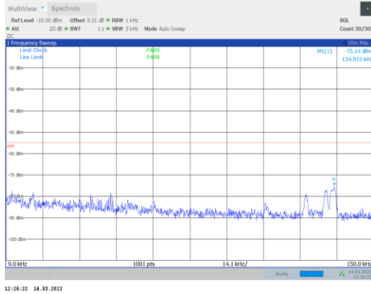
1-N41-PC3-30-100-H-2-CP-OFDM QPSK-Edge_1RB_Right-1 @272-0.009-0.15-Ant1--75.14--55-PASS
