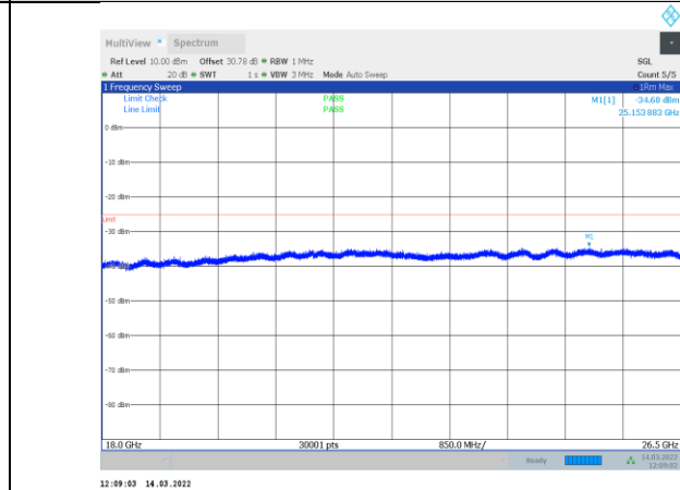
1-N41-PC3-30-100-L-1-CP-OFDM QPSK-Edge_1RB_Left-1 @0-18000-26500-Ant1--34.68--25-PASS
