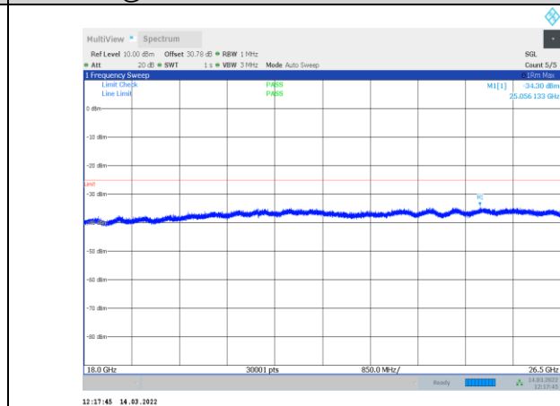
1-N41-PC3-30-100-M-1-CP-OFDM QPSK-Edge_1RB_Left-1 @0-18000-26500-Ant1--34.30--25-PASS
