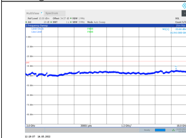
1-N41-PC3-30-100-M-2-CP-OFDM QPSK-Edge_1RB_Right-1 @272-3000-18000-Ant1--33.66--25-PASS
