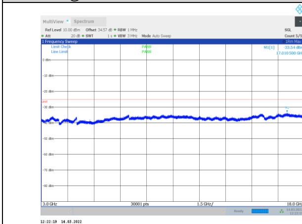
1-N41-PC3-30-100-M-3-CP-OFDM QPSK-Outter_Full-273 @0-3000-18000-Ant1--33.54--25-PASS
