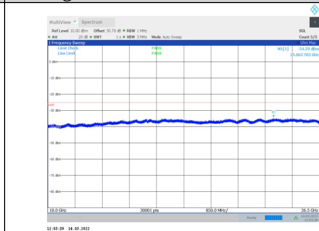
1-N41-PC3-30-60-H-2-CP-OFDM QPSK-Edge_1RB_Right-1 @161-18000-26500-Ant1--34.29--25-PASS
