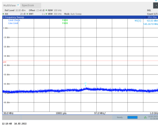
1-N41-PC3-30-100-L-2-CP-OFDM QPSK-Edge_1RB_Right-1 @272-30-1000-Ant1--62.52--35-PASS
