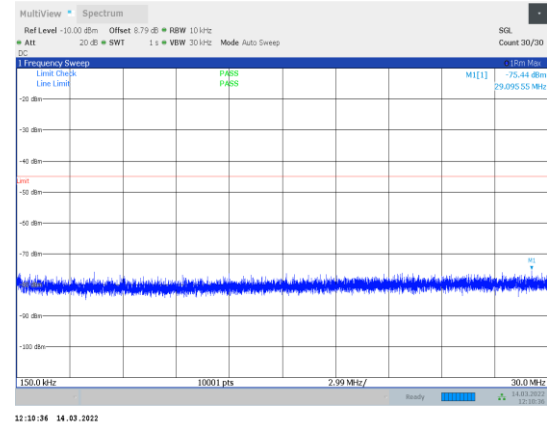
1-N41-PC3-30-100-L-2-CP-OFDM QPSK-Edge_1RB_Right-1 @272-0.15-30-Ant1--75.44--45-PASS
