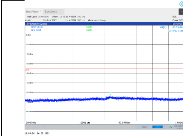
1-N41-PC3-30-100-L-1-CP-OFDM QPSK-Edge_1RB_Left-1 @0-30-1000-Ant1--63.25--35-PASS
