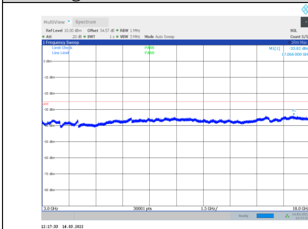
1-N41-PC3-30-100-M-1-CP-OFDM QPSK-Edge_1RB_Left-1 @0-3000-18000-Ant1--33.82--25-PASS
