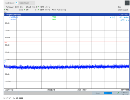
1-N41-PC3-30-100-H-2-CP-OFDM QPSK-Edge_1RB_Right-1 @272-0.15-30-Ant1--75.14--45-PASS
