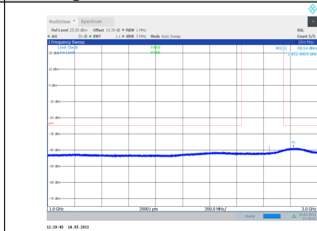
1-N41-PC3-30-100-M-2-CP-OFDM QPSK-Edge_1RB_Right-1 @272-1000-3000-Ant1--38.54--25-PASS
