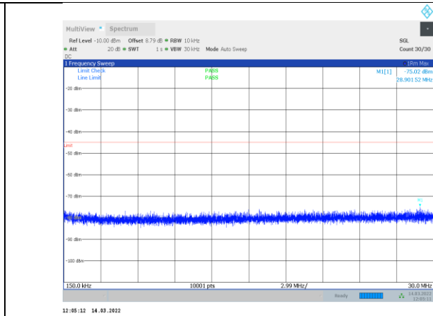
1-N41-PC3-30-60-H-3-CP-OFDM QPSK-Outer_Full-162 @0-0.15-30-Ant1--75.02--45-PASS
