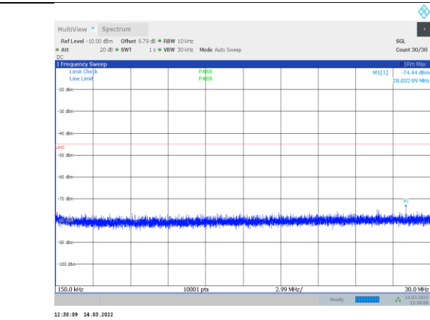
1-N41-PC3-30-100-H-3-CP-OFDM QPSK-Outter_Full-273 @0-0.15-30-Ant1--74.44--45-PASS
