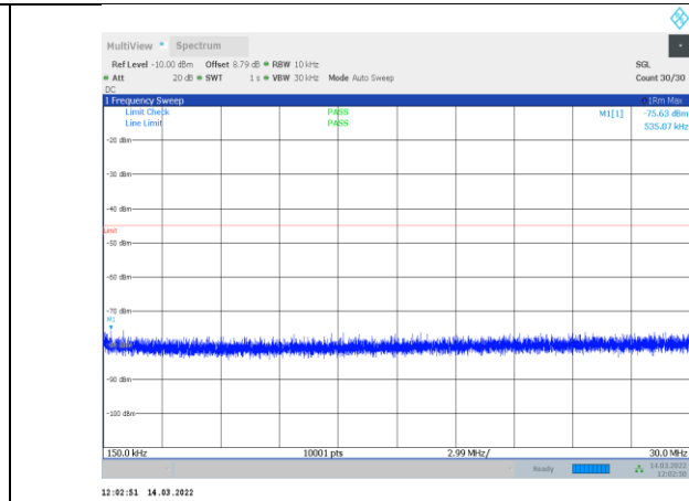
1-N41-PC3-30-60-H-2-CP-OFDM QPSK-Edge_1RB_Right-1 @161-0.15-30-Ant1--75.63--45-PASS
