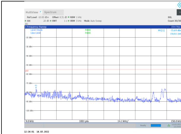
1-N41-PC3-30-100-H-1-CP-OFDM QPSK-Edge_1RB_Left-1 @0-0.009-0.15-Ant1--75.69--55-PASS
