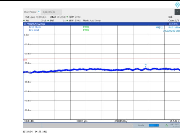
1-N41-PC3-30-100-H-1-CP-OFDM QPSK-Edge_1RB_Left-1 @0-18000-26500-Ant1--34.61--25-PASS
