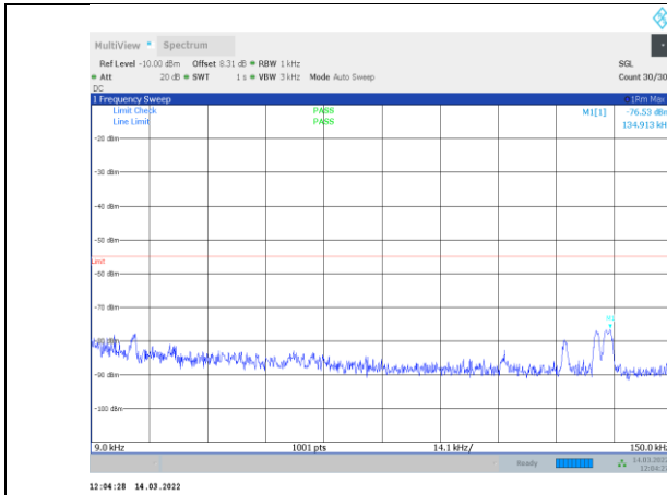
1-N41-PC3-30-60-H-3-CP-OFDM QPSK-Outer_Full-162 @0-0.009-0.15-Ant1--76.53--55-PASS
