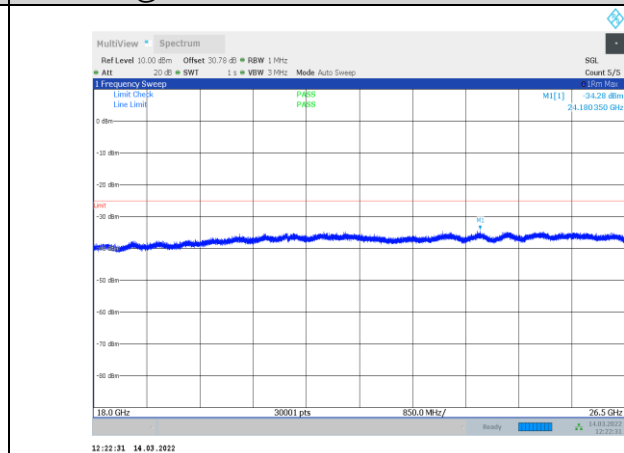
1-N41-PC3-30-100-M-3-CP-OFDM QPSK-Outter_Full-273 @0-18000-26500-Ant1--34.28--25-PASS
