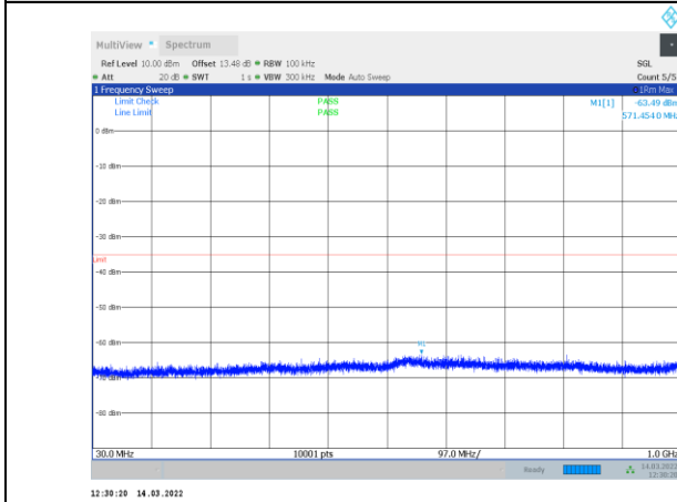
1-N41-PC3-30-100-H-3-CP-OFDM QPSK-Outter_Full-273 @0-30-1000-Ant1--63.49--35-PASS
