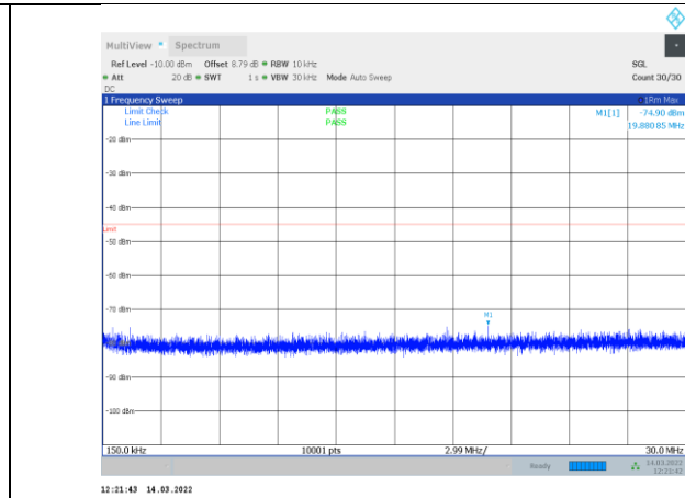
1-N41-PC3-30-100-M-3-CP-OFDM QPSK-Outter_Full-273 @0-0.15-30-Ant1--74.90--45-PASS
