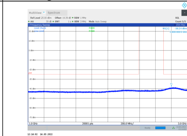
1-N41-PC3-30-100-L-3-CP-OFDM QPSK-Outter_Full-273 @0-1000-3000-Ant1--38.24--25-PASS
