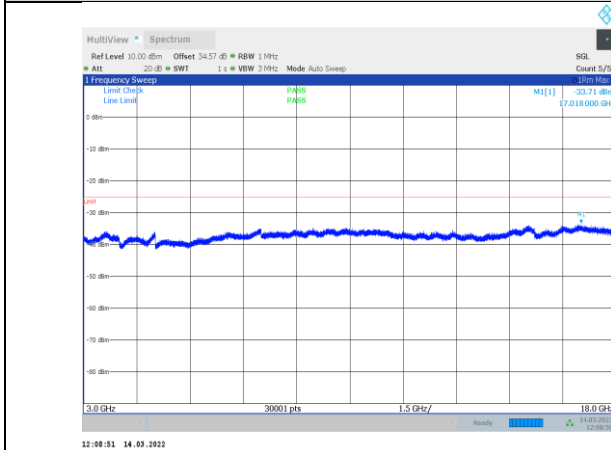
1-N41-PC3-30-100-L-1-CP-OFDM QPSK-Edge_1RB_Left-1 @0-3000-18000-Ant1--33.71--25-PASS
