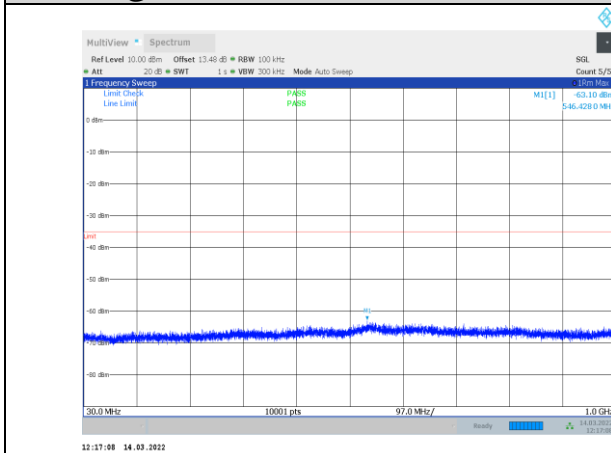
1-N41-PC3-30-100-M-1-CP-OFDM QPSK-Edge_1RB_Left-1 @0-30-1000-Ant1--63.10--35-PASS
