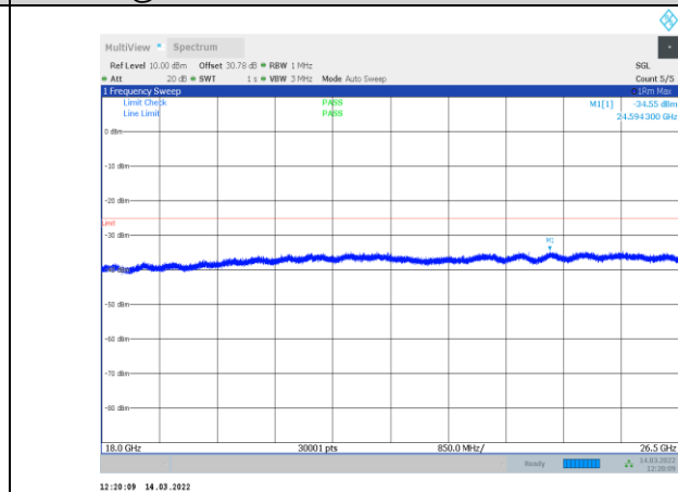
1-N41-PC3-30-100-M-2-CP-OFDM QPSK-Edge_1RB_Right-1 @272-18000-26500-Ant1--34.55--25-PASS
