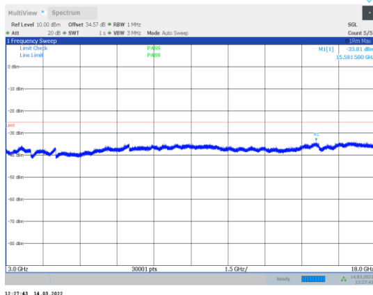
1-N41-PC3-30-100-H-2-CP-OFDM QPSK-Edge_1RB_Right-1 @272-3000-18000-Ant1--33.81--25-PASS
