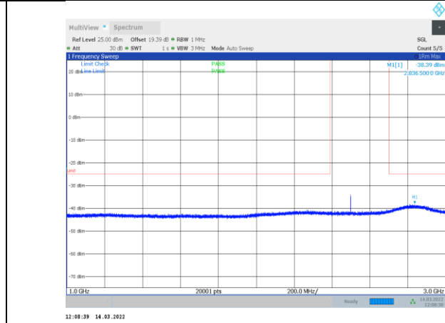
1-N41-PC3-30-100-L-1-CP-OFDM QPSK-Edge_1RB_Left-1 @0-1000-3000-Ant1--38.39--25-PASS
