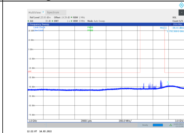
1-N41-PC3-30-100-M-3-CP-OFDM QPSK-Outter_Full-273 @0-1000-3000-Ant1--38.41--25-PASS
