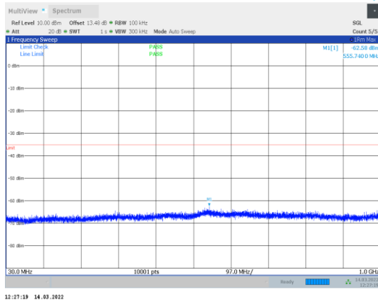
1-N41-PC3-30-100-H-2-CP-OFDM QPSK-Edge_1RB_Right-1 @272-30-1000-Ant1--62.58--35-PASS
