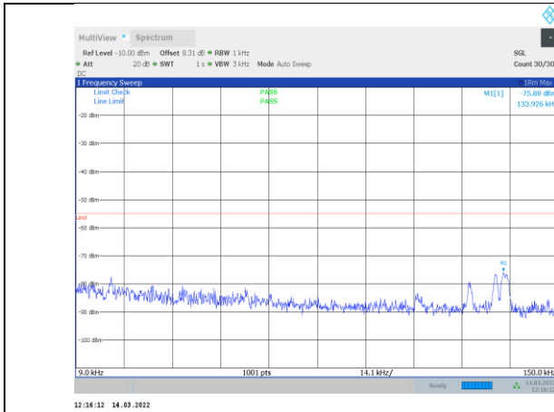
1-N41-PC3-30-100-M-1-CP-OFDM QPSK-Edge_1RB_Left-1 @0-0.009-0.15-Ant1--75.88--55-PASS
