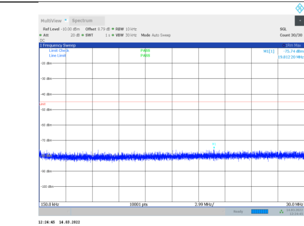
1-N41-PC3-30-100-H-1-CP-OFDM QPSK-Edge_1RB_Left-1 @0-0.15-30-Ant1--75.74--45-PASS
