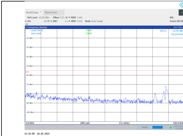
1-N41-PC3-30-100-M-3-CP-OFDM QPSK-Outter_Full-273 @0-0.009-0.15-Ant1--75.95--55-PASS
