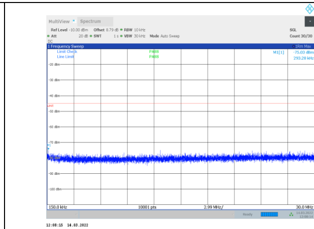
1-N41-PC3-30-100-L-1-CP-OFDM QPSK-Edge_1RB_Left-1 @0.15-30-Ant1--75.03--45-PASS
