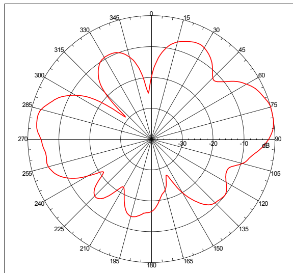
S5703BH 5.875 Ghz E Plane
