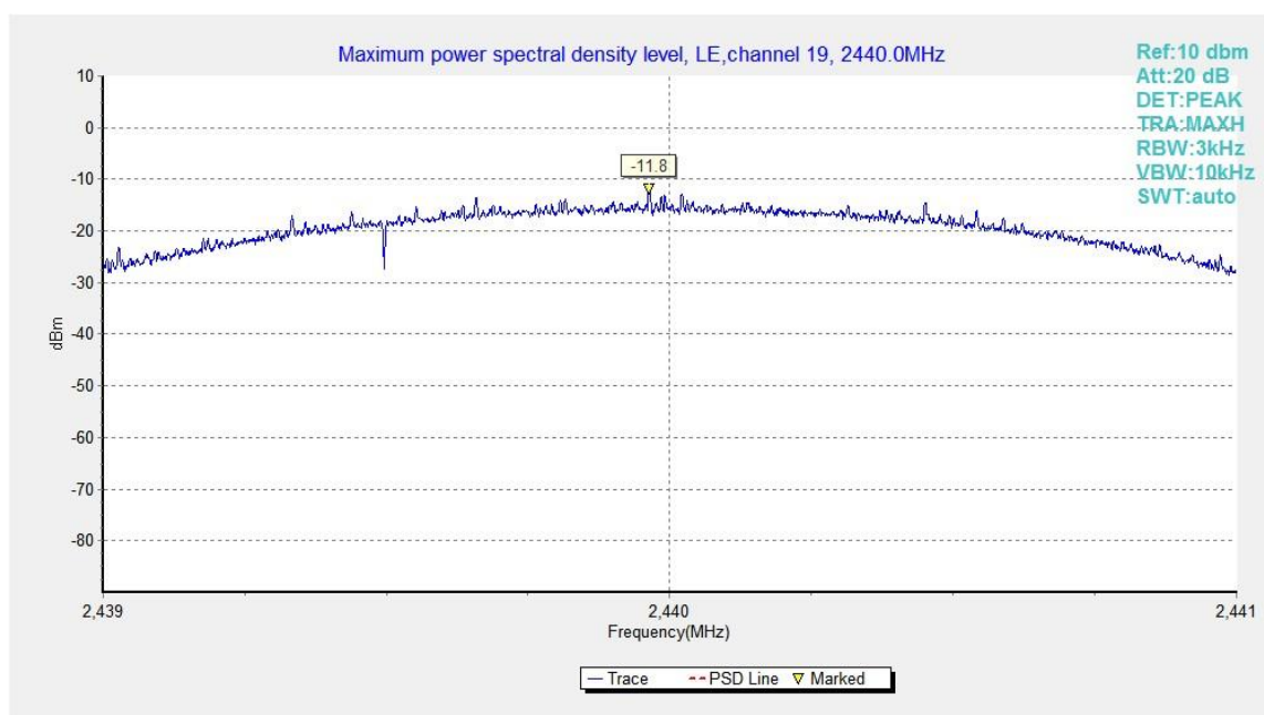
Fig.22. Maximum Power Spectral Density Level Function: GFSK, 2440 MHz
