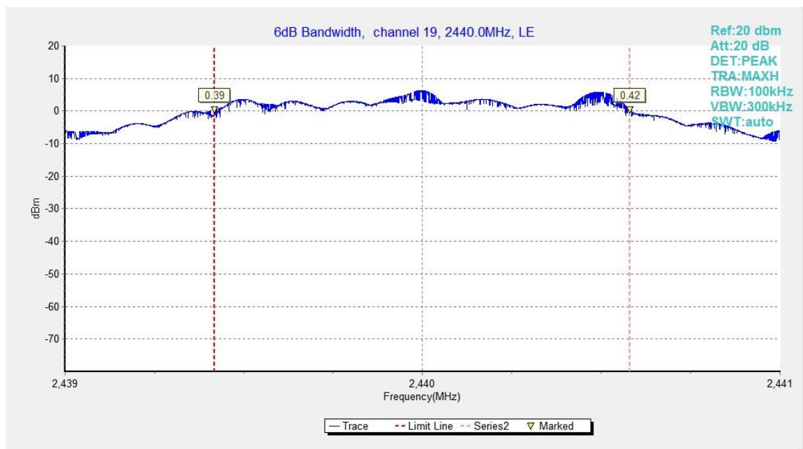
Fig.19. 6dB Bandwidth: GFSK, 2440 MHz
