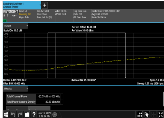
N41(60M)_DFT-s- OFDM_QPSK_Edge_1RB_Left_Low_CH_CHP_PASS
