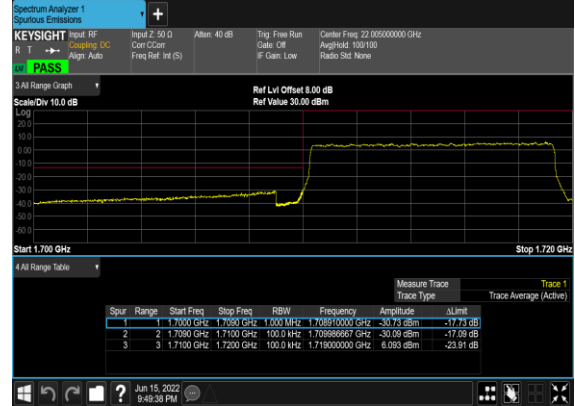
N66(10M)_DFT-s- OFDM_BPSK_Outer_Full_Low_CH
