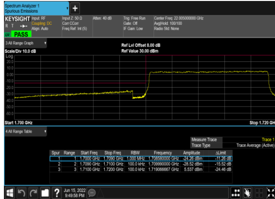
N66(10M)_DFT-s- OFDM_QPSK_Outer_Full_Low_CH
