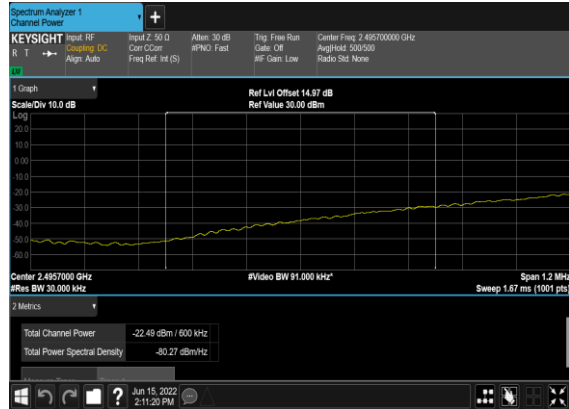
N41(60M)_DFT-s- OFDM_BPSK_Edge_1RB_Left_Low_CH_CHP_PASS
