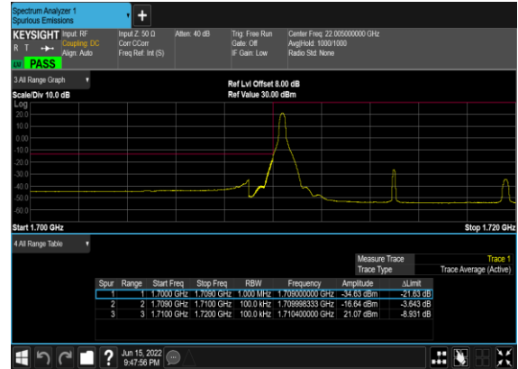
N66(10M)_DFT-s- OFDM_BPSK_Edge_1RB_Left_Low_CH
