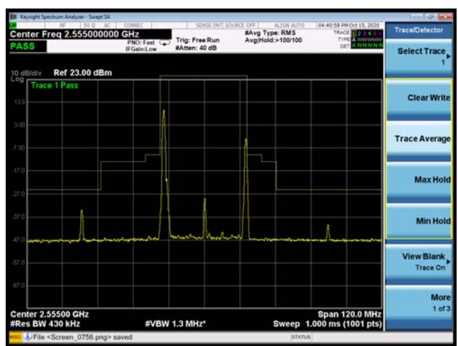
CA_7C 64QAM 20MHz+10MHz CH-High, 1 RB
