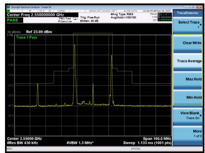
CA_7C QPSK 20MHz+20MHz CH-High, 100%RB
