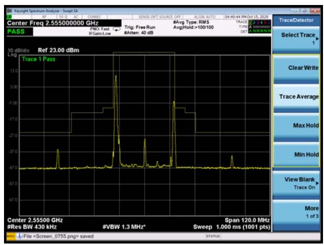
CA_7C 16QAM 20MHz+10MHz CH-High, 1 RB
