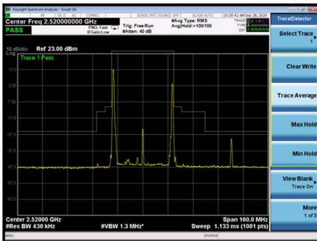
CA_7C QPSK 20MHz+20MHz CH-Low, 100%RB
