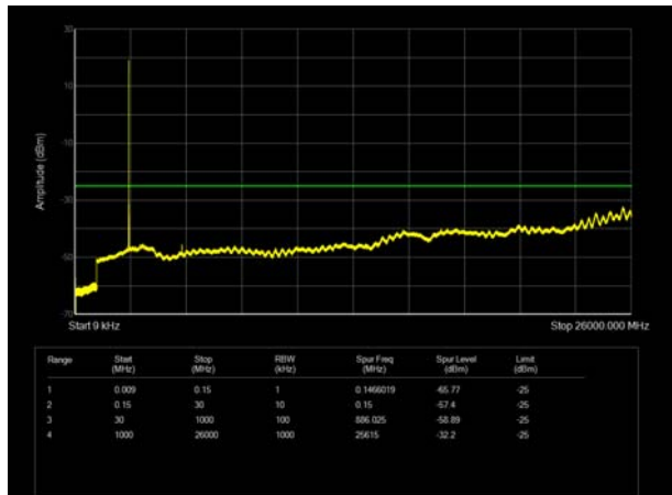
LTE Band 41 15MHz CH- Middle 9kHz~26GHz
