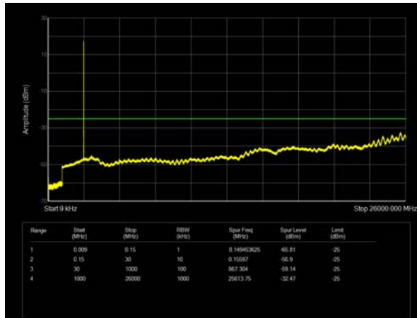
LTE Band 38 5MHz CH- Middle 9kHz~26GHz
