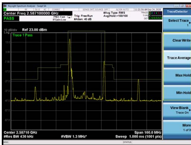
CA_41C 64QAM 20MHz+5MHz CH-Low, 1 RB
