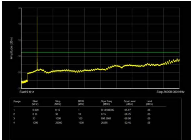
LTE Band 41 15MHz CH-High 9kHz~26GHz
