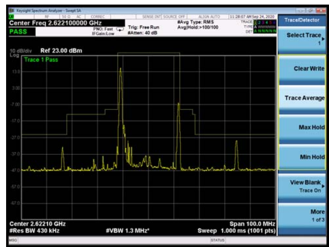
CA_41C 16QAM 20MHz+5MHz CH-High, 100%RB
