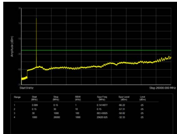
LTE Band 38 10MHz CH- High 9kHz~26GHz
