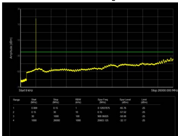
LTE Band 38 5MHz CH-High 9kHz~26GHz
