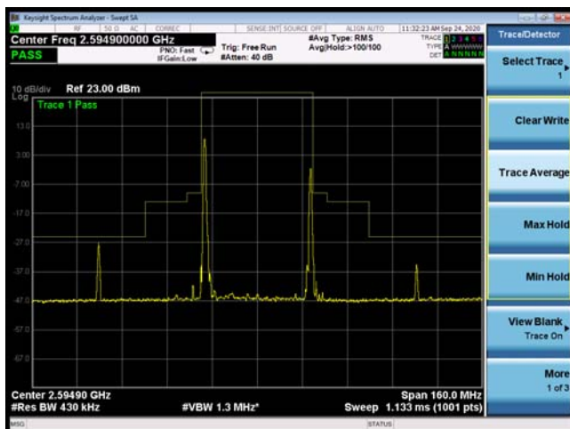
CA_41C 64QAM 20MHz+20MHz CH-Low, 1 RB
