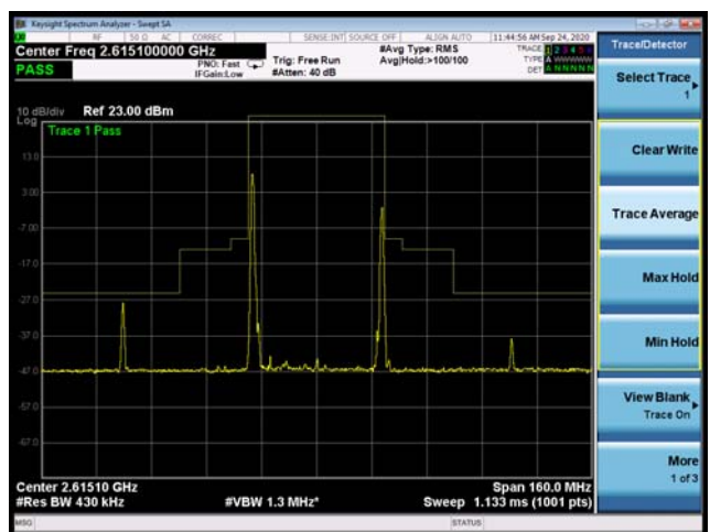
CA_41C 64QAM 20MHz+20MHz CH-High, 1 RB
