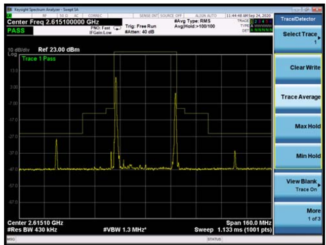
CA_41C 16QAM 20MHz+20MHz CH-High, 100%RB
