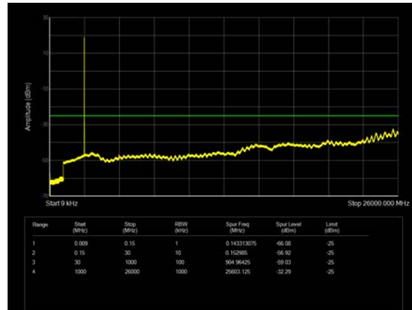
LTE Band 38 10MHz CH- Middle 9kHz~26GHz
