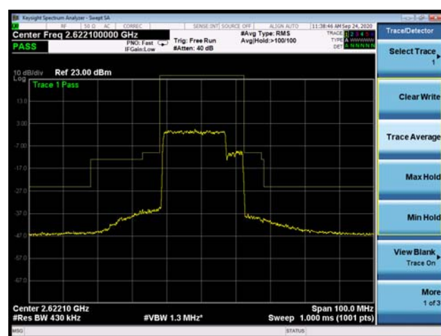
CA_41C QPSK 20MHz+20MHz CH-High, 1 RB
