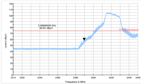
802.11g-Channel 3 Peak
