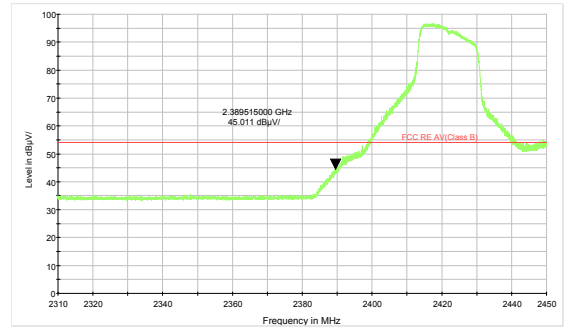
802.11g-Channel 3 Average
