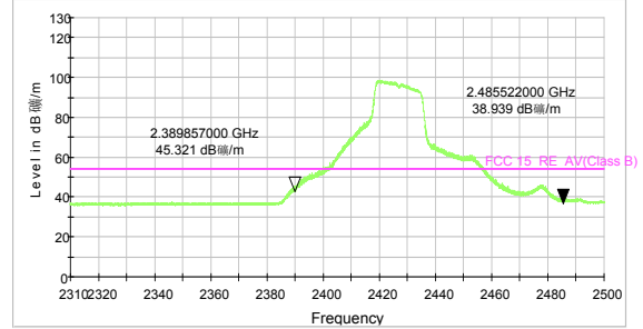
802.11g-Channel 4 Average
