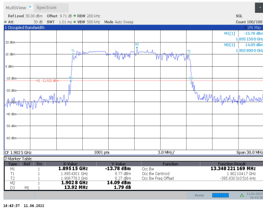
1-N2-PC3-15-15-H-7-DFT-16QAM-Out_ Full-75@0-Ant1-13.348-13.920-≤15-PASS
