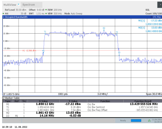
1-N2-PC3-15-15-L-7-DFT-16QAM-Outer_Full-75@0-Ant1-13.43-14.160-≤15-PASS
