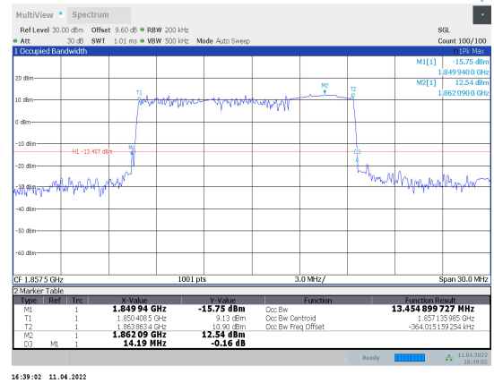
1-N2-PC3-15-15-L-6-DFT-QPSK-Outer_Full-75@0-Ant1-13.455-14.190-≤15-PASS
