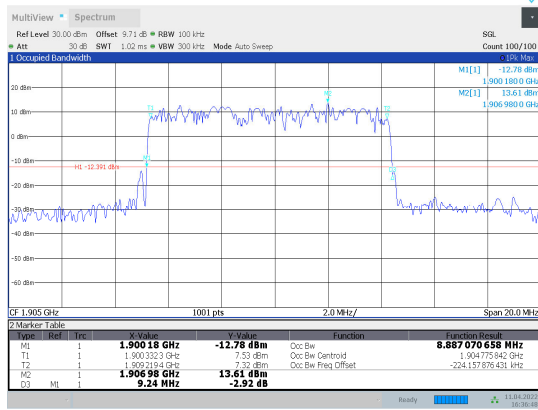
1-N2-PC3-15-10-H-6-DFT-QPSK-Outter_Full-50@0-Ant1-8.887-9.240-≤10-PASS
