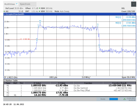
1-N2-PC3-15-15-H-6-DFT-QPSK-Out_ Full-75@0-Ant1-13.46-14.160-≤15-PASS
