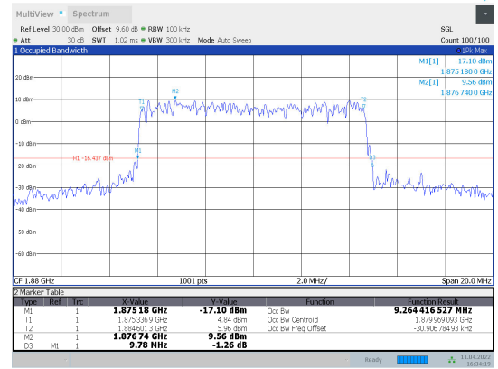
1-N2-PC3-15-10-M-4-CP-256QAM-Outter_Full-52@0-Ant1-9.264-9.780-≤10-PASS
