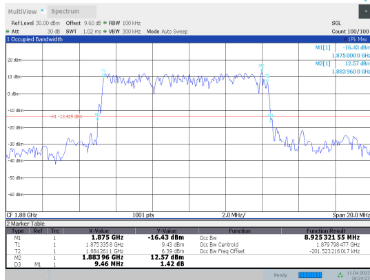
1-N2-PC3-15-10-M-5-DFT-PI/2BPSK-Outter_Full-50@0-Ant1-8.925-9.460-≤10-PASS
