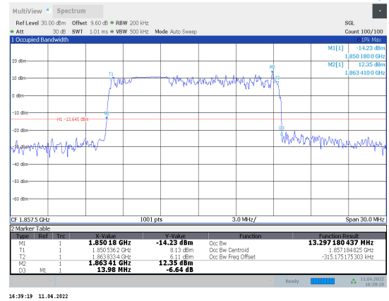
1-N2-PC3-15-15-L-8-DFT-64QAM-Outer_Full-75@0-Ant1-13.297-13.980-≤15-PASS
