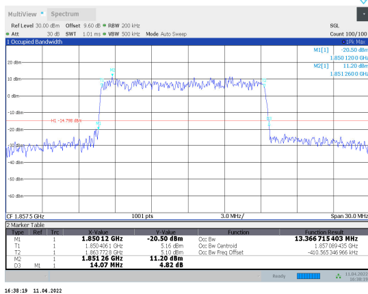
1-N2-PC3-15-15-L-1-CP-QPSK-Outter_Full-75@0-Ant1-13.367-14.070-≤15-PASS
