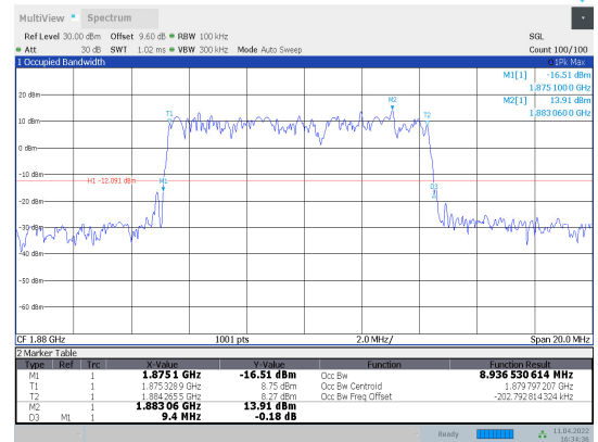
1-N2-PC3-15-10-M-6-DFT-QPSK-Outter_Full-50@0-Ant1-8.937-9.400-≤10-PASS
