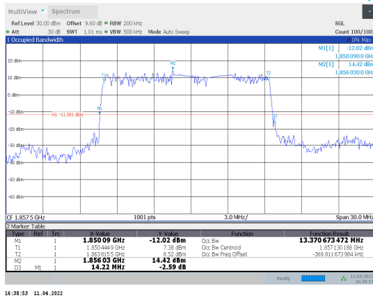
1-N2-PC3-15-15-L-5-DFT-PI/2BPSK-Outer_Full-75@0-Ant1-13.371-14.220-≤15-PASS
