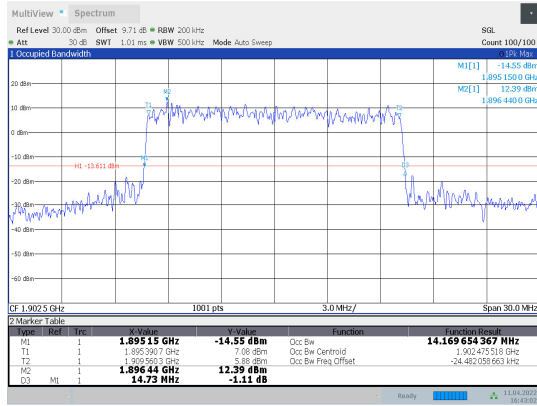
1-N2-PC3-15-15-H-3-CP-64QAM-Out_ Full-79@0-Ant1-14.17-14.730-≤15-PASS
