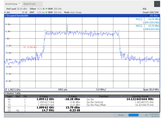
1-N2-PC3-15-15-H-4-CP-256QAM-Out_ Full-79@0-Ant1-14.123-14.700-≤15-PASS
