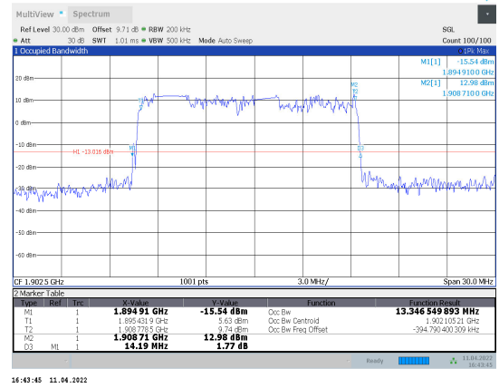
1-N2-PC3-15-15-H-8-DFT-64QAM-Out_ Full-75@0-Ant1-13.347-14.190-≤15-PASS
