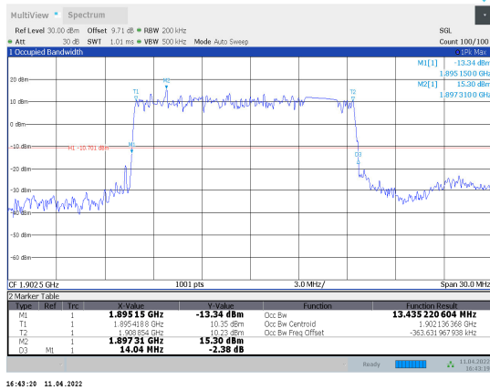
1-N2-PC3-15-15-H-5-DFT-PI/2BPSK-Out_ Full-75@0-Ant1-13.435-14.040-≤15-PASS
