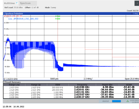
1-N38-PC3-30-10-H-31-CP-64QAM-Outer_Full-24@0-Ant1-PASS-see graph
