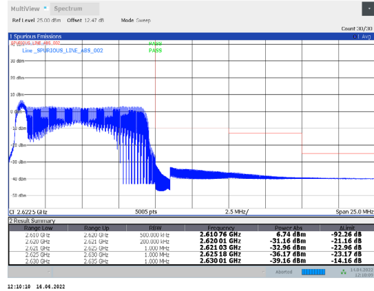
1-N38-PC3-30-10-H-15-DFT-64QAM-Outer_Full-24@0-Ant1-PASS-see graph
