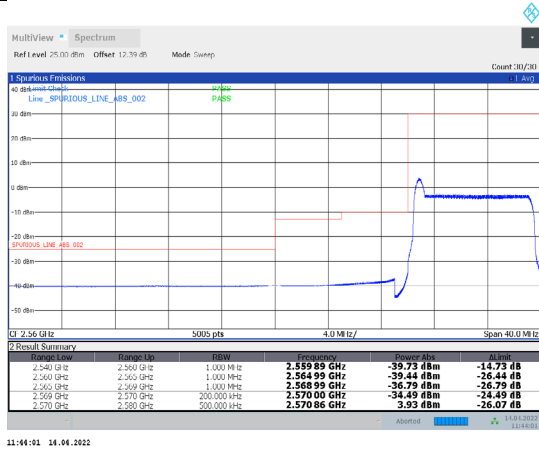
1-N38-PC3-30-10-L-36-CP-256QAM-Inner_Full-12@6-Ant1-PASS-see graph
