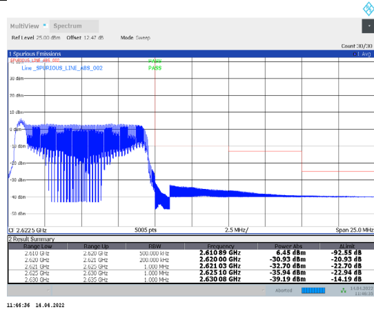
1-N38-PC3-30-10-H-1-DFT-PI/2BPSK-Inner_Full-12@6-Ant1-PASS-see graph
