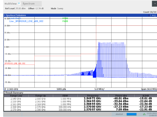
1-N38-PC3-30-20-L-11-DFT-16QAM-Outer_Full-50@0-A nt1-PASS-see graph
