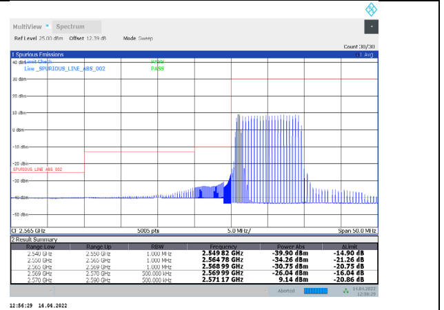
1-N38-PC3-30-20-L-5-DFT-QPSK-Edge_1RB_Left-1@0- Ant1-PASS-see graph
