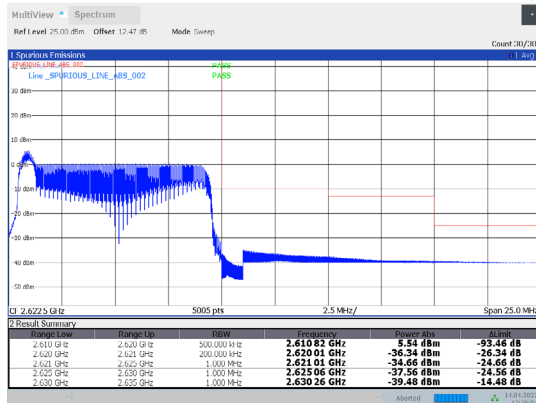
1-N38-PC3-30-10-H-24-CP-QPSK-Inner_Full-12@6-An t1-PASS-see graph
