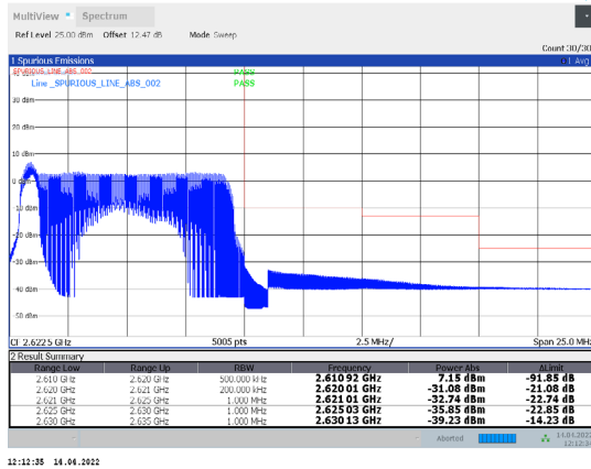
1-N38-PC3-30-10-H-16-DFT-64QAM-Inner_Full-12@6-Ant1-PASS-see graph
