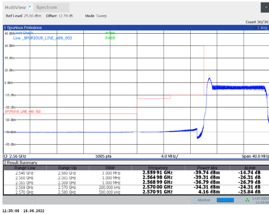
1-N38-PC3-30-10-L-28-CP-16QAM-Inner_Full-12@6-Ant1-PASS-see graph
