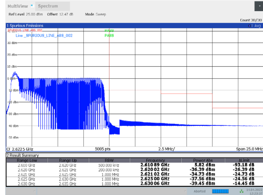
1-N38-PC3-30-10-H-23-CP-QPSK-Outer_Full-24@0-Ant 1-PASS-see graph
