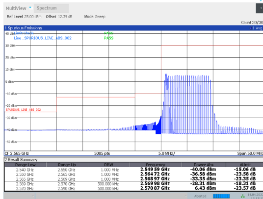
1-N38-PC3-30-20-L-15-DFT-64QAM-Outer_Full-50@0-Ant1-PASS-see graph
