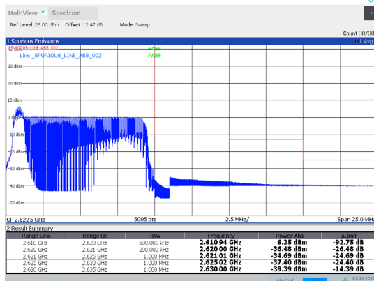
1-N38-PC3-30-10-H-27-CP-16QAM-Outer_Full-24@0-Ant1-PASS-see graph
