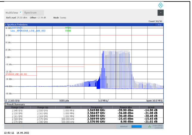
1-N38-PC3-30-20-L-2-DFT-PI/2BPSK-Edge_1RB_Left-1@ 0-Ant1-PASS-see graph
