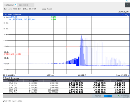
1-N38-PC3-30-20-L-24-CP-QPSK-Inner_Full-25@12-Ant1-PASS-see graph
