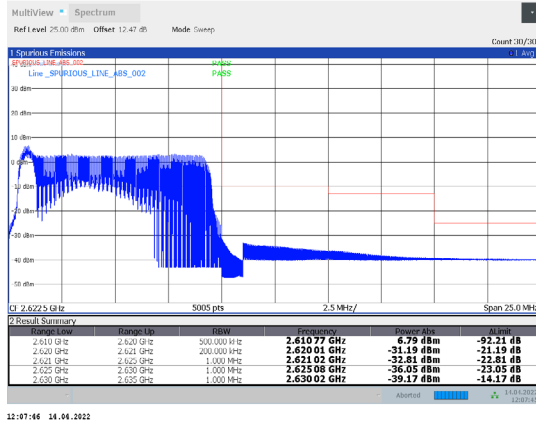
1-N38-PC3-30-10-H-14-DFT-64QAM-Edge_1RB_Right -1@23-Ant1-PASS-see graph
