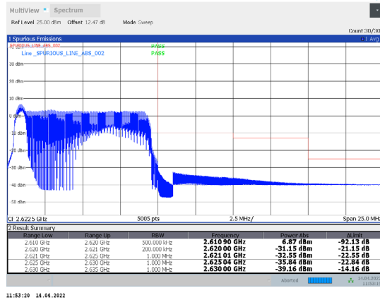
1-N38-PC3-30-10-H-6-DFT-QPSK-Edge_1RB_Right-1 @23-Ant1-PASS-see graph
