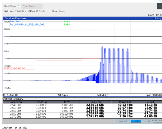
1-N38-PC3-30-20-L-23-CP-QPSK-Outer_Full-51@0-Ant1-PASS-see graph
