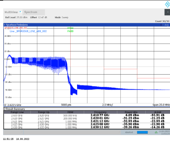
1-N38-PC3-30-10-H-4-DFT-PI/2BPSK-Outer_Full-24@0-Ant1-PASS-see graph
