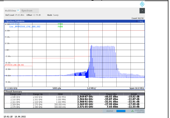
1-N38-PC3-30-20-L-8-DFT-QPSK-Inner_Full-25@12-Ant 1-PASS-see graph
