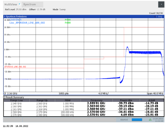
1-N38-PC3-30-10-L-29-CP-64QAM-Edge_1RB_Left-1 @0-Ant1-PASS-see graph
