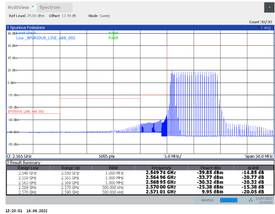
1-N38-PC3-30-20-L-19-DFT-256QAM-Outer_Full-50@ 0-Ant1-PASS-see graph
