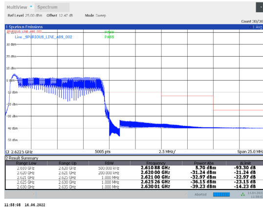
1-N38-PC3-30-10-H-8-DFT-QPSK-Inner_Full-12@6-A nt1-PASS-see graph
