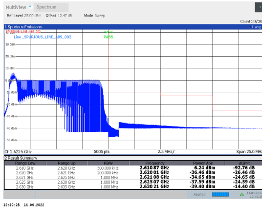
1-N38-PC3-30-10-H-32-CP-64QAM-Inner_Full-12@6-Ant1-PASS-see graph
