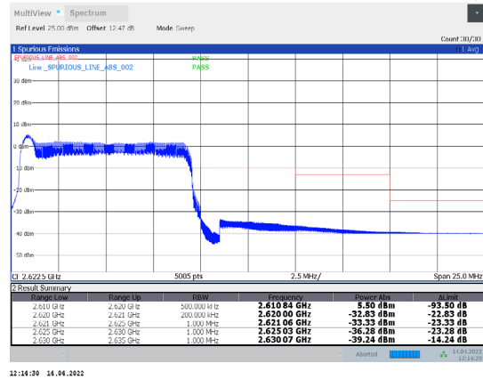
1-N38-PC3-30-10-H-18-DFT-256QAM-Edge_1RB_Right -1@23-Ant1-PASS-see graph
