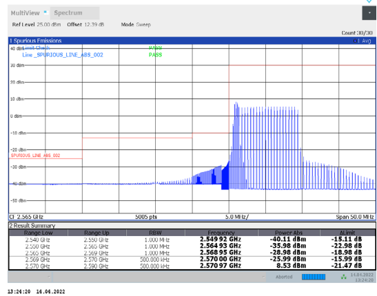
1-N38-PC3-30-20-L-21-CP-QPSK-Edge_1RB_Left-1 @0-Ant1-PASS-see graph
