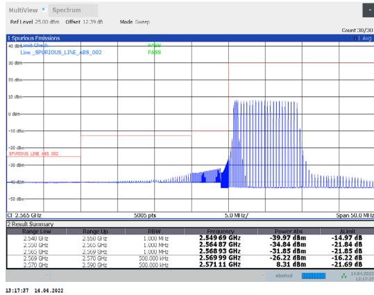
1-N38-PC3-30-20-L-17-DFT-256QAM-Edge_1RB_Left-1 @0-Ant1-PASS-see graph
