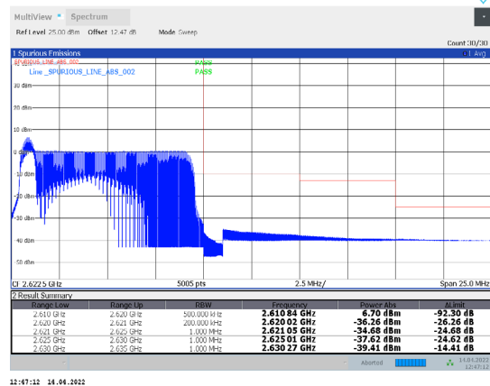
1-N38-PC3-30-10-H-36-CP-256QAM-Inner_Full-12@6-Ant1-PASS-see graph
