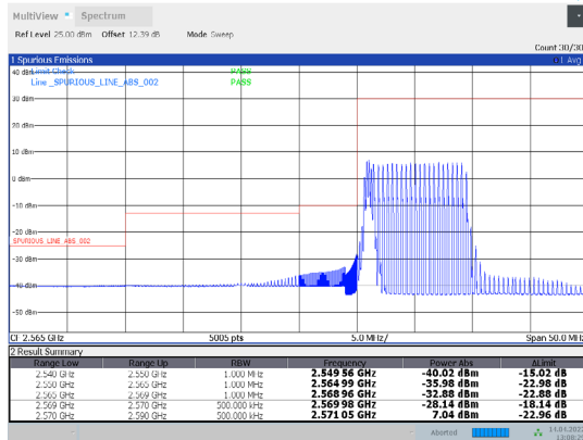
1-N38-PC3-30-20-L-12-DFT-16QAM-Inner_Full-25@12 -Ant1-PASS-see graph
