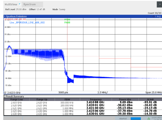
1-N38-PC3-30-10-H-26-CP-16QAM-Edge_1RB_Right-1 @23-Ant1-PASS-see graph
