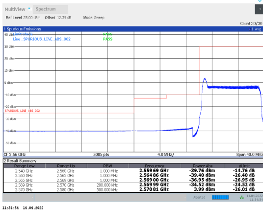
1-N38-PC3-30-10-L-31-CP-64QAM-Outer_Full-24@0-Ant1-PASS-see graph
