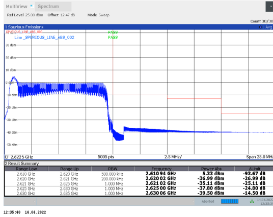
1-N38-PC3-30-10-H-30-CP-64QAM-Edge_1RB_Right-1@23-Ant1-PASS-see graph
