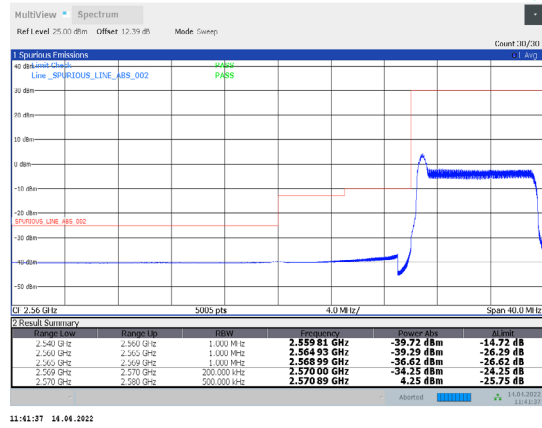
1-N38-PC3-30-10-L-35-CP-256QAM-Outer_Full-24@0-Ant1-PASS-see graph
