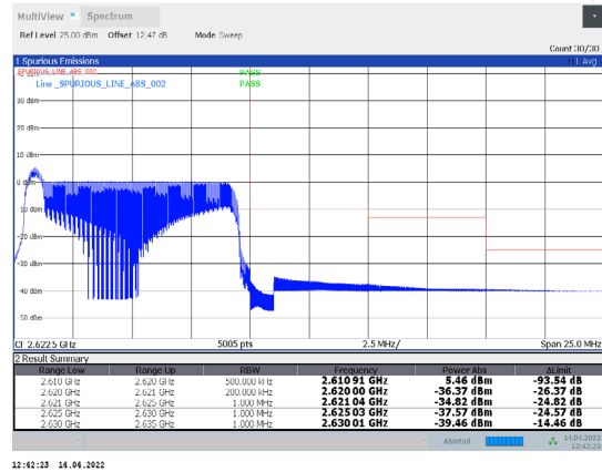
1-N38-PC3-30-10-H-34-CP-256QAM-Edge_1RB_Right-1@23-Ant1-PASS-see graph
