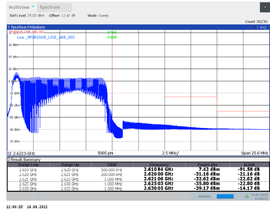
1-N38-PC3-30-10-H-10-DFT-16QAM-Edge_1RB_Right-1 @23-Ant1-PASS-see graph
