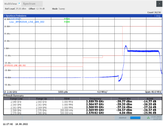
1-N38-PC3-30-10-L-27-CP-16QAM-Outer_Full-24@0-Ant1-PASS-see graph
