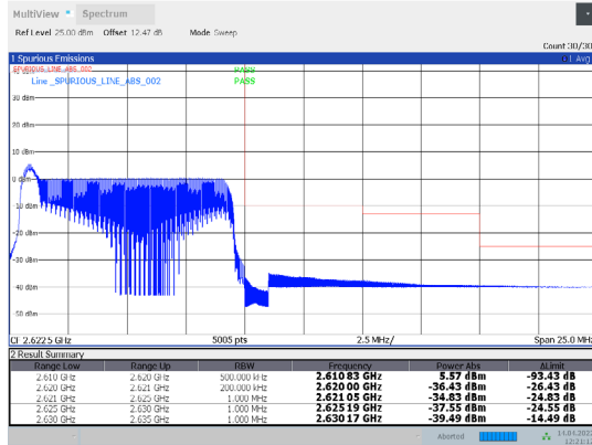
1-N38-PC3-30-10-H-22-CP-QPSK-Edge_1RB_Right-1 @23-Ant1-PASS-see graph
