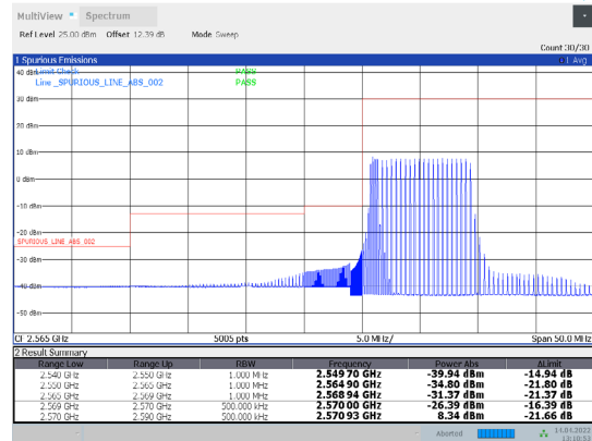
1-N38-PC3-30-20-L-13-DFT-64QAM-Edge_1RB_Left-1 @0-Ant1-PASS-see graph
