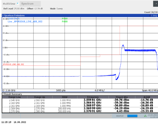
1-N38-PC3-30-10-L-25-CP-16QAM-Edge_1RB_Left-1 @0-Ant1-PASS-see graph
