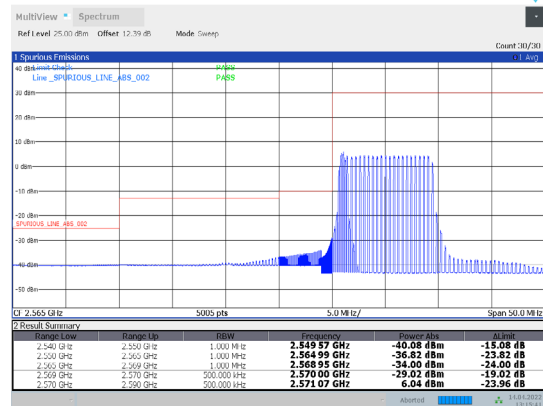
1-N38-PC3-30-20-L-16-DFT-64QAM-Inner_Full-25@12-Ant1-PASS-see graph
