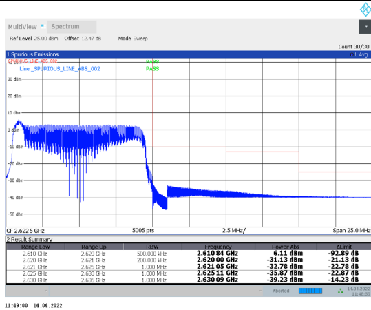
1-N38-PC3-30-10-H-3-DFT-PI/2BPSK-Edge_1RB_Right-1@23-Ant1-PASS-see graph
