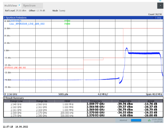
1-N38-PC3-30-10-L-32-CP-64QAM-Inner_Full-12@6-Ant1-PASS-see graph
