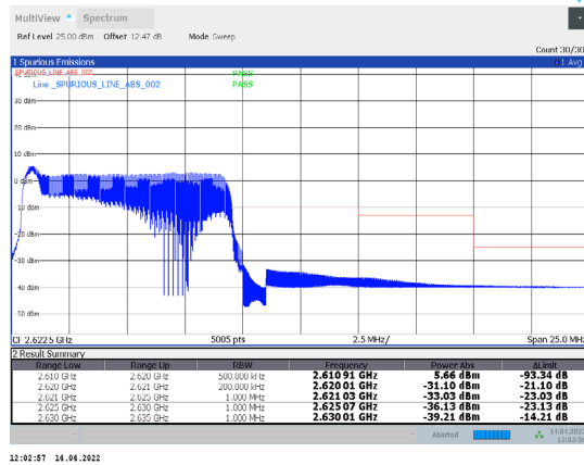
1-N38-PC3-30-10-H-11-DFT-16QAM-Outer_Full-24@0 -Ant1-PASS-see graph
