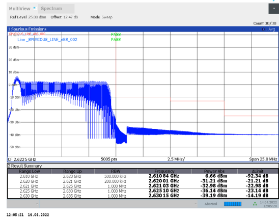
1-N38-PC3-30-10-H-12-DFT-16QAM-Inner_Full-12@6-A nt1-PASS-see graph
