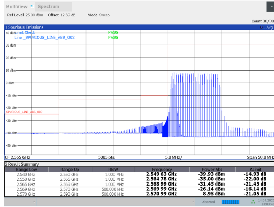
1-N38-PC3-30-20-L-9-DFT-16QAM-Edge_1RB_Left-1 @0-Ant1-PASS-see graph
