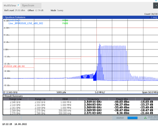
1-N38-PC3-30-20-L-20-DFT-256QAM-Inner_Full-25@12-Ant1-PASS-see graph
