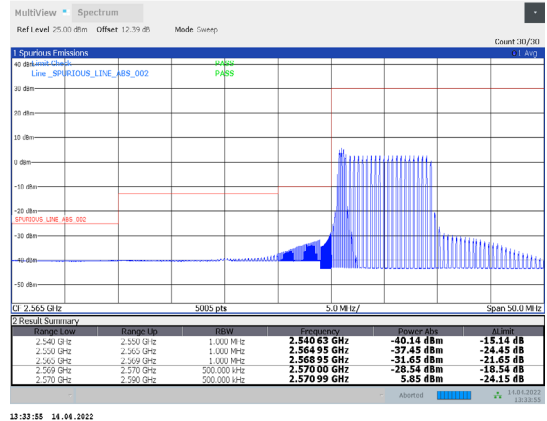
1-N38-PC3-30-20-L-27-CP-16QAM-Outer_Full-51@0-Ant1-PASS-see graph
