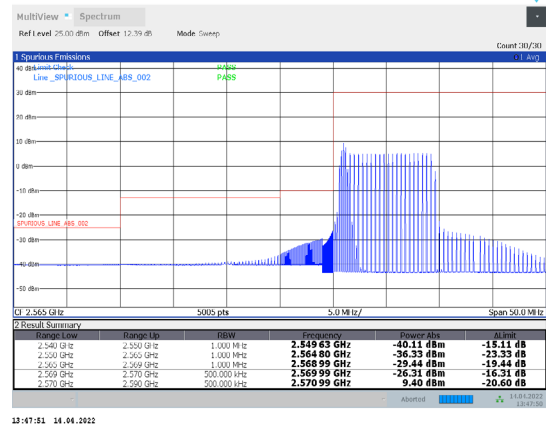
1-N38-PC3-30-20-L-35-CP-256QAM-Outer_Full-51@0-Ant1-PASS-see graph
