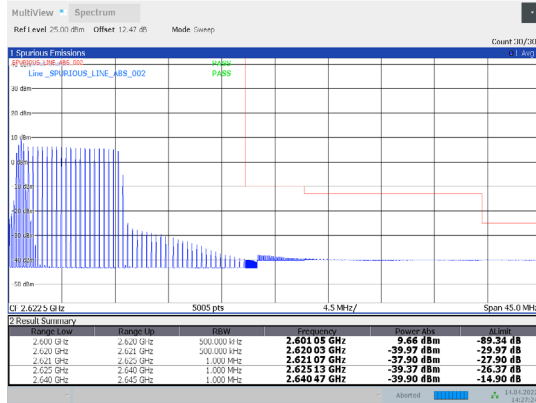
1-N38-PC3-30-20-H-22-CP-QPSK-Edge_1RB_Right-1 @50-Ant1-PASS-see graph
