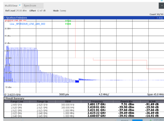
1-N38-PC3-30-20-H-28-CP-16QAM-Inner_Full-25@12-A nt1-PASS-see graph
