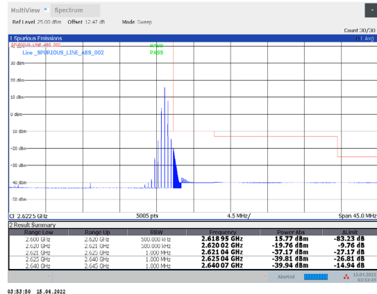
1-N38-PC3-30-20-H-34-CP-256QAM-Edge_1RB_Right-1@50-Ant1-PASS-see graph
