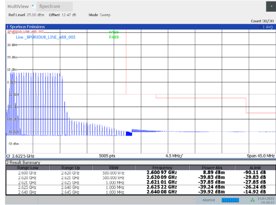
1-N38-PC3-30-20-H-15-DFT-64QAM-Outer_Full-50@0-Ant1-PASS-see graph
