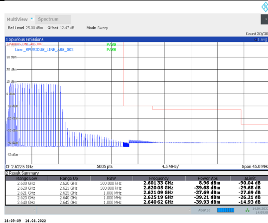
1-N38-PC3-30-20-H-11-DFT-16QAM-Outer_Full-50@0-Ant1-PASS-see graph
