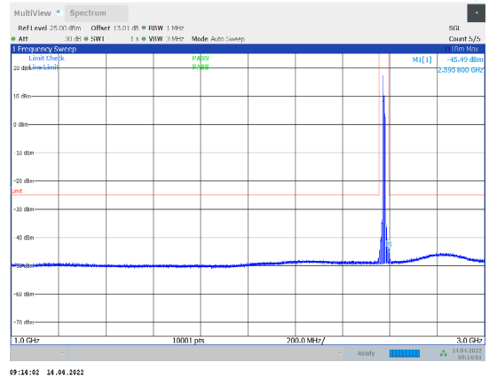
1-N38-PC3-30-10-L-3-CP-QPSK-Outer_Full-24@0-1000- 3000-Ant1--45.49--25-PASS
