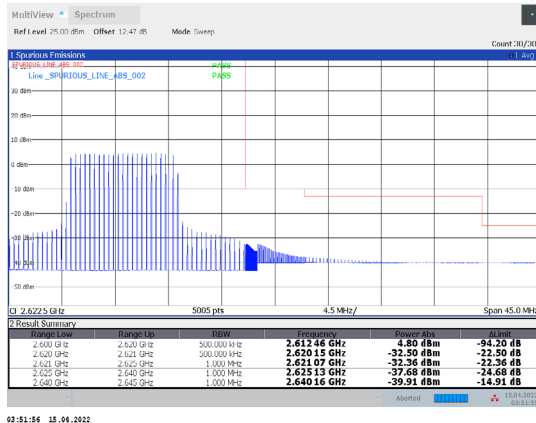
1-N38-PC3-30-20-H-32-CP-64QAM-Inner_Full-25@12-Ant1-PASS-see graph
