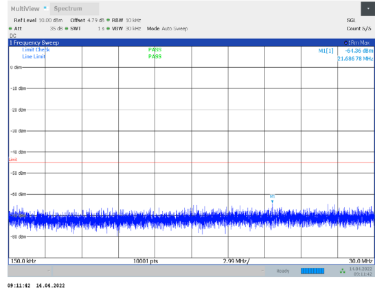
1-N38-PC3-30-10-L-2-CP-QPSK-Edge_1RB_Right-1@ 3-0.15-30-Ant1--64.36--45-PASS
