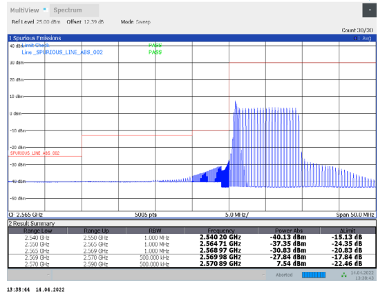
1-N38-PC3-30-20-L-29-CP-64QAM-Edge_1RB_Left-1 @0-Ant1-PASS-see graph
