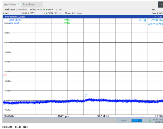
1-N38-PC3-30-10-L-2-CP-QPSK-Edge_1RB_Right-1@ 23-30-1000-Ant1--57.52--35-PASS
