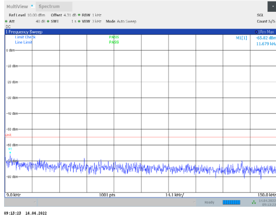
1-N38-PC3-30-10-L-3-CP-QPSK-Outer_Full-24@0-0.0 09-0.15-Ant1--65.82--55-PASS
