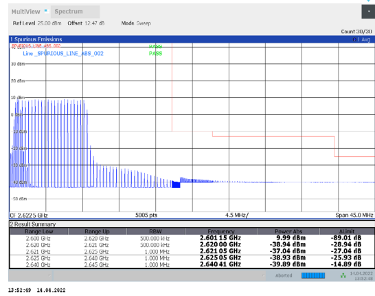
1-N38-PC3-30-20-H-1-DFT-PI/2BPSK-Inner_Full-25@12-Ant1-PASS-see graph
