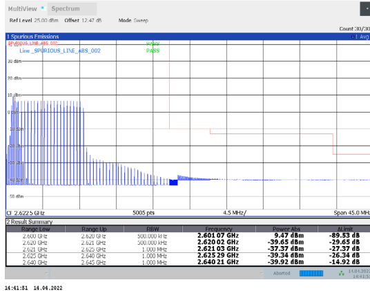
1-N38-PC3-30-20-H-30-CP-64QAM-Edge_1RB_Right-1@50-Ant1-PASS-see graph
