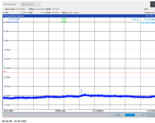
1-N38-PC3-30-10-L-3-CP-QPSK-Outer_Full-24@0-30- 1000-Ant1--57.31--35-PASS
