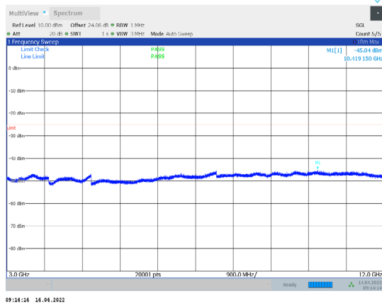
1-N38-PC3-30-10-L-3-CP-QPSK-Outer_Full-24@0-300 0-12000-Ant1--45.04--25-PASS
