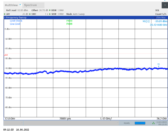
1-N38-PC3-30-10-L-2-CP-QPSK-Edge_1RB_Right-1@ 3-12000-26200-Ant1--39.09--25-PASS
