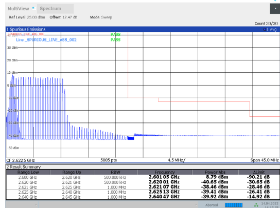
1-N38-PC3-30-20-H-20-DFT-256QAM-Inner_Full-25@12-Ant1-PASS-see graph
