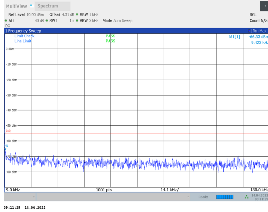
1-N38-PC3-30-10-L-2-CP-QPSK-Edge_1RB_Right-1@ 23-0.009-0.15-Ant1--66.33--55-PASS
