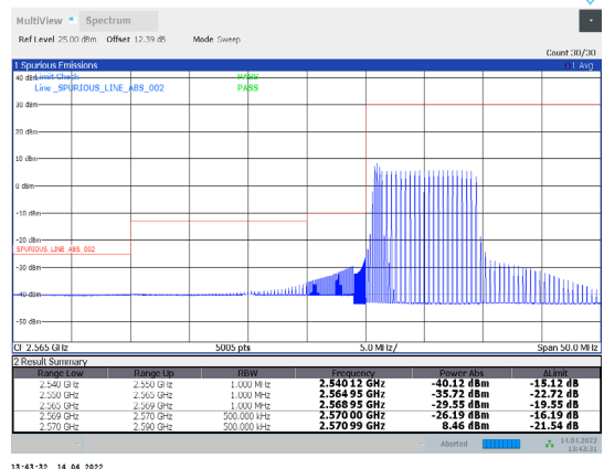
1-N38-PC3-30-20-L-32-CP-64QAM-Inner_Full-25@12-Ant1-PASS-see graph
