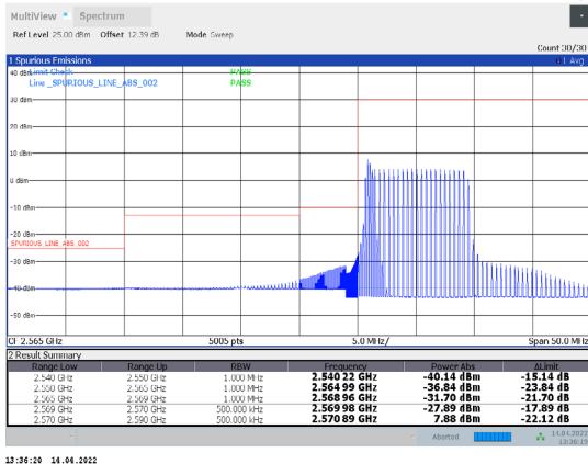
1-N38-PC3-30-20-L-28-CP-16QAM-Inner_Full-25@12-Ant1-PASS-see graph
