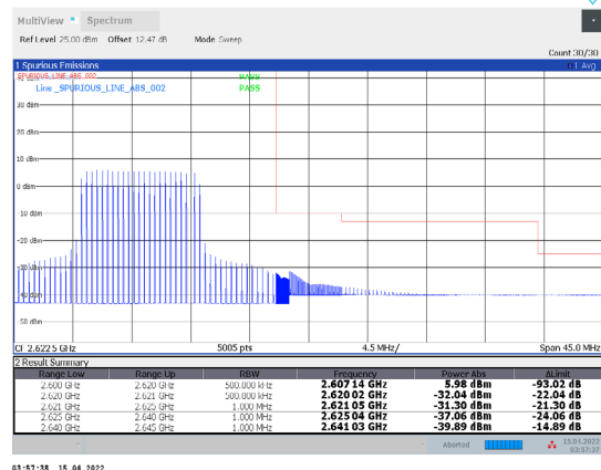
1-N38-PC3-30-20-H-36-CP-256QAM-Inner_Full-25@12-Ant1-PASS-see graph
