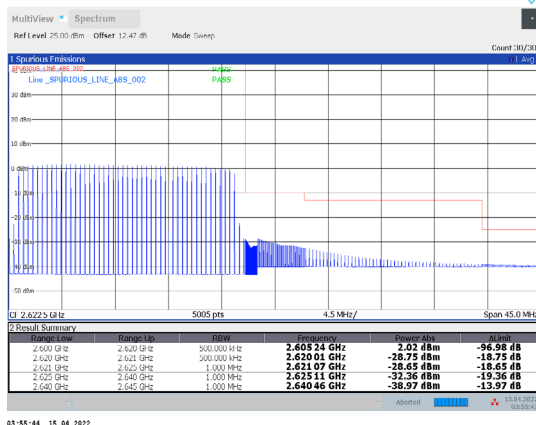
1-N38-PC3-30-20-H-35-CP-256QAM-Outer_Full-51@0-Ant1-PASS-see graph
