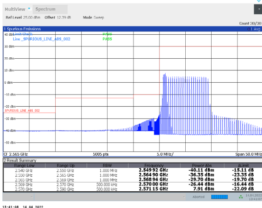
1-N38-PC3-30-20-L-31-CP-64QAM-Outer_Full-51@0-Ant1-PASS-see graph
