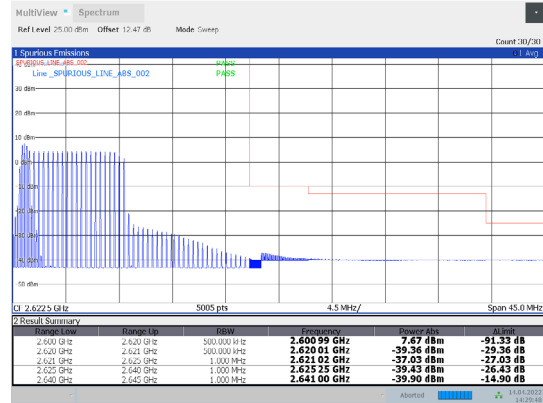
1-N38-PC3-30-20-H-23-CP-QPSK-Outer_Full-51@0-Ant 1-PASS-see graph
