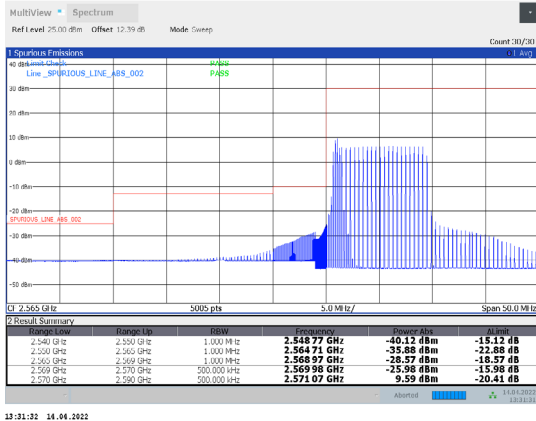
1-N38-PC3-30-20-L-25-CP-16QAM-Edge_1RB_Left-1 @0-Ant1-PASS-see graph
