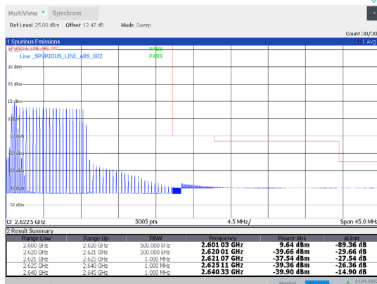
1-N38-PC3-30-20-H-27-CP-16QAM-Outer_Full-51@0-Ant1-PASS-see graph
