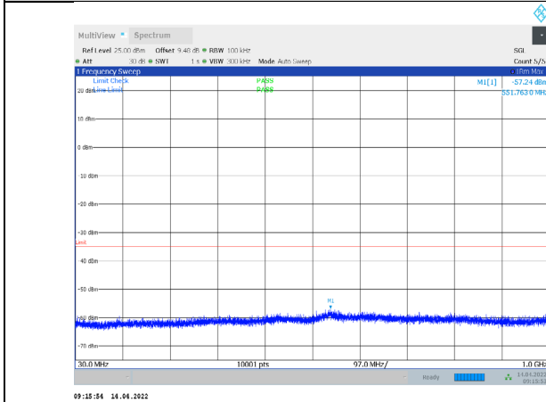
1-N38-PC3-30-10-M-1-CP-QPSK-Edge_1RB_Left-1@0 -30-1000-Ant1--57.24--35-PASS
