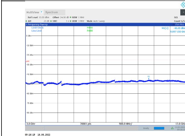
1-N38-PC3-30-10-M-1-CP-QPSK-Edge_1RB_Left-1@0 -3000-12000-Ant1--45.35--25-PASS
