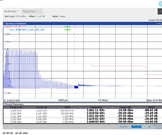
1-N38-PC3-30-20-H-8-DFT-QPSK-Inner_Full-25@12-Ant1-PASS-see graph
