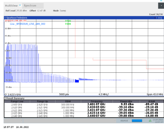
1-N38-PC3-30-20-H-4-DFT-PI/2BPSK-Outer_Full-50@0-Ant1-PASS-see graph
