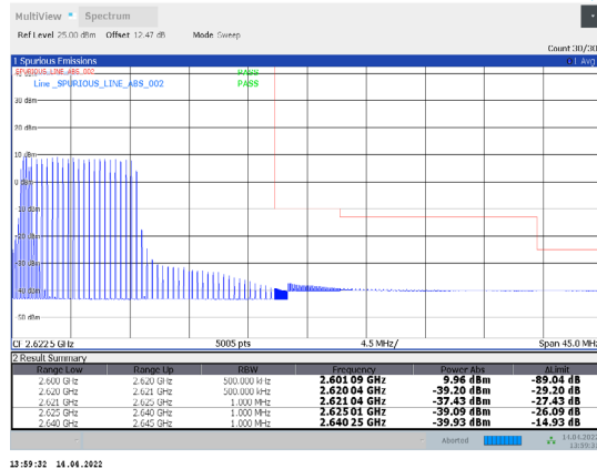
1-N38-PC3-30-20-H-6-DFT-QPSK-Edge_1RB_Right-1@50-Ant1-PASS-see graph
