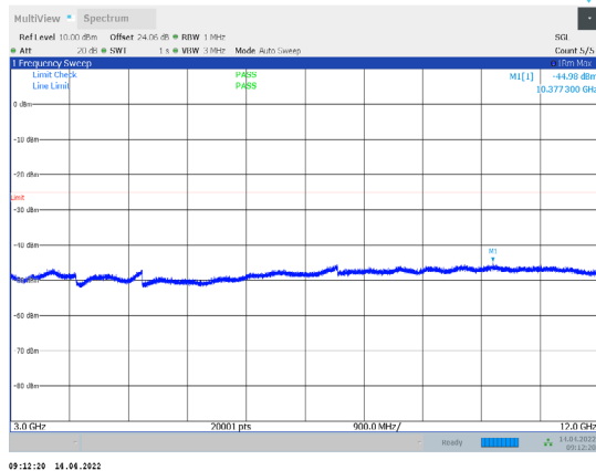
1-N38-PC3-30-10-L-2-CP-QPSK-Edge_1RB_Right-1@ 23-3000-12000-Ant1--44.98--25-PASS
