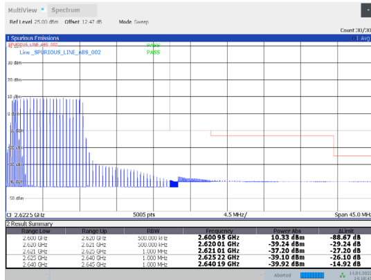
1-N38-PC3-30-20-H-16-DFT-64QAM-Inner_Full-25@12-Ant1-PASS-see graph
