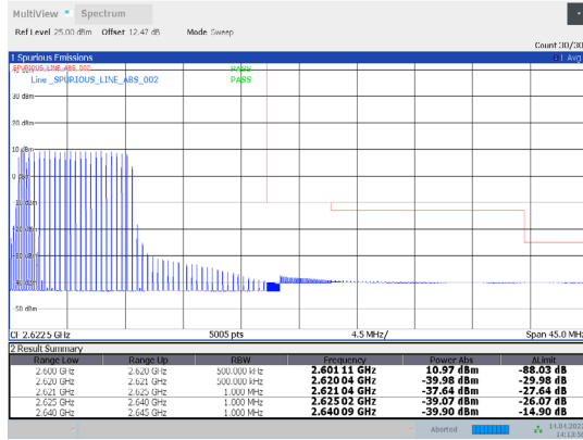
1-N38-PC3-30-20-H-14-DFT-64QAM-Edge_1RB_Right -1@50-Ant1-PASS-see graph
