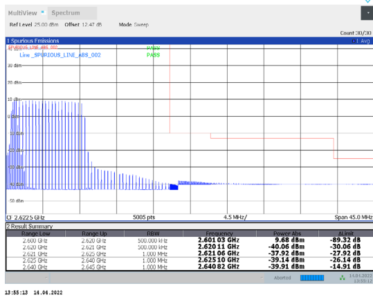
1-N38-PC3-30-20-H-3-DFT-PI/2BPSK-Edge_1RB_Right-1@50-Ant1-PASS-see graph
