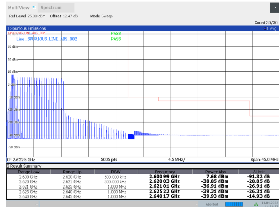
1-N38-PC3-30-20-H-26-CP-16QAM-Edge_1RB_Right-1 @50-Ant1-PASS-see graph
