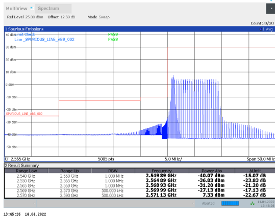
1-N38-PC3-30-20-L-33-CP-256QAM-Edge_1RB_Left-1@0-Ant1-PASS-see graph
