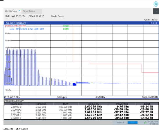
1-N38-PC3-30-20-H-12-DFT-16QAM-Inner_Full-25@12-Ant1-PASS-see graph
