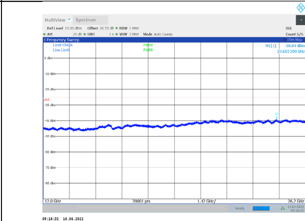
1-N38-PC3-30-10-M-1-CP-QPSK-Edge_1RB_Left-1@0 12000-26200-Ant1--38.84--25-PASS
