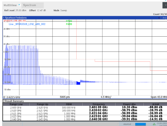
1-N38-PC3-30-20-H-19-DFT-256QAM-Outer_Full-50@0-Ant1-PASS-see graph
