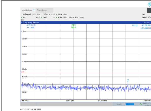
1-N38-PC3-30-10-M-1-CP-QPSK-Edge_1RB_Left-1@0 -0.009-0.15-Ant1--67.09--55-PASS
