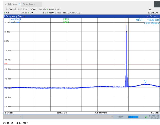
1-N38-PC3-30-10-L-2-CP-QPSK-Edge_1RB_Right-1@ 3-1000-3000-Ant1--45.33--25-PASS
