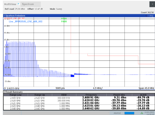
1-N38-PC3-30-20-H-18-DFT-256QAM-Edge_1RB_Right -1@50-Ant1-PASS-see graph
