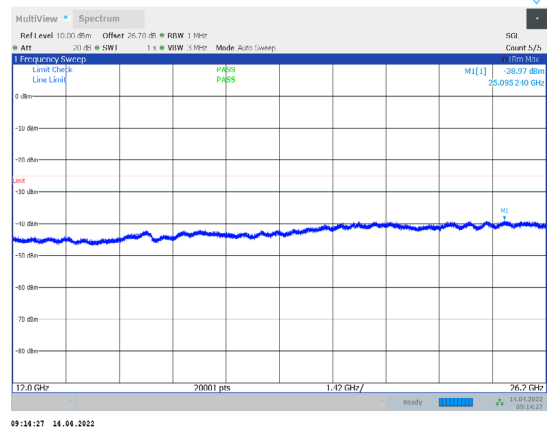
1-N38-PC3-30-10-L-3-CP-QPSK-Outer_Full-24@0-1200 0-26200-Ant1--38.97--25-PASS
