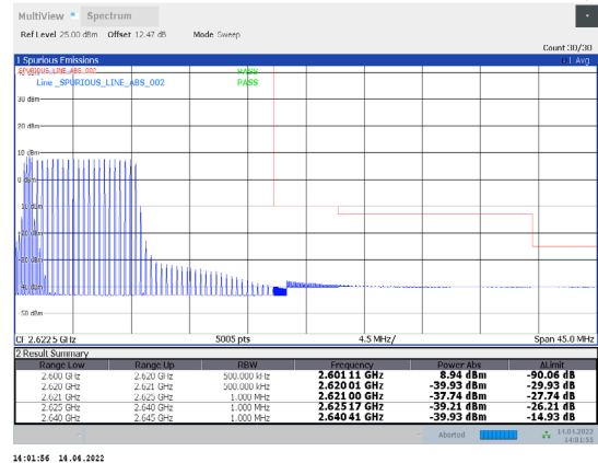
1-N38-PC3-30-20-H-7-DFT-QPSK-Outer_Full-50@0-Ant1-PASS-see graph
