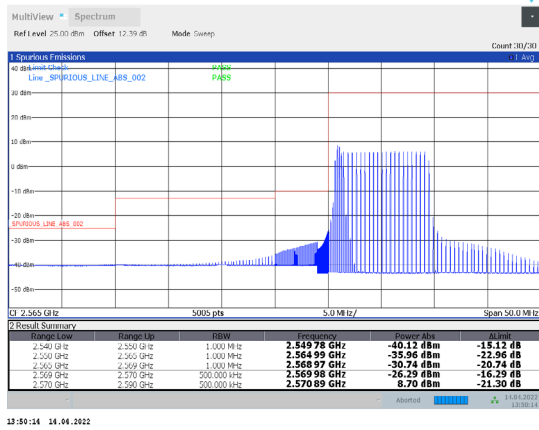
1-N38-PC3-30-20-L-36-CP-256QAM-Inner_Full-25@12-Ant1-PASS-see graph
