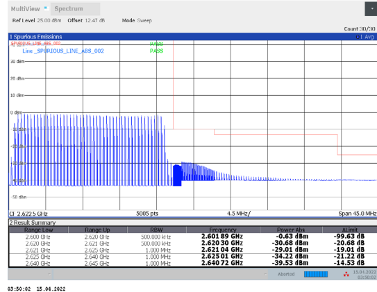
1-N38-PC3-30-20-H-31-CP-64QAM-Outer_Full-51@0-Ant1-PASS-see graph
