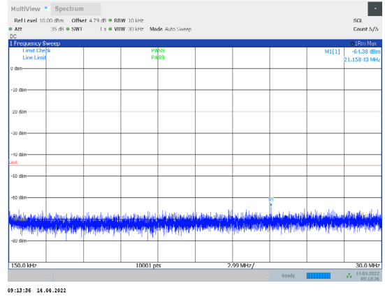
1-N38-PC3-30-10-L-3-CP-QPSK-Outer_Full-24@0-0.15- 30-Ant1--64.38--45-PASS
