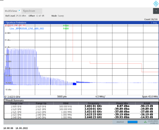
1-N38-PC3-30-20-H-10-DFT-16QAM-Edge_1RB_Right-1@50-Ant1-PASS-see graph
