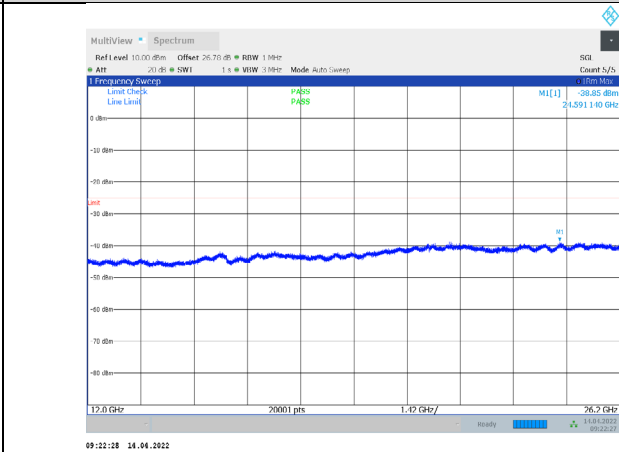
1-N38-PC3-30-10-H-1-CP-QPSK-Edge_1RB_Left-1@0 -12000-26200-Ant1--38.85--25-PASS
