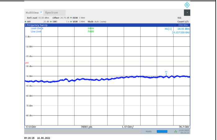
1-N38-PC3-30-10-H-2-CP-QPSK-Edge_1RB_Right-1@ 23-12000-26200-Ant1--38.95--25-PASS
