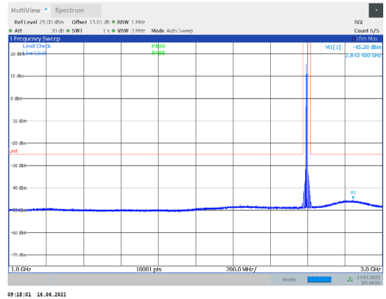
1-N38-PC3-30-10-M-2-CP-QPSK-Edge_1RB_Right-1@ 23-1000-3000-Ant1--45.38--25-PASS
