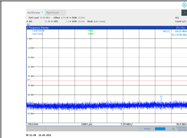
1-N38-PC3-30-10-H-1-CP-QPSK-Edge_1RB_Left-1@0 -0.15-30-Ant1--65.20--45-PASS
