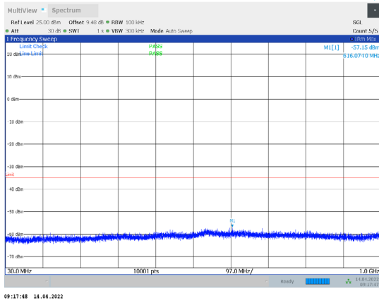
1-N38-PC3-30-10-M-2-CP-QPSK-Edge_1RB_Right-1@ 23-30-1000-Ant1--57.15--35-PASS
