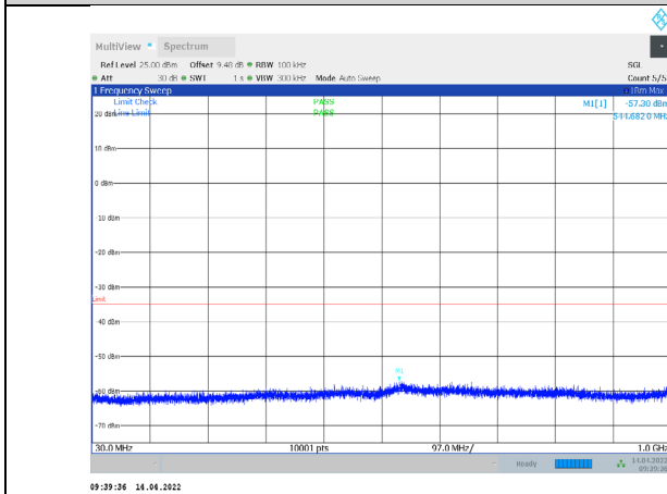
1-N38-PC3-30-15-H-1-CP-QPSK-Edge_1RB_Left-1@0 -30-1000-Ant1--57.30--35-PASS
