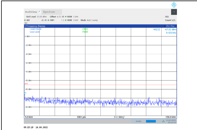
1-N38-PC3-30-10-H-2-CP-QPSK-Edge_1RB_Right-1@ 23-0.009-0.15-Ant1--67.32--55-PASS
