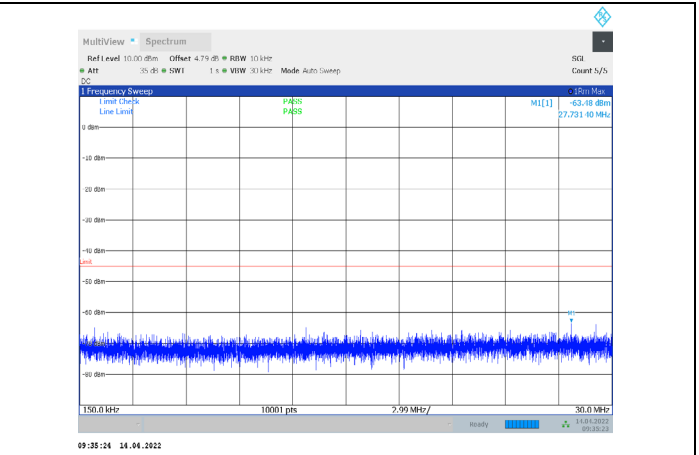
1-N38-PC3-30-15-M-2-CP-QPSK-Edge_1RB_Right-1@ 37-0.15-30-Ant1--63.48--45-PASS
