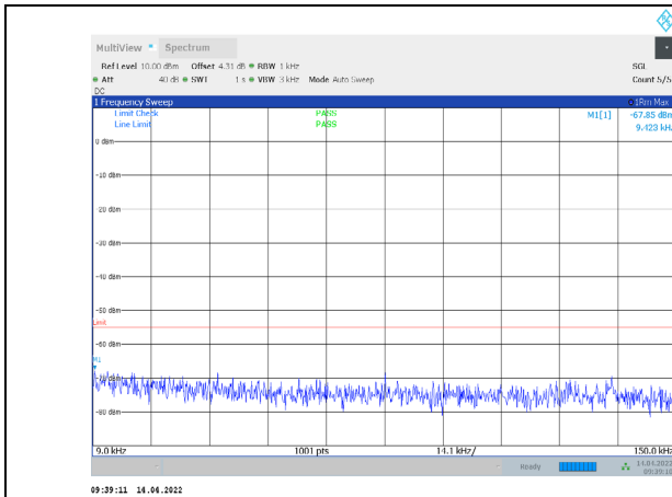
1-N38-PC3-30-15-H-1-CP-QPSK-Edge_1RB_Left-1@0 -0.009-0.15-Ant1--67.85--55-PASS
