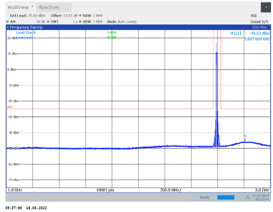
1-N38-PC3-30-15-M-3-CP-QPSK-Outer_Full-38@0-100 0-3000-Ant1--45.53--25-PASS
