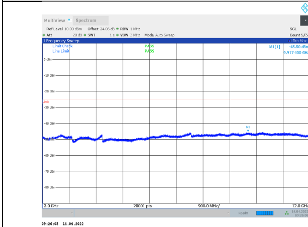
1-N38-PC3-30-10-H-3-CP-QPSK-Outer_Full-24@0-300 0-12000-Ant1--45.50--25-PASS
