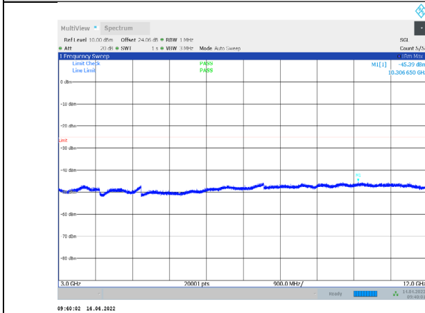
1-N38-PC3-30-15-H-1-CP-QPSK-Edge_1RB_Left-1@0 -3000-12000-Ant1--45.39--25-PASS
