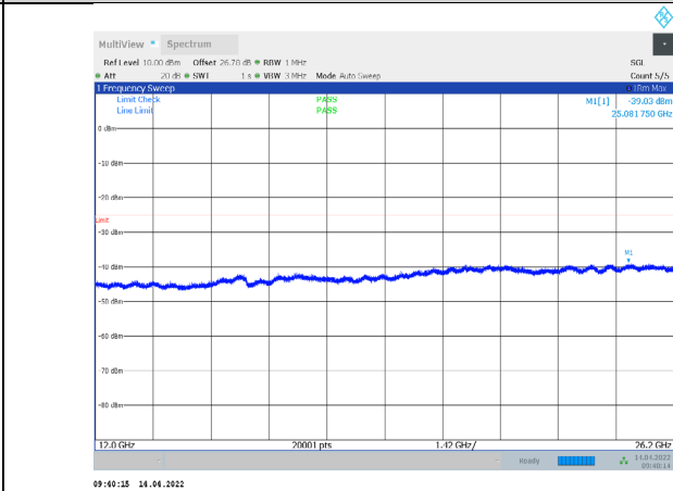
1-N38-PC3-30-15-H-1-CP-QPSK-Edge_1RB_Left-1@0- 12000-26200-Ant1--39.03--25-PASS
