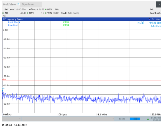
1-N38-PC3-30-15-M-3-CP-QPSK-Outer_Full-38@0-0.0 09-0.15-Ant1--66.46--55-PASS
