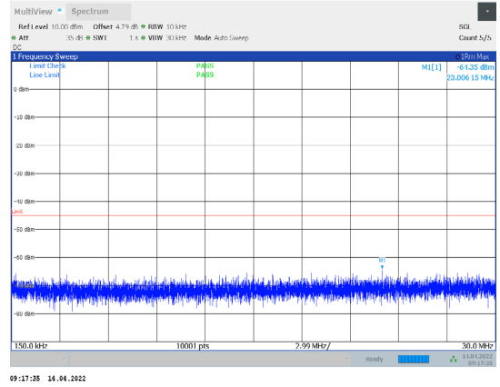
1-N38-PC3-30-10-M-2-CP-QPSK-Edge_1RB_Right-1@ 23-0.15-30-Ant1--64.35--45-PASS
