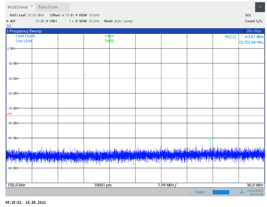
1-N38-PC3-30-10-M-3-CP-QPSK-Outer_Full-24@0-0.15 -30-Ant1--64.67--45-PASS
