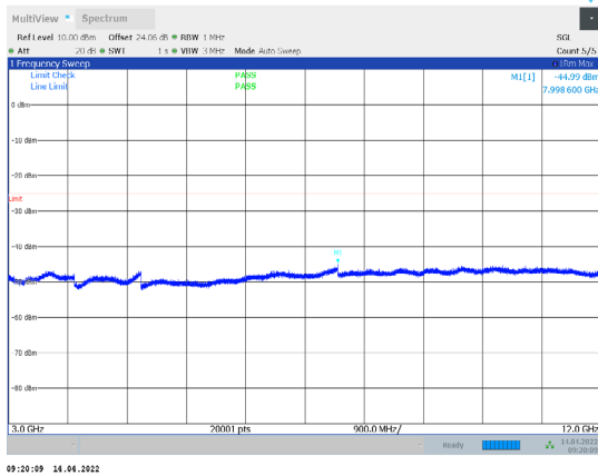
1-N38-PC3-30-10-M-3-CP-QPSK-Outer_Full-24@0-30 00-12000-Ant1--44.99--25-PASS
