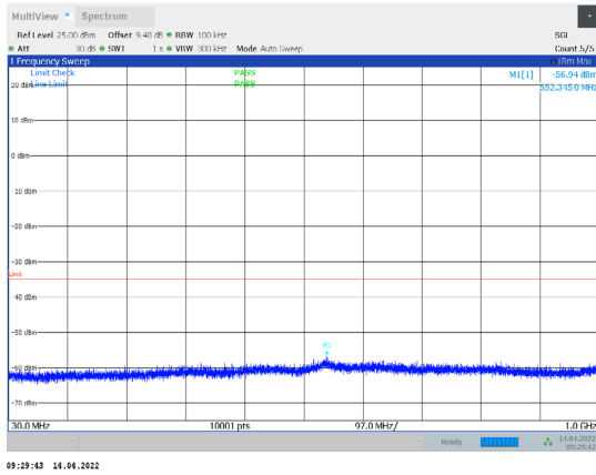
1-N38-PC3-30-15-L-2-CP-QPSK-Edge_1RB_Right-1@ 37-30-1000-Ant1--56.94--35-PASS
