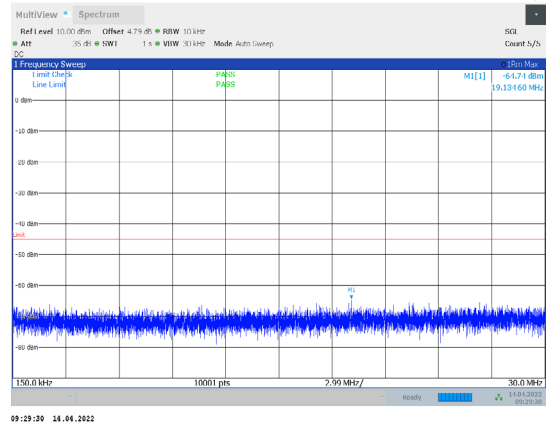
1-N38-PC3-30-15-L-2-CP-QPSK-Edge_1RB_Right-1@ 7-0.15-30-Ant1--64.74--45-PASS
