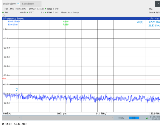
1-N38-PC3-30-10-M-2-CP-QPSK-Edge_1RB_Right-1@ 23-0.009-0.15-Ant1--67.75--55-PASS
