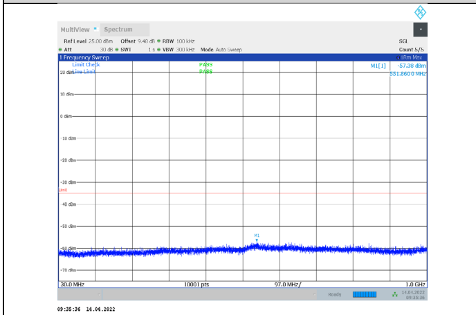
1-N38-PC3-30-15-M-2-CP-QPSK-Edge_1RB_Right-1@ 37-30-1000-Ant1--57.38--35-PASS
