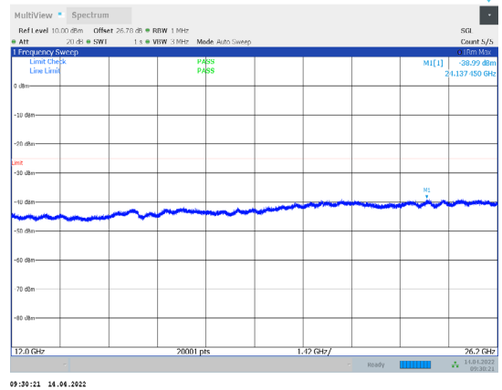
1-N38-PC3-30-15-L-2-CP-QPSK-Edge_1RB_Right-1@ 7-12000-26200-Ant1--38.99--25-PASS
