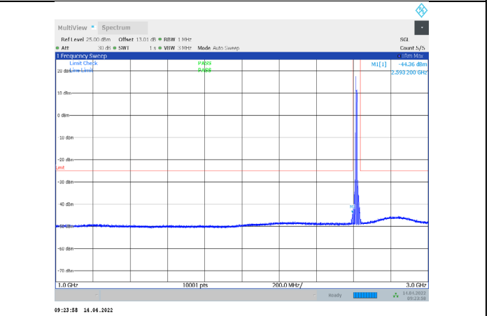
1-N38-PC3-30-10-H-2-CP-QPSK-Edge_1RB_Right-1@ 23-1000-3000-Ant1--44.36--25-PASS
