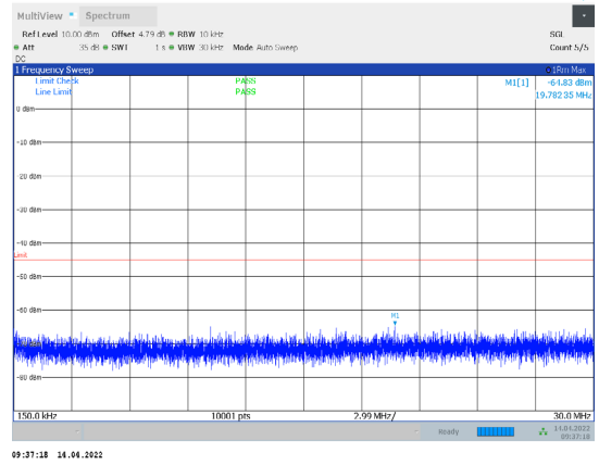
1-N38-PC3-30-15-M-3-CP-QPSK-Outer_Full-38@0-0.15 -30-Ant1--64.83--45-PASS
