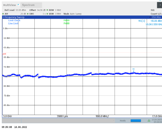
1-N38-PC3-30-15-L-2-CP-QPSK-Edge_1RB_Right-1@ 37-3000-12000-Ant1--45.56--25-PASS
