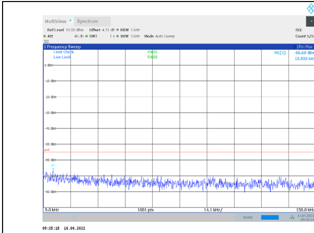
1-N38-PC3-30-10-H-3-CP-QPSK-Outer_Full-24@0-0.0 09-0.15-Ant1--66.68--55-PASS
