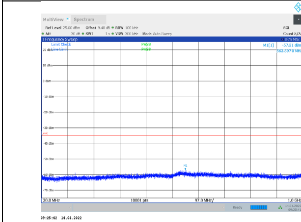
1-N38-PC3-30-10-H-3-CP-QPSK-Outer_Full-24@0-30- 1000-Ant1--57.31--35-PASS
