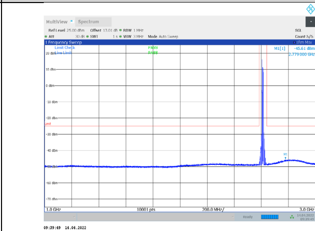
1-N38-PC3-30-15-H-1-CP-QPSK-Edge_1RB_Left-1@0- 1000-3000-Ant1--45.61--25-PASS
