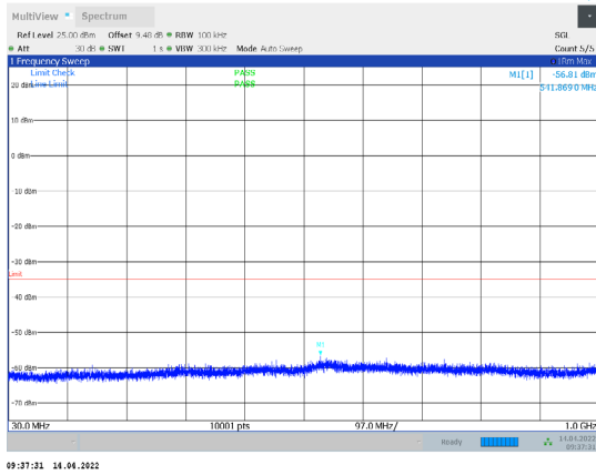
1-N38-PC3-30-15-M-3-CP-QPSK-Outer_Full-38@0-30- 1000-Ant1--56.81--35-PASS
