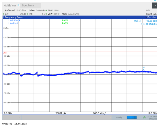
1-N38-PC3-30-15-L-3-CP-QPSK-Outer_Full-38@0-300 0-12000-Ant1--45.38--25-PASS
