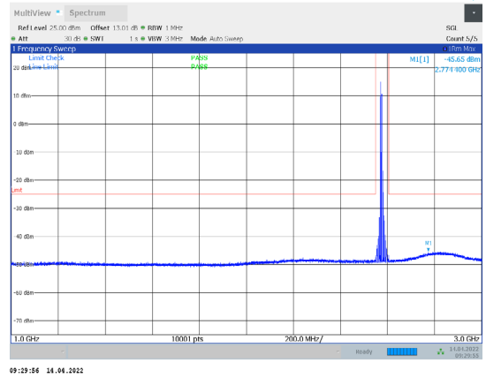
1-N38-PC3-30-15-L-2-CP-QPSK-Edge_1RB_Right-1@ 7-1000-3000-Ant1--45.65--25-PASS
