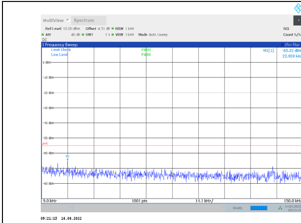
1-N38-PC3-30-10-H-1-CP-QPSK-Edge_1RB_Left-1@0 -0.009-0.15-Ant1--65.32--55-PASS
