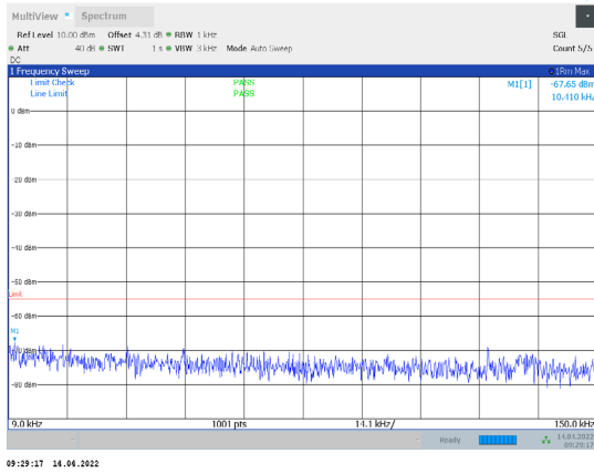
1-N38-PC3-30-15-L-2-CP-QPSK-Edge_1RB_Right-1@ 37-0.009-0.15-Ant1--67.65--55-PASS
