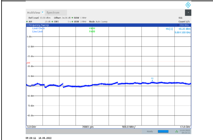
1-N38-PC3-30-10-H-2-CP-QPSK-Edge_1RB_Right-1@ 23-3000-12000-Ant1--45.35--25-PASS
