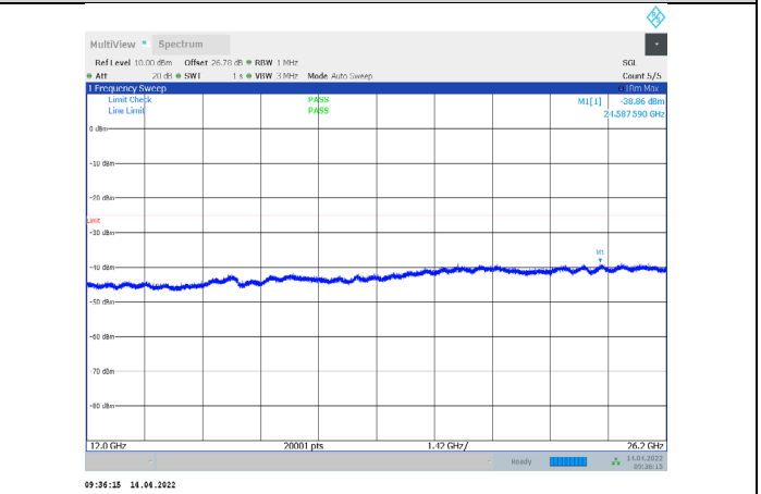
1-N38-PC3-30-15-M-2-CP-QPSK-Edge_1RB_Right-1@ 37-12000-26200-Ant1--38.86--25-PASS
