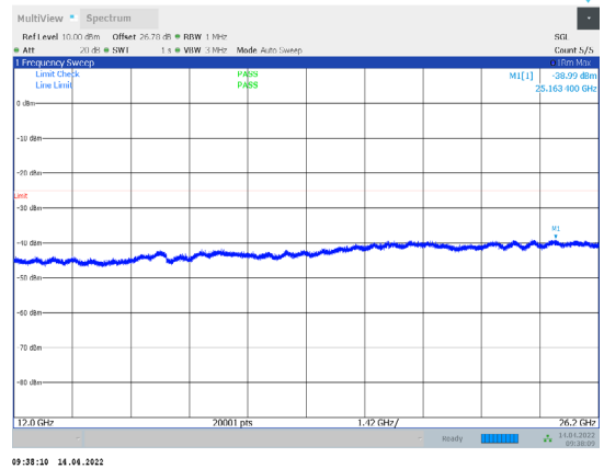
1-N38-PC3-30-15-M-3-CP-QPSK-Outer_Full-38@0-120 00-26200-Ant1--38.99--25-PASS
