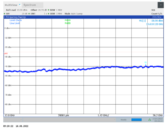
1-N38-PC3-30-10-M-3-CP-QPSK-Outer_Full-24@0-120 00-26200-Ant1--38.98--25-PASS
