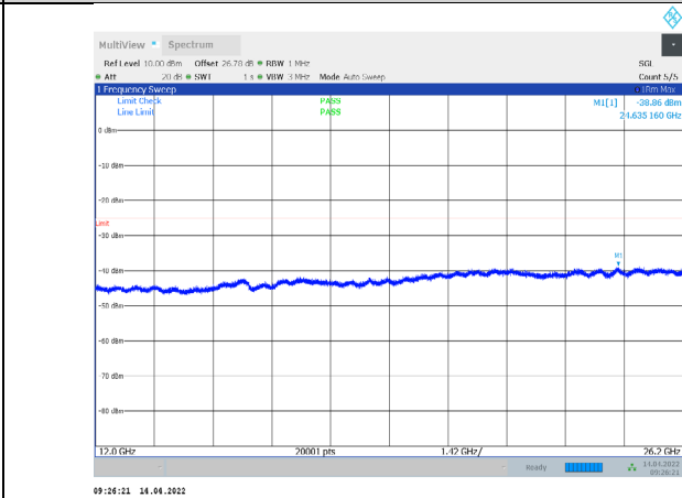
1-N38-PC3-30-10-H-3-CP-QPSK-Outer_Full-24@0-120 00-26200-Ant1--38.86--25-PASS
