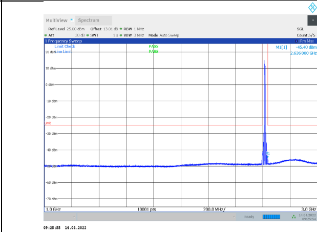
1-N38-PC3-30-10-H-3-CP-QPSK-Outer_Full-24@0-100 0-3000-Ant1--45.40--25-PASS
