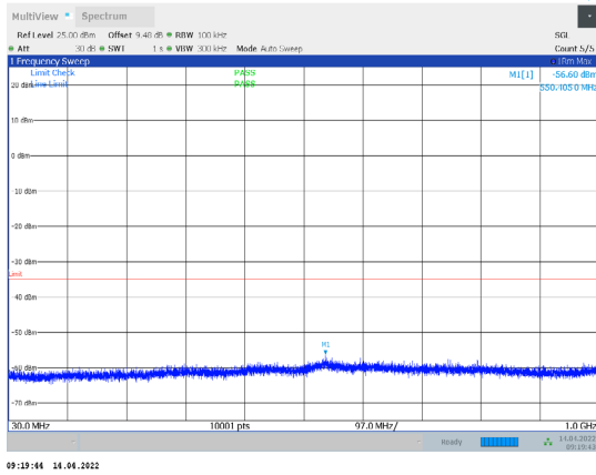
1-N38-PC3-30-10-M-3-CP-QPSK-Outer_Full-24@0-30- 1000-Ant1--56.60--35-PASS
