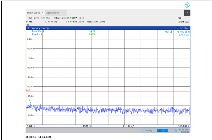
1-N38-PC3-30-15-M-2-CP-QPSK-Edge_1RB_Right-1@ 37-0.009-0.15-Ant1--67.62--55-PASS
