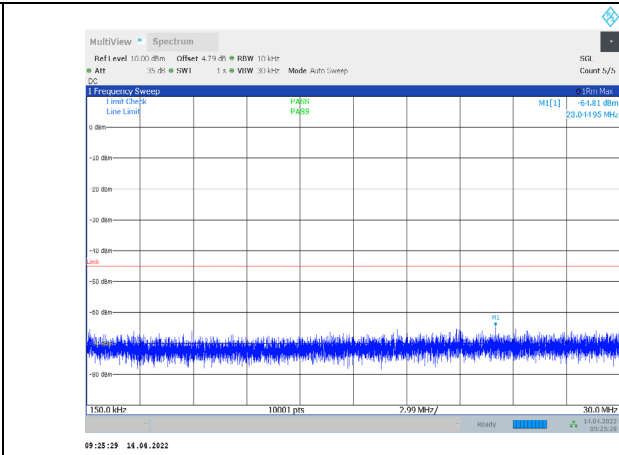
1-N38-PC3-30-10-H-3-CP-QPSK-Outer_Full-24@0-0.15 -30-Ant1--64.81--45-PASS
