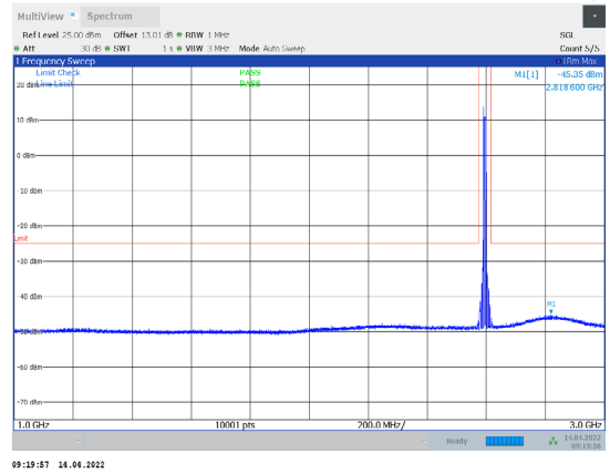
1-N38-PC3-30-10-M-3-CP-QPSK-Outer_Full-24@0-100 0-3000-Ant1--45.35--25-PASS
