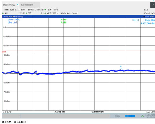
1-N38-PC3-30-15-M-3-CP-QPSK-Outer_Full-38@0-30 00-12000-Ant1--45.57--25-PASS
