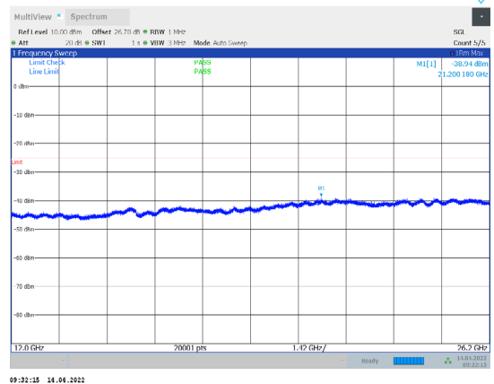
1-N38-PC3-30-15-L-3-CP-QPSK-Outer_Full-38@0-1200 0-26200-Ant1--38.94--25-PASS
