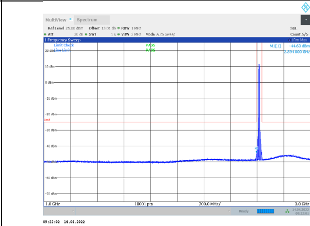
1-N38-PC3-30-10-H-1-CP-QPSK-Edge_1RB_Left-1@0 -1000-3000-Ant1--44.63--25-PASS
