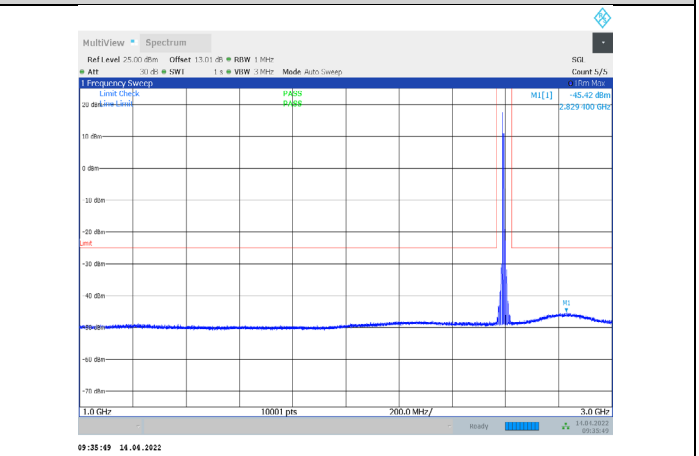
1-N38-PC3-30-15-M-2-CP-QPSK-Edge_1RB_Right-1@ 37-1000-3000-Ant1--45.42--25-PASS
