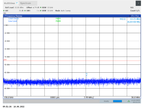
1-N38-PC3-30-15-L-3-CP-QPSK-Outer_Full-38@0-0.15- 30-Ant1--64.72--45-PASS
