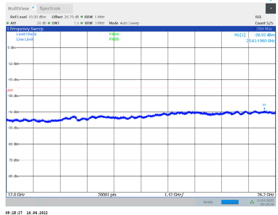
1-N38-PC3-30-10-M-2-CP-QPSK-Edge_1RB_Right-1@ 23-12000-26200-Ant1--38.92--25-PASS
