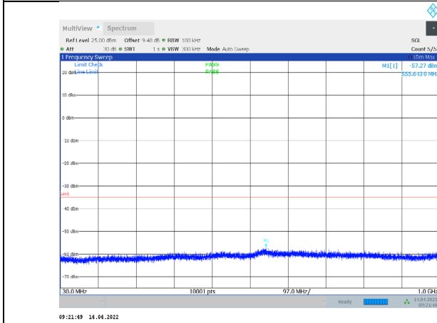
1-N38-PC3-30-10-H-1-CP-QPSK-Edge_1RB_Left-1@0 -30-1000-Ant1--57.27--35-PASS
