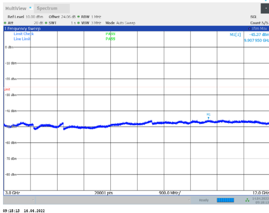
1-N38-PC3-30-10-M-2-CP-QPSK-Edge_1RB_Right-1@ 23-3000-12000-Ant1--45.37--25-PASS
