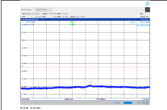
1-N38-PC3-30-10-H-2-CP-QPSK-Edge_1RB_Right-1@ 23-30-1000-Ant1--56.78--35-PASS
