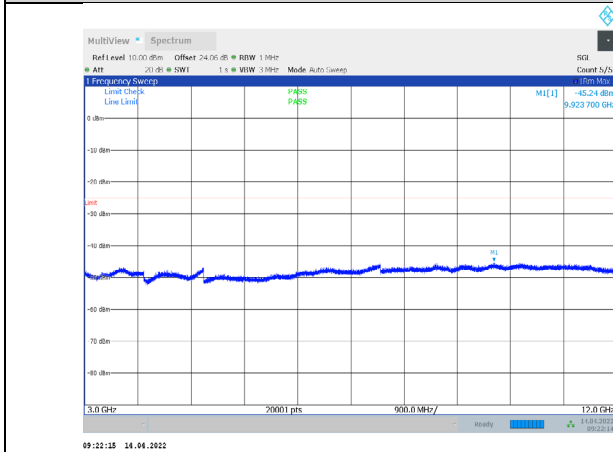
1-N38-PC3-30-10-H-1-CP-QPSK-Edge_1RB_Left-1@0 -3000-12000-Ant1--45.24--25-PASS
