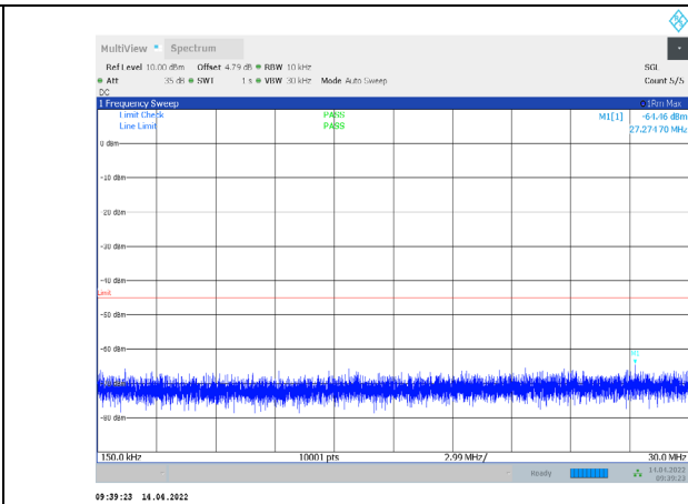
1-N38-PC3-30-15-H-1-CP-QPSK-Edge_1RB_Left-1@0- 0.15-30-Ant1--64.46--45-PASS
