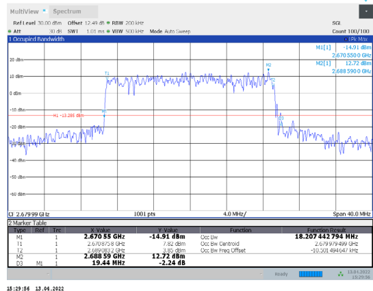
1-N41-PC3-30-20-H-4-CP-256QAM-Outer_Full-51@0-Ant1 -18.207-19.440-≤20-PASS
