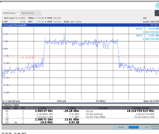
1-N41-PC3-30-20-M-2-CP-16QAM-Outer_Full-51@0-A nt1-18.217-19.000-≤20-PASS
