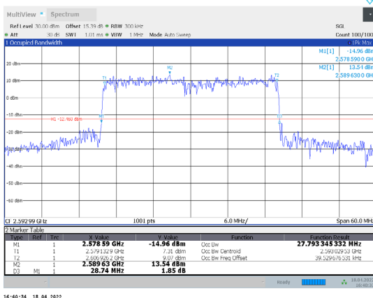
1-N41-PC3-30-30-M-2-CP-16QAM-Outer_Full-78@0-A nt1-27.793-28.740-≤30-PASS
