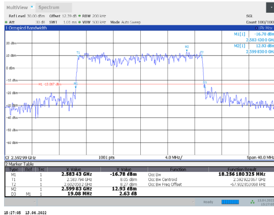
1-N41-PC3-30-20-M-4-CP-256QAM-Outer_Full-51@0-Ant1-18.256-19.080-≤20-PASS
