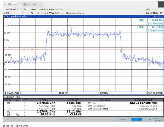
1-N41-PC3-30-20-H-2-CP-16QAM-Outer_Full-51@0-Ant1 -18.195-18.880-≤20-PASS
