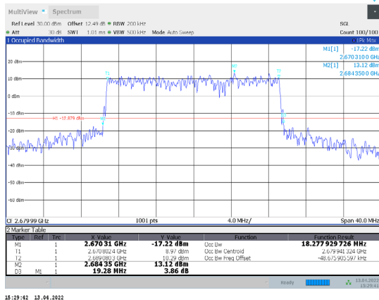
1-N41-PC3-30-20-H-3-CP-64QAM-Outer_Full-51@0-Ant1 1-18.278-19.280-≤20-PASS
