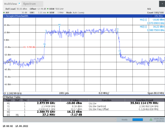
1-N41-PC3-30-40-M-5-DFT-PI/2BPSK-Outer_Full-100@0-Ant1-35.615-37.200-≤40-PASS
