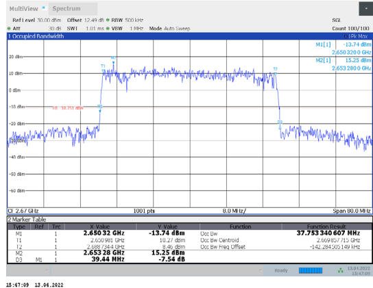
1-N41-PC3-30-40-H-2-CP-16QAM-Outter_Full-106@0-Ant 1-37.74-39.440-≤40-PASS
