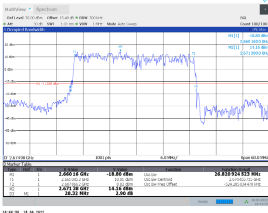
1-N41-PC3-30-30-H-5-DFT-PI/2BPSK-Outter_Full-75@0-A Ant1-26.821-28.320-≤30-PASS
