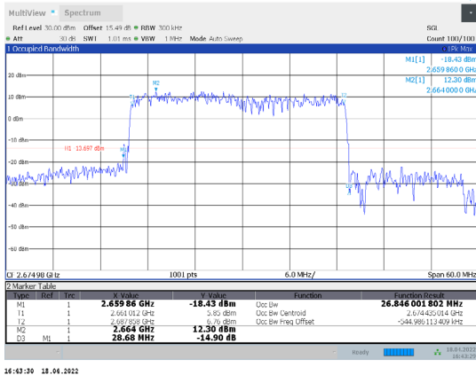
1-N41-PC3-30-30-H-1-CP-QPSK-Outter_Full-78@0-Ant1 -26.846-28.680-≤30-PASS
