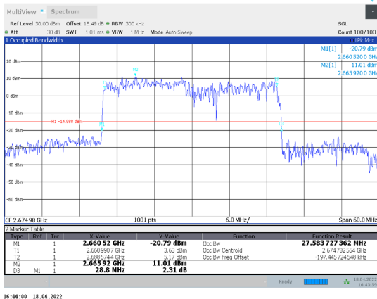
1-N41-PC3-30-30-H-3-CP-64QAM-Outter_Full-78@0-Ant 1-27.584-28.800-≤30-PASS
