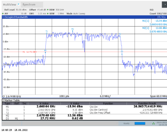
1-N41-PC3-30-30-H-9-DFT-256QAM-Outer_Full-75@0-A nt1-26.563-27.720-≤30-PASS
