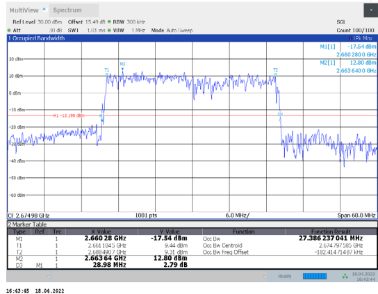
1-N41-PC3-30-30-H-2-CP-16QAM-Outter_Full-78@0-A nt1-27.386-28.980-≤30-PASS
