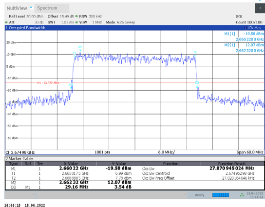
1-N41-PC3-30-30-H-4-CP-256QAM-Outter_Full-78@0-A Ant1-27.871-29.160-≤30-PASS
