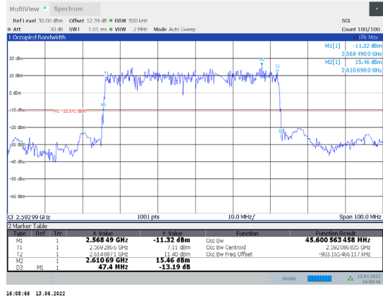
1-N41-PC3-30-50-M-5-DFT-PI/2BPSK-Outer_Full-128@0-Ant1-45.601-47.400-≤50-PASS
