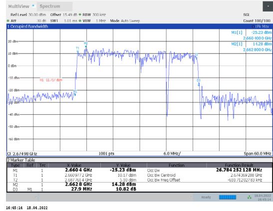
1-N41-PC3-30-30-H-8-DFT-64QAM-Outer_Full-75@0-A nt1-26.784-27.900-≤30-PASS
