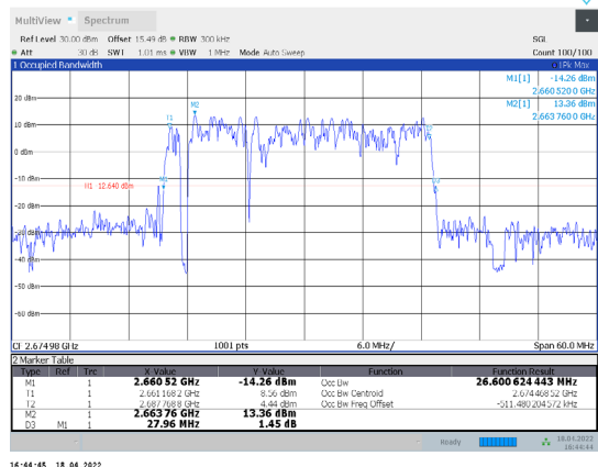
1-N41-PC3-30-30-H-6-DFT-QPSK-Outter_Full-75@0-A nt1-26.601-27.960-≤30-PASS
