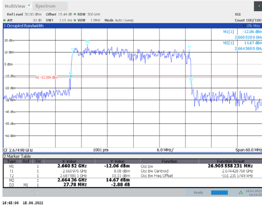
1-N41-PC3-30-30-H-7-DFT-16QAM-Outer_Full-75@0-A nt1-26.905-27.780-≤30-PASS
