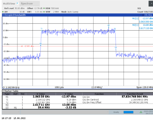
1-N41-PC3-30-60-M-4-CP-256QAM-Outer_Full-162@0-Ant1-57.835-59.400-≤60-PASS
