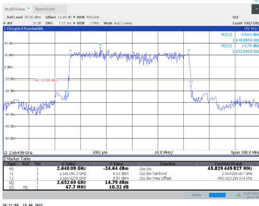
1-N41-PC3-30-50-H-5-DFT-PI/2BPSK-Outter_Full-128@0-Ant1 1-45.829-47.700-≤50-PASS
