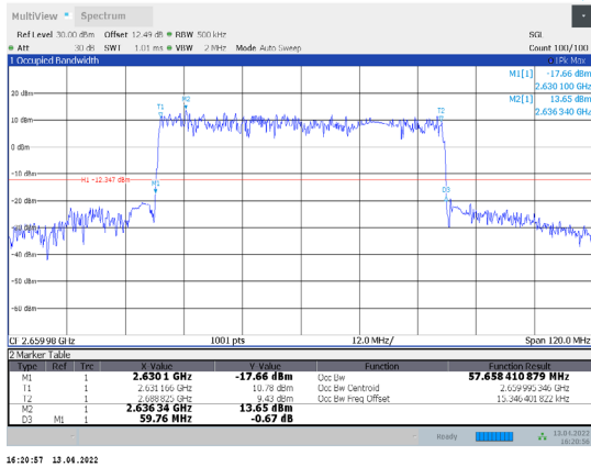
1-N41-PC3-30-60-H-7-DFT-16QAM-Outter_Full-162@0-A nt1-57.658-59.760-≤60-PASS
