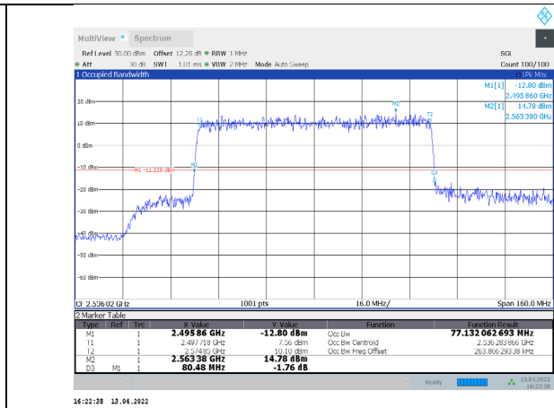
1-N41-PC3-30-80-L-2-CP-16QAM-Outer_Full-217@0-Ant 1-77.132-80.480-≤80-PASS
