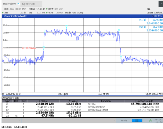
1-N41-PC3-30-50-H-7-DFT-16QAM-Outer_Full-128@0-Ant1-45.794-47.500-≤50-PASS
