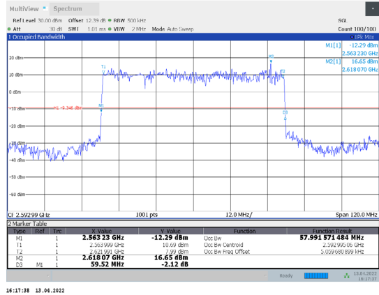
1-N41-PC3-30-60-M-5-DFT-PI/2BPSK-Outer_Full-162@0-Ant1-57.992-59.520-≤60-PASS
