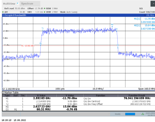
1-N41-PC3-30-80-M-4-CP-256QAM-Outer_Full-217@0-Ant1-76.941-80.320-≤80-PASS
