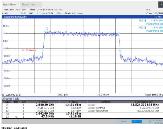
1-N41-PC3-30-50-H-3-CP-64QAM-Outter_Full-133@0-Ant1 1-45.524-47.500-≤50-PASS
