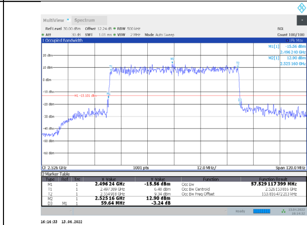
1-N41-PC3-30-60-L-4-CP-256QAM-Outer_Full-162@0-Ant 1-57.529-59.640-≤60-PASS
