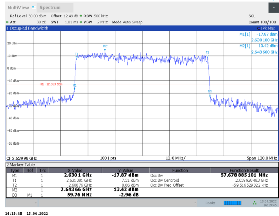
1-N41-PC3-30-60-H-2-CP-16QAM-Outter_Full-162@0-Ant 1-57.679-59.760-≤60-PASS
