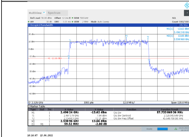
1-N41-PC3-30-60-L-5-DFT-PI/2BPSK-Outer_Full-162@0-Ant 1-57.734-59.520-≤60-PASS
