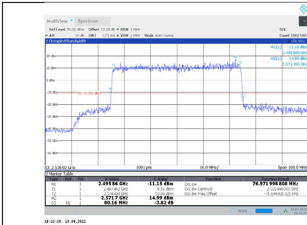
1-N41-PC3-30-80-L-1-CP-QPSK-Outer_Full-217@0-Ant 1-76.972-80.160-≤80-PASS
