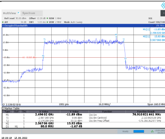
1-N41-PC3-30-80-L-9-DFT-256QAM-Outer_Full-216@0-Ant1-76.911-80.000-≤80-PASS
