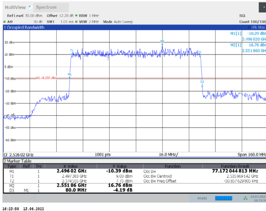
1-N41-PC3-30-80-L-7-DFT-16QAM-Outer_Full-216@0-Ant1-77.172-80.000-≤80-PASS
