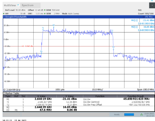
1-N41-PC3-30-50-H-6-DFT-QPSK-Outter_Full-128@0-Ant1 1-45.651-47.600-≤50-PASS
