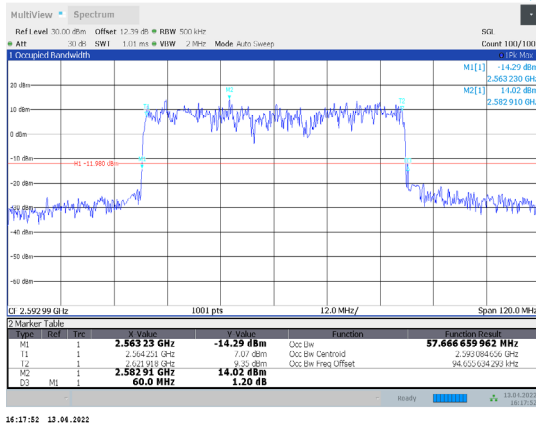
1-N41-PC3-30-60-M-6-DFT-QPSK-Outer_Full-162@0-Ant1-57.667-60.000-≤60-PASS
