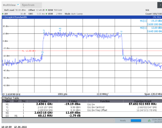
1-N41-PC3-30-60-H-3-CP-64QAM-Outter_Full-162@0-Ant 1-57.653-60.120-≤60-PASS
