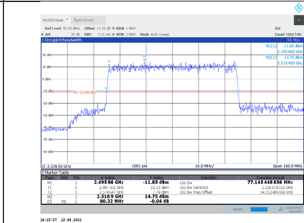
1-N41-PC3-30-80-L-4-CP-256QAM-Outer_Full-217@0-Ant 1-77.145-80.320-≤80-PASS
