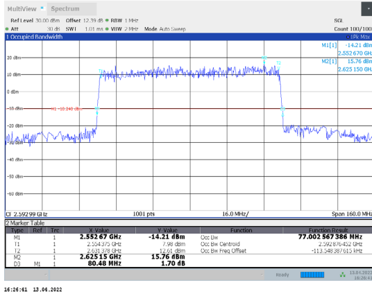
1-N41-PC3-30-80-M-6-DFT-QPSK-Outer_Full-216@0-Ant1-77.003-80.480-≤80-PASS
