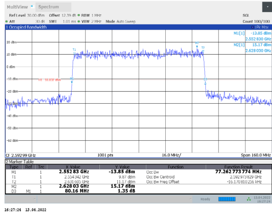
1-N41-PC3-30-80-M-9-DFT-256QAM-Outer_Full-216@0-Ant1-77.263-80.160-≤80-PASS
