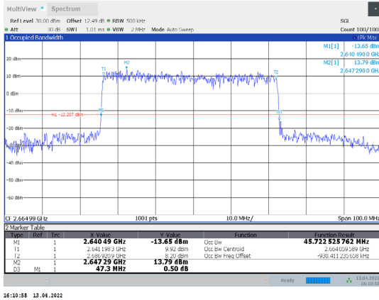
1-N41-PC3-30-50-H-1-CP-QPSK-Outter_Full-133@0-Ant 1-45.723-47.300-≤50-PASS
