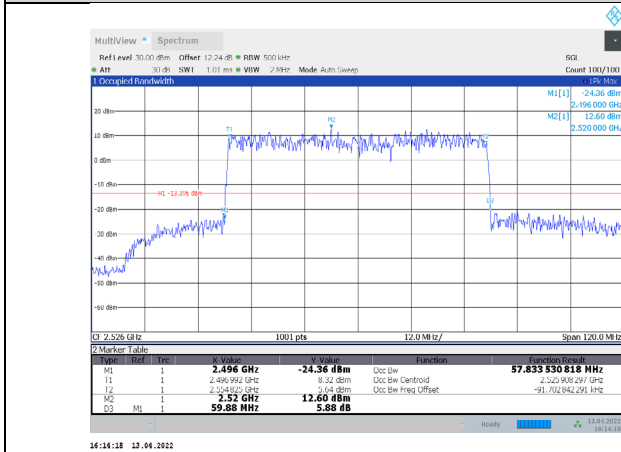
1-N41-PC3-30-60-L-3-CP-64QAM-Outer_Full-162@0-Ant 1-57.834-59.880-≤60-PASS
