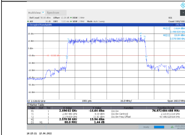
1-N41-PC3-30-80-L-5-DFT-PI/2BPSK-Outer_Full-216@0-Ant 1-76.973-80.000-≤80-PASS
