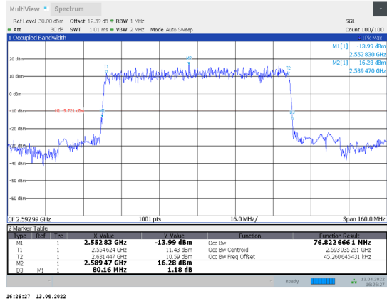
1-N41-PC3-30-80-M-5-DFT-PI/2BPSK-Outer_Full-216@0-Ant1-76.823-80.160-≤80-PASS
