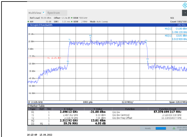
1-N41-PC3-30-60-L-1-CP-QPSK-Outer_Full-162@0-Ant 1-57.378-59.760-≤60-PASS
