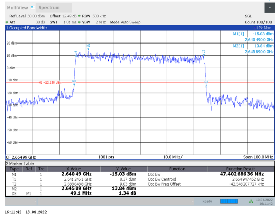
1-N41-PC3-30-50-H-4-CP-256QAM-Outter_Full-133@0-Ant1 1-47.403-49.100-≤50-PASS
