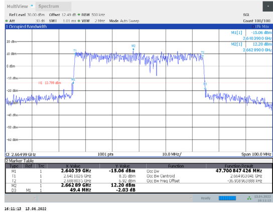
1-N41-PC3-30-50-H-2-CP-16QAM-Outter_Full-133@0-Ant1 1-47.701-49.400-≤50-PASS
