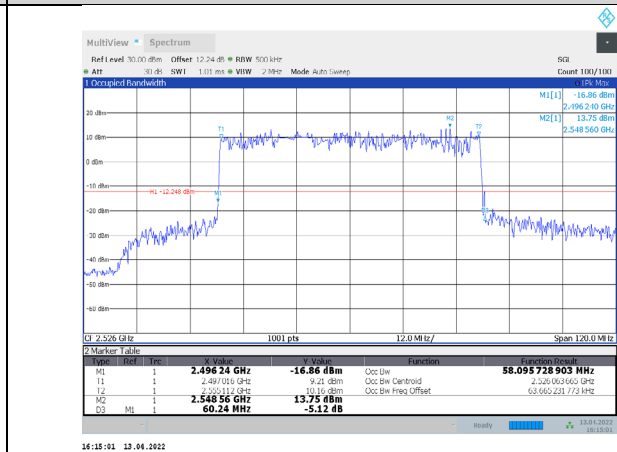
1-N41-PC3-30-60-L-6-DFT-QPSK-Outer_Full-162@0-Ant 1-58.096-60.240-≤60-PASS
