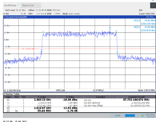
1-N41-PC3-30-60-M-3-CP-64QAM-Outer_Full-162@0-Ant1-57.732-59.640-≤60-PASS
