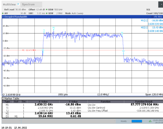
1-N41-PC3-30-60-H-1-CP-QPSK-Outter_Full-162@0-Ant 1-57.777-59.640-≤60-PASS
