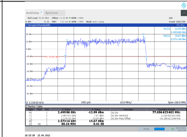
1-N41-PC3-30-80-L-6-DFT-QPSK-Outer_Full-216@0-Ant 1-77.057-80.160-≤80-PASS
