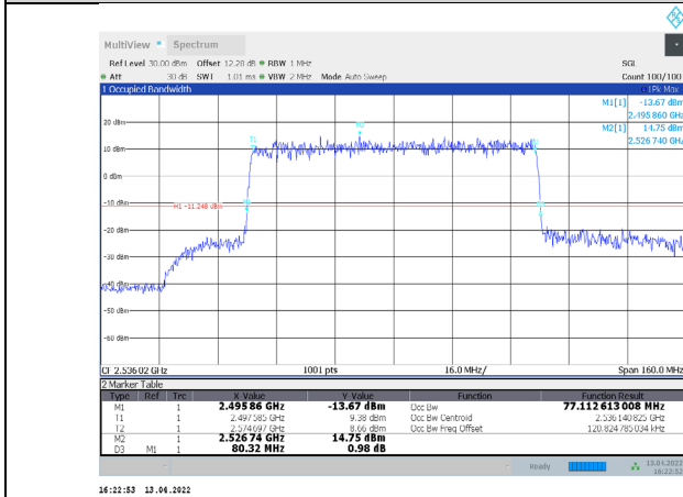
1-N41-PC3-30-80-L-3-CP-64QAM-Outer_Full-217@0-Ant 1-77.113-80.320-≤80-PASS
