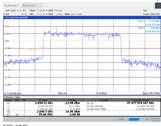
1-N41-PC3-30-60-H-6-DFT-QPSK-Outter_Full-162@0-Ant 1-57.578-59.640-≤60-PASS
