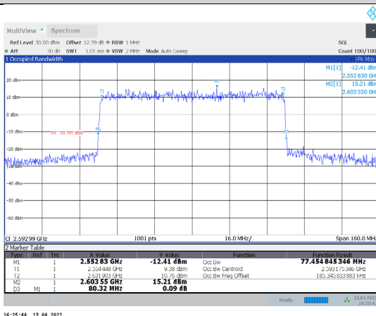
1-N41-PC3-30-80-M-2-CP-16QAM-Outer_Full-217@0-Ant1-77.455-80.320-≤80-PASS
