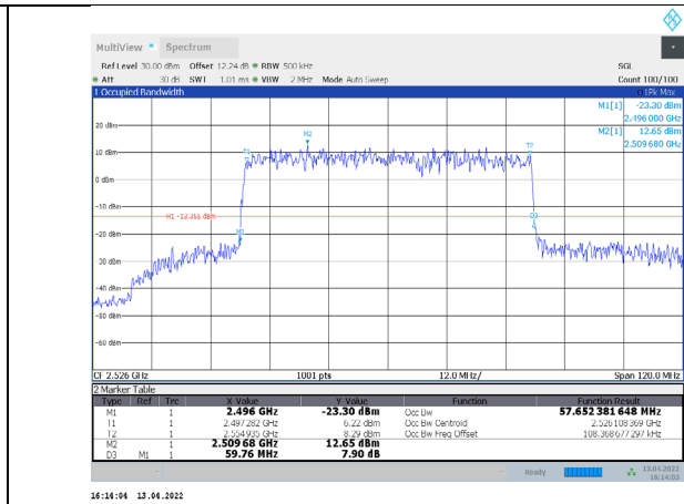
1-N41-PC3-30-60-L-2-CP-16QAM-Outer_Full-162@0-Ant 1-57.652-59.760-≤60-PASS
