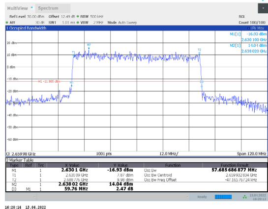
1-N41-PC3-30-60-H-4-CP-256QAM-Outter_Full-162@0-Ant 1-57.686-59.760-≤60-PASS
