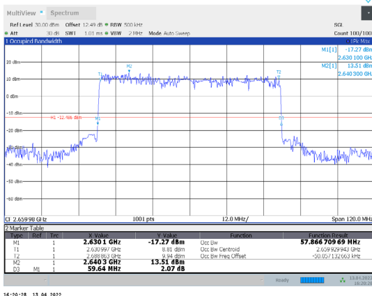
1-N41-PC3-30-60-H-5-DFT-PI/2BPSK-Outter_Full-162@0-Ant 1-57.867-59.640-≤60-PASS
