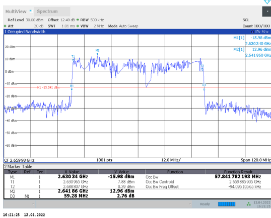
1-N41-PC3-30-60-H-9-DFT-256QAM-Outter_Full-162@0-A nt1-57.842-59.280-≤60-PASS
