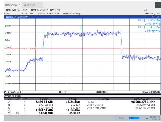
1-N41-PC3-30-100-L-4-CP-256QAM-Outer_Full-273@0-A Ant1-96.908-100.800-≤100-PASS
