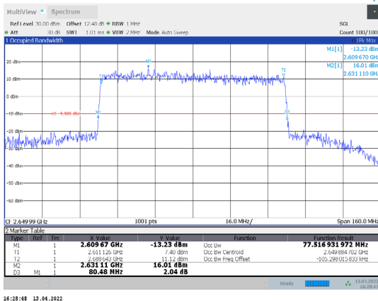
1-N41-PC3-30-80-H-3-CP-64QAM-Outter_Full-217@0-Ant 1-77.517-80.480-≤80-PASS
