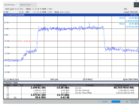
1-N41-PC3-30-100-L-6-DFT-QPSK-Outer_Full-270@0-A Ant1-95.746-99.600-≤100-PASS
