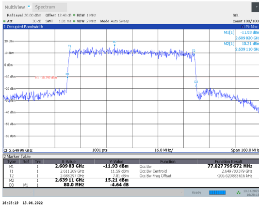
1-N41-PC3-30-80-H-1-CP-QPSK-Outter_Full-217@0-Ant 1-77.028-80.000-≤80-PASS
