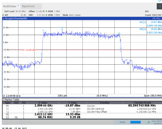
1-N41-PC3-30-90-H-5-DFT-PI/2BPSK-Outter_Full-240@0-Ant1-85.396-88.740-≤90-PASS
