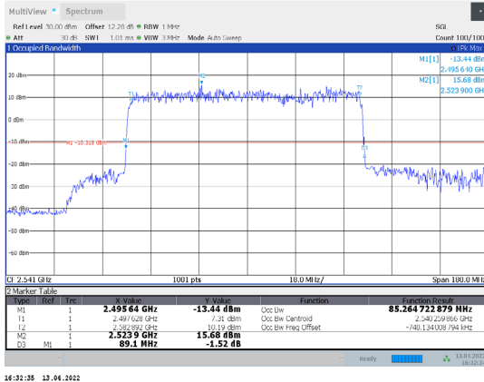
1-N41-PC3-30-90-L-7-DFT-16QAM-Outer_Full-240@0-Ant1-85.265-89.100-≤90-PASS
