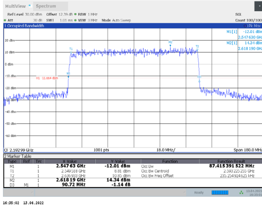
1-N41-PC3-30-90-M-4-CP-256QAM-Outter_Full-245@0-Ant1-87.415-90.720-≤90-PASS
