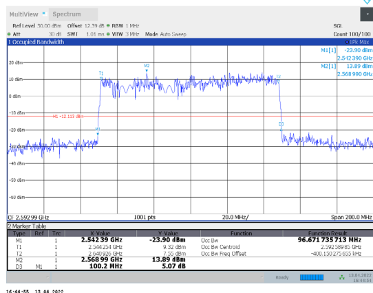
1-N41-PC3-30-100-M-9-DFT-256QAM-Outer_Full-270@ 0-Ant1-96.672-100.200-≤100-PASS
