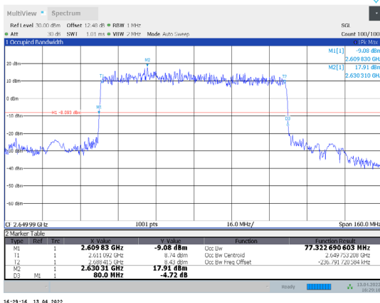
1-N41-PC3-30-80-H-5-DFT-PI/2BPSK-Outter_Full-216@0-Ant 1-77.323-80.000-≤80-PASS
