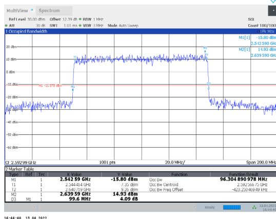
1-N41-PC3-30-100-M-8-DFT-64QAM-Outer_Full-270@ 0-Ant1-96.305-99.600-≤100-PASS
