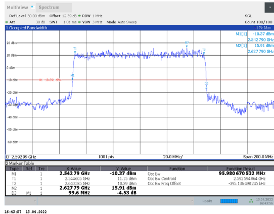
1-N41-PC3-30-100-M-5-DFT-PI/2BPSK-Outer_Full-270 @0-Ant1-95.981-99.600-≤100-PASS
