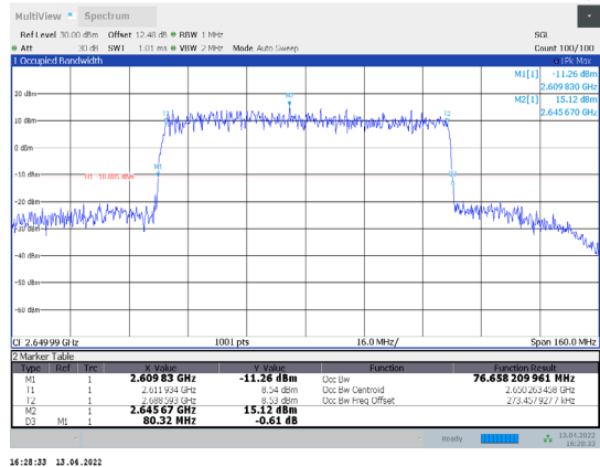
1-N41-PC3-30-80-H-2-CP-16QAM-Outter_Full-217@0-Ant 1-76.658-80.320-≤80-PASS
