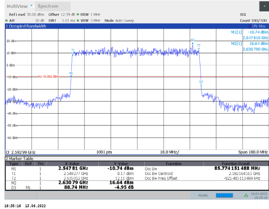
1-N41-PC3-30-90-M-5-DFT-PI/2BPSK-Outter_Full-240@0-Ant1-85.774-88.740-≤90-PASS
