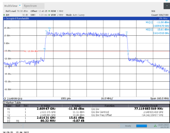
1-N41-PC3-30-80-H-6-DFT-QPSK-Outter_Full-216@0-Ant 1-77.12-80.320-≤80-PASS
