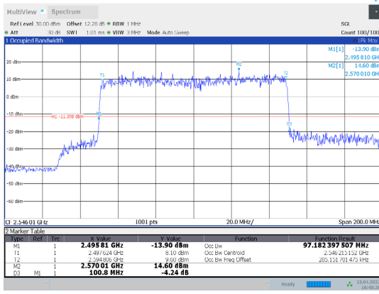
1-N41-PC3-30-100-L-3-CP-64QAM-Outer_Full-273@0-A Ant1-97.182-100.800-≤100-PASS
