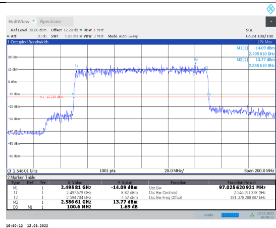
1-N41-PC3-30-100-L-2-CP-16QAM-Outer_Full-273@0-A Ant1-97.026-100.600-≤100-PASS
