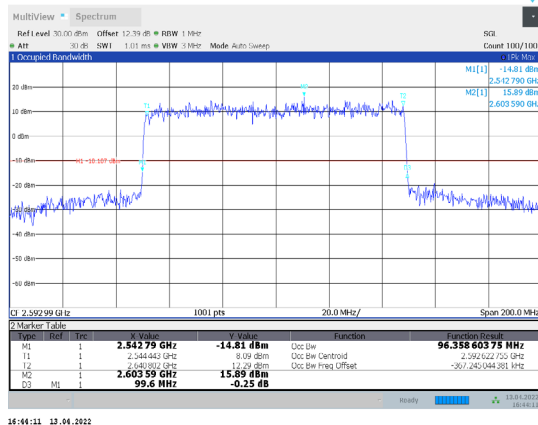
1-N41-PC3-30-100-M-6-DFT-QPSK-Outer_Full-270@0- Ant1-96.359-99.600-≤100-PASS
