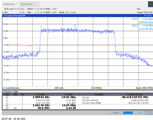
1-N41-PC3-30-90-H-1-CP-QPSK-Outter_Full-245@0-Ant 1-86.418-90.000-≤90-PASS
