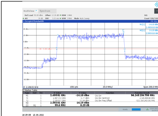
1-N41-PC3-30-100-L-1-CP-QPSK-Outer_Full-273@0-A nt1-96.245-99.600-≤100-PASS
