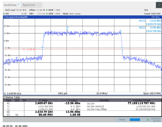
1-N41-PC3-30-80-H-4-CP-256QAM-Outter_Full-217@0-Ant 1-77.185-80.480-≤80-PASS
