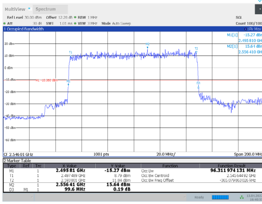
1-N41-PC3-30-100-L-5-DFT-PI/2BPSK-Outer_Full-270@0-A Ant1-96.312-99.600-≤100-PASS
