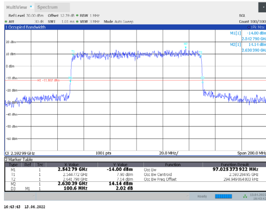
1-N41-PC3-30-100-M-4-CP-256QAM-Outer_Full-273@ 0-Ant1-97.025-100.600-≤100-PASS
