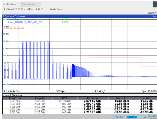
1-N41-PC3-30-20-H-24-CP-QPSK-Inner_Full-25@12-A nt1-PASS-see graph
