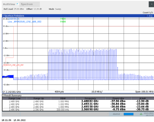
1-N41-PC3-30-100-L-20-DFT-256QAM-Inner_Full-135@67-Ant1-PASS-see graph
