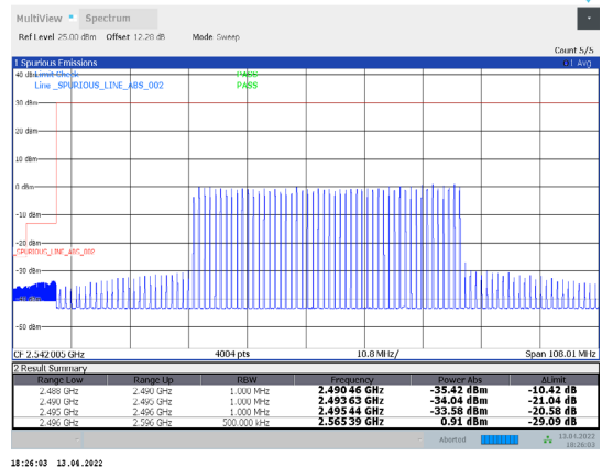
1-N41-PC3-30-100-L-32-CP-64QAM-Inner_Full-137@6 8-Ant1-PASS-see graph
