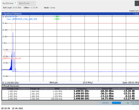
1-N41-PC3-30-100-L-25-CP-16QAM-Edge_1RB_Left-1 @0-Ant1-PASS-see graph
