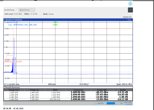
1-N41-PC3-30-100-L-5-DFT-QPSK-Edge_1RB_Left-1@0-Ant1-PASS-see graph
