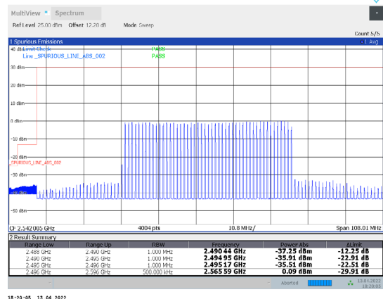
1-N41-PC3-30-100-L-16-DFT-64QAM-Inner_Full-135@6 7-Ant1-PASS-see graph
