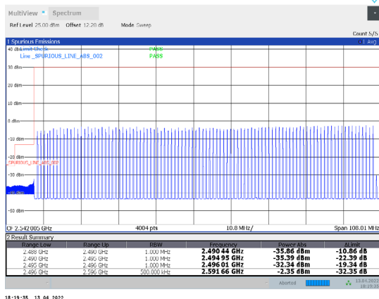
1-N41-PC3-30-100-L-15-DFT-64QAM-Outer_Full-270 @0-Ant1-PASS-see graph
