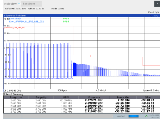
1-N41-PC3-30-20-H-23-CP-QPSK-Outer_Full-51@0-Ant 1-PASS-see graph
