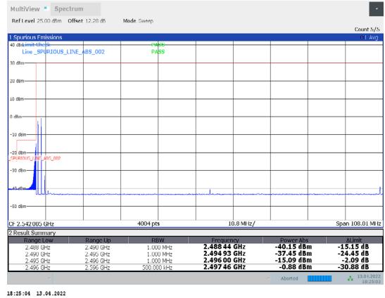
1-N41-PC3-30-100-L-29-CP-64QAM-Edge_1RB_Left-1 @0-Ant1-PASS-see graph
