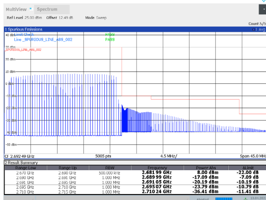
1-N41-PC3-30-20-H-35-CP-256QAM-Outer_Full-51@0-Ant1-PASS-see graph
