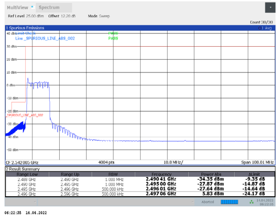
1-N41-PC3-30-100-L-21-CP-QPSK-Edge_1RB_Left-1@0-Ant1-PASS-see graph
