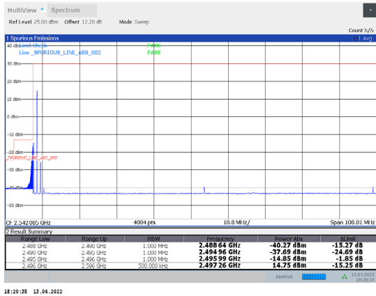
1-N41-PC3-30-100-L-17-DFT-256QAM-Edge_1RB_Left-1@0-Ant1-PASS-see graph
