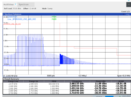
1-N41-PC3-30-20-H-36-CP-256QAM-Inner_Full-25@12-Ant1-PASS-see graph
