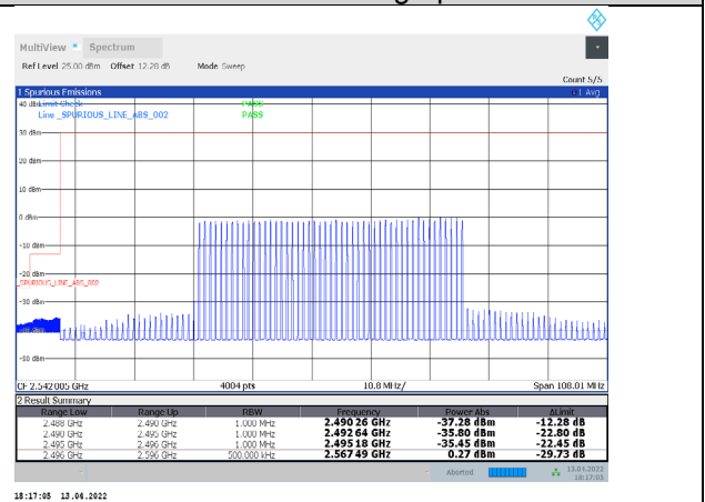
1-N41-PC3-30-100-L-8-DFT-QPSK-Inner_Full-135@67-Ant1-PASS-see graph
