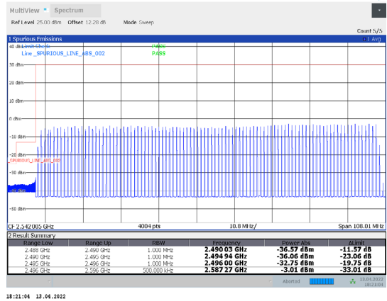
1-N41-PC3-30-100-L-19-DFT-256QAM-Outer_Full-270@0-Ant1-PASS-see graph
