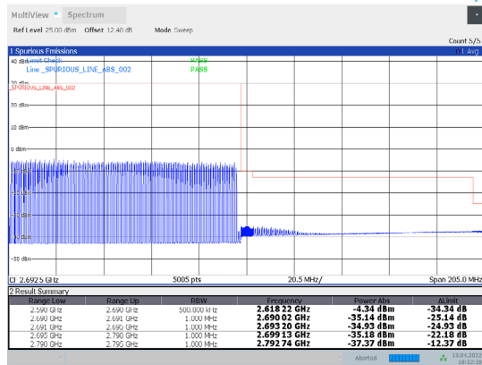
1-N41-PC3-30-100-H-11-DFT-16QAM-Outer_Full-270@0-Ant1-PASS-see graph
