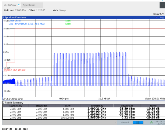
1-N41-PC3-30-100-L-36-CP-256QAM-Inner_Full-137@68 -Ant1-PASS-see graph
