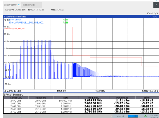
1-N41-PC3-30-20-H-28-CP-16QAM-Inner_Full-25@12-A nt1-PASS-see graph
