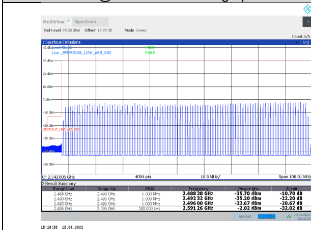
1-N41-PC3-30-100-L-7-DFT-QPSK-Outer_Full-270@0-Ant1-PASS-see graph
