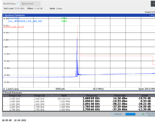
1-N41-PC3-30-100-H-14-DFT-64QAM-Edge_1RB_Rig t-1@272-Ant1-PASS-see graph
