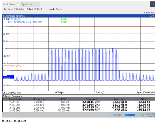
1-N41-PC3-30-100-L-12-DFT-16QAM-Inner_Full-135@ 67-Ant1-PASS-see graph
