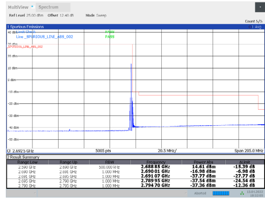
1-N41-PC3-30-100-H-10-DFT-16QAM-Edge_1RB_Right-1@272-Ant1-PASS-see graph
