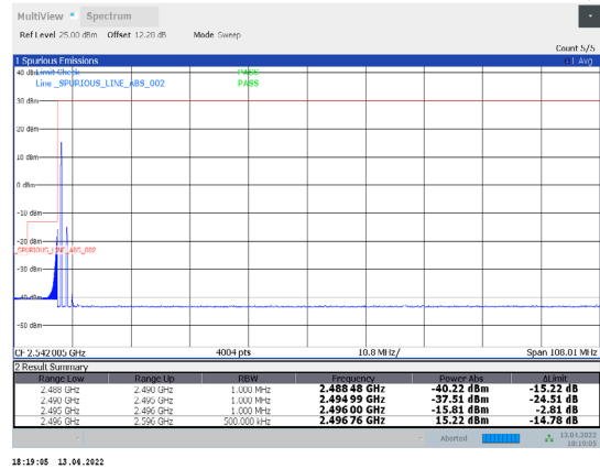
1-N41-PC3-30-100-L-13-DFT-64QAM-Edge_1RB_Left-1 @0-Ant1-PASS-see graph
