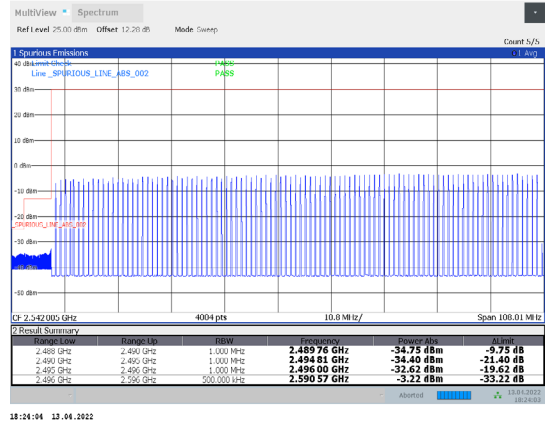
1-N41-PC3-30-100-L-27-CP-16QAM-Outer_Full-273@0 -Ant1-PASS-see graph
