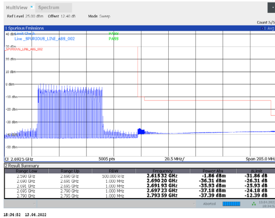
1-N41-PC3-30-100-H-16-DFT-64QAM-Inner_Full-135@ 67-Ant1-PASS-see graph
