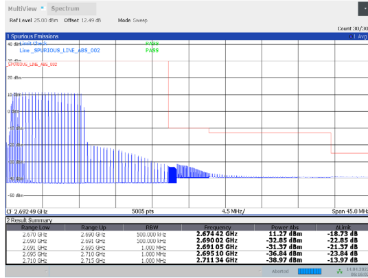
1-N41-PC3-30-20-H-22-CP-QPSK-Edge_1RB_Right-1 @50-Ant1-PASS-see graph
