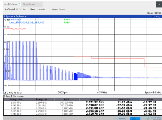
1-N41-PC3-30-20-H-34-CP-256QAM-Edge_1RB_Right-1@50-Ant1-PASS-see graph
