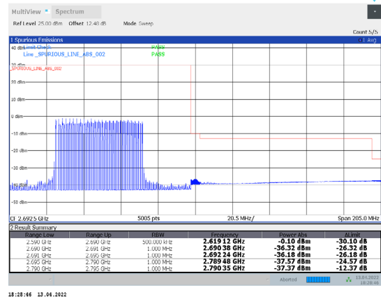
1-N41-PC3-30-100-H-1-DFT-PI/2BPSK-Inner_Full-13 5@67-Ant1-PASS-see graph
