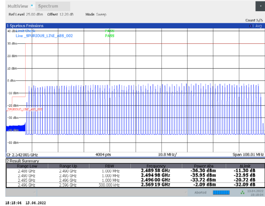
1-N41-PC3-30-100-L-11-DFT-16QAM-Outer_Full-270@ 0-Ant1-PASS-see graph
