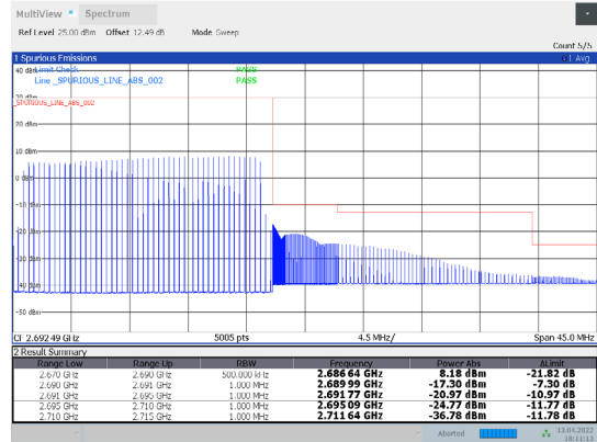
1-N41-PC3-30-20-H-31-CP-64QAM-Outer_Full-51@0-Ant1-PASS-see graph
