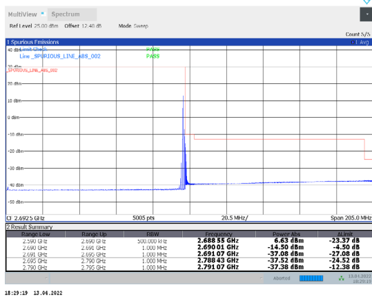
1-N41-PC3-30-100-H-3-DFT-PI/2BPSK-Edge_1RB_Right-1 @272-Ant1-PASS-see graph
