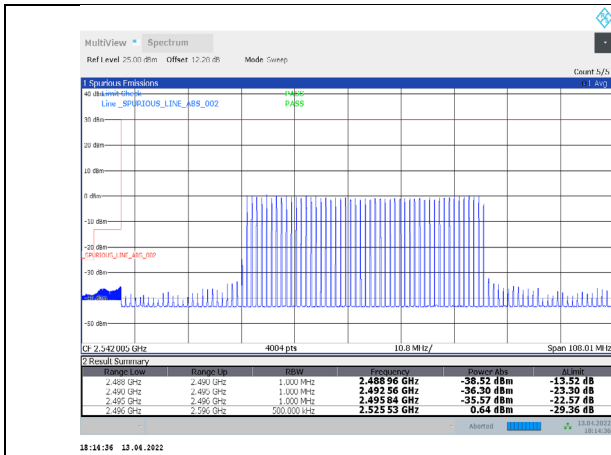
1-N41-PC3-30-100-L-1-DFT-PI/2BPSK-Inner_Full-135 @67-Ant1-PASS-see graph
