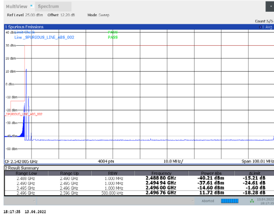
1-N41-PC3-30-100-L-9-DFT-16QAM-Edge_1RB_Left-1 @0-Ant1-PASS-see graph
