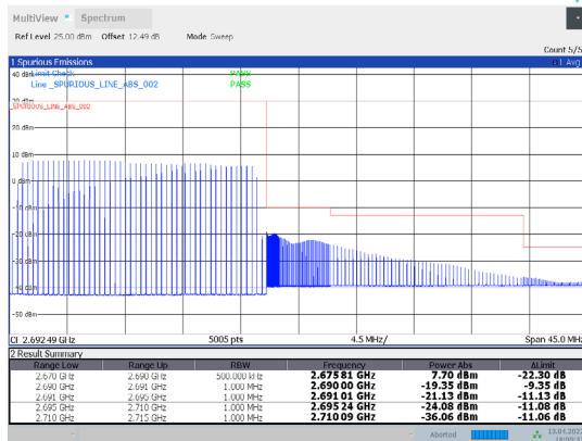
1-N41-PC3-30-20-H-27-CP-16QAM-Outer_Full-51@0-Ant1-PASS-see graph
