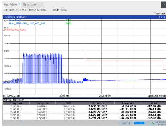
1-N41-PC3-30-100-H-8-DFT-QPSK-Inner_Full-135@67-Ant1-PASS-see graph
