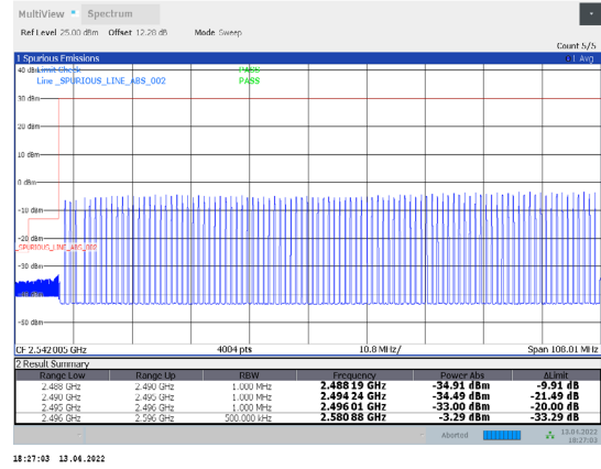
1-N41-PC3-30-100-L-35-CP-256QAM-Outer_Full-273 @0-Ant1-PASS-see graph
