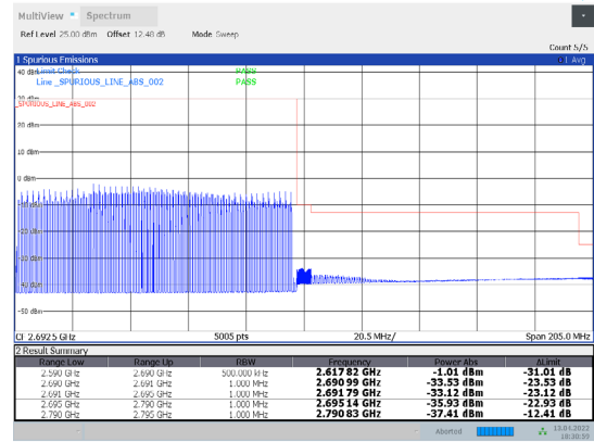
1-N41-PC3-30-100-H-7-DFT-QPSK-Outer_Full-270@0-Ant1-PASS-see graph
