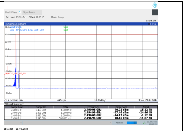
1-N41-PC3-30-100-L-2-DFT-PI/2BPSK-Edge_1RB_Left-1@0-Ant1-PASS-see graph
