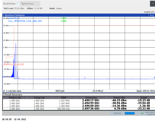
1-N41-PC3-30-100-L-33-CP-256QAM-Edge_1RB_Left-1 @0-Ant1-PASS-see graph
