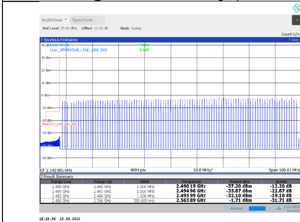
1-N41-PC3-30-100-L-4-DFT-PI/2BPSK-Outer_Full-270 @0-Ant1-PASS-see graph
