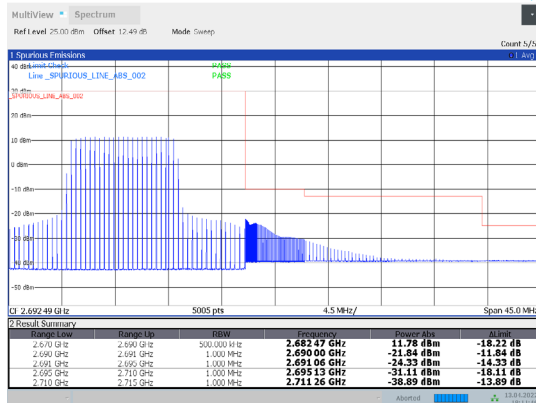
1-N41-PC3-30-20-H-32-CP-64QAM-Inner_Full-25@12-Ant1-PASS-see graph
