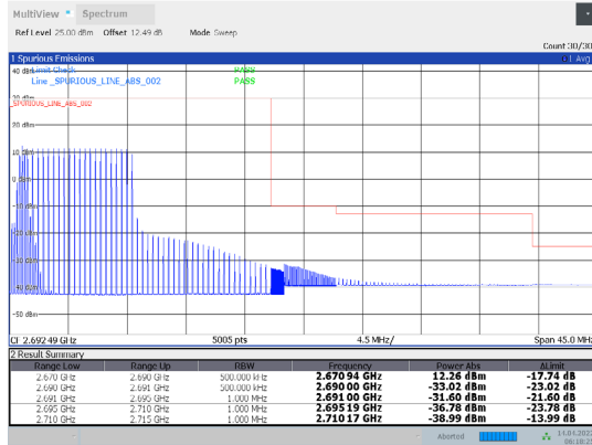
1-N41-PC3-30-20-H-30-CP-64QAM-Edge_1RB_Right-1@50-Ant1-PASS-see graph
