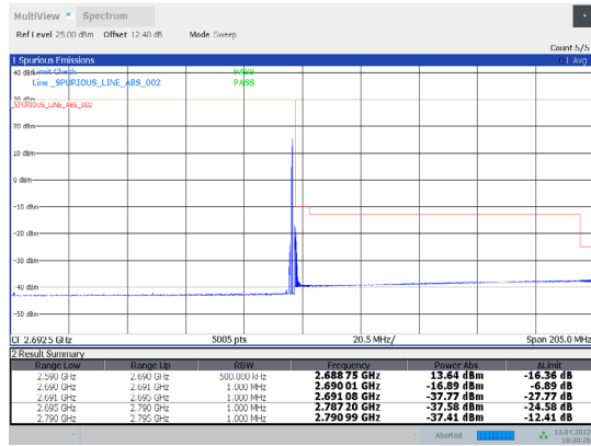
1-N41-PC3-30-100-H-6-DFT-QPSK-Edge_1RB_Right-1@272-Ant1-PASS-see graph
