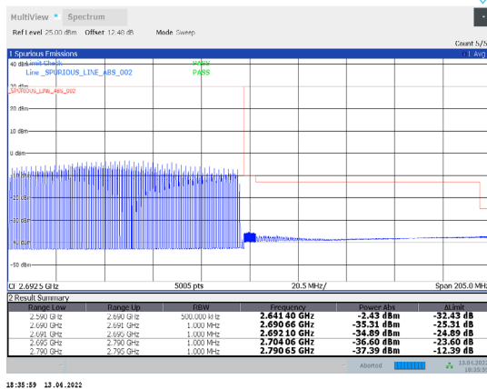
1-N41-PC3-30-100-H-19-DFT-256QAM-Outer_Full-270 @0-Ant1-PASS-see graph
