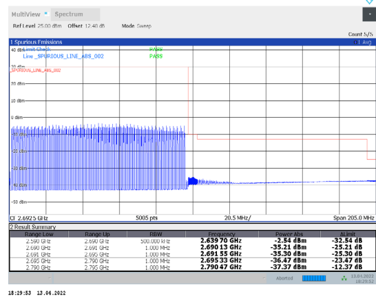
1-N41-PC3-30-100-H-4-DFT-PI/2BPSK-Outer_Full-27 0@0-Ant1-PASS-see graph
