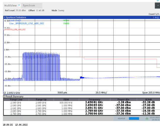
1-N41-PC3-30-100-H-20-DFT-256QAM-Inner_Full-135 @67-Ant1-PASS-see graph
