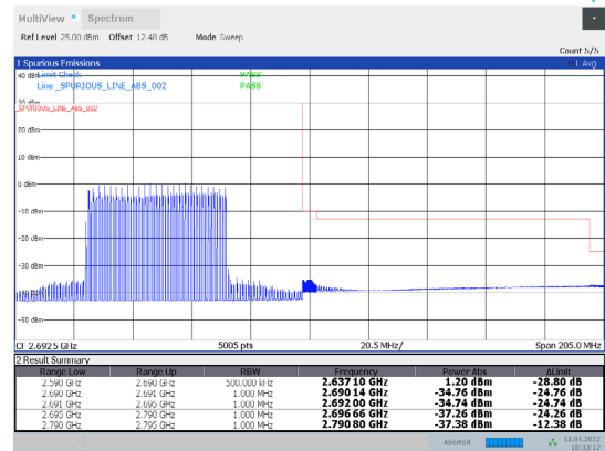
1-N41-PC3-30-100-H-12-DFT-16QAM-Inner_Full-135@67-Ant1-PASS-see graph
