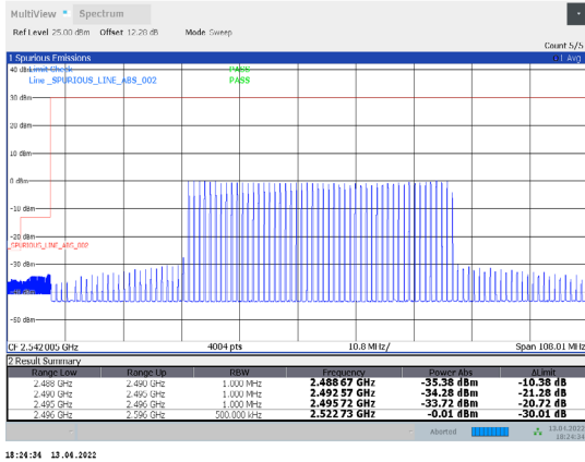
1-N41-PC3-30-100-L-28-CP-16QAM-Inner_Full-137@6 8-Ant1-PASS-see graph
