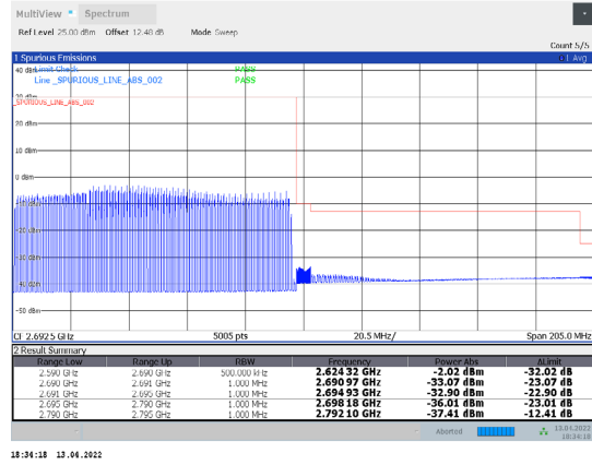
1-N41-PC3-30-100-H-15-DFT-64QAM-Outer_Full-270@ 0-Ant1-PASS-see graph
