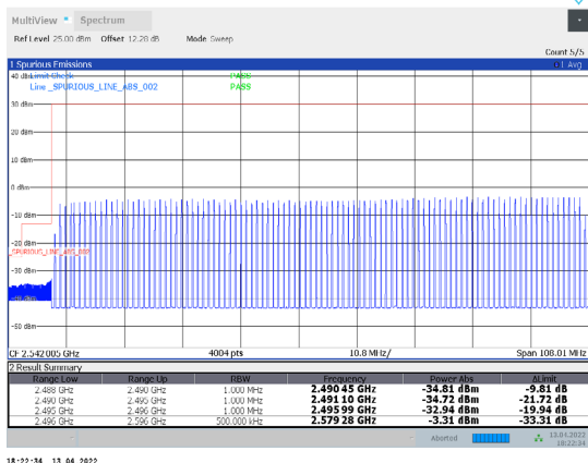
1-N41-PC3-30-100-L-23-CP-QPSK-Outer_Full-273@0-Ant1-PASS-see graph
