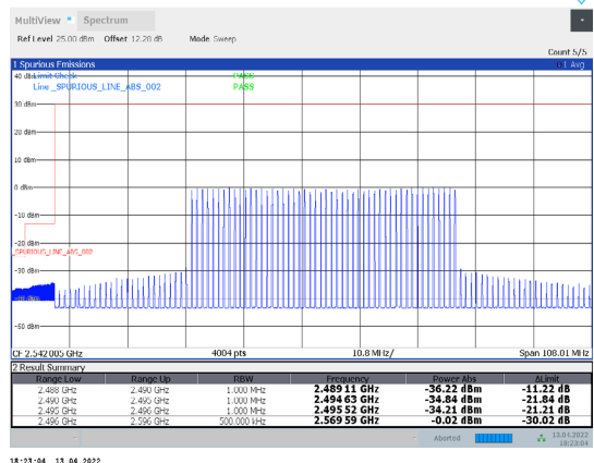
1-N41-PC3-30-100-L-24-CP-QPSK-Inner_Full-137@68-Ant1-PASS-see graph
