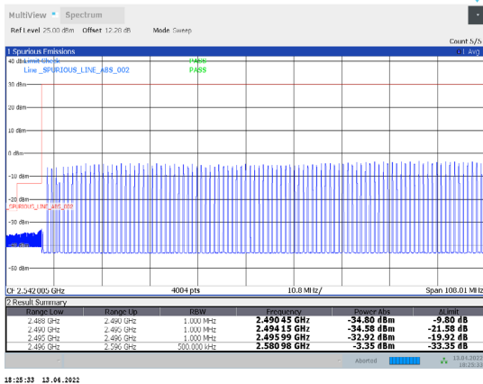
1-N41-PC3-30-100-L-31-CP-64QAM-Outer_Full-273@0 -Ant1-PASS-see graph
