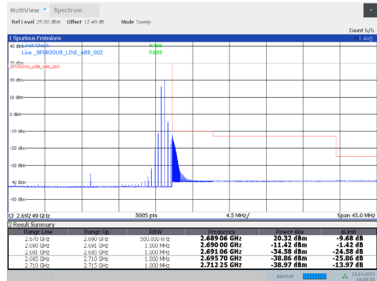
1-N41-PC3-30-20-H-26-CP-16QAM-Edge_1RB_Right-1 @50-Ant1-PASS-see graph
