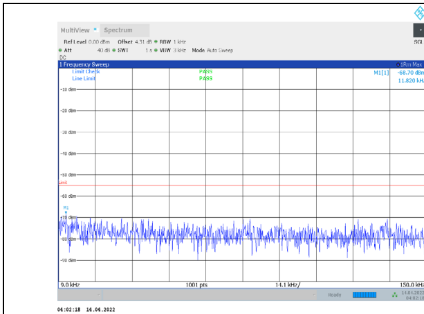
1-N41-PC3-30-20-H-3-CP-QPSK-Outer_Full-51@0-0.0 09-0.15-Ant1--68.70--55-PASS
