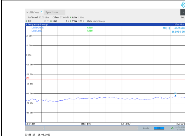
1-N41-PC3-30-20-L-3-CP-QPSK-Outer_Full-51@0-300 0-18000-Ant1--43.05--25-PASS
