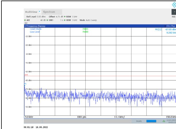
1-N41-PC3-30-20-H-2-CP-QPSK-Edge_1RB_Right-1@ 50-0.009-0.15-Ant1--67.05--55-PASS
