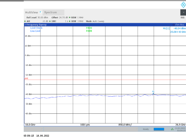
1-N41-PC3-30-20-L-2-CP-QPSK-Edge_1RB_Right-1@5 0-18000-26900-Ant1--40.34--25-PASS
