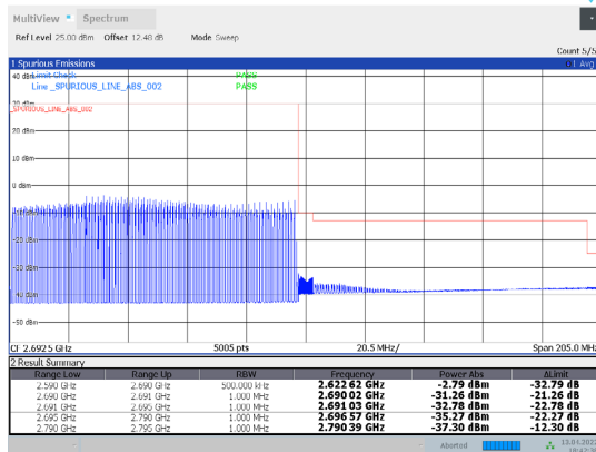
1-N41-PC3-30-100-H-35-CP-256QAM-Outer_Full-273 @0-Ant1-PASS-see graph
