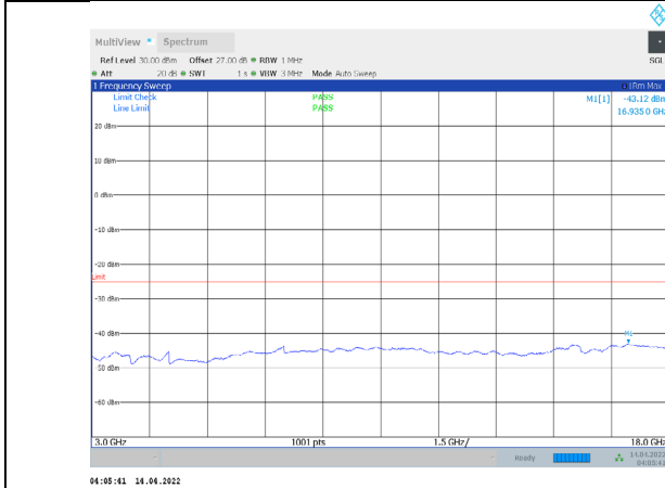
1-N41-PC3-30-60-L-2-CP-QPSK-Edge_1RB_Right-1@ 161-3000-18000-Ant1--43.12--25-PASS
