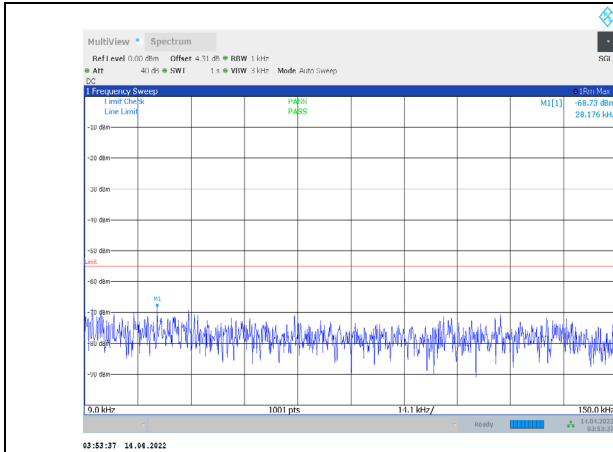
1-N41-PC3-30-20-L-2-CP-QPSK-Edge_1RB_Right-1@ 50-0.009-0.15-Ant1--68.73--55-PASS
