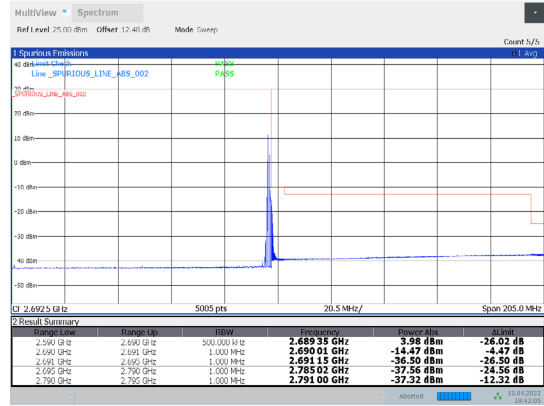
1-N41-PC3-30-100-H-34-CP-256QAM-Edge_1RB_Right -1@272-Ant1-PASS-see graph
