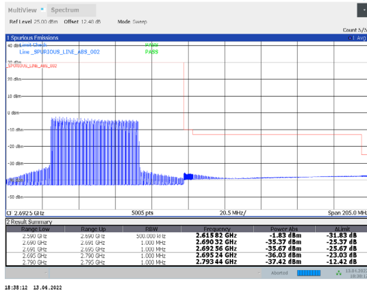
1-N41-PC3-30-100-H-24-CP-QPSK-Inner_Full-137@68-Ant1-PASS-see graph
