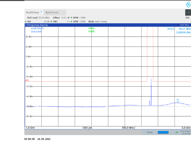
1-N41-PC3-30-20-L-2-CP-QPSK-Edge_1RB_Right-1@5 0-1000-3000-Ant1--46.27--25-PASS
