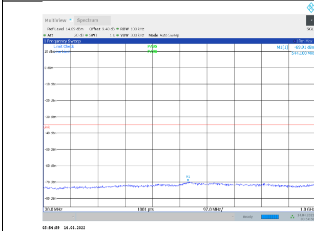
1-N41-PC3-30-20-L-3-CP-QPSK-Outer_Full-51@0-30- 1000-Ant1--69.91--35-PASS
