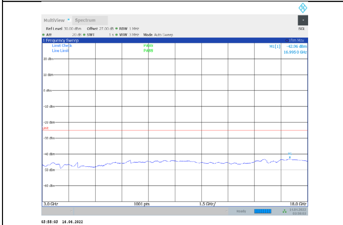
1-N41-PC3-30-20-M-2-CP-QPSK-Edge_1RB_Right-1@ 50-3000-18000-Ant1--42.96--25-PASS
