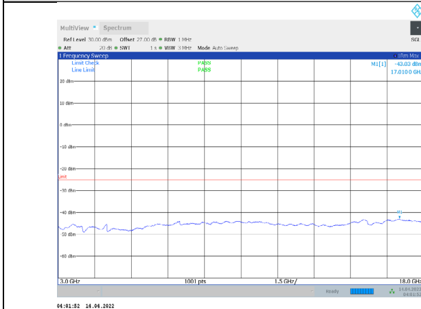
1-N41-PC3-30-20-H-2-CP-QPSK-Edge_1RB_Right-1@ 50-3000-18000-Ant1--43.03--25-PASS
