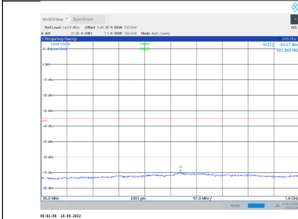
1-N41-PC3-30-20-H-2-CP-QPSK-Edge_1RB_Right-1@ 50-30-1000-Ant1--69.57--35-PASS
