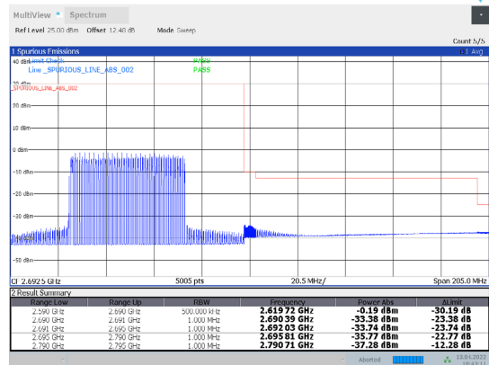
1-N41-PC3-30-100-H-36-CP-256QAM-Inner_Full-137@68-Ant1-PASS-see graph
