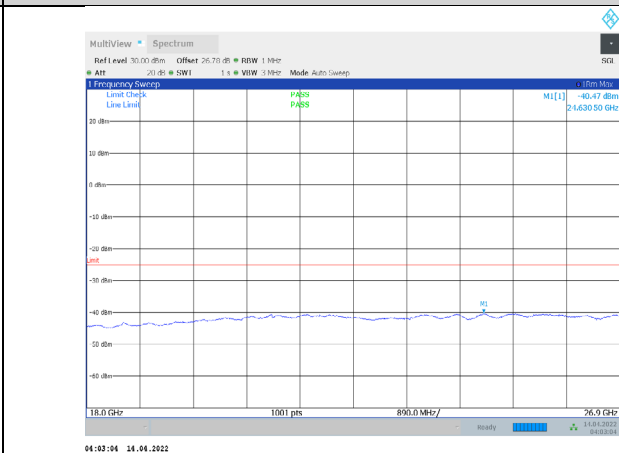
1-N41-PC3-30-20-H-3-CP-QPSK-Outer_Full-51@0-180 00-26900-Ant1--40.47--25-PASS
