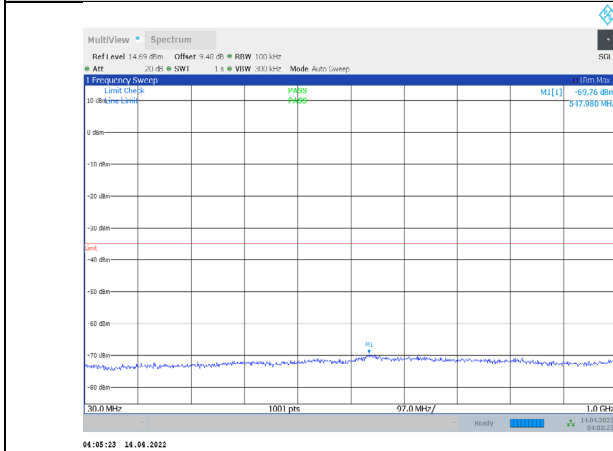
1-N41-PC3-30-60-L-2-CP-QPSK-Edge_1RB_Right-1@ 161-30-1000-Ant1--69.76--35-PASS
