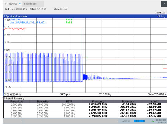
1-N41-PC3-30-100-H-31-CP-64QAM-Outer_Full-273@0 -Ant1-PASS-see graph
