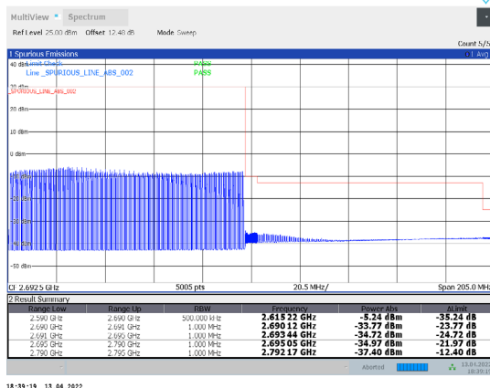
1-N41-PC3-30-100-H-27-CP-16QAM-Outer_Full-273@0-Ant1-PASS-see graph
