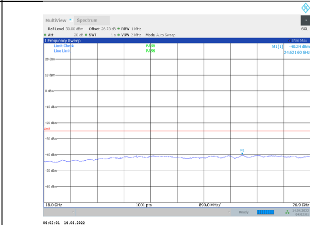
1-N41-PC3-30-20-H-2-CP-QPSK-Edge_1RB_Right-1@ 50-18000-26900-Ant1--40.34--25-PASS
