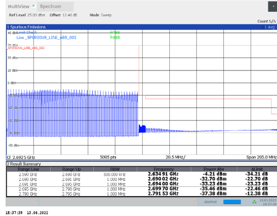
1-N41-PC3-30-100-H-23-CP-QPSK-Outer_Full-273@0-Ant1-PASS-see graph
