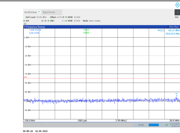
1-N41-PC3-30-60-L-2-CP-QPSK-Edge_1RB_Right-1@ 61-0.15-30-Ant1--65.12--45-PASS
