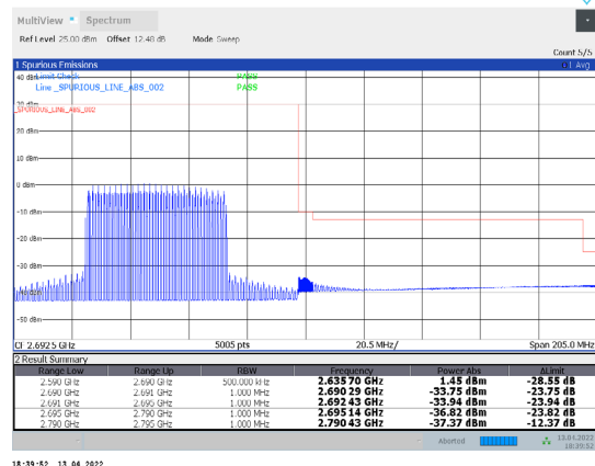
1-N41-PC3-30-100-H-28-CP-16QAM-Inner_Full-137@68-Ant1-PASS-see graph
