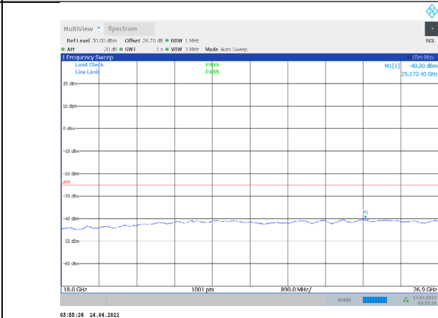
1-N41-PC3-30-20-L-3-CP-QPSK-Outer_Full-51@0-1800 0-26900-Ant1--40.30--25-PASS
