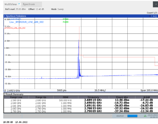
1-N41-PC3-30-100-H-26-CP-16QAM-Edge_1RB_Right-1@272-Ant1-PASS-see graph
