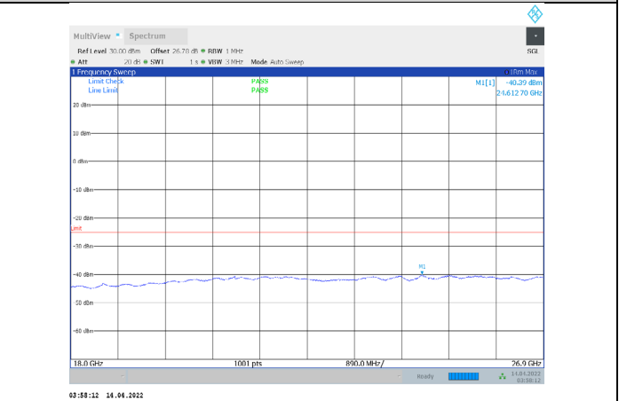
1-N41-PC3-30-20-M-2-CP-QPSK-Edge_1RB_Right-1@ 50-18000-26900-Ant1--40.39--25-PASS
