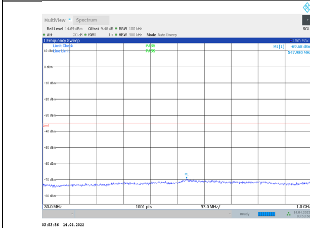
1-N41-PC3-30-20-L-2-CP-QPSK-Edge_1RB_Right-1@ 50-30-1000-Ant1--69.68--35-PASS
