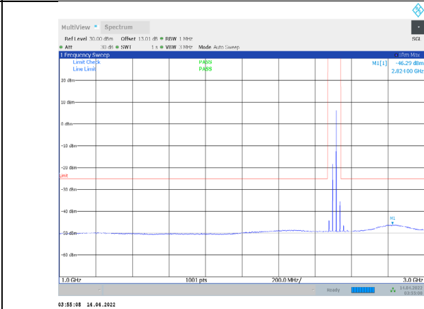
1-N41-PC3-30-20-L-3-CP-QPSK-Outer_Full-51@0-1000- 3000-Ant1--46.29--25-PASS
