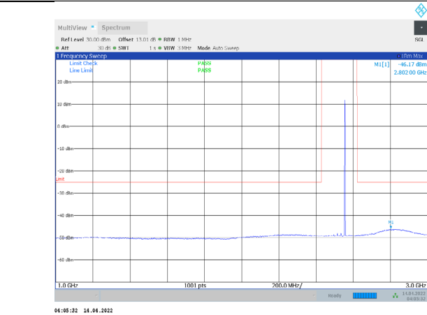
1-N41-PC3-30-60-L-2-CP-QPSK-Edge_1RB_Right-1@ 61-1000-3000-Ant1--46.17--25-PASS
