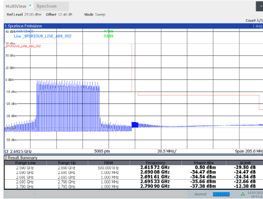
1-N41-PC3-30-100-H-32-CP-64QAM-Inner_Full-137@6 8-Ant1-PASS-see graph
