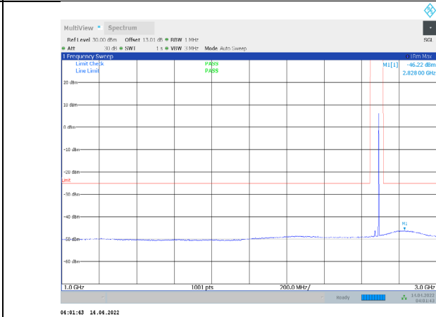
1-N41-PC3-30-20-H-2-CP-QPSK-Edge_1RB_Right-1@ 50-1000-3000-Ant1--46.22--25-PASS
