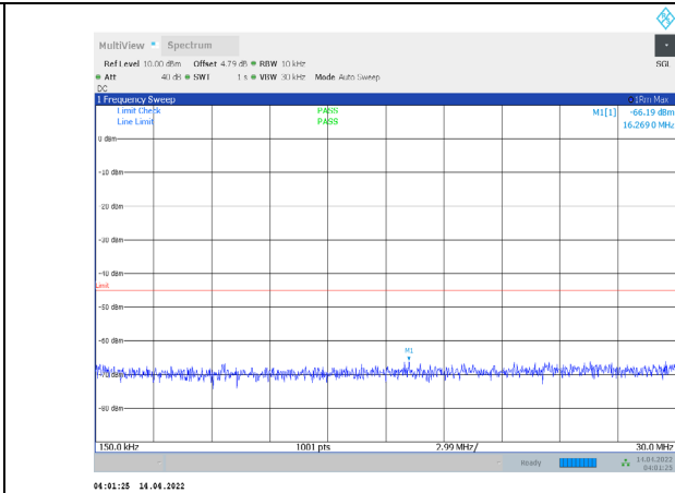
1-N41-PC3-30-20-H-2-CP-QPSK-Edge_1RB_Right-1@ 50-0.15-30-Ant1--66.19--45-PASS
