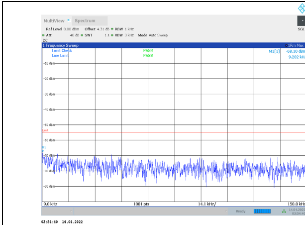
1-N41-PC3-30-20-L-3-CP-QPSK-Outer_Full-51@0-0.0 09-0.15-Ant1--68.10--55-PASS
