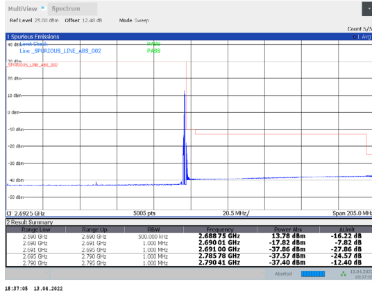
1-N41-PC3-30-100-H-22-CP-QPSK-Edge_1RB_Right-1@272-Ant1-PASS-see graph
