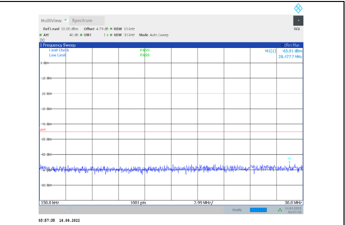
1-N41-PC3-30-20-M-2-CP-QPSK-Edge_1RB_Right-1@ 50-0.15-30-Ant1--65.91--45-PASS
