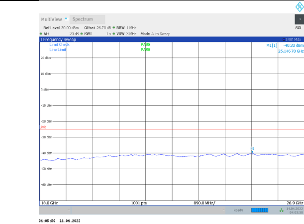
1-N41-PC3-30-60-L-2-CP-QPSK-Edge_1RB_Right-1@ 61-18000-26900-Ant1--40.33--25-PASS
