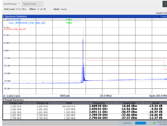
1-N41-PC3-30-100-H-30-CP-64QAM-Edge_1RB_Right -1@272-Ant1-PASS-see graph
