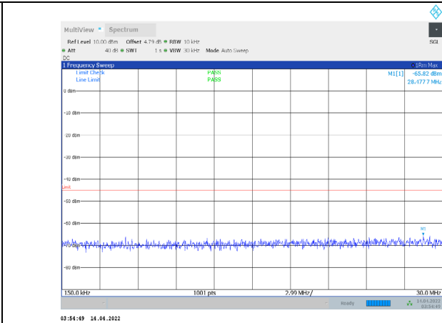
1-N41-PC3-30-20-L-3-CP-QPSK-Outer_Full-51@0-0.15- 30-Ant1--65.82--45-PASS
