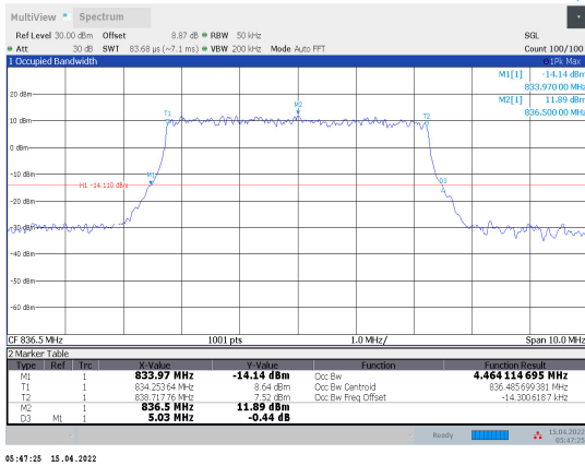
1-N5-PC3-15-5-M-4-CP-256QAM-Outter_Full-25@ 0-Ant1-4.464-5.030-≤5-PASS
