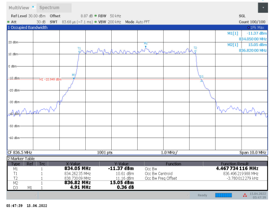
1-N5-PC3-15-5-M-5-DFT-PI/2BPSK-Outter_Full-25@ 0-Ant1-4.468-4.910-≤5-PASS
