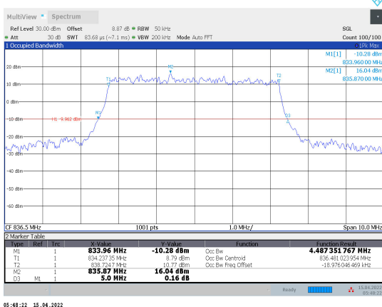
1-N5-PC3-15-5-M-8-DFT-64QAM-Outter_Full-25@ 0-Ant1-4.487-5.000-≤5-PASS
