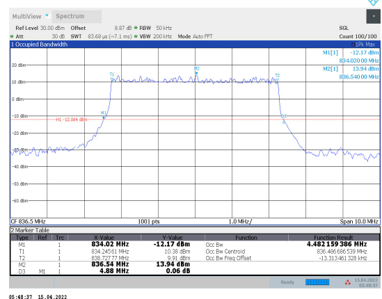
1-N5-PC3-15-5-M-9-DFT-256QAM-Outter_Full-25@ 0-Ant1-4.482-4.880-≤5-PASS
