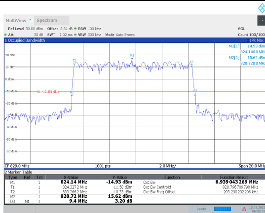
1-N5-PC3-15-10-L-6-DFT-QPSK-Out_52@0 -Ant1-8.939-9.400-≤10-PASS
