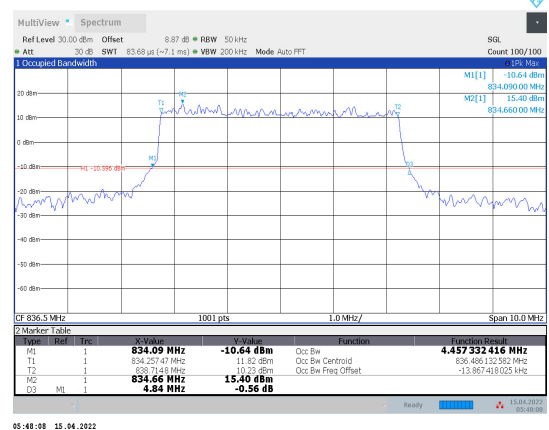
1-N5-PC3-15-5-M-7-DFT-16QAM-Outter_Full-25@0- Ant1-4.457-4.840-≤5-PASS
