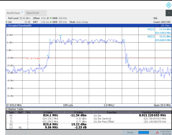
1-N5-PC3-15-10-L-7-DFT-16QAM-Out_52@0- Ant1-8.921-9.560-≤10-PASS
