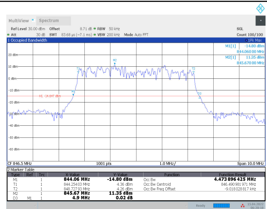
1-N5-PC3-15-5-H-2-CP-16QAM-Outter_Full-25@0-Ant1-4.454-4.920-≤5-PASS
