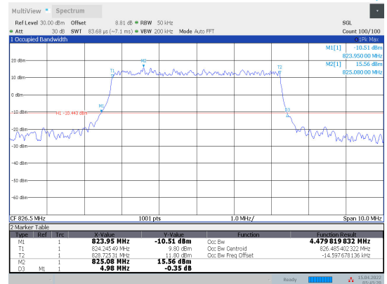
1-N5-PC3-15-5-L-8-DFT-64QAM-Outter_Full-25@0-Ant1-4.48-4.980-≤5-PASS
