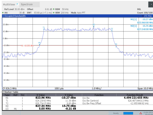
1-N5-PC3-15-5-L-7-DFT-16QAM-Outter_Full-25@0-Ant1-4.494-5.050-≤5-PASS
