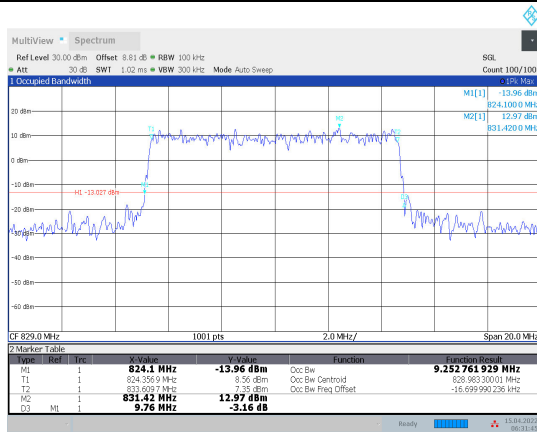
1-N5-PC3-15-10-L-2-CP-16QAM-Out_52@ 0-Ant1-9.253-9.760-≤10-PASS
