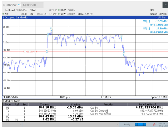
1-N5-PC3-15-5-H-7-DFT-16QAM-Outer_Full-25@0-Ant1-4.422-4.620-≤5-PASS
