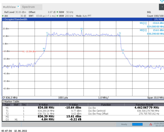
1-N5-PC3-15-5-M-6-DFT-QPSK-Outter_Full-25@0- Ant1-4.462-4.840-≤5-PASS
