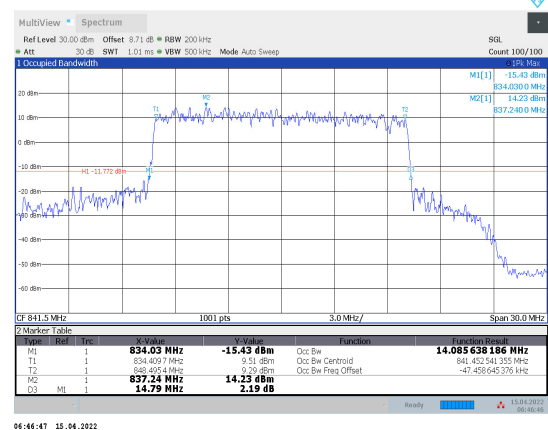
1-N5-PC3-15-15-H-2-CP-16QAM-Outter_Full-79@0- Ant1-14.086-14.790≤15-PASS
