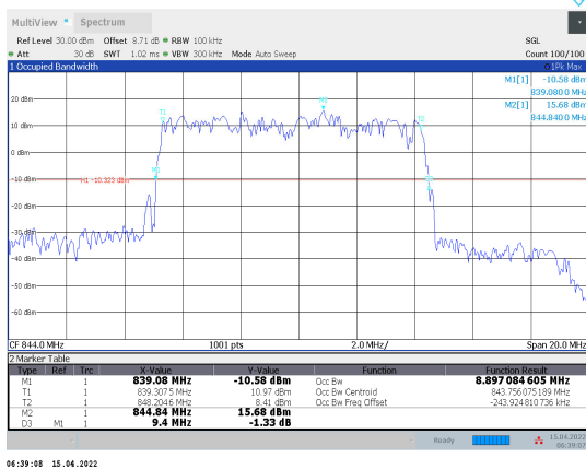
1-N5-PC3-15-10-H-6-DFT-QPSK-Out_50@0 -Ant1-8.897-9.400-≤10-PASS
