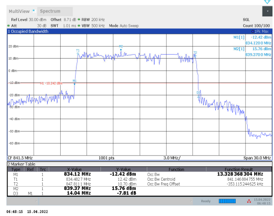
1-N5-PC3-15-15-H-8-DFT-64QAM-Outter_Full-75 @0-Ant1-13.328-14.040-≤15-PASS
