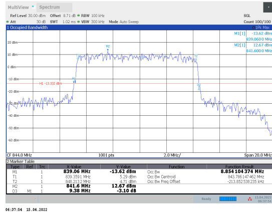
1-N5-PC3-15-10-H-1-CP-QPSK-Outter_Full-50@0-Ant1-8.854-9.380-≤10-PASS
