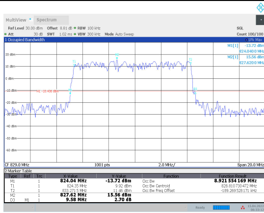
1-N5-PC3-15-10-L-8-DFT-64QAM-Out_50@0-Ant1-8.922-9.580-≤10-PASS
