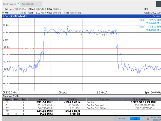
1-N5-PC3-15-10-M-5-DFT-PI/2BPSK-Outter_Full-50 @0-Ant1-8.93-9.280-≤10-PASS
