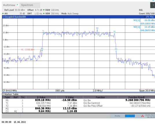
1-N5-PC3-15-10-H-2-CP-16QAM-Out_52@ 0-Ant1-9.268-9.640-≤10-PASS
