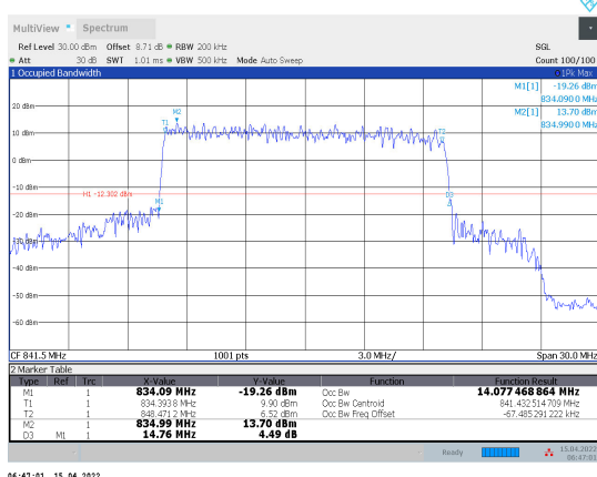
1-N5-PC3-15-15-H-3-CP-64QAM-Outter_Full-79@0 -Ant1-14.077-14.760≤15-PASS
