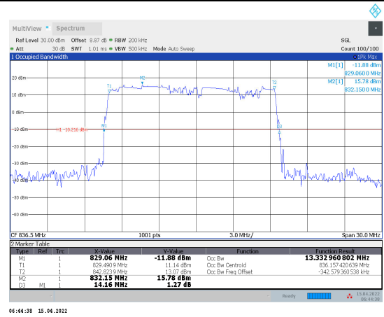
1-N5-PC3-15-15-M-5-DFT-PI/2BPSK-Outer_Full-75 @0-Ant1-13.333-14.160≤15-PASS
