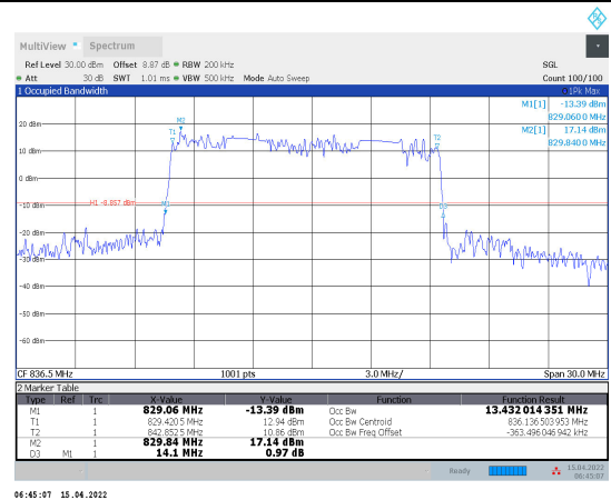
1-N5-PC3-15-15-M-7-DFT-16QAM-Outer_Full-75@ 0-Ant1-13.432-14.100≤15-PASS
