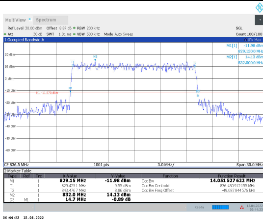
1-N5-PC3-15-15-M-4-CP-256QAM-Outer_Full-79 @0-Ant1-14.052-14.700≤15-PASS
