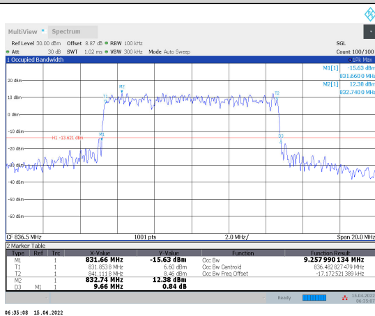
1-N5-PC3-15-10-M-3-CP-64QAM-Out_52@0-Ant1-9.258-9.660-≤10-PASS
