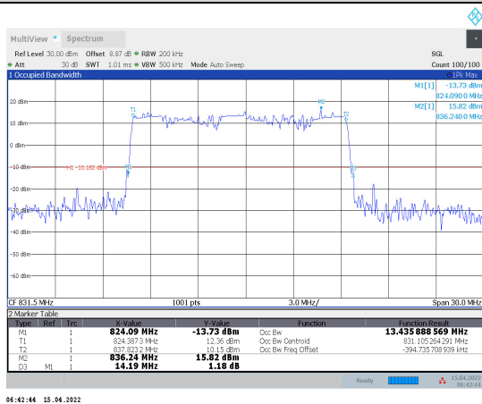
1-N5-PC3-15-15-L-9-DFT-256QAM-Outter_Full-75@0-Ant1-13.436-14.190-≤15-PASS
