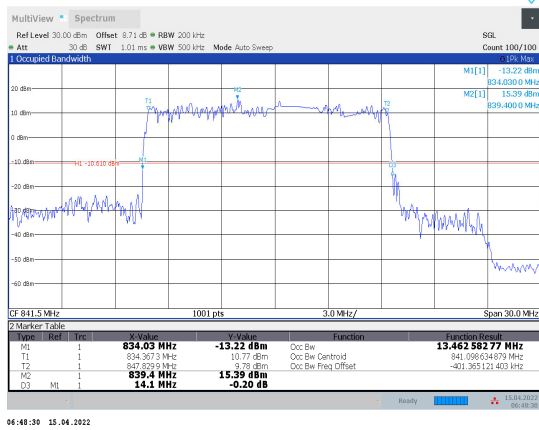
1-N5-PC3-15-15-H-9-DFT-256QAM-Outter_Full-75@ 0-Ant1-13.463-14.100-≤15-PASS
