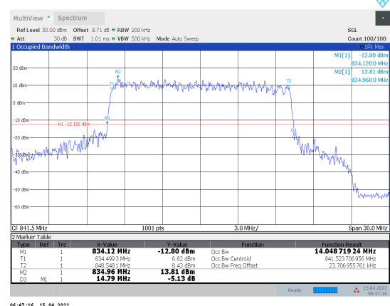
1-N5-PC3-15-15-H-4-CP-256QAM-Outter_Full-79@ 0-Ant1-14.049-14.790≤15-PASS
