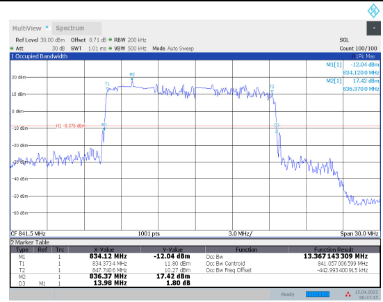
1-N5-PC3-15-15-H-6-DFT-QPSK-Outter_Full-75@0 -Ant1-13.367-13.980-≤15-PASS
