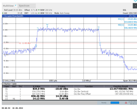
1-N5-PC3-15-15-H-1-CP-QPSK-Outter_Full-75@0- Ant1-13.448-14.130≤15-PASS
