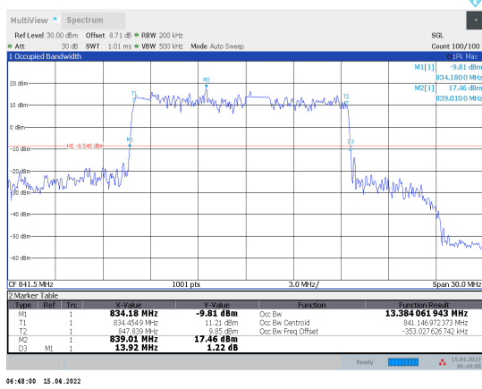
1-N5-PC3-15-15-H-7-DFT-16QAM-Outter_Full-75@0 -Ant1-13.384-13.920-≤15-PASS
