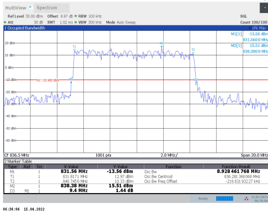
1-N5-PC3-15-10-M-7-DFT-16QAM-Outter_Full-50@0-Ant1-8.928-9.400-≤10-PASS
