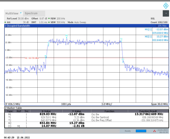
1-N5-PC3-15-15-M-1-CP-QPSK-Outter_Full-75@0-Ant1-13.318-14.070-≤15-PASS
