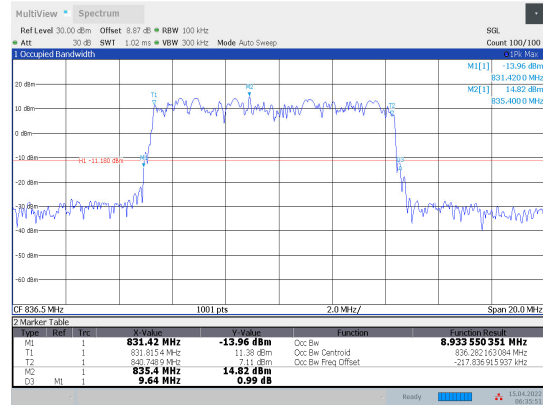
1-N5-PC3-15-10-M-6-DFT-QPSK-Outter_Full-50@0 -Ant1-8.934-9.640-≤10-PASS
