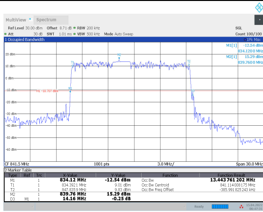
1-N5-PC3-15-15-H-5-DFT-PI/2BPSK-Outter_Full-75 @0-Ant1-13.444-14.160-≤15-PASS
