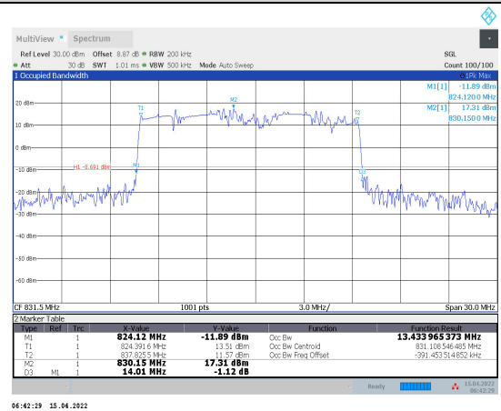
1-N5-PC3-15-15-L-8-DFT-64QAM-Outter_Full-75@0-Ant1-13.434-14.010-≤15-PASS
