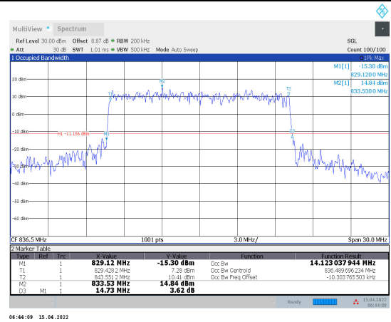
1-N5-PC3-15-15-M-3-CP-64QAM-Outer_Full-79@0- Ant1-14.123-14.730≤15-PASS
