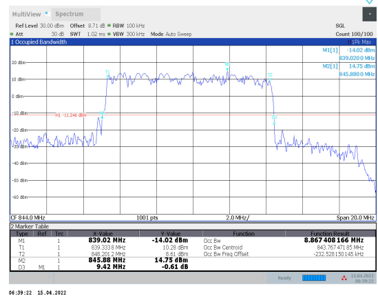
1-N5-PC3-15-10-H-7-DFT-16QAM-Out_50@0 -Ant1-8.867-9.420-≤10-PASS
