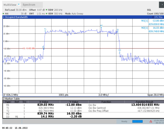
1-N5-PC3-15-15-M-8-DFT-64QAM-Outter_Full-75@ 0-Ant1-13.404-14.100≤15-PASS
