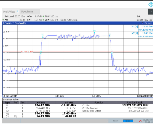
1-N5-PC3-15-15-L-5-DFT-PI/2BPSK-Outter_Full-75@0-Ant1-13.371-14.190-≤15-PASS
