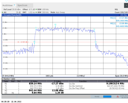
1-N5-PC3-15-10-H-4-CP-256QAM-Out_52 @0-Ant1-9.198-9.640-≤10-PASS
