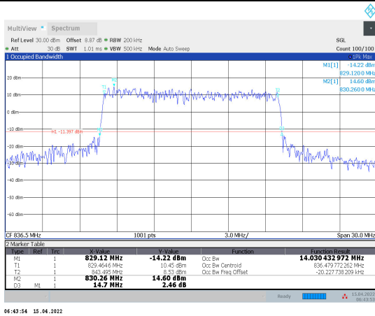
1-N5-PC3-15-15-M-2-CP-16QAM-Outer_Full-79@ 0-Ant1-14.03-14.700≤15-PASS
