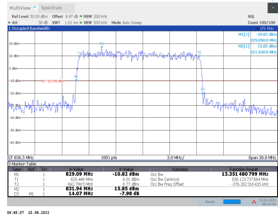
1-N5-PC3-15-15-M-9-DFT-256QAM-Outter_Full-75 @0-Ant1-13.351-14.070≤15-PASS
