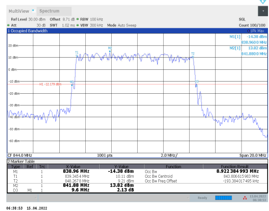
1-N5-PC3-15-10-H-5-DFT-PI/2BPSK-Out_50 @0-Ant1-8.922-9.600-≤10-PASS
