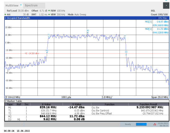
1-N5-PC3-15-10-H-3-CP-64QAM-Out_52@0- Ant1-9.255-9.620-≤10-PASS
