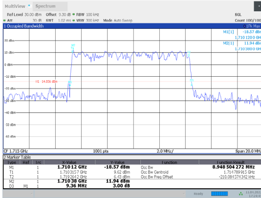
1-N66-PC3-15-10-L-7-DFT-16QAM-Outer_Full-50@0-A nt1-8.949-9.360-≤10-PASS
