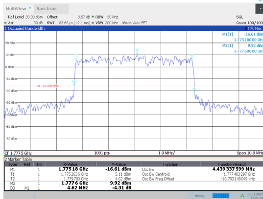
1-N66-PC3-15-5-H-3-CP-64QAM-Outet_Full-25@0-Ant1-4.439-4.620-≤5-PASS
