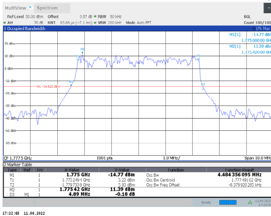
1-N66-PC3-15-5-H-9-DFT-256QAM-Outer_Full-25@0-A nt1-4.484-4.890-≤5-PASS
