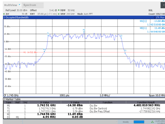
1-N66-PC3-15-5-M-8-DFT-64QAM-Out_ Full-25@0-A nt1-4.482-4.950-≤5-PASS
