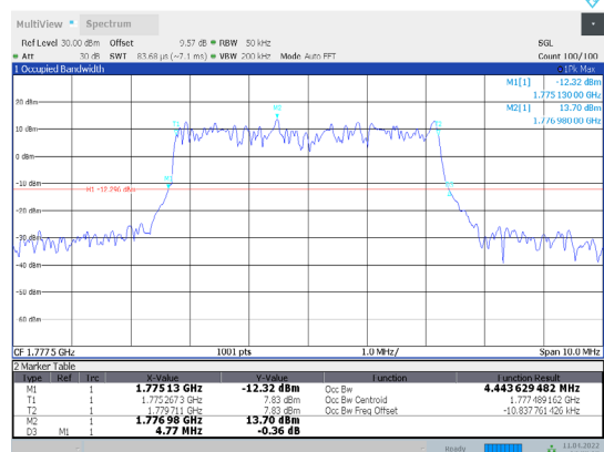
1-N66-PC3-15-5-H-6-DFT-QPSK-Outet_Full-25@0-Ant1-4.444-4.770-≤5-PASS
