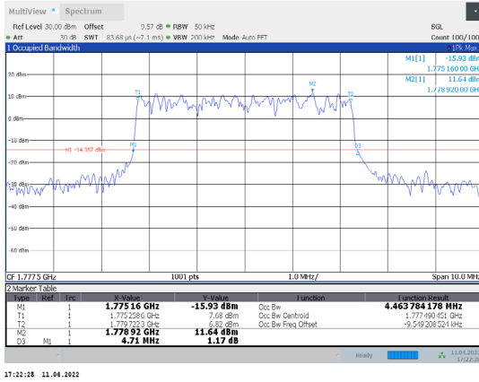
1-N66-PC3-15-5-H-7-DFT-16QAM-Outer_Full-25@0-Ant 1-4.464-4.710-≤5-PASS
