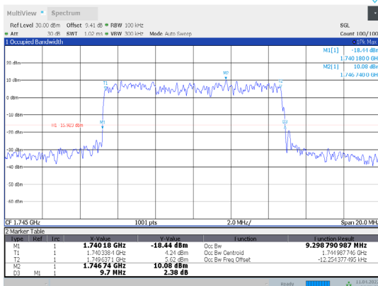
1-N66-PC3-15-10-M-2-CP-16QAM-Outer_Full-52@0-A t1-9.299-9.700-≤10-PASS
