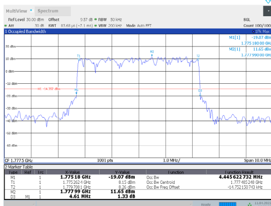
1-N66-PC3-15-5-H-5-DFT-PI/2BPSK-Outet_Full-25@0-Ant1-4.446-4.610-≤5-PASS
