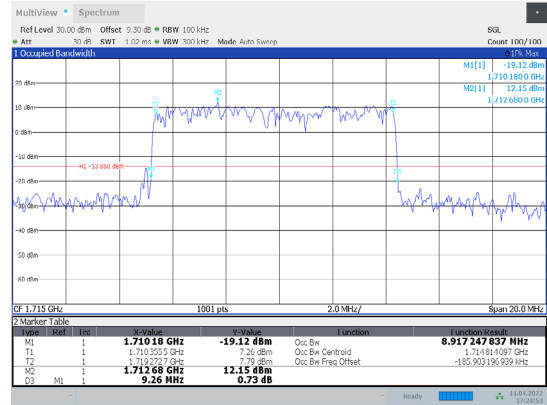
1-N66-PC3-15-10-L-8-DFT-64QAM-Outer_Full-50@0-A nt1-8.917-9.260-≤10-PASS
