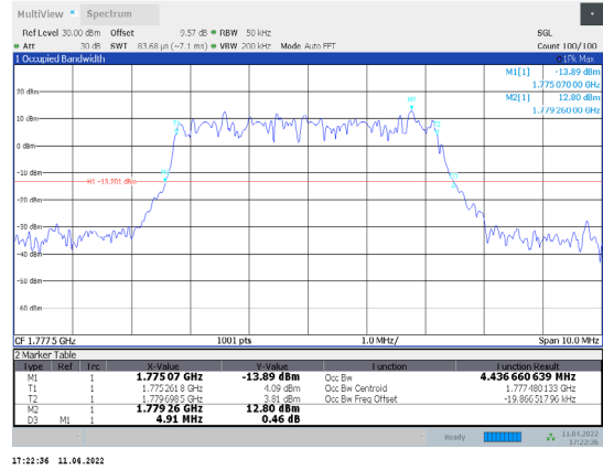
1-N66-PC3-15-5-H-8-DFT-64QAM-Outer_Full-25@0-A nt1-4.437-4.910-≤5-PASS
