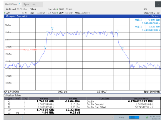
1-N66-PC3-15-5-M-5-DFT-PI/2BPSK-Out_ Full-25@0-A nt1-4.471-4.940-≤5-PASS
