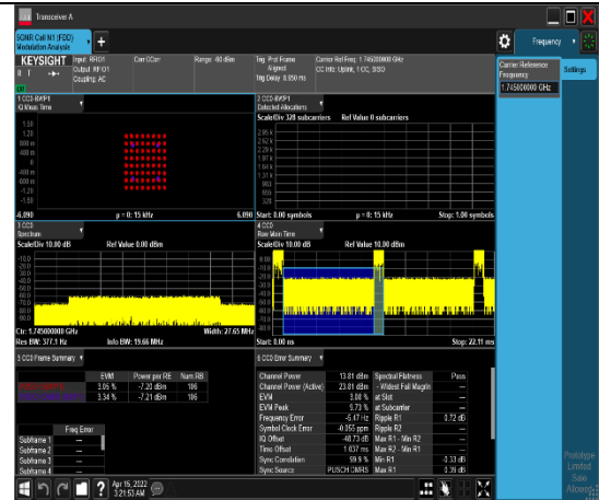
1-N66-PC3-15-20-M-8-CP-64QAM-Outer_Full-106@0- Ant1-see graph-PASS
