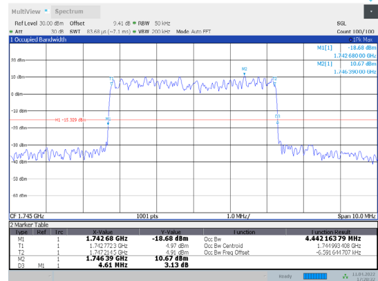
1-N66-PC3-15-5-M-9-DFT-256QAM-Out_ Full-25@0-A nt1-4.442-4.610-≤5-PASS
