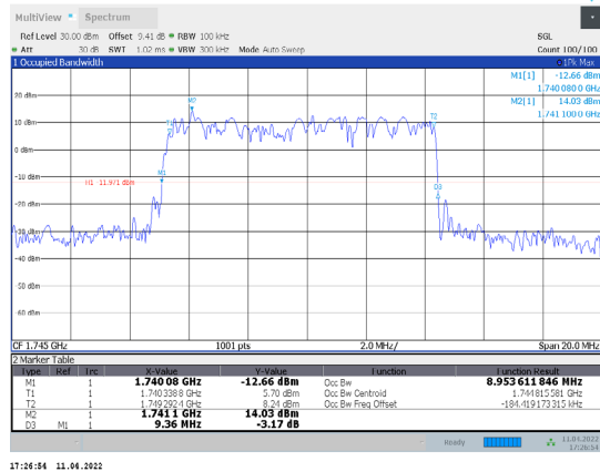
1-N66-PC3-15-10-M-6-DFT-QPSK-Outer_Full-50@0-Ant1-8.954-9.360-≤10-PASS
