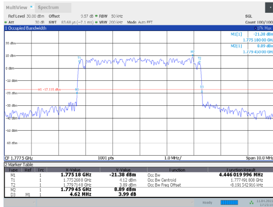
1-N66-PC3-15-5-H-1-CP-QPSK-Outet_Full-25@0-Ant1-4.446-4.620-≤5-PASS
