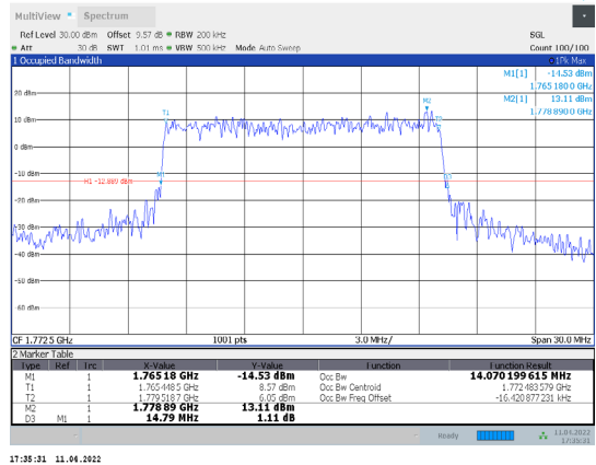
1-N66-PC3-15-15-H-2-CP-16QAM-Outer_Full-79@0-A nt1-14.07-14.790≤15-PASS
