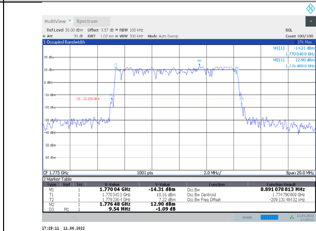
1-N66-PC3-15-10-H-6-DFT-QPSK-Outer_Full-50@0-Ant1 -8.891-9.540≤10-PASS
