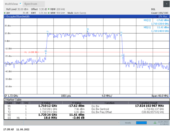
1-N66-PC3-15-20-L-8-DFT-64QAM-Outer_Full-100@0-Ant1-17.824-18.600-≤20-PASS
