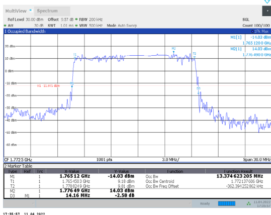
1-N66-PC3-15-15-H-5-DFT-PI/2BPSK-Outer_Full-75@0-A Ant1-13.375-14.160≤15-PASS
