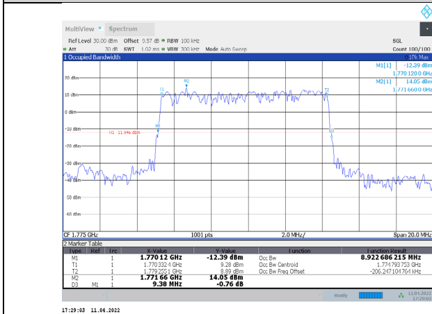
1-N66-PC3-15-10-H-5-DFT-PI/2BPSK-Outer_Full-50@0-Ant1 -8.923-9.380≤10-PASS
