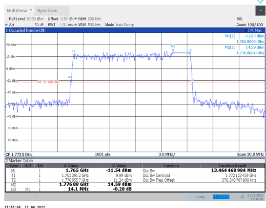
1-N66-PC3-15-15-H-6-DFT-QPSK-Outer_Full-75@0-A nt1-13.464-14.100≤15-PASS
