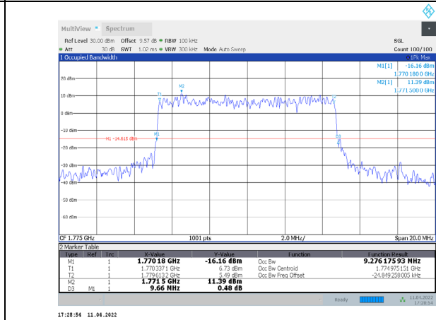
1-N66-PC3-15-10-H-4-CP-256QAM-Outer_Full-52@0-Ant1 -9.276-9.660≤10-PASS
