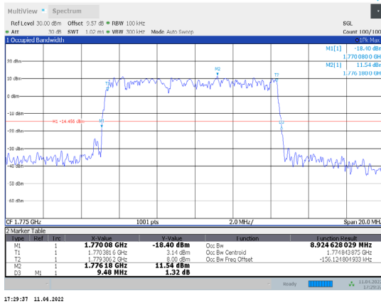
1-N66-PC3-15-10-H-9-DFT-256QAM-Outer_Full-50@0- Ant1-8.925-9.480-≤10-PASS
