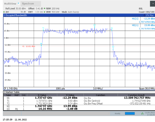
1-N66-PC3-15-15-M-5-DFT-PI/2BPSK-Outer_Full-75@0-Ant1-13.51-14.160≤15-PASS
