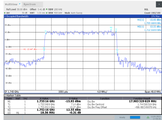
1-N66-PC3-15-20-M-5-DFT-PI/2BPSK-Outer_Full-100@0-Ant1-17.903-18.560-≤20-PASS
