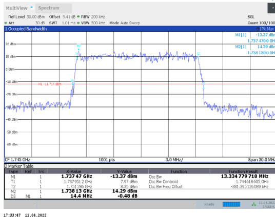
1-N66-PC3-15-15-M-6-DFT-QPSK-Outer_Full-75@0-Ant1-13.335-14.400≤15-PASS
