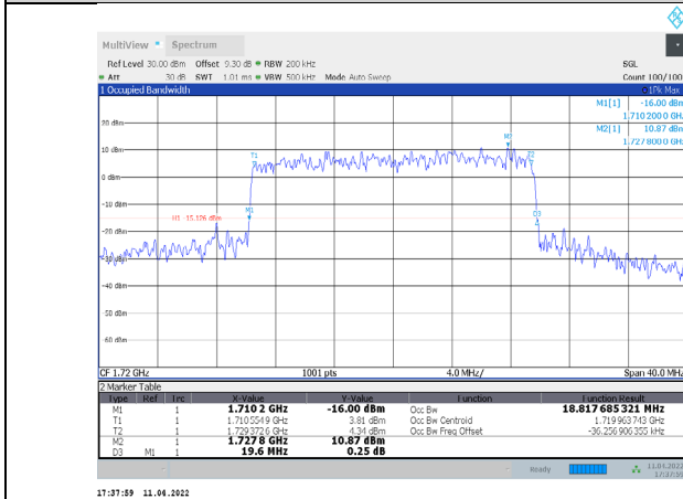
1-N66-PC3-15-20-L-3-CP-64QAM-Outer_Full-106@0-Ant t1-18.818-19.600-≤20-PASS
