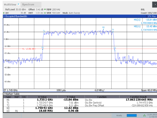
1-N66-PC3-15-20-M-6-DFT-QPSK-Outer_Full-100@0-Ant1-17.863-18.680-≤20-PASS
