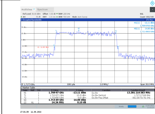
1-N66-PC3-15-15-L-6-DFT-QPSK-Outer_Full-75@0-Ant1-13.381-14.340-≤15-PASS
