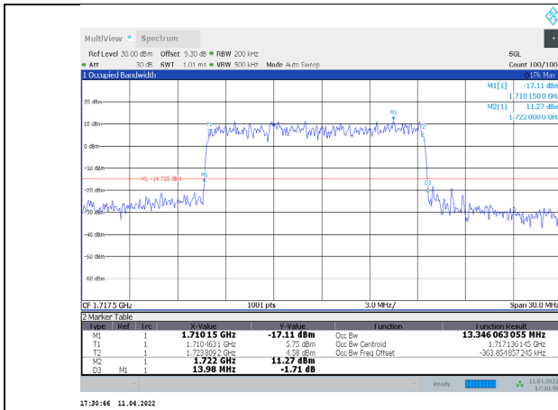
1-N66-PC3-15-15-L-1-CP-QPSK-Outer_Full-75@0-Ant1-13.346-13.980-≤15-PASS
