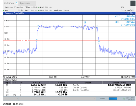
1-N66-PC3-15-15-H-8-DFT-64QAM-Outer_Full-75@0-A Ant1-13.398-14.130-≤15-PASS
