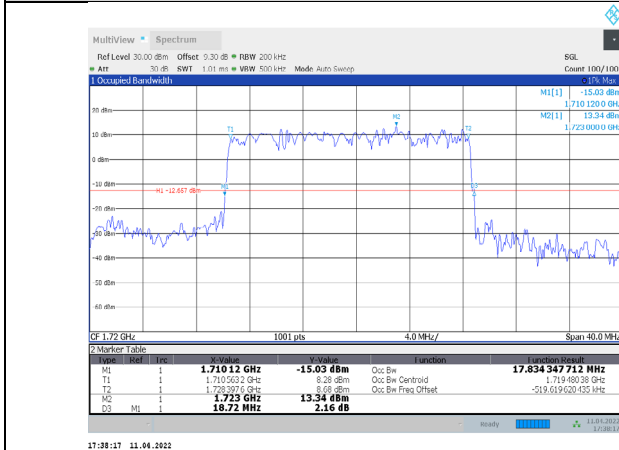
1-N66-PC3-15-20-L-5-DFT-PI/2BPSK-Outer_Full-100@0-Ant1-17.834-18.720-≤20-PASS
