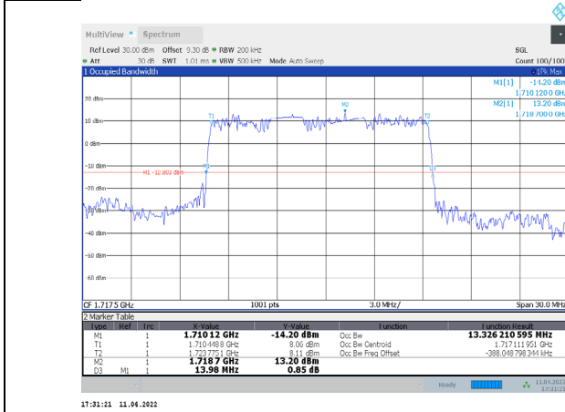
1-N66-PC3-15-15-L-5-DFT-PI/2BPSK-Outer_Full-75@0-Ant1-13.326-13.980-≤15-PASS
