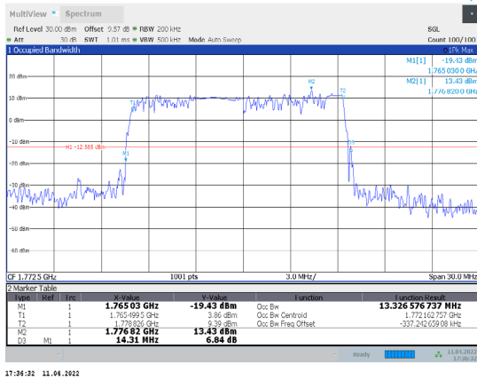
1-N66-PC3-15-15-H-9-DFT-256QAM-Outer_Full-75@0-A Ant1-13.327-14.310-≤15-PASS
