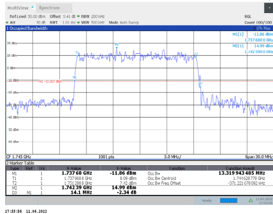
1-N66-PC3-15-15-M-7-DFT-16QAM-Outer_Full-75@0-Ant1-13.32-14.100≤15-PASS
