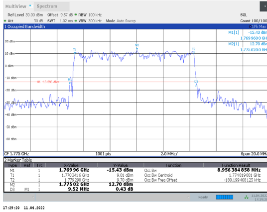
1-N66-PC3-15-10-H-7-DFT-16QAM-Outer_Full-50@0-A Ant1-8.956-9.520-≤10-PASS
