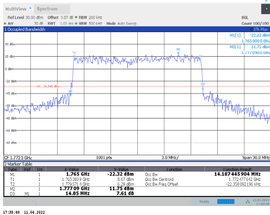
1-N66-PC3-15-15-H-3-CP-64QAM-Outer_Full-79@0-Ant 1-14.187-14.850≤15-PASS
