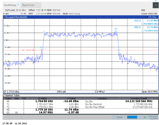
1-N66-PC3-15-15-H-4-CP-256QAM-Outer_Full-79@0-A Ant1-14.122-14.970≤15-PASS
