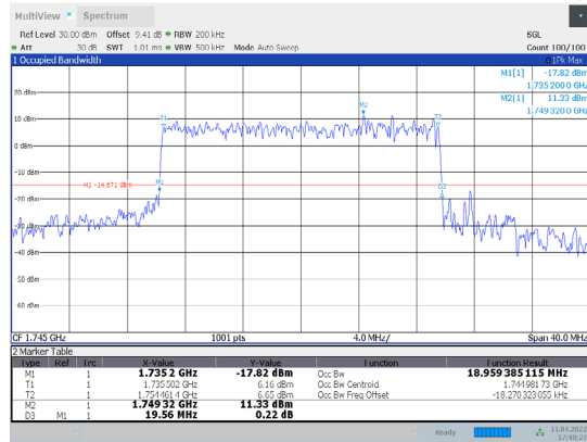
1-N66-PC3-15-20-M-4-CP-256QAM-Outer_Full-106@0-Ant1-18.959-19.560-≤20-PASS
