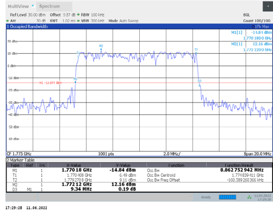
1-N66-PC3-15-10-H-8-DFT-64QAM-Outer_Full-50@0- Ant1-8.863-9.340-≤10-PASS
