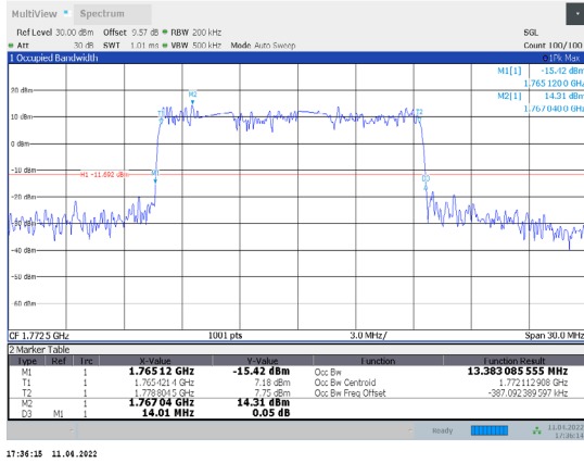
1-N66-PC3-15-15-H-7-DFT-16QAM-Outer_Full-75@0-A Ant1-13.383-14.010-≤15-PASS
