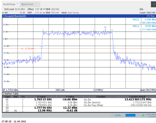
1-N66-PC3-15-15-H-1-CP-QPSK-Outer_Full-75@0-Ant1 -13.414-13.980≤15-PASS
