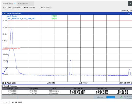
1-N66-PC3-15-20-L-17-DFT-256QAM-Edge_1RB_Left-1 @0-Ant1-seegraph-PASS-see graph
