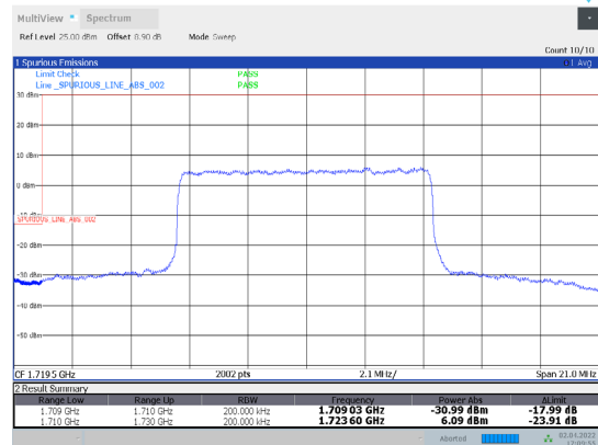
1-N66-PC3-15-20-L-16-DFT-64QAM-Inner_Full-50@25-Ant1-seegraph-PASS-see graph
