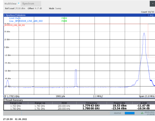
1-N66-PC3-15-20-H-18-DFT-256QAM-Edge_1RB_Right-1@105-Ant1-seegraph-PASS-see graph
