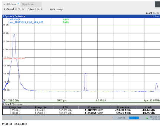
1-N66-PC3-15-20-L-33-CP-256QAM-Edge_1RB_Left-1@0-Ant1-seegraph-PASS-see graph
