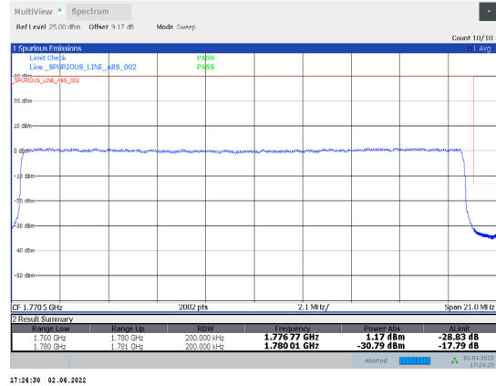
1-N66-PC3-15-20-H-31-CP-64QAM-Outer_Full-106@0-Ant1-seegraph-PASS-see graph
