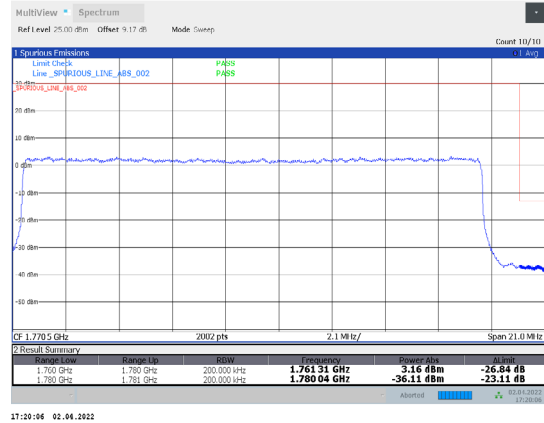
1-N66-PC3-15-20-H-15-DFT-64QAM-Outer_Full-100@0-Ant1-seegraph-PASS-see graph
