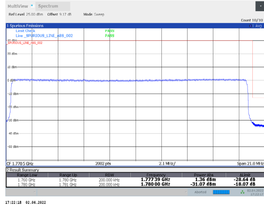
1-N66-PC3-15-20-H-23-CP-QPSK-Outer_Full-106@0-A nt1-seegraph-PASS-see graph
