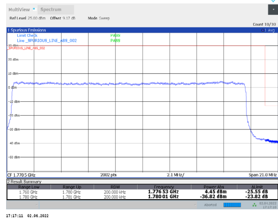
1-N66-PC3-15-20-H-4-DFT-PI/2BPSK-Outer_Full-100@0-Ant1-seegraph-PASS-see graph
