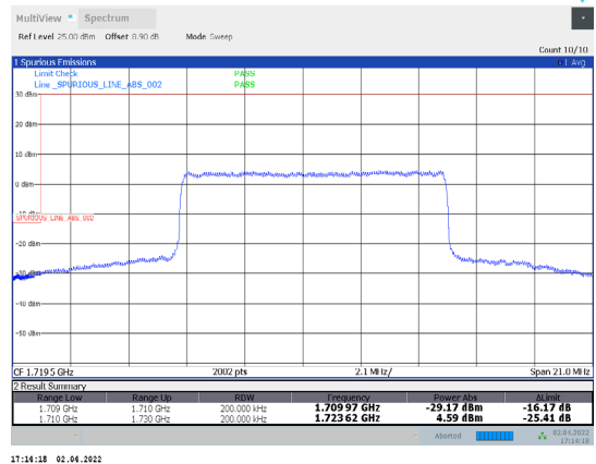
1-N66-PC3-15-20-L-32-CP-64QAM-Inner_Full-53@26-Ant1-seegraph-PASS-see graph
