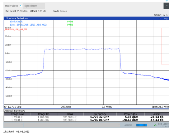
1-N66-PC3-15-20-H-28-CP-16QAM-Inner_Full-53@26-Ant1-seegraph-PASS-see graph
