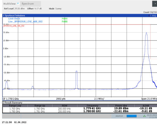
1-N66-PC3-15-20-H-22-CP-QPSK-Edge_1RB_Right-1 @105-Ant1-seegraph-PASS-see graph
