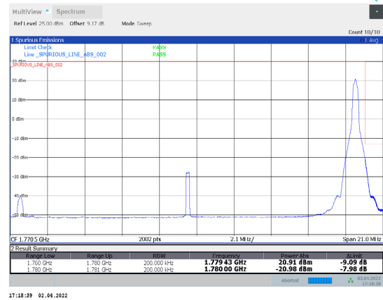
1-N66-PC3-15-20-H-10-DFT-16QAM-Edge_1RB_Right-1 @105-Ant1-seegraph-PASS-see graph
