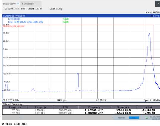
1-N66-PC3-15-20-H-30-CP-64QAM-Edge_1RB_Right-1 @105-Ant1-seegraph-PASS-see graph
