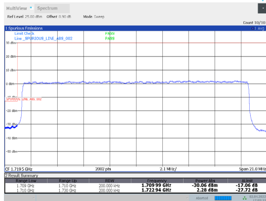
1-N66-PC3-15-20-L-15-DFT-64QAM-Outer_Full-100@0-Ant1-seegraph-PASS-see graph
