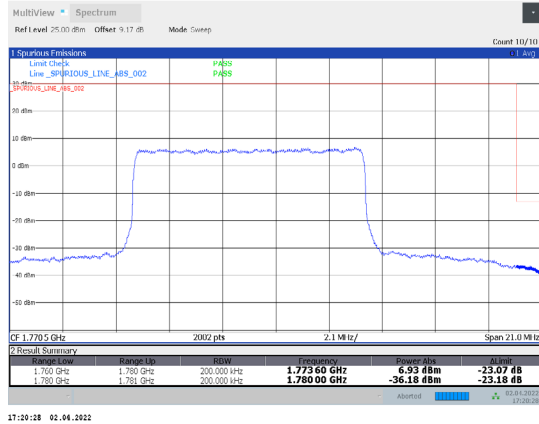
1-N66-PC3-15-20-H-16-DFT-64QAM-Inner_Full-50@25-Ant1-seegraph-PASS-see graph
