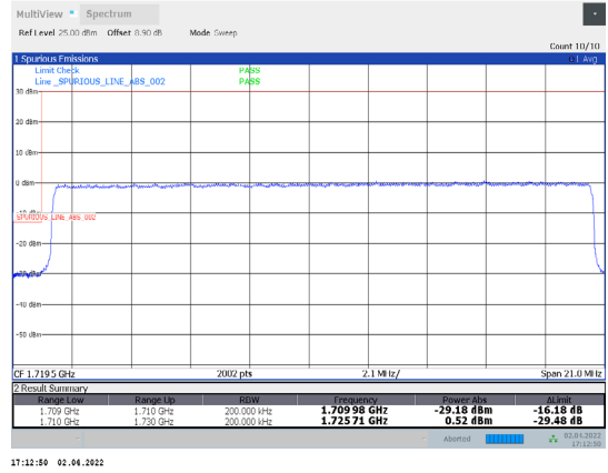
1-N66-PC3-15-20-L-27-CP-16QAM-Outer_Full-106@0-Ant1-seegraph-PASS-see graph
