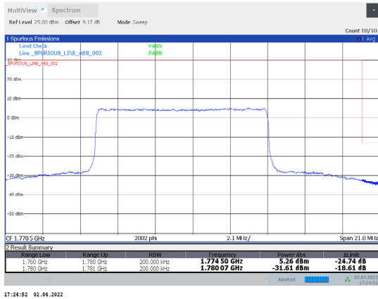
1-N66-PC3-15-20-H-32-CP-64QAM-Inner_Full-53@26-Ant1-seegraph-PASS-see graph
