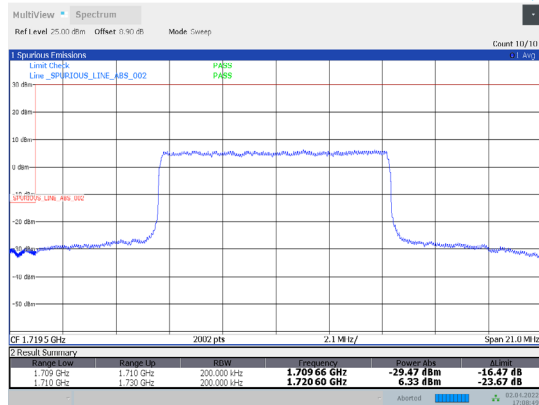
1-N66-PC3-15-20-L-12-DFT-16QAM-Inner_Full-50@25-Ant1-seegraph-PASS-see graph
