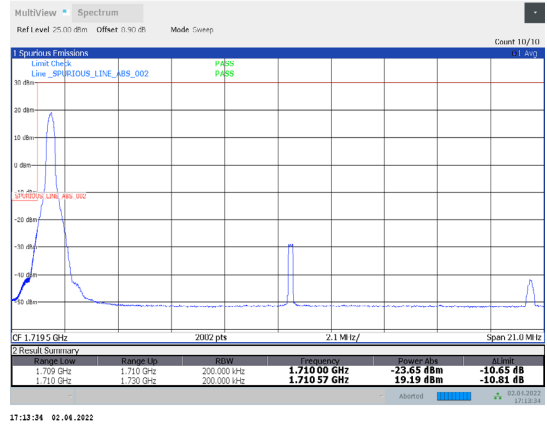
1-N66-PC3-15-20-L-29-CP-64QAM-Edge_1RB_Left-1 @0-Ant1-seegraph-PASS-see graph
