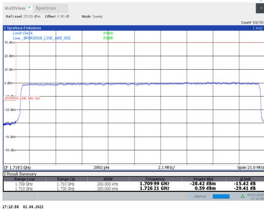
1-N66-PC3-15-20-L-31-CP-64QAM-Outer_Full-106@0-Ant1-seegraph-PASS-see graph
