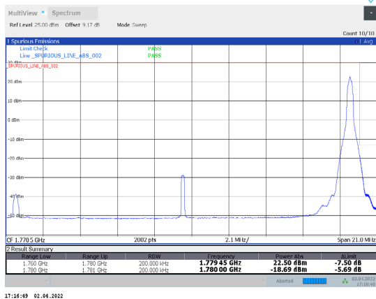
1-N66-PC3-15-20-H-3-DFT-PI/2BPSK-Edge_1RB_Right-1@105-Ant1-seegraph-PASS-see graph
