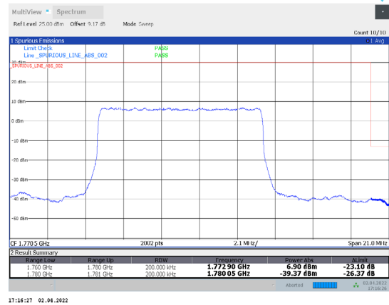
1-N66-PC3-15-20-H-1-DFT-PI/2BPSK-Inner_Full-50@25-Ant1-seegraph-PASS-see graph
