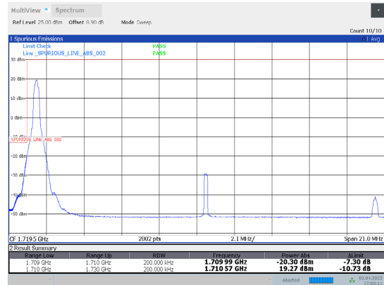
1-N66-PC3-15-20-L-13-DFT-64QAM-Edge_1RB_Left-1 @0-Ant1-seegraph-PASS-see graph
