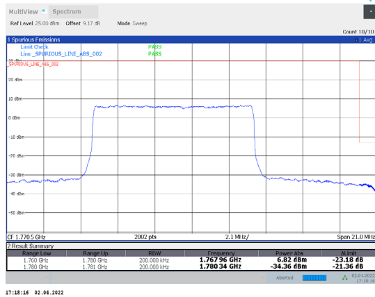
1-N66-PC3-15-20-H-8-DFT-QPSK-Inner_Full-50@25-A nt1-seegraph-PASS-see graph
