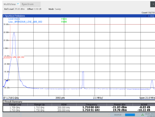
1-N66-PC3-15-20-L-9-DFT-16QAM-Edge_1RB_Left-1 @0-Ant1-seegraph-PASS-see graph
