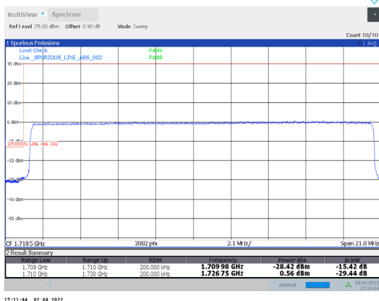
1-N66-PC3-15-20-L-23-CP-QPSK-Outer_Full-106@0-Ant1-seegraph-PASS-see graph
