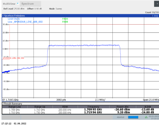
1-N66-PC3-15-20-L-28-CP-16QAM-Inner_Full-53@26-Ant1-seegraph-PASS-see graph
