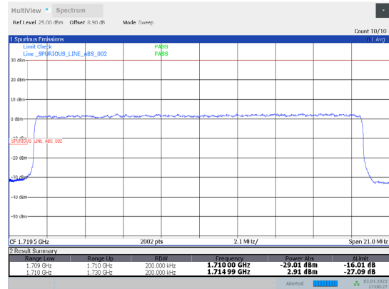
1-N66-PC3-15-20-L-11-DFT-16QAM-Outer_Full-100@0-Ant1-seegraph-PASS-see graph
