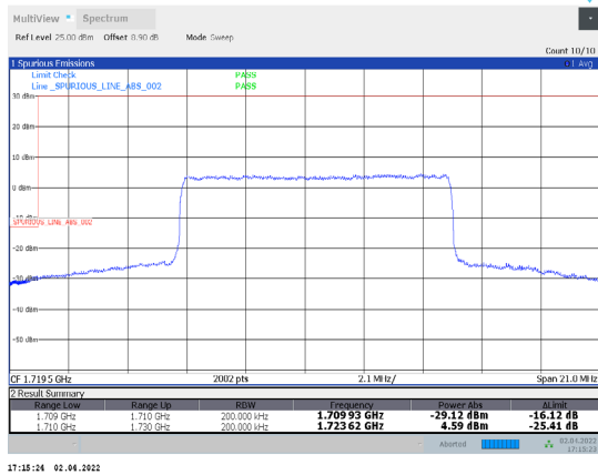
1-N66-PC3-15-20-L-36-CP-256QAM-Inner_Full-53@26-Ant1-seegraph-PASS-see graph
