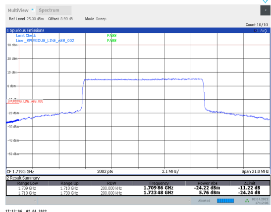
1-N66-PC3-15-20-L-24-CP-QPSK-Inner_Full-53@26-Ant1-seegraph-PASS-see graph
