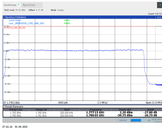
1-N66-PC3-15-20-H-19-DFT-256QAM-Outer_Full-100@0-Ant1-seegraph-PASS-see graph
