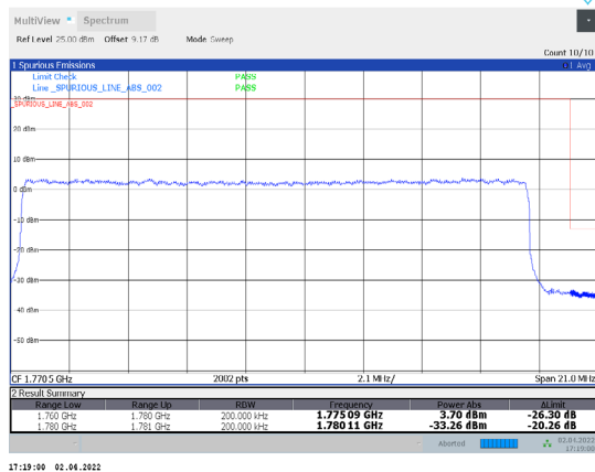
1-N66-PC3-15-20-H-11-DFT-16QAM-Outer_Full-100@0-Ant1-seegraph-PASS-see graph
