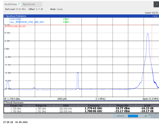
1-N66-PC3-15-20-H-34-CP-256QAM-Edge_1RB_Right-1@105-Ant1-seegraph-PASS-see graph
