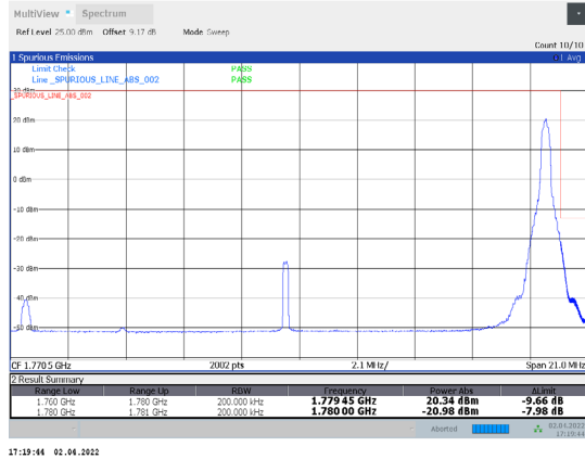
1-N66-PC3-15-20-H-14-DFT-64QAM-Edge_1RB_Right-1@105-Ant1-seegraph-PASS-see graph
