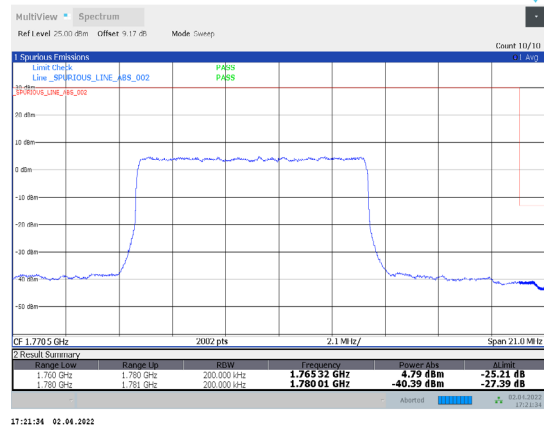
1-N66-PC3-15-20-H-20-DFT-256QAM-Inner_Full-50@25-Ant1-seegraph-PASS-see graph
