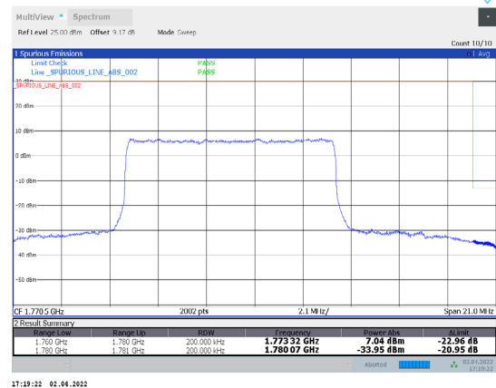
1-N66-PC3-15-20-H-12-DFT-16QAM-Inner_Full-50@25-Ant1-seegraph-PASS-see graph
