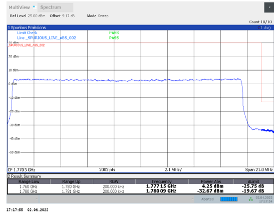
1-N66-PC3-15-20-H-7-DFT-QPSK-Outer_Full-100@0-A nt1-seegraph-PASS-see graph
