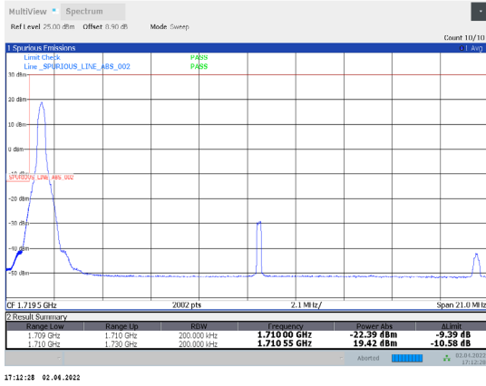
1-N66-PC3-15-20-L-25-CP-16QAM-Edge_1RB_Left-1 @0-Ant1-seegraph-PASS-see graph
