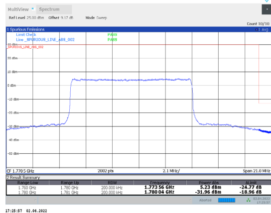
1-N66-PC3-15-20-H-36-CP-256QAM-Inner_Full-53@26-Ant1-seegraph-PASS-see graph
