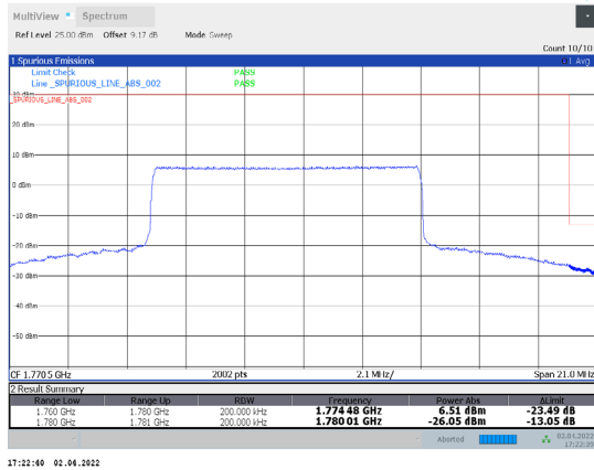
1-N66-PC3-15-20-H-24-CP-QPSK-Inner_Full-53@26-A nt1-seegraph-PASS-see graph
