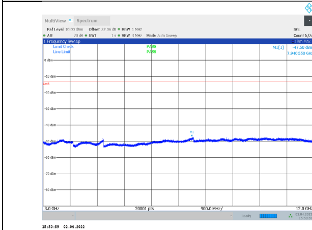
1-N66-PC3-15-5-H-3-CP-QPSK-Outter_Full-25@0-3000 -12000-Ant1--47.50--13-PASS
