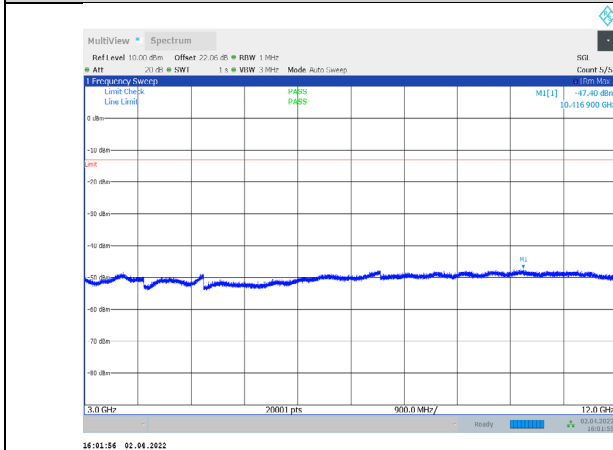
1-N66-PC3-15-15-H-1-CP-QPSK-Edge_1RB_Left-1@0 -3000-12000-Ant1--47.40--13-PASS
