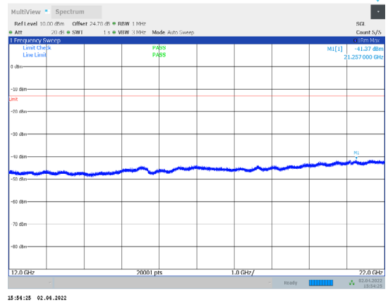
1-N66-PC3-15-15-L-2-CP-QPSK-Edge_1RB_Right-1@ 8-12000-22000-Ant1--41.37--13-PASS
