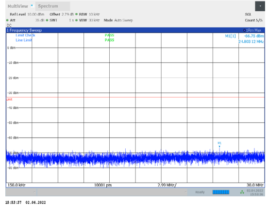
1-N66-PC3-15-15-L-2-CP-QPSK-Edge_1RB_Right-1@ 8-0.15-30-Ant1--66.75--33-PASS
