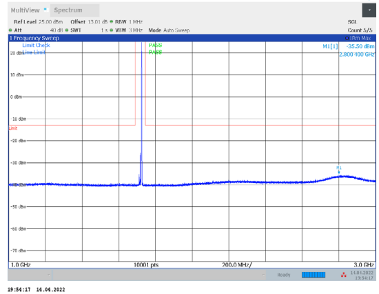
1-N66-PC3-15-15-L-2-CP-QPSK-Edge_1RB_Right-1@ 8-1000-3000-Ant1--35.50--13-PASS
