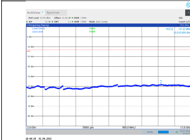
1-N66-PC3-15-5-M-3-CP-QPSK-Outer_Full-25@0-300 0-12000-Ant1--47.43--13-PASS
