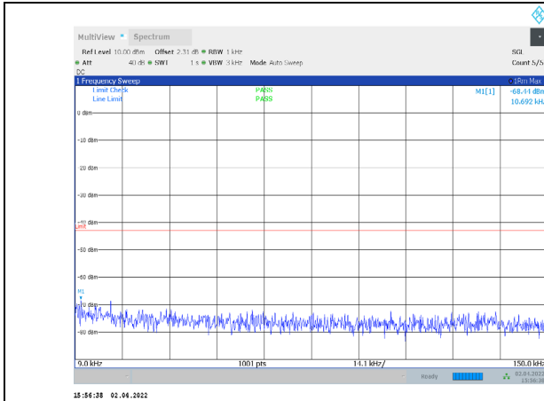
1-N66-PC3-15-15-M-1-CP-QPSK-Edge_1RB_Left-1@0 -0.009-0.15-Ant1--68.44--43-PASS
