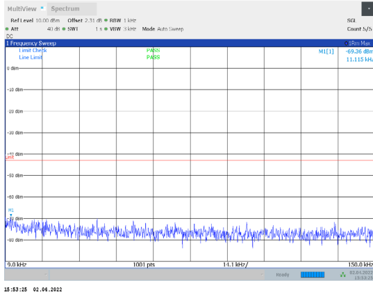
1-N66-PC3-15-15-L-2-CP-QPSK-Edge_1RB_Right-1@ 78-0.009-0.15-Ant1--69.36--43-PASS
