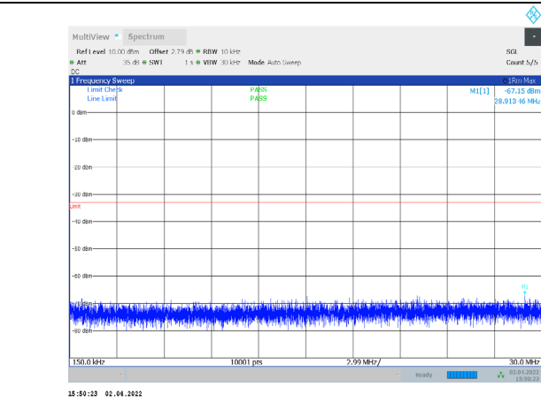
1-N66-PC3-15-5-H-3-CP-QPSK-Outter_Full-25@0-0.15- 30-Ant1--67.15--33-PASS
