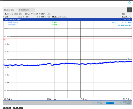
1-N66-PC3-15-15-H-1-CP-QPSK-Edge_1RB_Left-1@0- 12000-22000-Ant1--41.37--13-PASS
