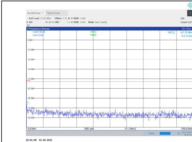
1-N66-PC3-15-15-H-1-CP-QPSK-Edge_1RB_Left-1@0 -0.009-0.15-Ant1--67.75--43-PASS
