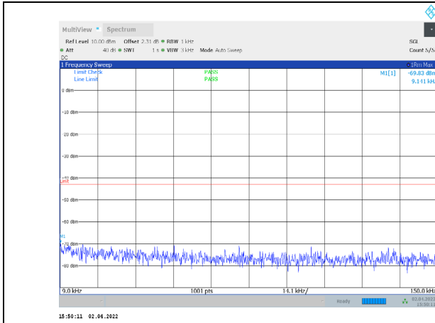
1-N66-PC3-15-5-H-3-CP-QPSK-Outter_Full-25@0-0.00 9-0.15-Ant1--69.83--43-PASS
