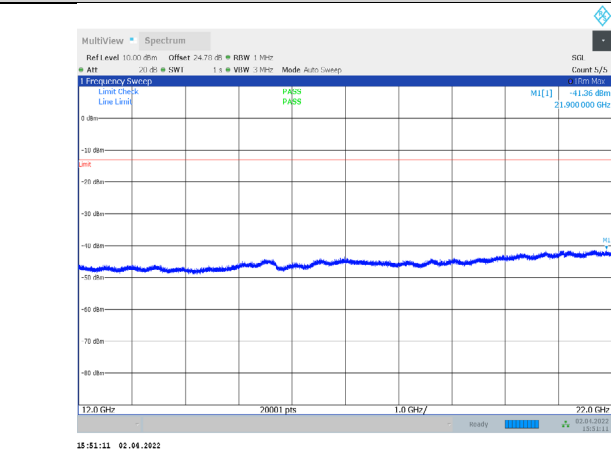
1-N66-PC3-15-5-H-3-CP-QPSK-Outter_Full-25@0-1200 0-22000-Ant1--41.36--13-PASS
