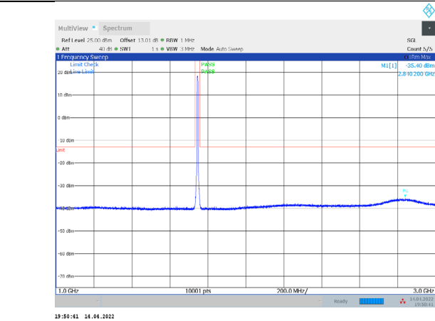
1-N66-PC3-15-5-M-3-CP-QPSK-Outer_Full-25@0-1000- 3000-Ant1--35.40--13-PASS
