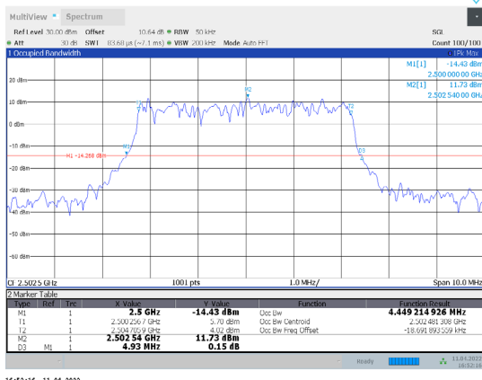
1-N7-PC3-15-5-L-9-DFT-256QAM-Outer_Full-25@0-Ant1 1-4.449-4.930-≤5-PASS
