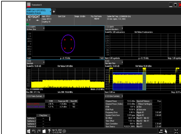
1-N7-PC3-15-20-M-1-DFT-PI/2BPSK-Outter_Full -100@0-Ant1-see graph-PASS
