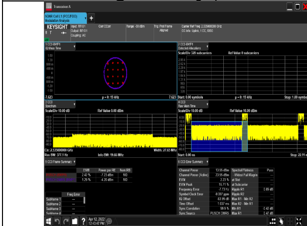
1-N7-PC3-15-20-M-3-DFT-16QAM-Outter_Full -100@0-Ant1-see graph-PASS
