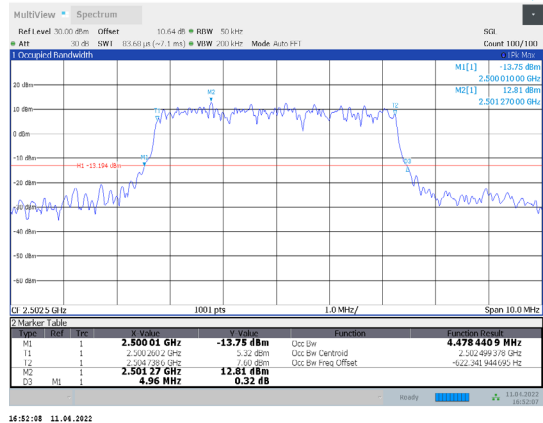
1-N7-PC3-15-5-L-8-DFT-64QAM-Outer_Full-25@0-Ant1 1-4.478-4.960-≤5-PASS
