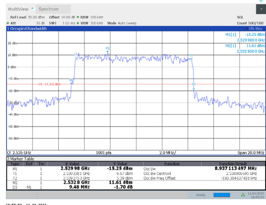
1-N7-PC3-15-10-M-1-CP-QPSK-Outer_Full-50@0-Ant 1-8.937-9.480-≤10-PASS
