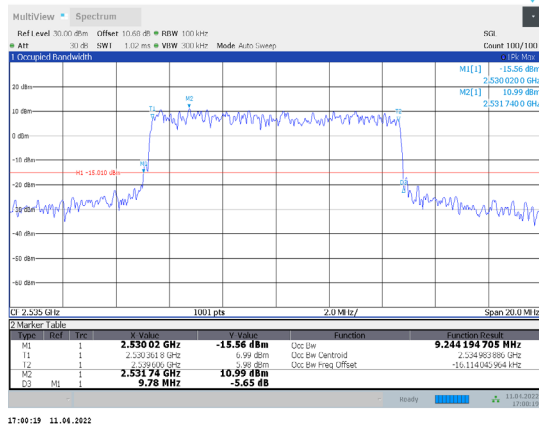
1-N7-PC3-15-10-M-4-CP-256QAM-Outer_Full-52@0-A nt1-9.244-9.780-≤10-PASS
