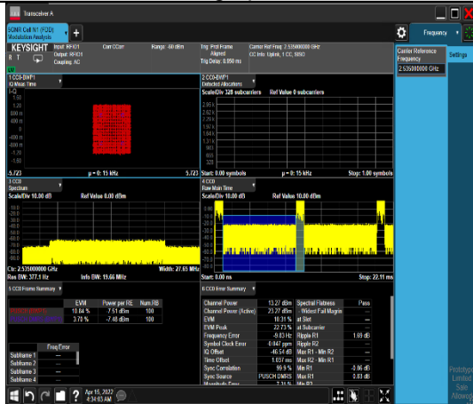
1-N7-PC3-15-20-M-9-CP-256QAM-Outer_Full-106@0-Ant1-see graph-PASS
