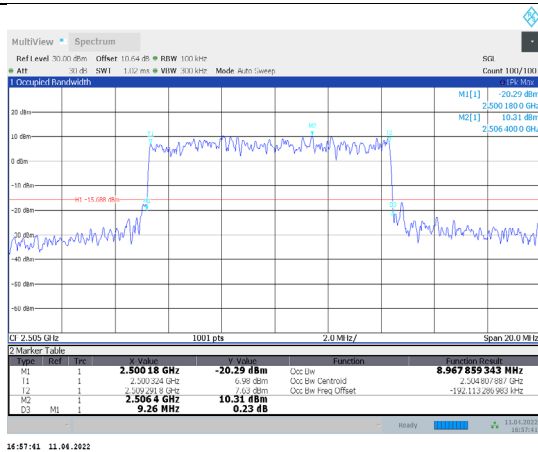
1-N7-PC3-15-10-L-1-CP-QPSK-Outer_Full-50@0-Ant1-8 9.968-9.260≤10-PASS
