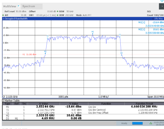
1-N7-PC3-15-5-M-2-CP-16QAM-Outer_Full-25@0-Ant1- 4.446-4.690-≤5-PASS
