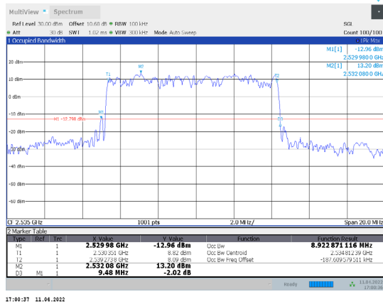
1-N7-PC3-15-10-M-6-DFT-QPSK-Outer_Full-50@0-An t1-8.923-9.480-≤10-PASS
