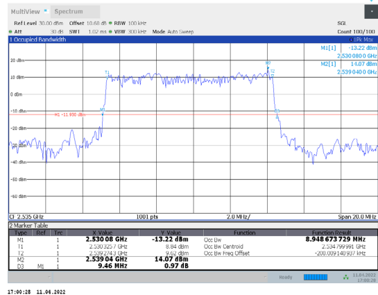
1-N7-PC3-15-10-M-5-DFT-PI/2BPSK-Outer_Full-50@0-Ant1-8.949-9.460-≤10-PASS
