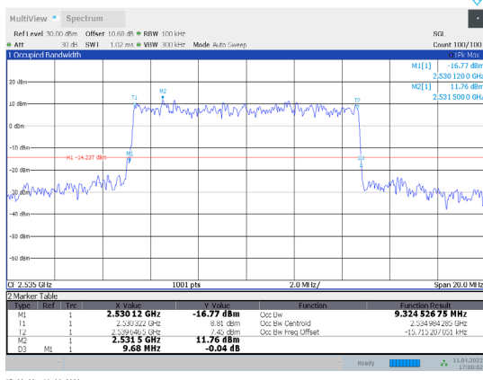
1-N7-PC3-15-10-M-2-CP-16QAM-Outer_Full-52@0-Ant 1-9.325-9.680-≤10-PASS
