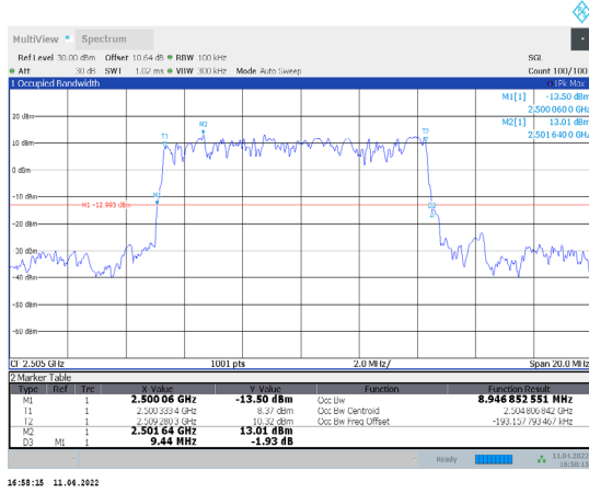
1-N7-PC3-15-10-L-5-DFT-PI/2BPSK-Outer_Full-50@0-A nt1-8.947-9.440≤10-PASS
