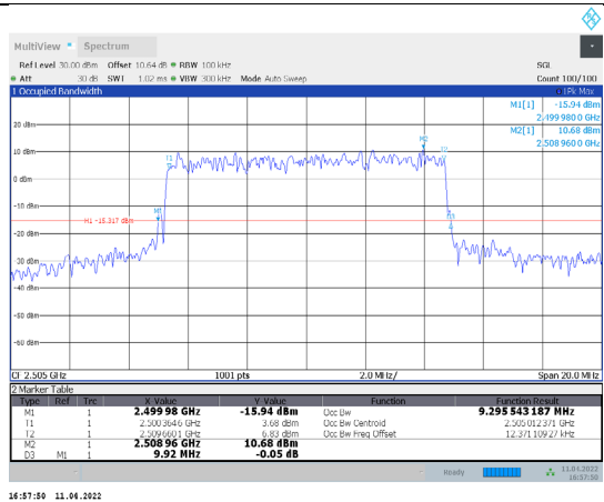
1-N7-PC3-15-10-L-2-CP-16QAM-Outer_Full-52@0-Ant 1-9.296-9.920≤10-PASS
