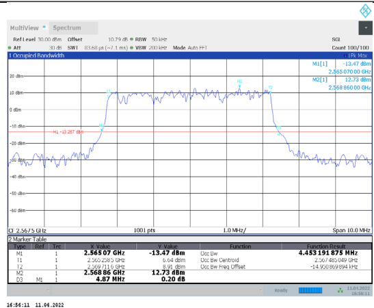
1-N7-PC3-15-5-H-6-DFT-QPSK-Outer_Full-25@0-Ant1 -4.453-4.870-≤5-PASS
