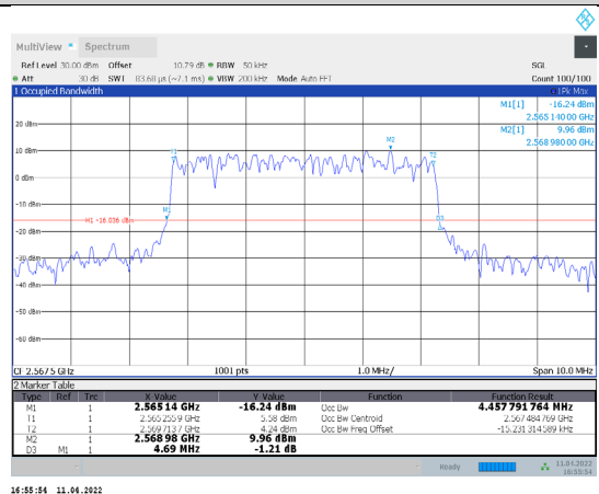
1-N7-PC3-15-5-H-4-CP-256QAM-Outer_Full-25@0-Ant 1-4.458-4.690-≤5-PASS
