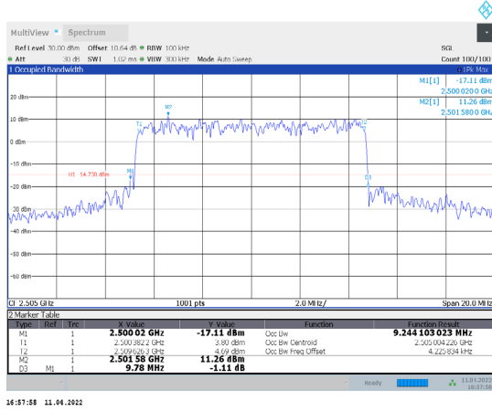
1-N7-PC3-15-10-L-3-CP-64QAM-Outer_Full-52@0-Ant1-1 9.244-9.780≤10-PASS
