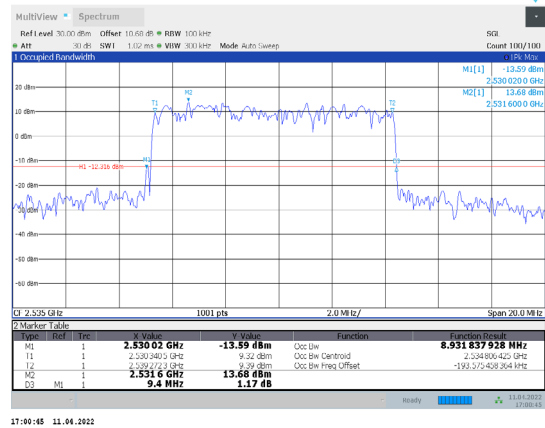
1-N7-PC3-15-10-M-7-DFT-16QAM-Outer_Full-50@0-Ant 1-8.932-9.400-≤10-PASS
