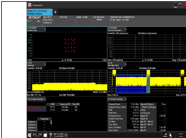
1-N7-PC3-15-20-M-7-CP-16QAM-Outer_Full-106@0-Ant1-see graph-PASS
