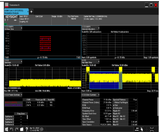
1-N7-PC3-15-20-M-8-CP-64QAM-Outer_Full-106@0-Ant1-see graph-PASS
