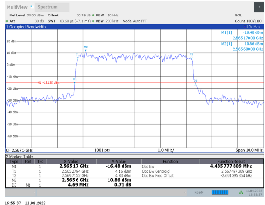
1-N7-PC3-15-5-H-2-CP-16QAM-Outer_Full-25@0-Ant1 -4.436-4.690-≤5-PASS
