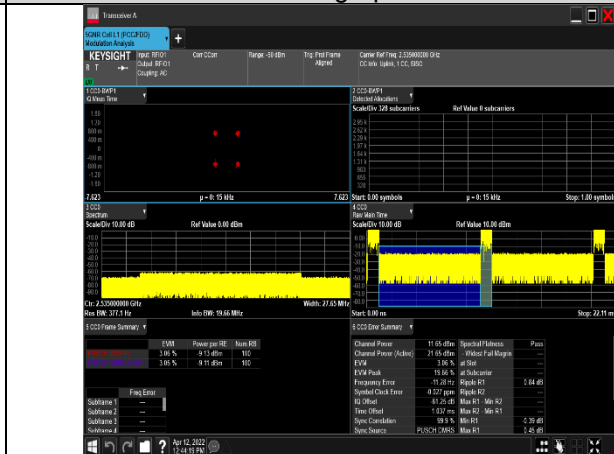
1-N7-PC3-15-20-M-6-CP-QPSK-Outter_Full-106@0-Ant1-see graph-PASS
