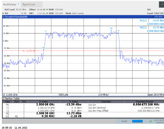
1-N7-PC3-15-10-L-7-DFT-16QAM-Outer_Full-50@0-Ant 1-8.957-9.380-≤10-PASS
