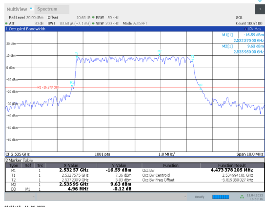
1-N7-PC3-15-5-M-1-CP-QPSK-Outer_Full-25@0-Ant1- 4.473-4.960-≤5-PASS
