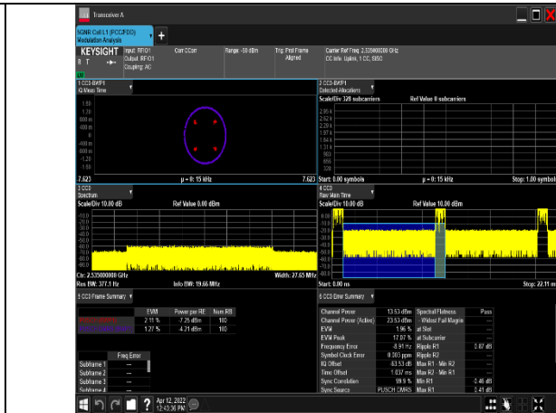
1-N7-PC3-15-20-M-2-DFT-QPSK-Outter_Full-100@0-Ant1-see graph-PASS
