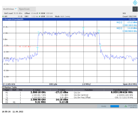
1-N7-PC3-15-10-L-6-DFT-QPSK-Outer_Full-50@0-Ant 1-8.935-9.320≤10-PASS
