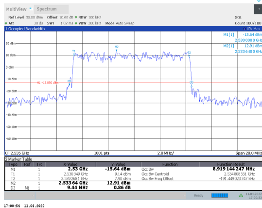
1-N7-PC3-15-10-M-8-DFT-64QAM-Outer_Full-50@0-A nt1-8.919-9.440-≤10-PASS
