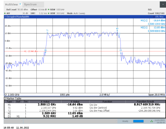
1-N7-PC3-15-10-L-8-DFT-64QAM-Outer_Full-50@0-Ant 1-8.917-9.320-≤10-PASS
