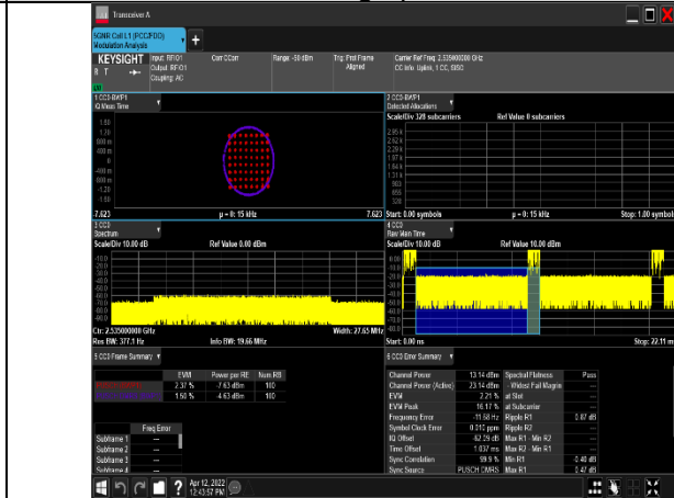
1-N7-PC3-15-20-M-4-DFT-64QAM-Outter_Full-100@0-Ant1-see graph-PASS
