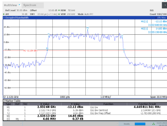
1-N7-PC3-15-5-M-6-DFT-QPSK-Outer_Full-25@0-Ant 1-4.446-4.660-≤5-PASS
