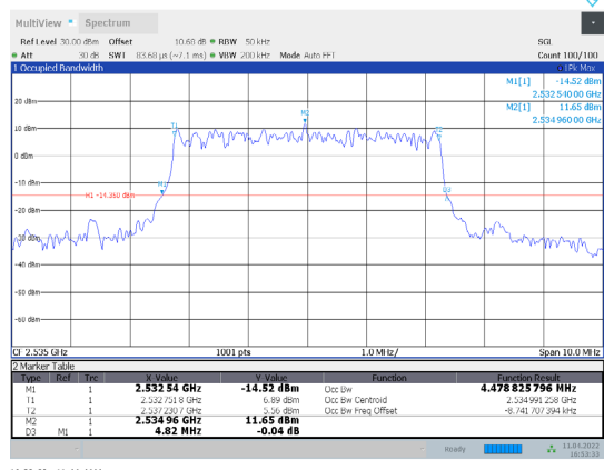
1-N7-PC3-15-5-M-3-CP-64QAM-Outer_Full-25@0-Ant1 -4.479-4.820-≤5-PASS
