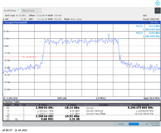
1-N7-PC3-15-10-L-4-CP-256QAM-Outer_Full-52@0-Ant nt1-9.294-9.880≤10-PASS
