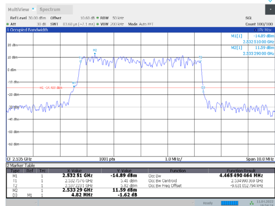
1-N7-PC3-15-5-M-9-DFT-256QAM-Outter_Full-25@0-Ant 1-4.465-4.820-≤5-PASS
