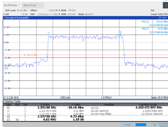
1-N7-PC3-15-5-M-4-CP-256QAM-Outer_Full-25@0-An t1-4.453-4.630-≤5-PASS
