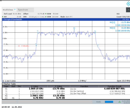
1-N7-PC3-15-5-H-5-DFT-PI/2BPSK-Outer_Full-25@0-A nt1-4.466-4.780-≤5-PASS
