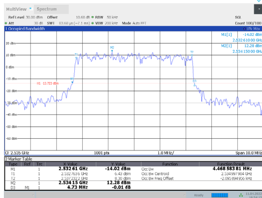
1-N7-PC3-15-5-M-8-DFT-64QAM-Outer_Full-25@0-An t1-4.469-4.730-≤5-PASS
