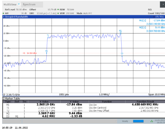
1-N7-PC3-15-5-H-1-CP-QPSK-Outer_Full-25@0-Ant1-4. 458-4.620-≤5-PASS
