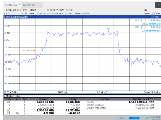
1-N7-PC3-15-5-M-7-DFT-16QAM-Outer_Full-25@0-Ant1 -4.463-4.900-≤5-PASS
