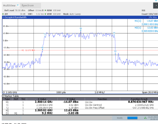
1-N7-PC3-15-10-L-9-DFT-256QAM-Outer_Full-50@0-Ant 1-8.877-9.300-≤10-PASS
