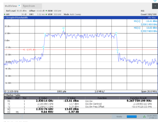
1-N7-PC3-15-10-M-3-CP-64QAM-Outer_Full-52@0-Ant 1-9.268-9.640-≤10-PASS
