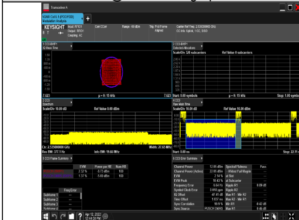
1-N7-PC3-15-20-M-4-DFT-256QAM-Outter_Full-100@0-Ant1-see graph-PASS
