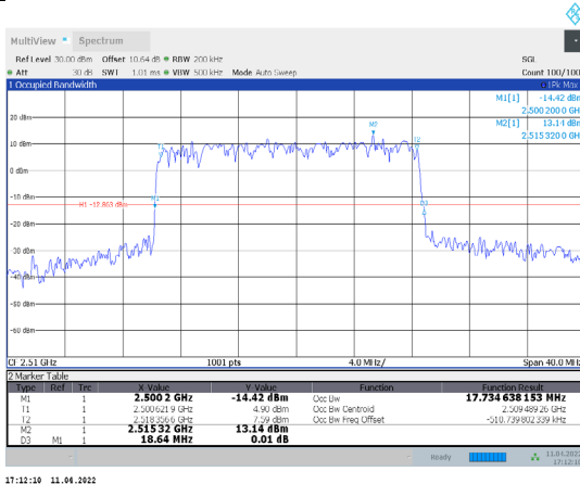
1-N7-PC3-15-20-L-9-DFT-256QAM-Outer_Full-100@0-A Ant1-17.735-18.640-≤20-PASS
