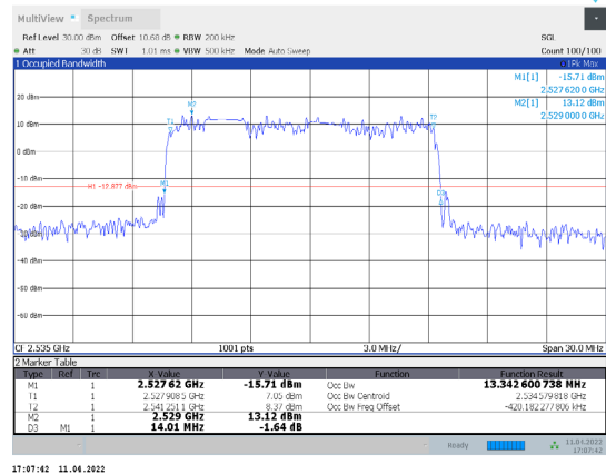
1-N7-PC3-15-15-M-9-DFT-256QAM-Outer_Full-75@0-A nt1-13.343-14.010≤15-PASS
