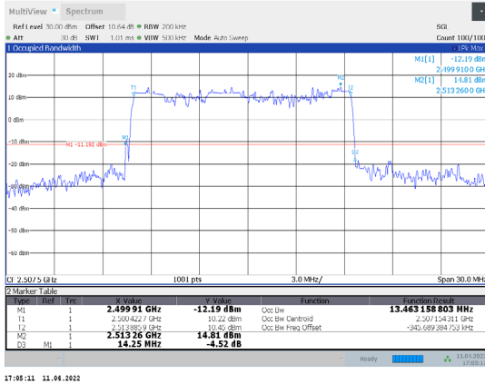
1-N7-PC3-15-15-L-7-DFT-16QAM-Outer_Full-75@0-Ant 1-13.463-14.250-≤15-PASS
