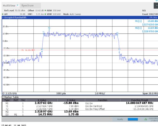
1-N7-PC3-15-15-M-2-CP-16QAM-Outer_Full-79@0-Ant 1-14.08-14.730-≤15-PASS
