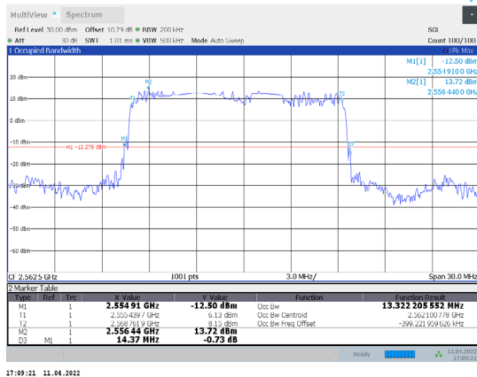
1-N7-PC3-15-15-H-5-DFT-PI/2BPSK-Outer_Full-75@0-Ant1-13.322-14.370-≤15-PASS
