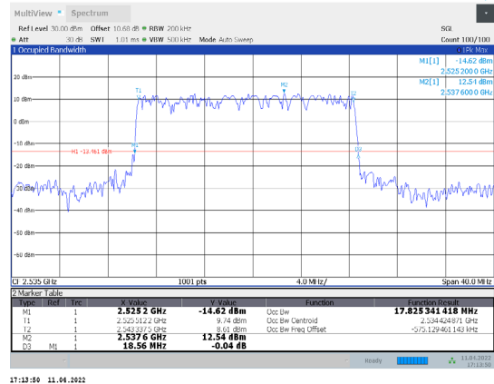
1-N7-PC3-15-20-M-5-DFT-PI/2BPSK-Outter_Full-100@0-Ant1-17.825-18.560-≤20-PASS
