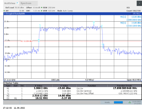
1-N7-PC3-15-20-L-8-DFT-64QAM-Outer_Full-100@0-A nt1-17.899-18.520-≤20-PASS
