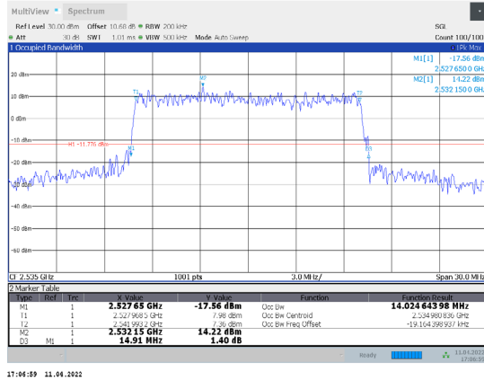
1-N7-PC3-15-15-M-4-CP-256QAM-Outer_Full-79@0-A nt1-14.025-14.910≤15-PASS
