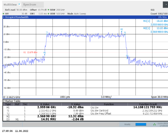
1-N7-PC3-15-15-H-3-CP-64QAM-Outer_Full-79@0-Ant1-14.108-14.910-≤15-PASS
