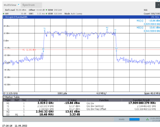
1-N7-PC3-15-20-M-8-DFT-64QAM-Outter_Full-100@0-Ant1-17.909-18.480-≤20-PASS
