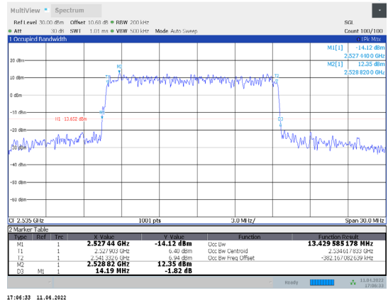
1-N7-PC3-15-15-M-1-CP-QPSK-Outer_Full-75@0-Ant1- 13.43-14.190-≤15-PASS
