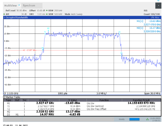
1-N7-PC3-15-15-M-3-CP-64QAM-Outer_Full-79@0-Ant 1-14.154-14.970-≤15-PASS
