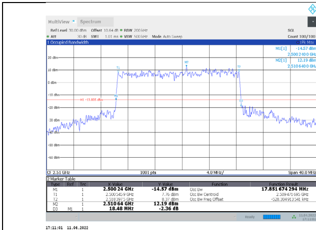
1-N7-PC3-15-20-L-1-CP-QPSK-Outer_Full-100@0-Ant1-17.852-18.480-≤20-PASS
