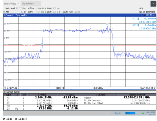
1-N7-PC3-15-15-L-8-DFT-64QAM-Outer_Full-75@0-Ant 1-13.388-13.950-≤15-PASS
