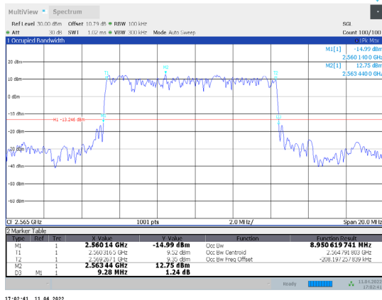
1-N7-PC3-15-10-H-5-DFT-PI/2BPSK-Outter_Full-50@0-Ant1-8.951-9.280-≤10-PASS
