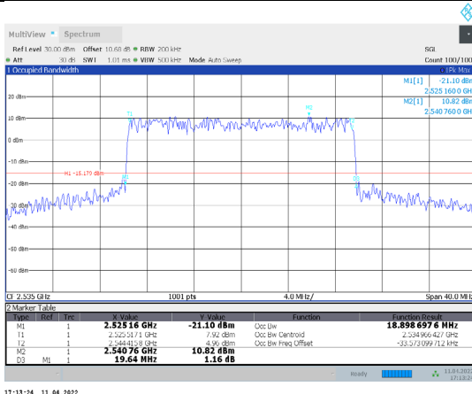
1-N7-PC3-15-20-M-2-CP-16QAM-Outer_Full-106@0-A nt1-18.899-19.640-≤20-PASS
