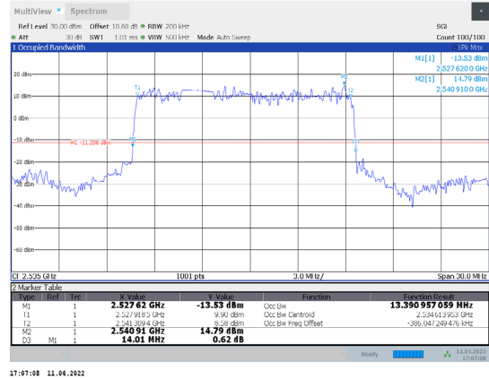
1-N7-PC3-15-15-M-5-DFT-PI/2BPSK-Outer_Full-75@0-A nt1-13.391-14.010≤15-PASS
