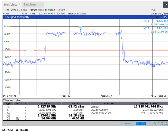
1-N7-PC3-15-15-M-6-DFT-QPSK-Outer_Full-75@0-A nt1-13.358-14.040≤15-PASS
