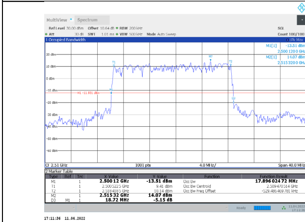
1-N7-PC3-15-20-L-5-DFT-PI/2BPSK-Outer_Full-100@0-Ant1-17.896-18.720-≤20-PASS
