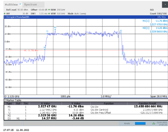
1-N7-PC3-15-15-M-7-DFT-16QAM-Outer_Full-75@0-A nt1-13.458-14.370≤15-PASS
