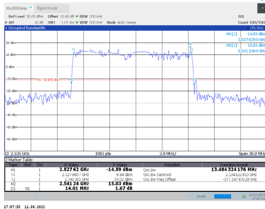
1-N7-PC3-15-15-M-8-DFT-64QAM-Outer_Full-75@0-A nt1-13.484-14.010≤15-PASS
