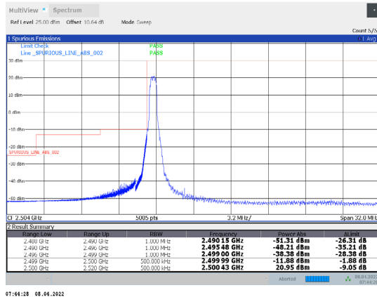
1-N7-PC3-15-20-L-25-CP-16QAM-Edge_1RB_Left-1@0-Ant1-PASS-see graph
