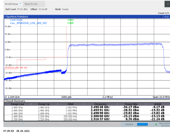
1-N7-PC3-15-20-L-11-DFT-16QAM-Outer_Full-100@0-Ant1-PASS-see graph
