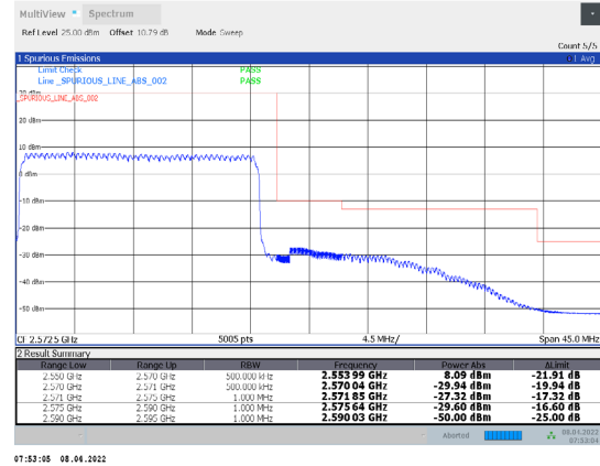
1-N7-PC3-15-20-H-15-DFT-64QAM-Outer_Full-100@0- Ant1-PASS-see graph
