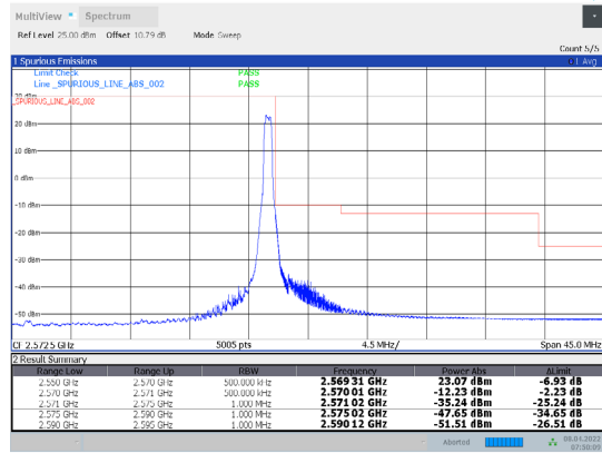
1-N7-PC3-15-20-H-6-DFT-QPSK-Edge_1RB_Right-1 @105-Ant1-PASS-see graph
