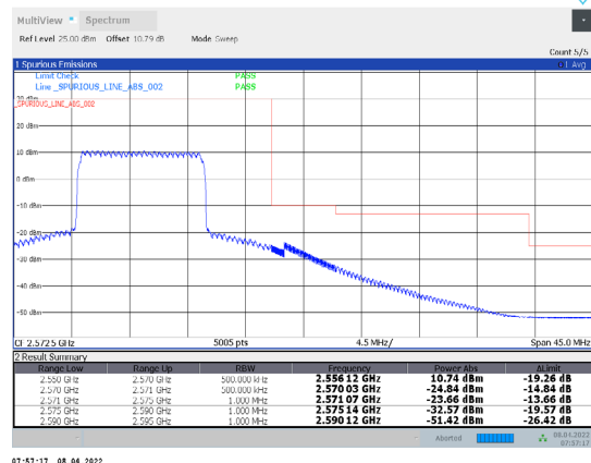
1-N7-PC3-15-20-H-28-CP-16QAM-Inner_Full-53@26-Ant1-PASS-see graph
