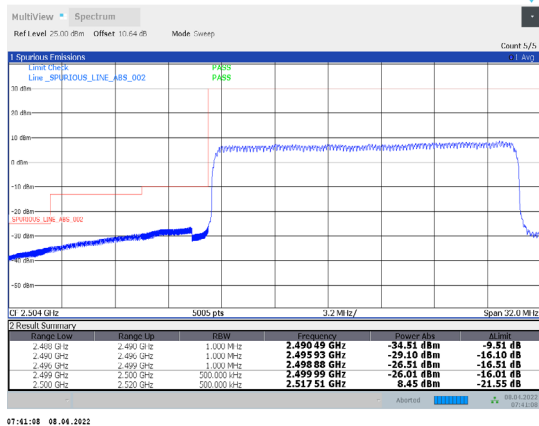
1-N7-PC3-15-20-L-15-DFT-64QAM-Outer_Full-100@0-Ant1-PASS-see graph
