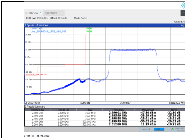
1-N7-PC3-15-20-L-1-DFT-PI/2BPSK-Inner_Full-50@2 5-Ant1-PASS-see graph
