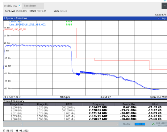
1-N7-PC3-15-20-H-11-DFT-16QAM-Outer_Full-100@0 -Ant1-PASS-see graph
