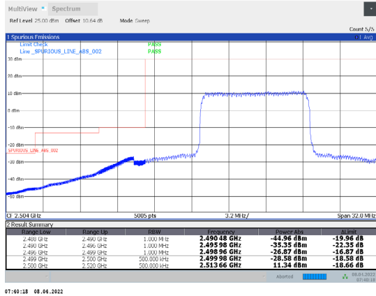
1-N7-PC3-15-20-L-12-DFT-16QAM-Inner_Full-50@25-Ant1-PASS-see graph
