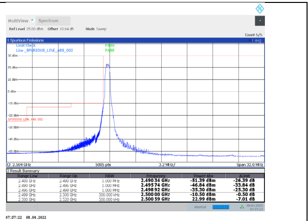
1-N7-PC3-15-20-L-2-DFT-PI/2BPSK-Edge_1RB_Left-1 @0-Ant1-PASS-see graph
