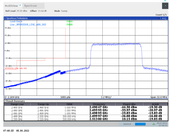
1-N7-PC3-15-20-L-32-CP-64QAM-Inner_Full-53@26-Ant1-PASS-see graph
