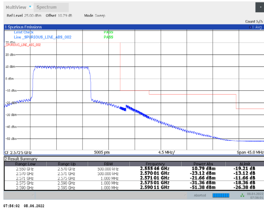
1-N7-PC3-15-20-H-24-CP-QPSK-Inner_Full-53@26-Ant1-PASS-see graph
