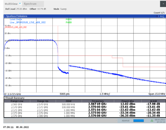
1-N7-PC3-15-5-H-31-CP-64QAM-Outer_Full-25@0-Ant1-PASS-see graph
