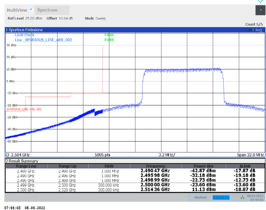
1-N7-PC3-15-20-L-24-CP-QPSK-Inner_Full-53@26-Ant1-PASS-see graph
