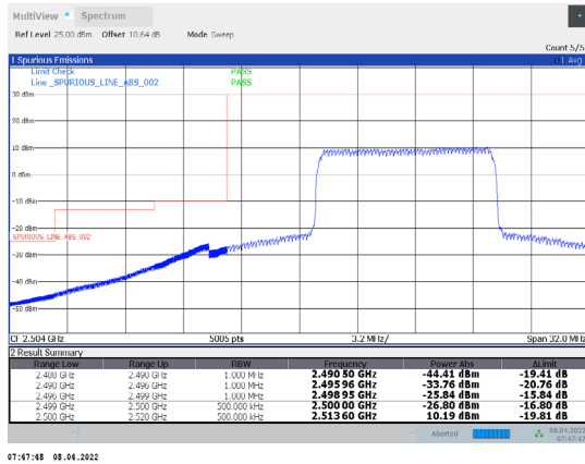
1-N7-PC3-15-20-L-36-CP-256QAM-Inner_Full-53@26-Ant1-PASS-see graph
