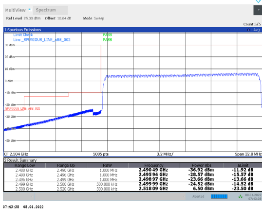
1-N7-PC3-15-20-L-23-CP-QPSK-Outer_Full-106@0-Ant1-PASS-see graph
