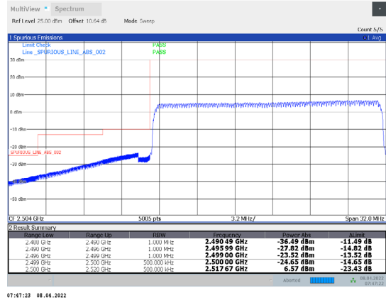
1-N7-PC3-15-20-L-35-CP-256QAM-Outer_Full-106@0-Ant1-PASS-see graph
