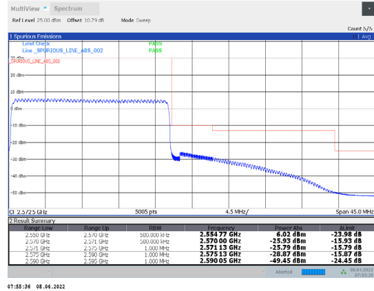
1-N7-PC3-15-20-H-23-CP-QPSK-Outer_Full-106@0-Ant1-PASS-see graph
