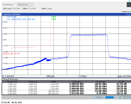
1-N7-PC3-15-20-L-20-DFT-256QAM-Inner_Full-50@25-Ant1-PASS-see graph
