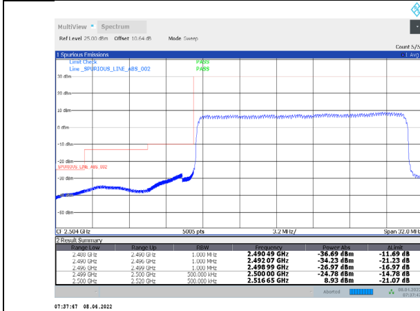
1-N7-PC3-15-20-L-4-DFT-PI/2BPSK-Outer_Full-100@ 0-Ant1-PASS-see graph
