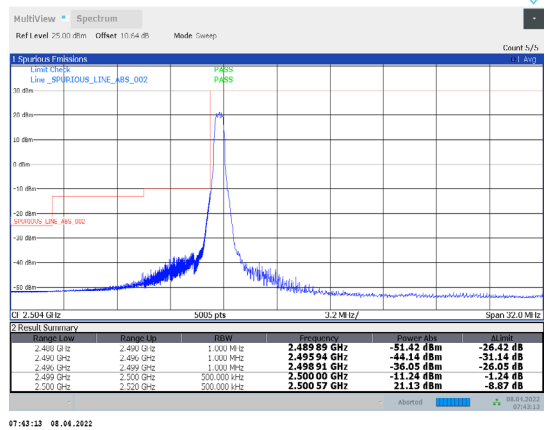
1-N7-PC3-15-20-L-21-CP-QPSK-Edge_1RB_Left-1@0-Ant1-PASS-see graph
