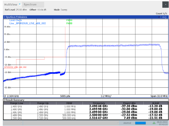
1-N7-PC3-15-20-L-19-DFT-256QAM-Outer_Full-100@0-Ant1-PASS-see graph
