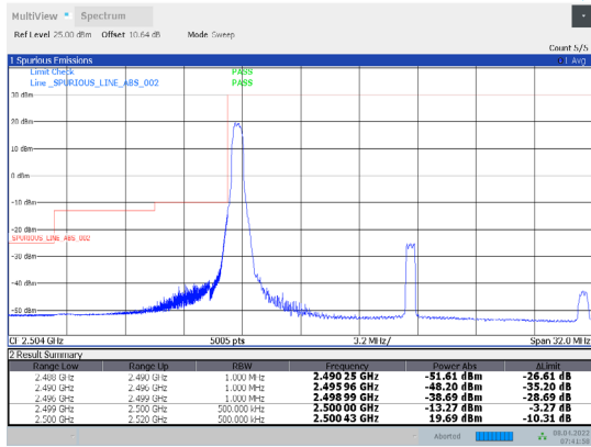
1-N7-PC3-15-20-L-17-DFT-256QAM-Edge_1RB_Left-1@0-Ant1-PASS-see graph
