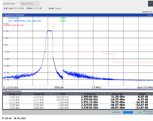
1-N7-PC3-15-5-H-30-CP-64QAM-Edge_1RB_Right-1@24-Ant1-PASS-see graph
