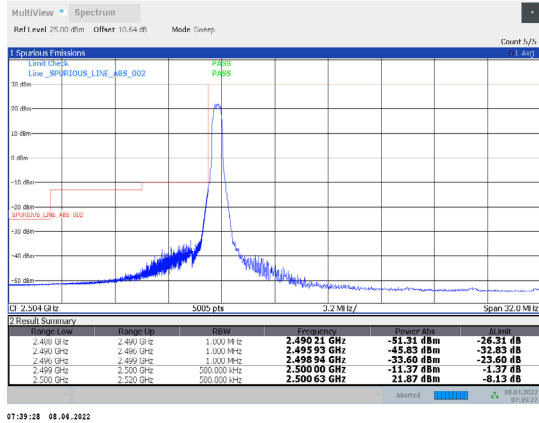
1-N7-PC3-15-20-L-9-DFT-16QAM-Edge_1RB_Left-1@0-Ant1-PASS-see graph
