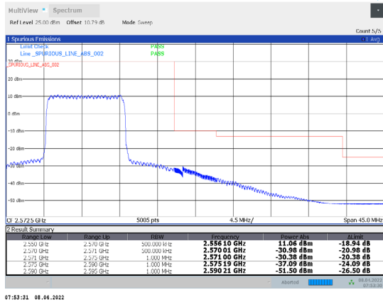
1-N7-PC3-15-20-H-16-DFT-64QAM-Inner_Full-50@25- Ant1-PASS-see graph
