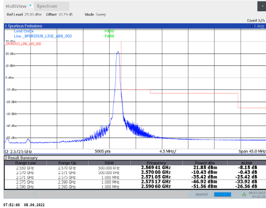
1-N7-PC3-15-20-H-14-DFT-64QAM-Edge_1RB_Right- 1@105-Ant1-PASS-see graph
