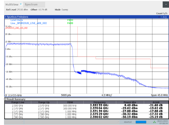
1-N7-PC3-15-20-H-7-DFT-QPSK-Outer_Full-100@0-Ant 1-PASS-see graph
