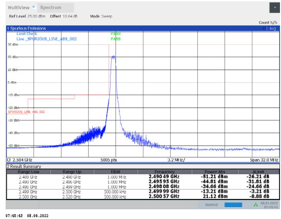
1-N7-PC3-15-20-L-29-CP-64QAM-Edge_1RB_Left-1@0-Ant1-PASS-see graph
