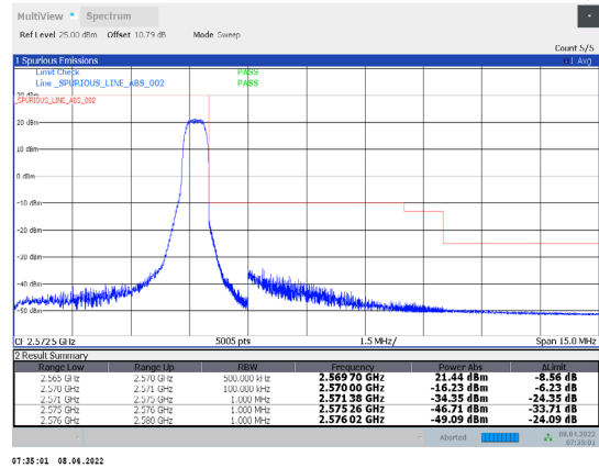
1-N7-PC3-15-5-H-34-CP-256QAM-Edge_1RB_Right-1@24-Ant1-PASS-see graph
