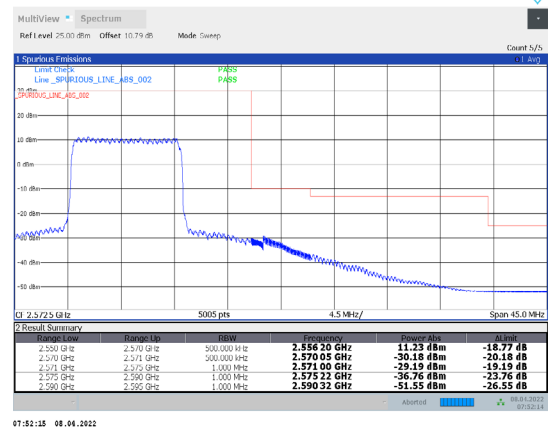
1-N7-PC3-15-20-H-12-DFT-16QAM-Inner_Full-50@25-A nt1-PASS-see graph
