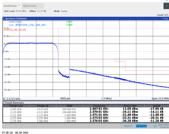
1-N7-PC3-15-5-H-35-CP-256QAM-Outer_Full-25@0-Ant1-PASS-see graph
