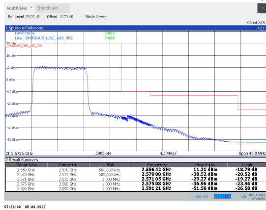
1-N7-PC3-15-20-H-8-DFT-QPSK-Inner_Full-50@25-A nt1-PASS-see graph
