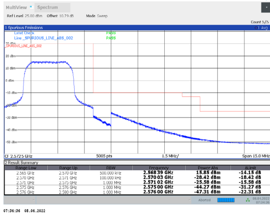
1-N7-PC3-15-5-H-32-CP-64QAM-Inner_Full-13@6-Ant1-PASS-see graph
