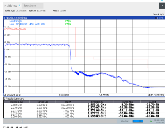
1-N7-PC3-15-20-H-4-DFT-PI/2BPSK-Outer_Full-100@0-Ant1-PASS-see graph
