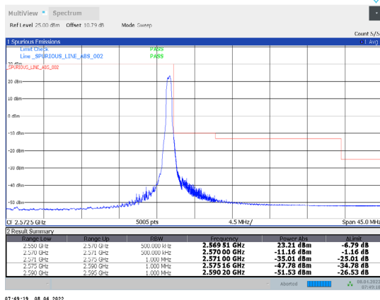
1-N7-PC3-15-20-H-3-DFT-PI/2BPSK-Edge_1RB_Right-1@105-Ant1-PASS-see graph
