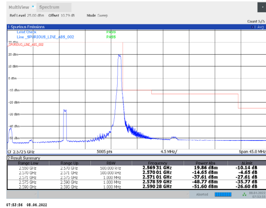
1-N7-PC3-15-20-H-18-DFT-256QAM-Edge_1RB_Right- 1@105-Ant1-PASS-see graph
