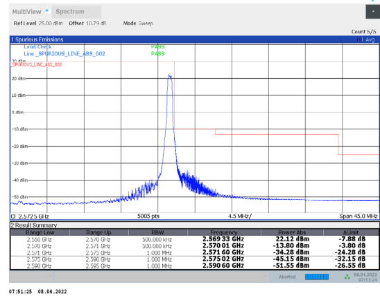
1-N7-PC3-15-20-H-10-DFT-16QAM-Edge_1RB_Right-1 @105-Ant1-PASS-see graph
