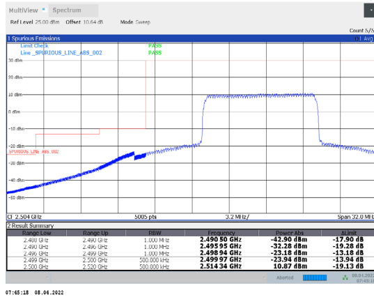
1-N7-PC3-15-20-L-28-CP-16QAM-Inner_Full-53@26-Ant1-PASS-see graph
