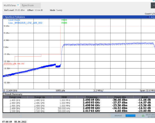
1-N7-PC3-15-20-L-31-CP-64QAM-Outer_Full-106@0-Ant1-PASS-see graph
