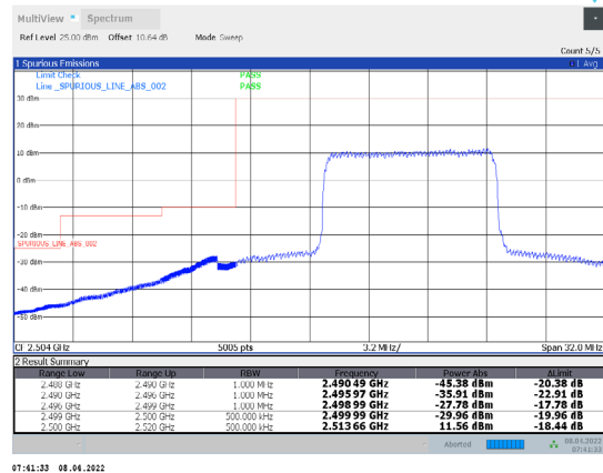
1-N7-PC3-15-20-L-16-DFT-64QAM-Inner_Full-50@25-Ant1-PASS-see graph
