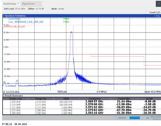
1-N7-PC3-15-20-H-22-CP-QPSK-Edge_1RB_Right-1@105-Ant1-PASS-see graph
