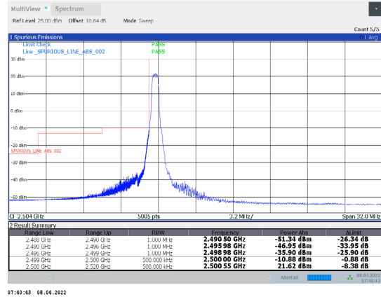
1-N7-PC3-15-20-L-13-DFT-64QAM-Edge_1RB_Left-1@0-Ant1-PASS-see graph
