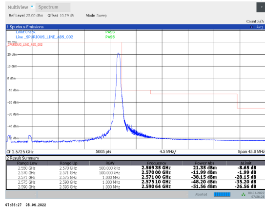
1-N7-PC3-15-20-H-26-CP-16QAM-Edge_1RB_Right-1@105-Ant1-PASS-see graph
