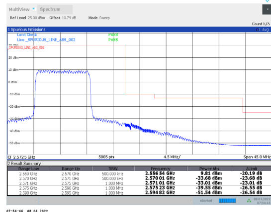
1-N7-PC3-15-20-H-20-DFT-256QAM-Inner_Full-50@25- Ant1-PASS-see graph
