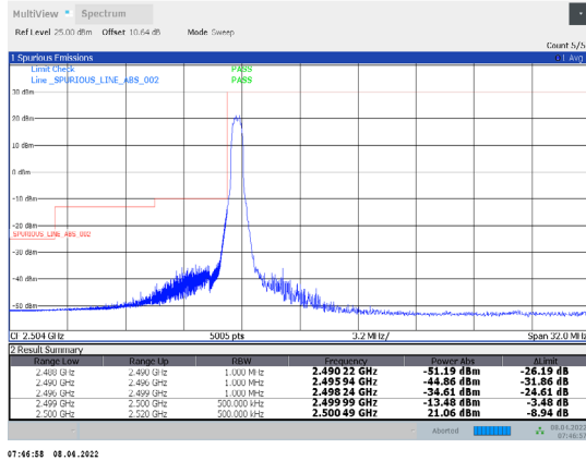
1-N7-PC3-15-20-L-33-CP-256QAM-Edge_1RB_Left-1@0-Ant1-PASS-see graph
