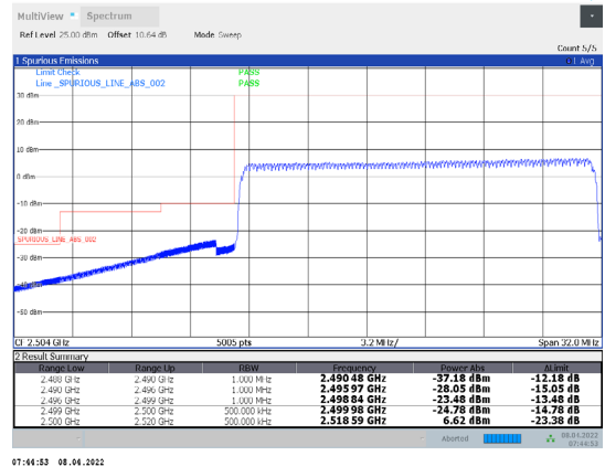
1-N7-PC3-15-20-L-27-CP-16QAM-Outer_Full-106@0-Ant1-PASS-see graph
