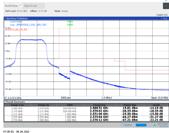
1-N7-PC3-15-5-H-36-CP-256QAM-Inner_Full-13@6-Ant1-PASS-see graph
