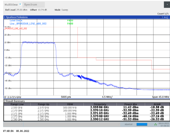
1-N7-PC3-15-20-H-1-DFT-PI/2BPSK-Inner_Full-50@25-Ant1-PASS-see graph
