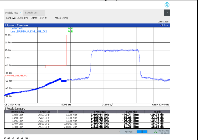
1-N7-PC3-15-20-L-8-DFT-QPSK-Inner_Full-50@25-Ant1 -PASS-see graph
