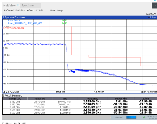
1-N7-PC3-15-20-H-19-DFT-256QAM-Outer_Full-100@ 0-Ant1-PASS-see graph
