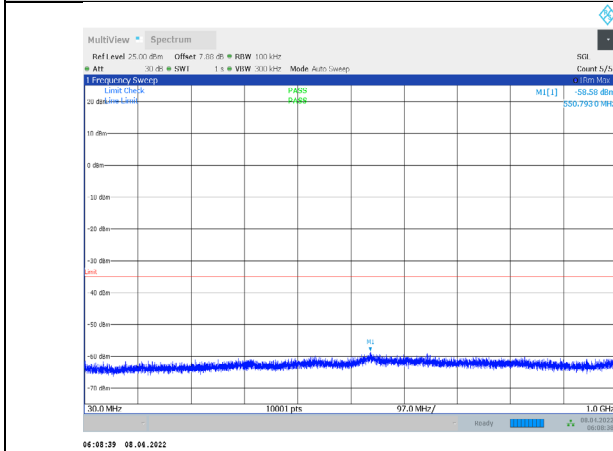
1-N7-PC3-15-5-L-2-CP-QPSK-Edge_1RB_Right-1@24 -30-1000-Ant1--58.58--35-PASS
