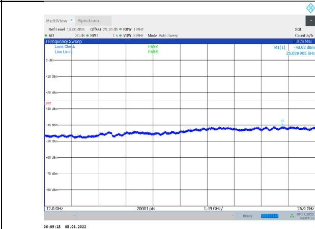
1-N7-PC3-15-5-L-2-CP-QPSK-Edge_1RB_Right-1@24 -12000-26900-Ant1--40.62--25-PASS
