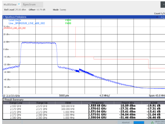
1-N7-PC3-15-20-H-32-CP-64QAM-Inner_Full-53@26-A nt1-PASS-see graph
