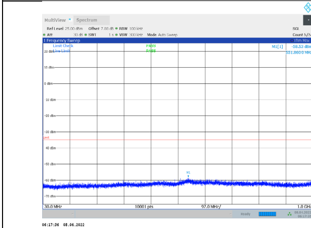
1-N7-PC3-15-5-H-2-CP-QPSK-Edge_1RB_Right-1@24 -30-1000-Ant1--58.53--35-PASS
