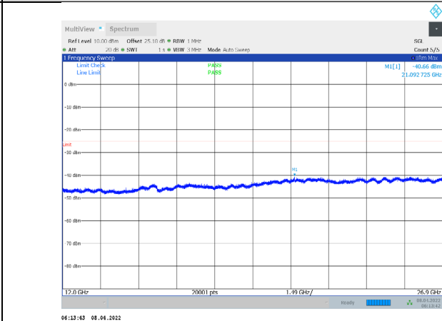
1-N7-PC3-15-5-M-2-CP-QPSK-Edge_1RB_Right-1@24 12000-26900-Ant1--40.66--25-PASS
