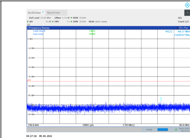
1-N7-PC3-15-5-H-2-CP-QPSK-Edge_1RB_Right-1@24 -0.15-30-Ant1--66.17--45-PASS
