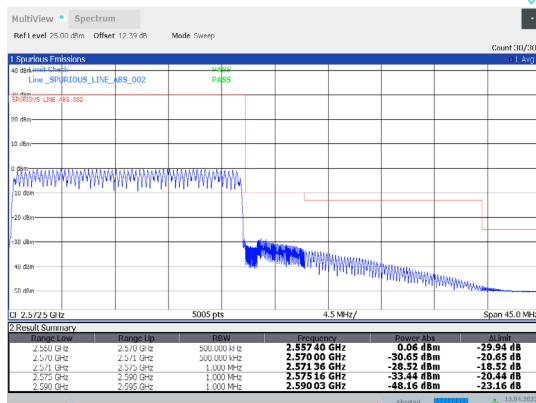
1-N7-PC3-15-20-H-35-CP-256QAM-Outer_Full-106@0-Ant1-PASS-see graph
