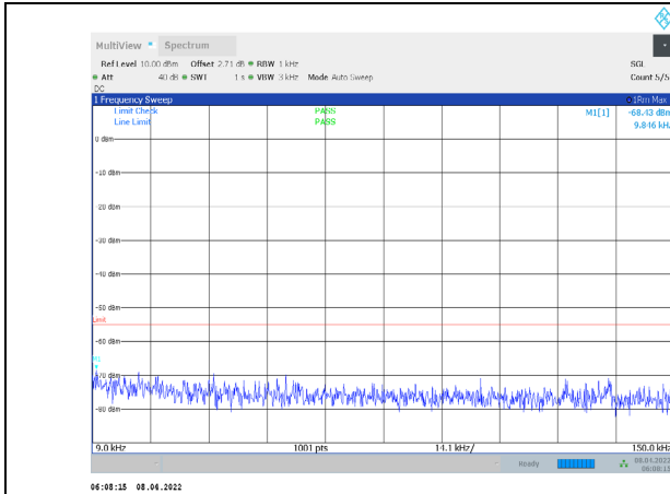
1-N7-PC3-15-5-L-2-CP-QPSK-Edge_1RB_Right-1@24 -0.009-0.15-Ant1--68.43--55-PASS
