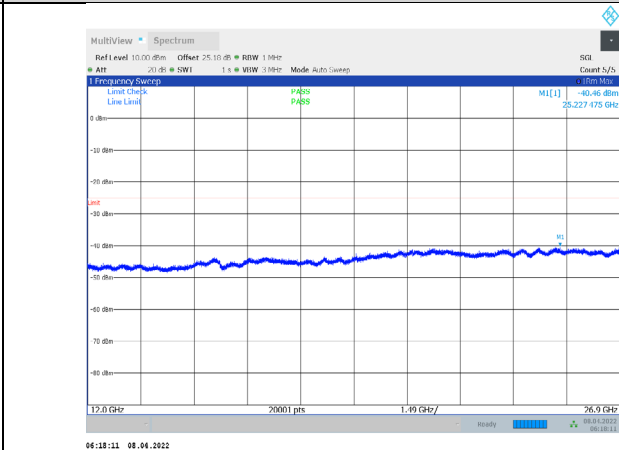
1-N7-PC3-15-5-H-2-CP-QPSK-Edge_1RB_Right-1@24 -12000-26900-Ant1--40.46--25-PASS
