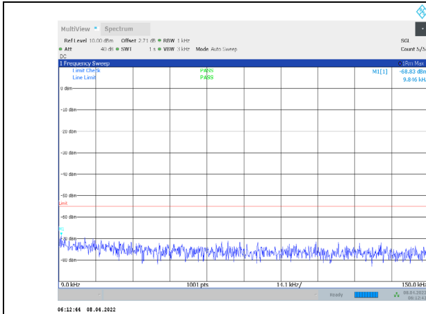
1-N7-PC3-15-5-M-2-CP-QPSK-Edge_1RB_Right-1@24 -0.009-0.15-Ant1--68.83--55-PASS
