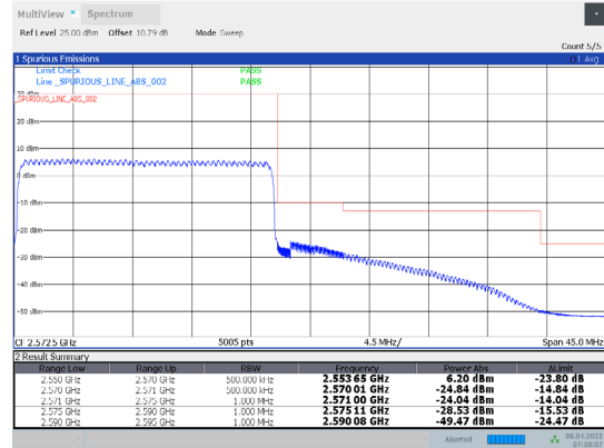
1-N7-PC3-15-20-H-31-CP-64QAM-Outer_Full-106@0-A nt1-PASS-see graph
