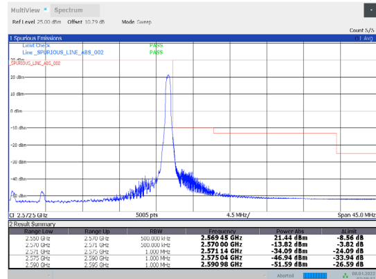
1-N7-PC3-15-20-H-34-CP-256QAM-Edge_1RB_Right-1 @105-Ant1-PASS-see graph
