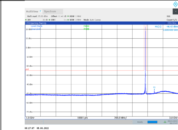
1-N7-PC3-15-5-H-2-CP-QPSK-Edge_1RB_Right-1@24 -1000-3000-Ant1--46.42--25-PASS
