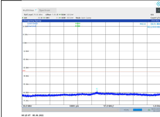
1-N7-PC3-15-5-M-2-CP-QPSK-Edge_1RB_Right-1@24 -30-1000-Ant1--58.91--35-PASS
