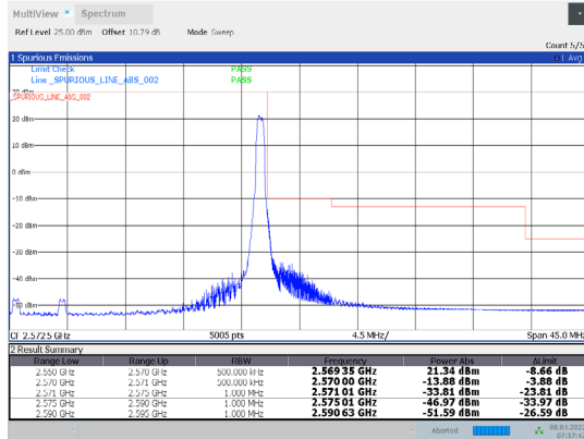
1-N7-PC3-15-20-H-30-CP-64QAM-Edge_1RB_Right-1 @105-Ant1-PASS-see graph
