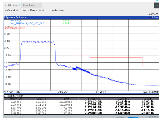
1-N7-PC3-15-20-H-36-CP-256QAM-Inner_Full-53@26-Ant1-PASS-see graph
