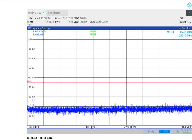
1-N7-PC3-15-5-L-2-CP-QPSK-Edge_1RB_Right-1@24 -0.15-30-Ant1--66.55--45-PASS
