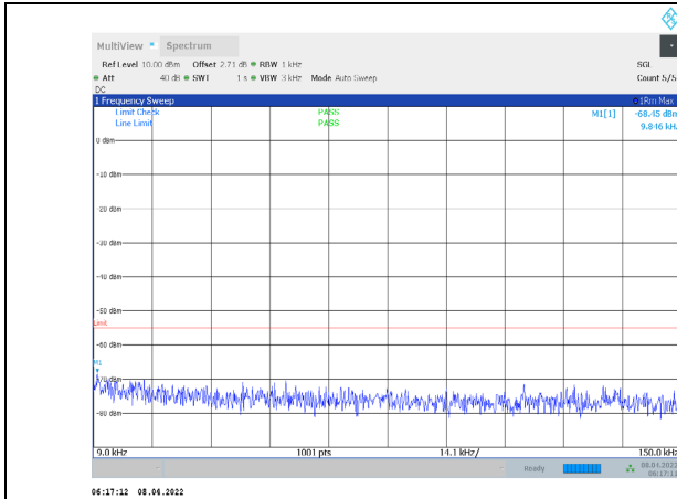
1-N7-PC3-15-5-H-2-CP-QPSK-Edge_1RB_Right-1@24 -0.009-0.15-Ant1--68.45--55-PASS
