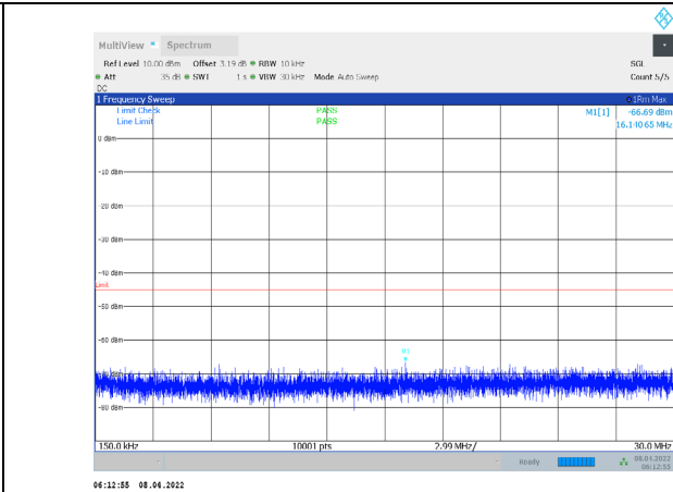
1-N7-PC3-15-5-M-2-CP-QPSK-Edge_1RB_Right-1@24 0.15-30-Ant1--66.69--45-PASS
