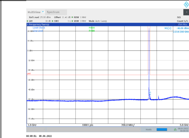
1-N7-PC3-15-5-L-2-CP-QPSK-Edge_1RB_Right-1@24 -1000-3000-Ant1--46.06--25-PASS
