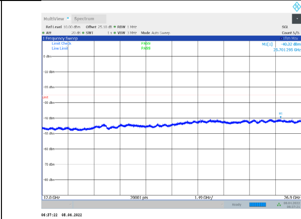
1-N7-PC3-15-20-L-3-CP-QPSK-Outter_Full-106@0-1200- 0-26900-Ant1--40.32--25-PASS
