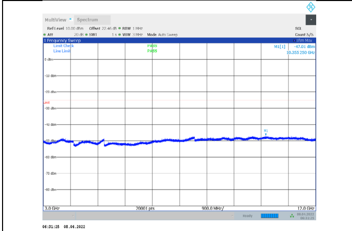
1-N7-PC3-15-15-H-2-CP-QPSK-Edge_1RB_Right-1@7 8-3000-12000-Ant1--47.01--25-PASS
