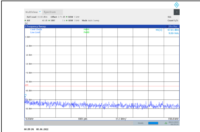
1-N7-PC3-15-20-M-2-CP-QPSK-Edge_1RB_Right-1@1 05-0.009-0.15-Ant1--67.81--55-PASS
