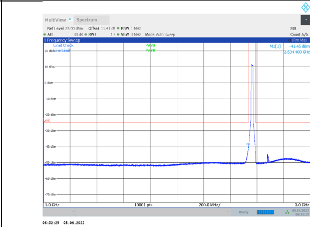
1-N7-PC3-15-15-H-3-CP-QPSK-Outter_Full-79@0-1000- 3000-Ant1--41.45--25-PASS
