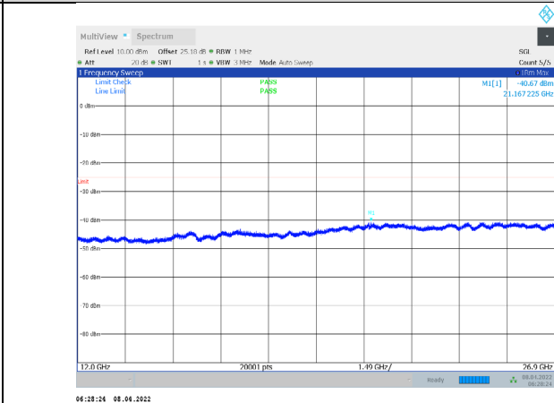
1-N7-PC3-15-15-M-3-CP-QPSK-Outter_Full-79@0-1200 0-26900-Ant1--40.67--25-PASS
