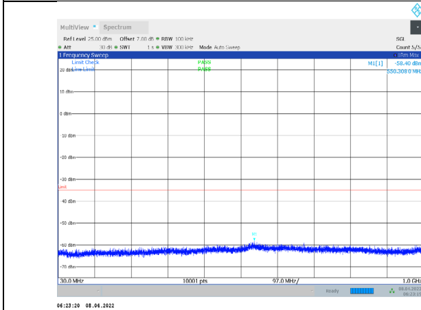
1-N7-PC3-15-15-L-3-CP-QPSK-Outter_Full-79@0-30-1 000-Ant1--58.40--35-PASS
