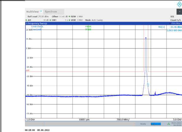
1-N7-PC3-15-15-M-3-CP-QPSK-Outter_Full-79@0-1000- 3000-Ant1--41.46--25-PASS
