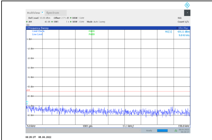
1-N7-PC3-15-15-H-2-CP-QPSK-Edge_1RB_Right-1@7 8-0.009-0.15-Ant1--69.11--55-PASS
