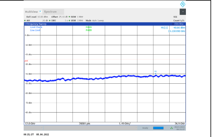
1-N7-PC3-15-15-H-2-CP-QPSK-Edge_1RB_Right-1@7 8-12000-26900-Ant1--40.66--25-PASS
