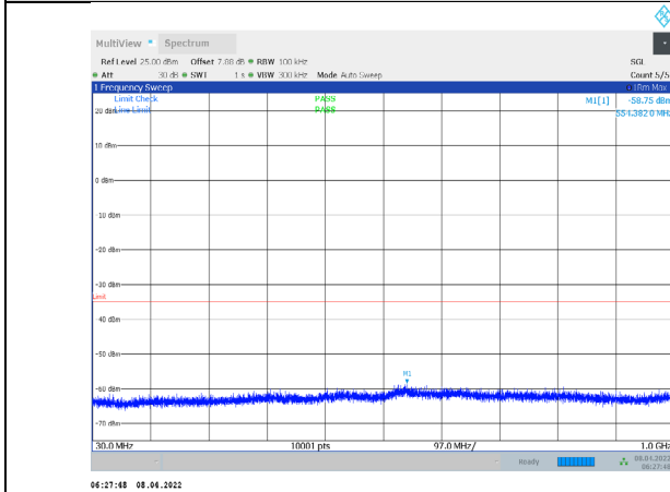
1-N7-PC3-15-15-M-3-CP-QPSK-Outter_Full-79@0-30-1 000-Ant1--58.75--35-PASS
