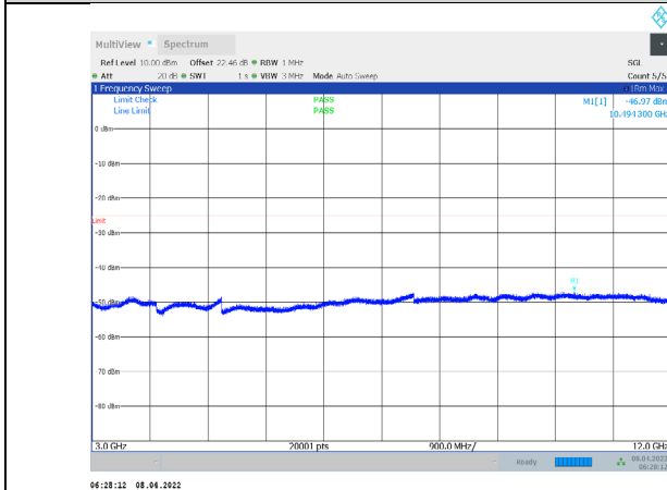
1-N7-PC3-15-15-M-3-CP-QPSK-Outter_Full-79@0-300 0-12000-Ant1--46.97--25-PASS
