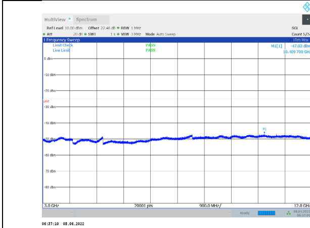
1-N7-PC3-15-20-L-3-CP-QPSK-Outter_Full-106@0-300- 0-12000-Ant1--47.03--25-PASS
