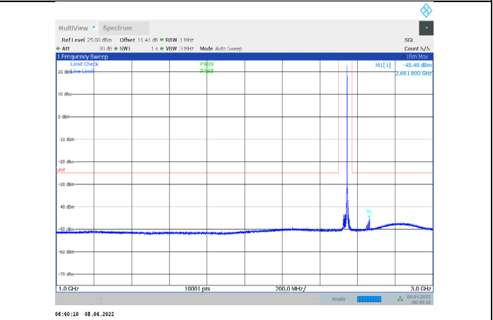
1-N7-PC3-15-20-M-2-CP-QPSK-Edge_1RB_Right-1@1 05-1000-3000-Ant1--45.48--25-PASS
