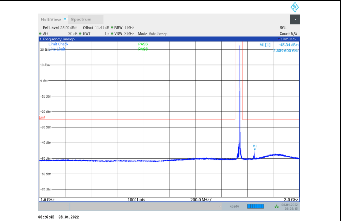
1-N7-PC3-15-15-M-2-CP-QPSK-Edge_1RB_Right-1@7 8-1000-3000-Ant1--45.34--25-PASS
