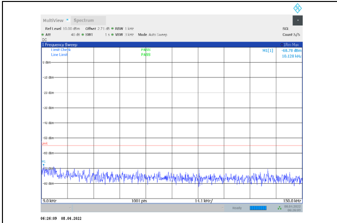
1-N7-PC3-15-15-M-2-CP-QPSK-Edge_1RB_Right-1@7 8-0.009-0.15-Ant1--68.78--55-PASS
