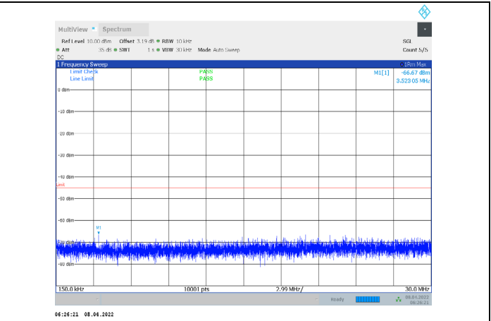
1-N7-PC3-15-15-M-2-CP-QPSK-Edge_1RB_Right-1@7 8-0.15-30-Ant1--66.67--45-PASS
