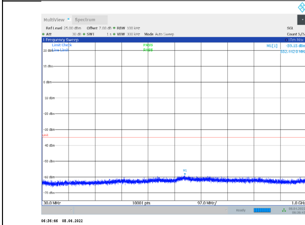
1-N7-PC3-15-20-L-3-CP-QPSK-Outter_Full-106@0-30- 1000-Ant1--59.15--35-PASS
