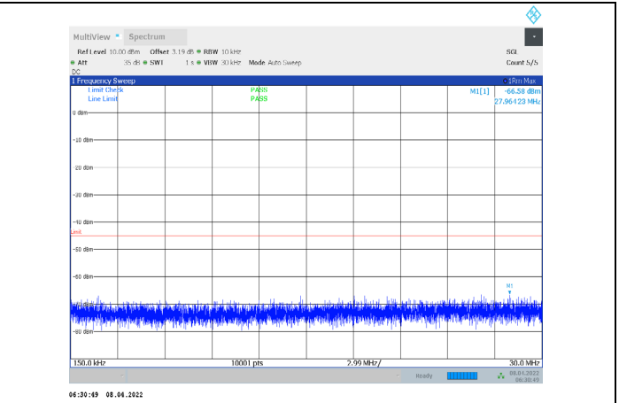
1-N7-PC3-15-15-H-2-CP-QPSK-Edge_1RB_Right-1@7 8-0.15-30-Ant1--66.58--45-PASS
