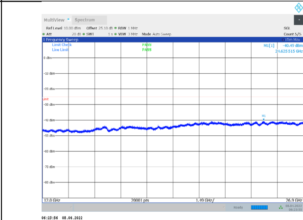
1-N7-PC3-15-15-L-3-CP-QPSK-Outter_Full-79@0-12000 -26900-Ant1--40.49--25-PASS
