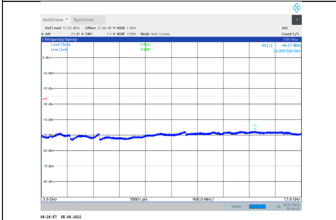
1-N7-PC3-15-15-M-2-CP-QPSK-Edge_1RB_Right-1@7 8-3000-12000-Ant1--46.97--25-PASS
