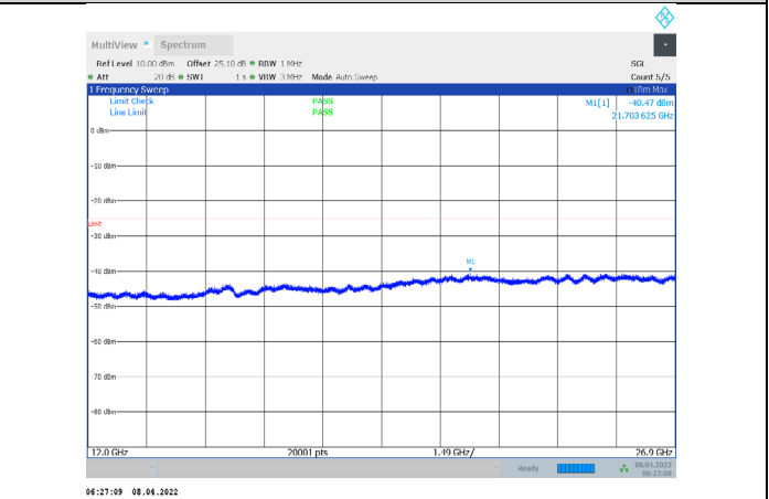
1-N7-PC3-15-15-M-2-CP-QPSK-Edge_1RB_Right-1@7 8-12000-26900-Ant1--40.47--25-PASS
