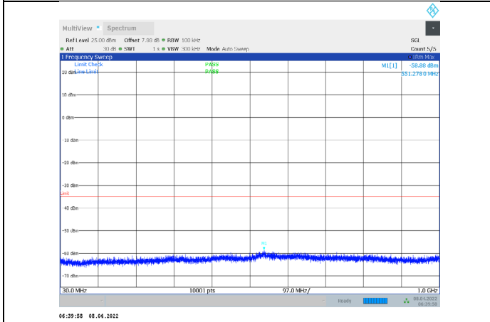
1-N7-PC3-15-20-M-2-CP-QPSK-Edge_1RB_Right-1@1 05-30-1000-Ant1--58.88--35-PASS
