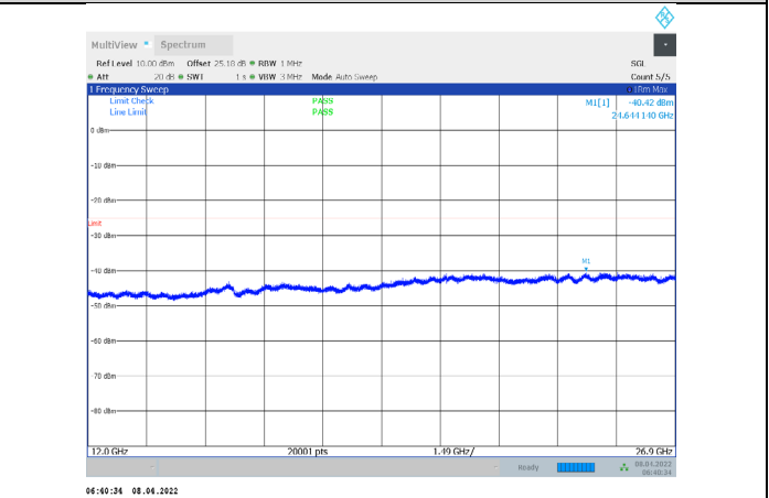
1-N7-PC3-15-20-M-2-CP-QPSK-Edge_1RB_Right-1@1 05-12000-26900-Ant1--40.42--25-PASS
