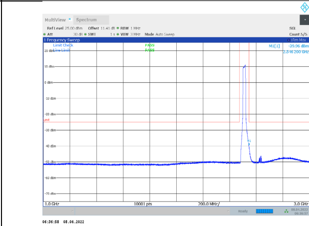
1-N7-PC3-15-20-L-3-CP-QPSK-Outter_Full-106@0-1000- 3000-Ant1--39.96--25-PASS
