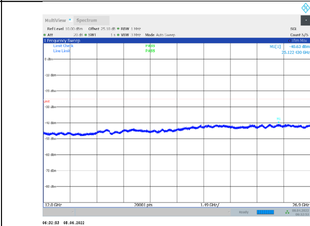
1-N7-PC3-15-15-H-3-CP-QPSK-Outter_Full-79@0-1200 0-26900-Ant1--40.63--25-PASS
