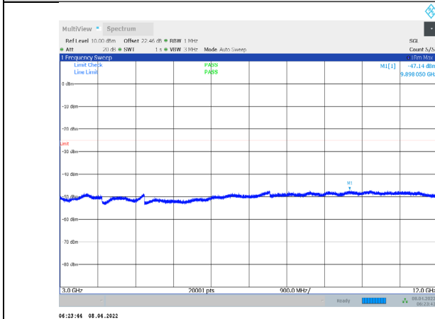
1-N7-PC3-15-15-L-3-CP-QPSK-Outter_Full-79@0-3000 -12000-Ant1--47.14--25-PASS
