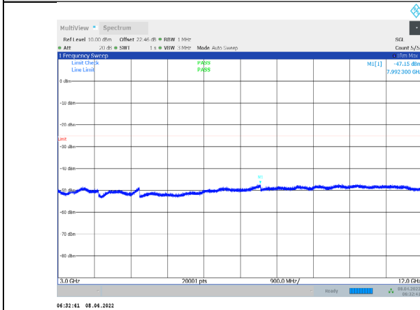
1-N7-PC3-15-15-H-3-CP-QPSK-Outter_Full-79@0-3000 -12000-Ant1--47.15--25-PASS
