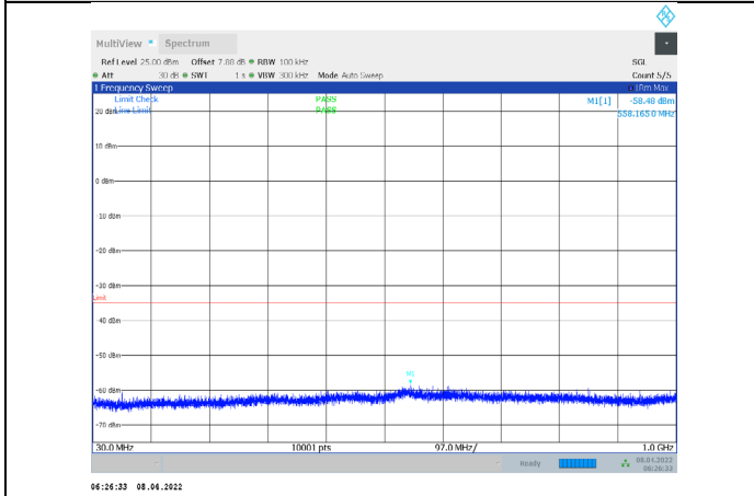
1-N7-PC3-15-15-M-2-CP-QPSK-Edge_1RB_Right-1@7 8-30-1000-Ant1--58.48--35-PASS
