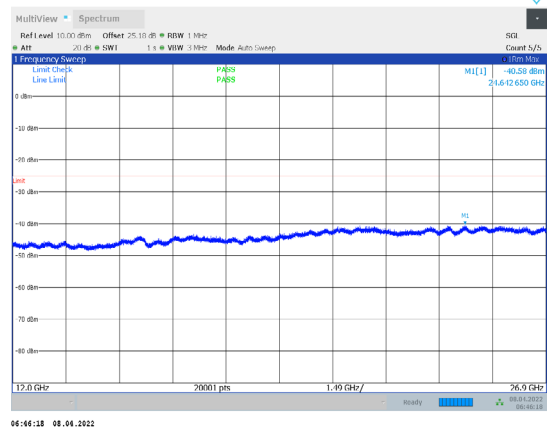
1-N7-PC3-15-20-H-3-CP-QPSK-Outter_Full-106@0-120 00-26900-Ant1--40.58--25-PASS
