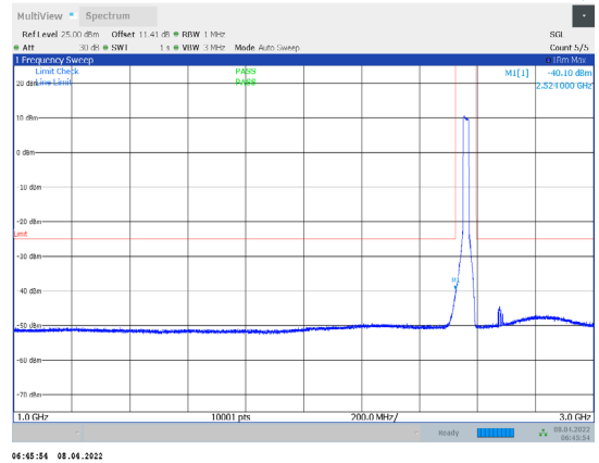
1-N7-PC3-15-20-H-3-CP-QPSK-Outter_Full-106@0-100 0-3000-Ant1--40.10--25-PASS
