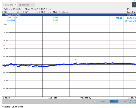
1-N7-PC3-15-20-H-3-CP-QPSK-Outter_Full-106@0-300 0-12000-Ant1--47.09--25-PASS
