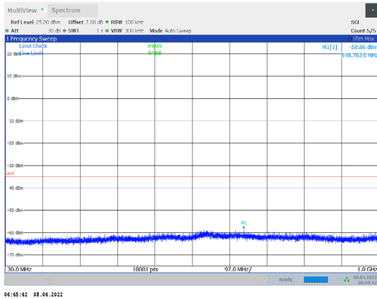
1-N7-PC3-15-20-H-3-CP-QPSK-Outter_Full-106@0-30- 1000-Ant1--58.86--35-PASS
