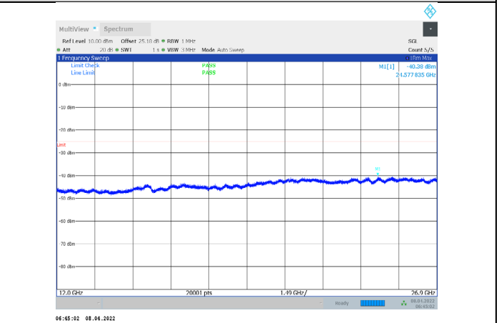
1-N7-PC3-15-20-H-2-CP-QPSK-Edge_1RB_Right-1@1 05-12000-26900-Ant1--40.38--25-PASS
