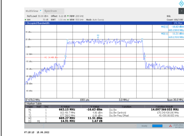
1-N71-PC3-15-15-L-4-CP-256QAM-Outer_Full-79@0-A nt1-14.098-14.910-≤15-PASS
