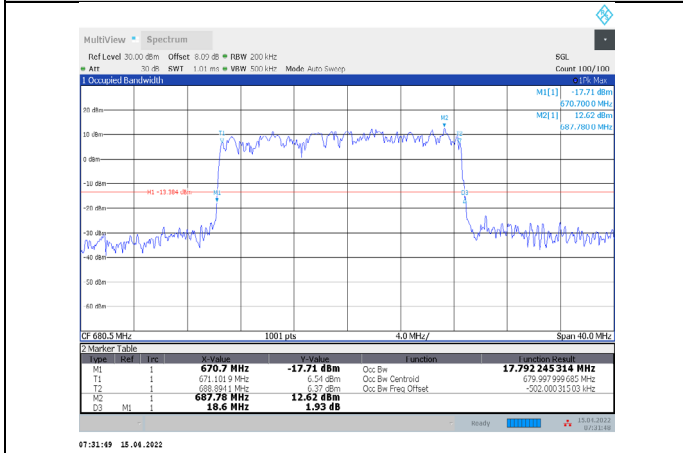
1-N71-PC3-15-20-M-8-DFT-64QAM-Outer_Full-100@0-Ant1-17.792-18.600-≤20-PASS
