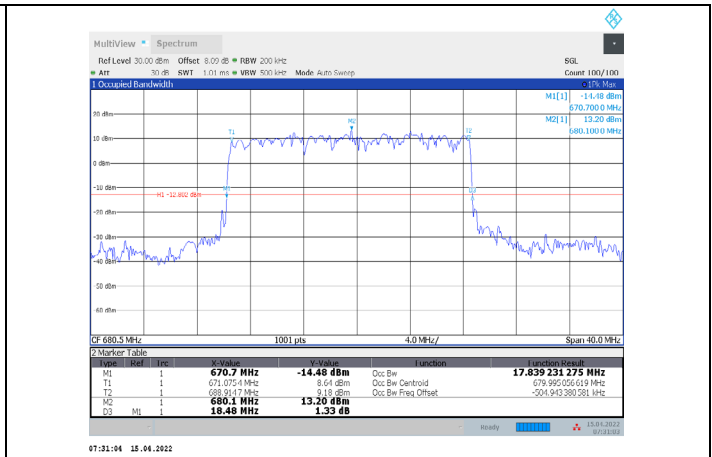
1-N71-PC3-15-20-M-5-DFT-PI/2BPSK-Outer_Full-100@0-Ant1-17.839-18.480-≤20-PASS
