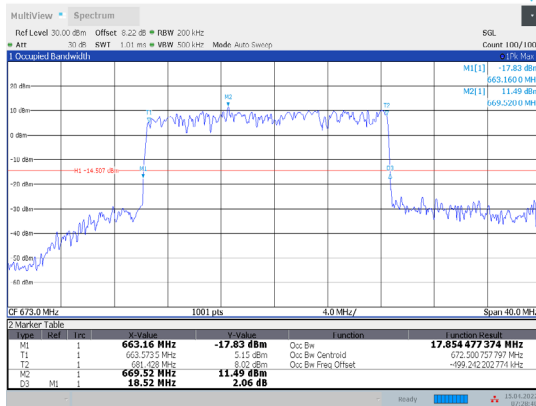
1-N71-PC3-15-20-L-9-DFT-256QAM-Outer_Full-100@0-Ant1-17.854-18.520-≤20-PASS
