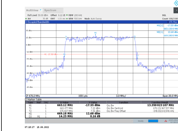
1-N71-PC3-15-15-L-5-DFT-PI/2BPSK-Outer_Full-75@0- Ant1-13.35-14.250-≤15-PASS
