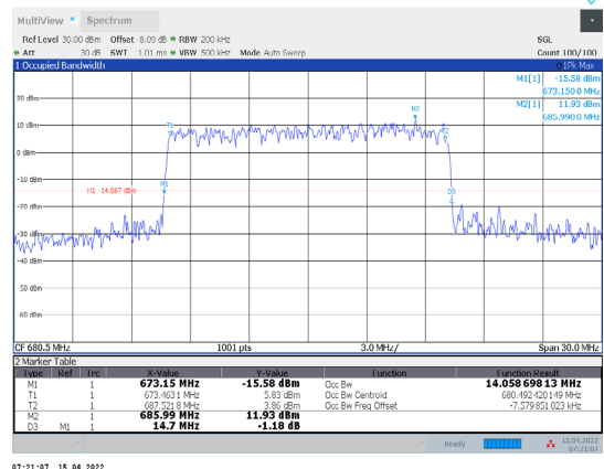
1-N71-PC3-15-15-M-3-CP-64QAM-Outer_Full-79@0-A nt1-14.059-14.700-≤15-PASS
