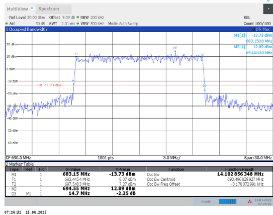
1-N71-PC3-15-15-H-4-CP-256QAM-Outer_Full-79@0-A Ant1-14.103-14.700≤15-PASS
