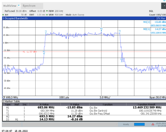
1-N71-PC3-15-15-H-5-DFT-PI/2BPSK-Outer_Full-75@0-A Ant1-13.469-14.130≤15-PASS
