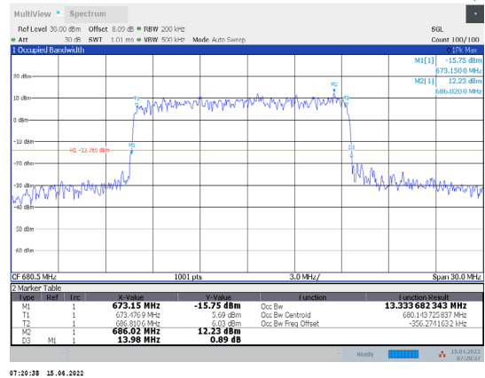
1-N71-PC3-15-15-M-1-CP-QPSK-Outer_Full-75@0-Ant 1-13.334-13.980-≤15-PASS
