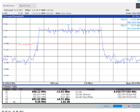
1-N71-PC3-15-10-H-5-DFT-PI/2BPSK-Outer_Full-50@0-Ant1 -8.921-9.340-≤10-PASS
