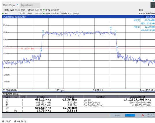
1-N71-PC3-15-15-H-3-CP-64QAM-Outer_Full-79@0-Ant 1-14.123-14.730≤15-PASS
