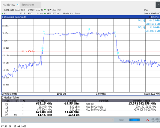
1-N71-PC3-15-15-L-9-DFT-256QAM-Outer_Full-75@0-A Ant1-13.372-14.160-≤15-PASS
