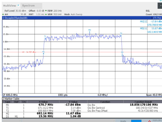
1-N71-PC3-15-20-M-2-CP-16QAM-Outer_Full-106@0-Ant1-18.856-19.560-≤20-PASS
