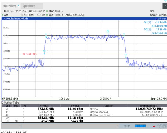
1-N71-PC3-15-15-M-2-CP-16QAM-Outer_Full-79@0-A t1-14.024-14.700-≤15-PASS
