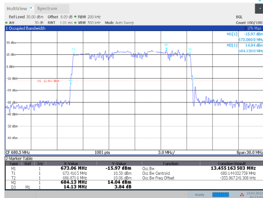
1-N71-PC3-15-15-M-6-DFT-QPSK-Out_75@0-Ant1-13.455-14.130-≤15-PASS
