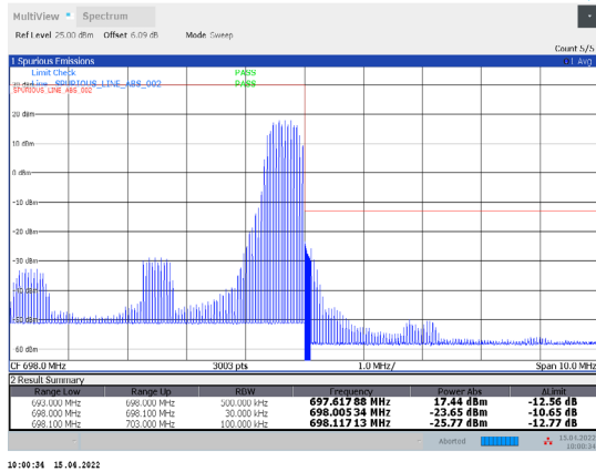
1-N71-PC3-15-5-H-22-CP-QPSK-Edge_1RB_Right-1@24-Ant1-PASS-see graph
