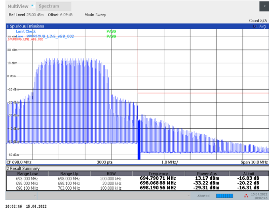
1-N71-PC3-15-5-H-28-CP-16QAM-Inner_Full-13@6-Ant 1-PASS-see graph
