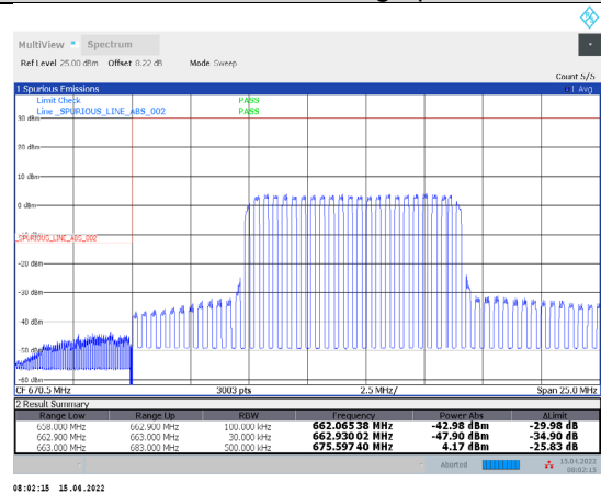
1-N71-PC3-15-20-L-8-DFT-QPSK-Inner_Full-50@25-Ant1-PASS-see graph
