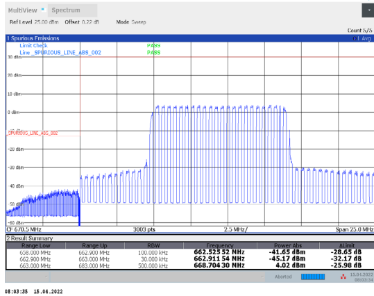
1-N71-PC3-15-20-L-12-DFT-16QAM-Inner_Full-50@25-Ant1-PASS-see graph
