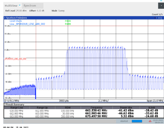
1-N71-PC3-15-20-L-16-DFT-64QAM-Inner_Full-50@25-Ant1-PASS-see graph
