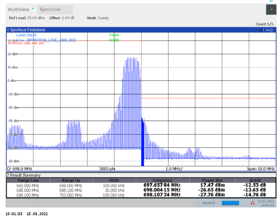
1-N71-PC3-15-5-H-26-CP-16QAM-Edge_1RB_Right-1@24-Ant1-PASS-see graph
