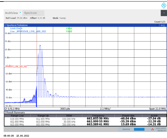
1-N71-PC3-15-20-L-2-DFT-PI/2BPSK-Edge_1RB_Left-1@0-Ant1-PASS-see graph
