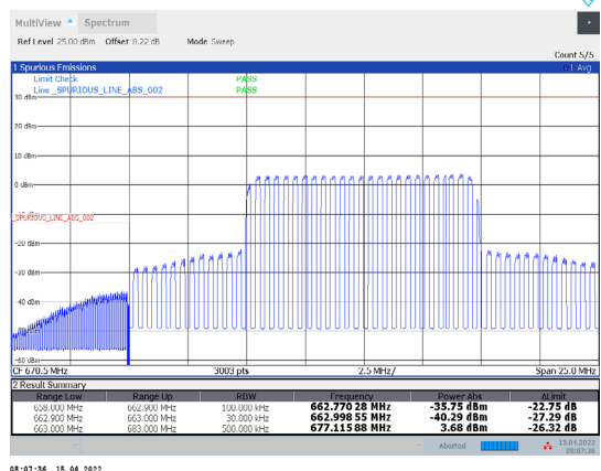
1-N71-PC3-15-20-L-24-CP-QPSK-Inner_Full-53@26-Ant1-PASS-see graph
