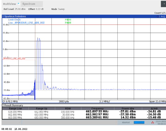
1-N71-PC3-15-20-L-25-CP-16QAM-Edge_1RB_Left-1 @0-Ant1-PASS-see graph
