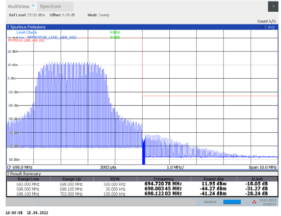
1-N71-PC3-15-5-H-20-DFT-256QAM-Inner_Full-12@6-Ant1-PASS-see graph
