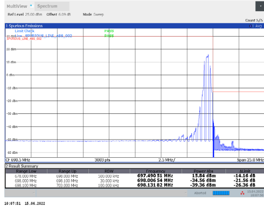
1-N71-PC3-15-20-H-6-DFT-QPSK-Edge_1RB_Right-1 @105-Ant1-PASS-see graph
