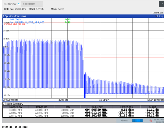
1-N71-PC3-15-5-H-19-DFT-256QAM-Outer_Full-25@0-Ant1-PASS-see graph
