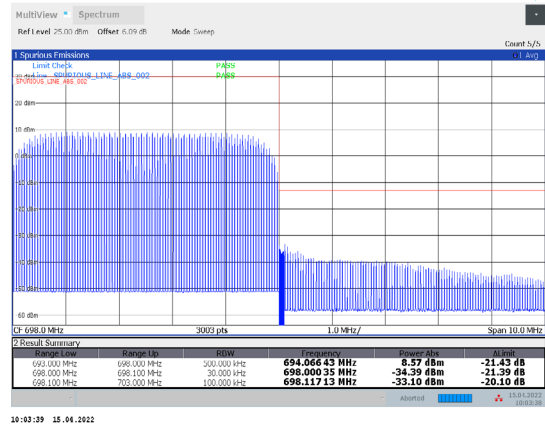
1-N71-PC3-15-5-H-31-CP-64QAM-Outer_Full-25@0-Ant 1-PASS-see graph
