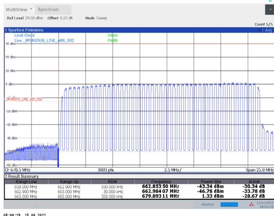
1-N71-PC3-15-20-L-15-DFT-64QAM-Outer_Full-100@0-Ant1-PASS-see graph
