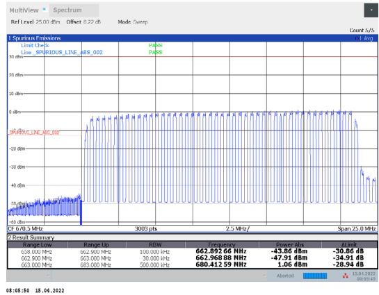
1-N71-PC3-15-20-L-19-DFT-256QAM-Outer_Full-100 @0-Ant1-PASS-see graph
