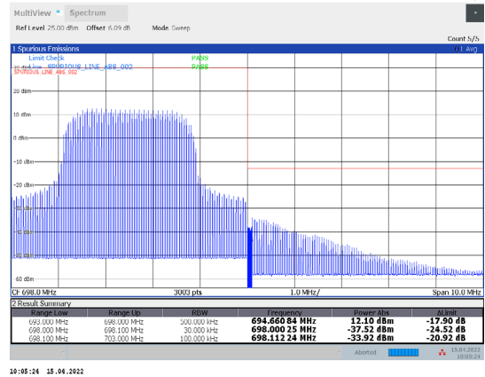
1-N71-PC3-15-5-H-36-CP-256QAM-Inner_Full-13@6-A nt1-PASS-see graph
