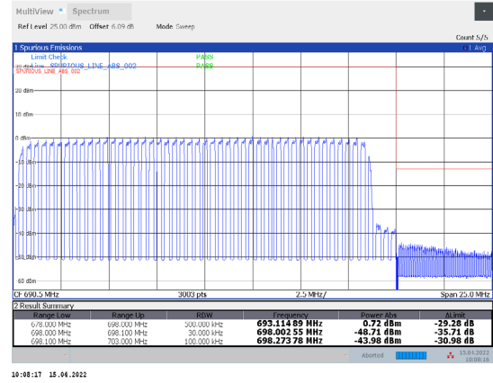
1-N71-PC3-15-20-H-7-DFT-QPSK-Outer_Full-100@0-An t1-PASS-see graph
