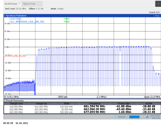
1-N71-PC3-15-20-L-11-DFT-16QAM-Outer_Full-100@0-Ant1-PASS-see graph
