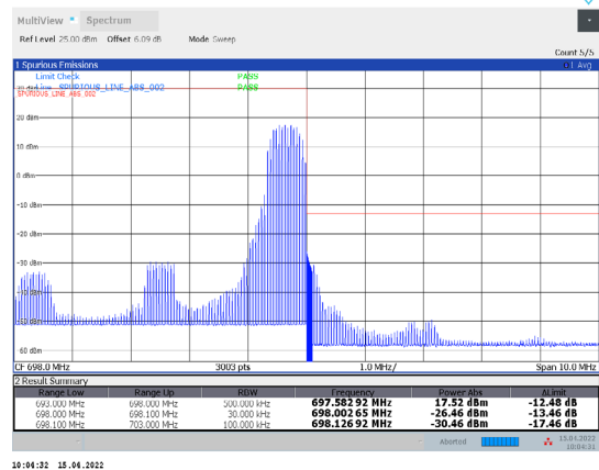
1-N71-PC3-15-5-H-34-CP-256QAM-Edge_1RB_Right-1 @24-Ant1-PASS-see graph
