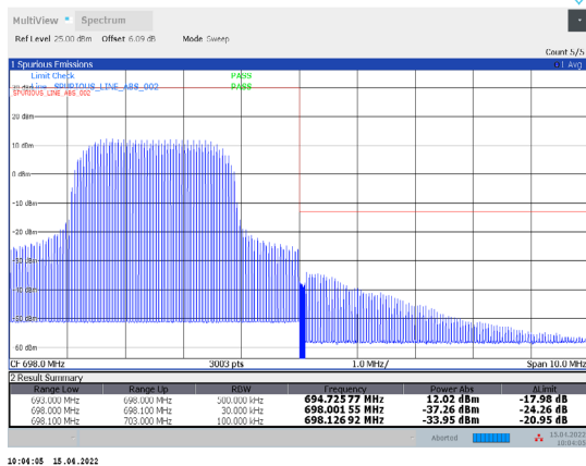
1-N71-PC3-15-5-H-32-CP-64QAM-Inner_Full-13@6-Ant t1-PASS-see graph
