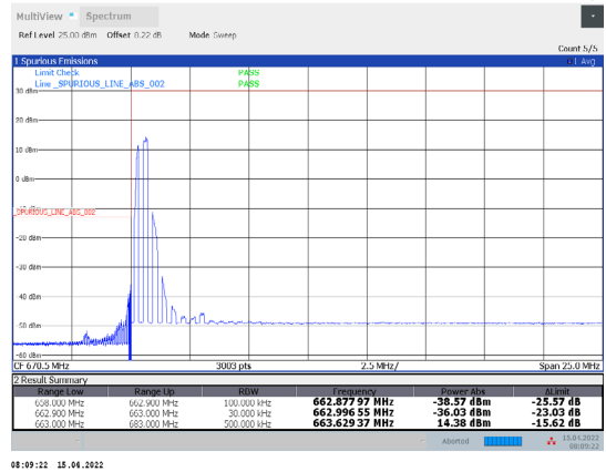
1-N71-PC3-15-20-L-29-CP-64QAM-Edge_1RB_Left-1 @0-Ant1-PASS-see graph
