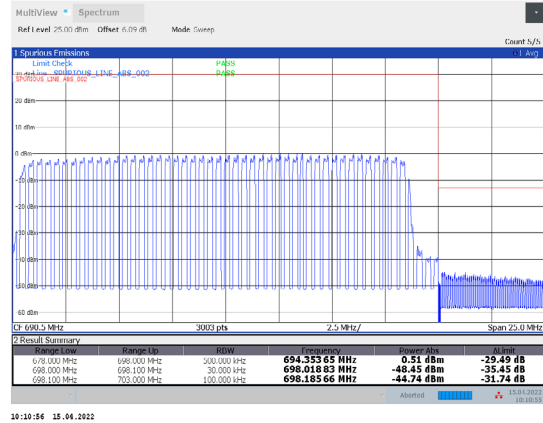
1-N71-PC3-15-20-H-15-DFT-64QAM-Outer_Full-100@0 -Ant1-PASS-see graph
