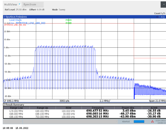
1-N71-PC3-15-20-H-8-DFT-QPSK-Inner_Full-50@25-Ant1-PASS-see graph
