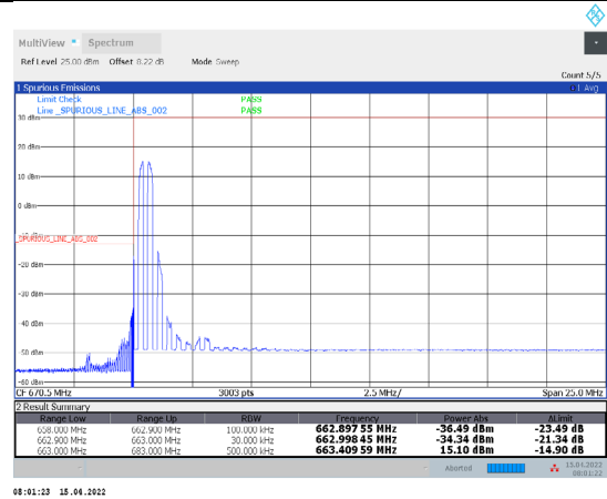
1-N71-PC3-15-20-L-5-DFT-QPSK-Edge_1RB_Left-1@0-Ant1-PASS-see graph
