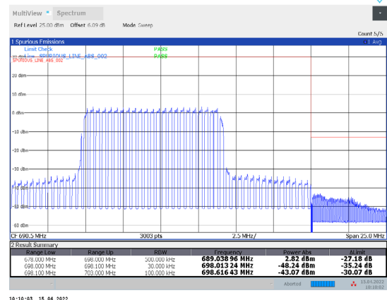
1-N71-PC3-15-20-H-12-DFT-16QAM-Inner_Full-50@25-Ant1-PASS-see graph
