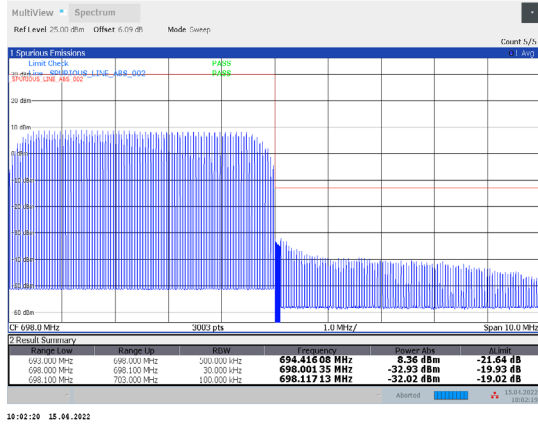
1-N71-PC3-15-5-H-27-CP-16QAM-Outer_Full-25@0-A nt1-PASS-see graph
