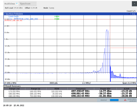
1-N71-PC3-15-20-H-10-DFT-16QAM-Edge_1RB_Right-1 @105-Ant1-PASS-see graph
