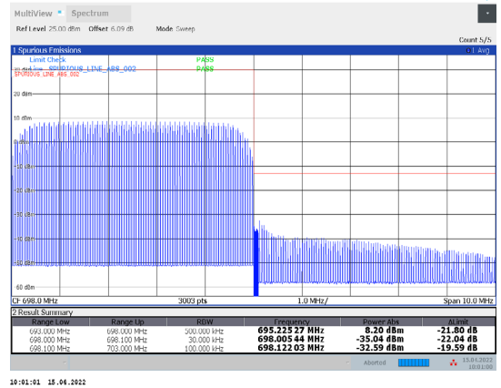
1-N71-PC3-15-5-H-23-CP-QPSK-Outer_Full-25@0-Ant1-PASS-see graph
