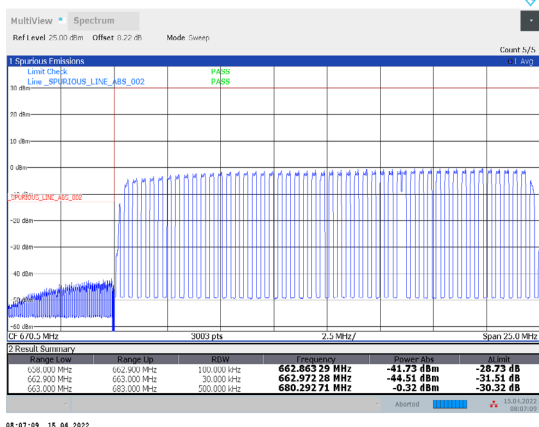
1-N71-PC3-15-20-L-23-CP-QPSK-Outer_Full-106@0-Ant1-PASS-see graph
