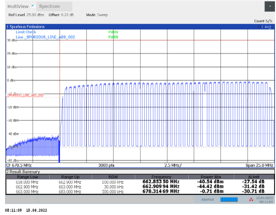
1-N71-PC3-15-20-L-35-CP-256QAM-Outer_Full-106@0 -Ant1-PASS-see graph
