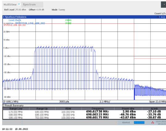
1-N71-PC3-15-20-H-16-DFT-64QAM-Inner_Full-50@25 -Ant1-PASS-see graph
