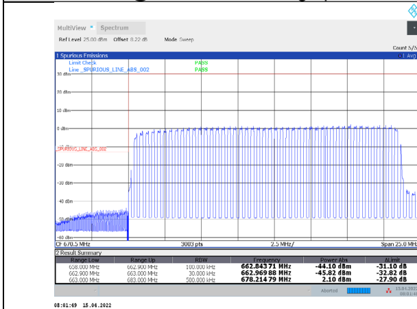
1-N71-PC3-15-20-L-7-DFT-QPSK-Outer_Full-100@0-Ant1-PASS-see graph
