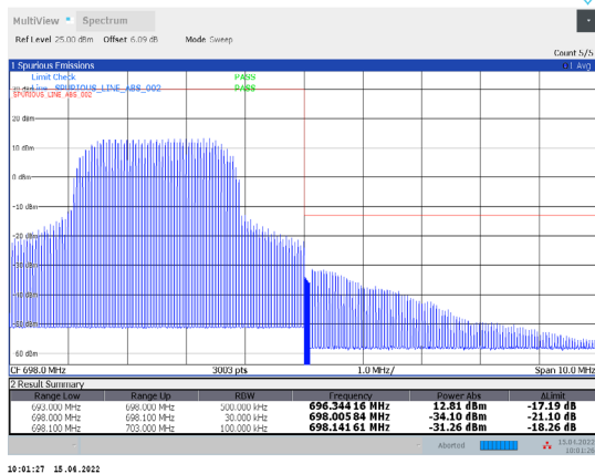
1-N71-PC3-15-5-H-24-CP-QPSK-Inner_Full-13@6-Ant1-PASS-see graph
