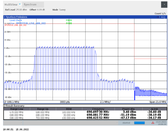
1-N71-PC3-15-20-H-1-DFT-PI/2BPSK-Inner_Full-50@2 5-Ant1-PASS-see graph
