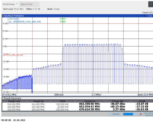
1-N71-PC3-15-20-L-28-CP-16QAM-Inner_Full-53@26-Ant1-PASS-see graph
