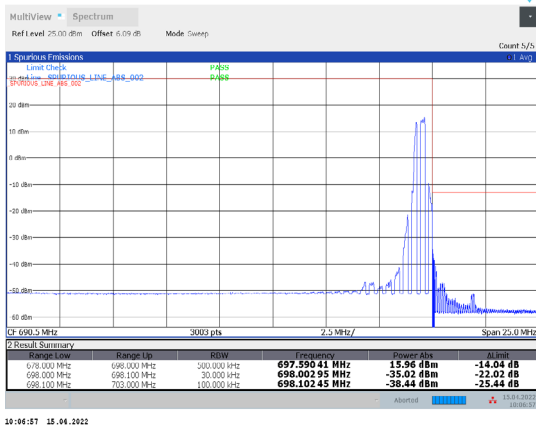
1-N71-PC3-15-20-H-3-DFT-PI/2BPSK-Edge_1RB_Right -1@105-Ant1-PASS-see graph
