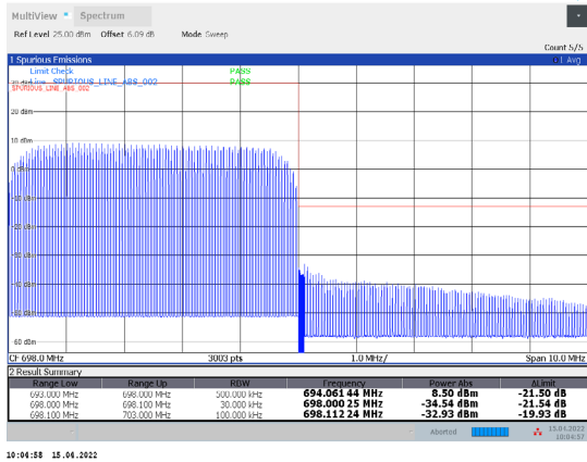
1-N71-PC3-15-5-H-35-CP-256QAM-Outer_Full-25@0-A nt1-PASS-see graph
