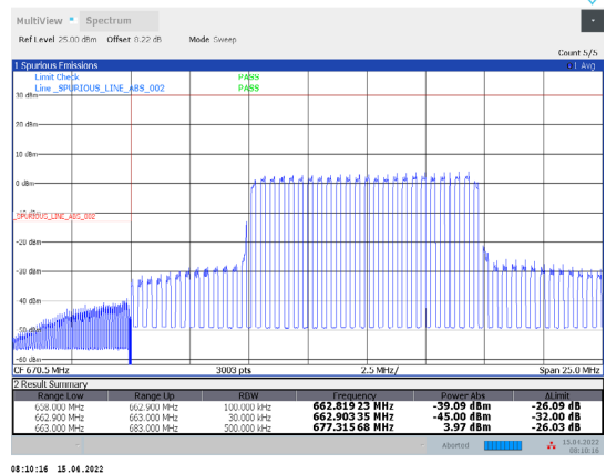
1-N71-PC3-15-20-L-32-CP-64QAM-Inner_Full-53@26-Ant1-PASS-see graph
