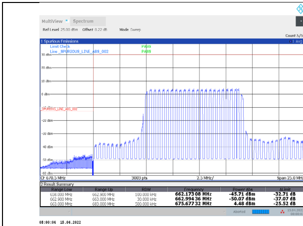
1-N71-PC3-15-20-L-1-DFT-PI/2BPSK-Inner_Full-50@25-Ant1-PASS-see graph
