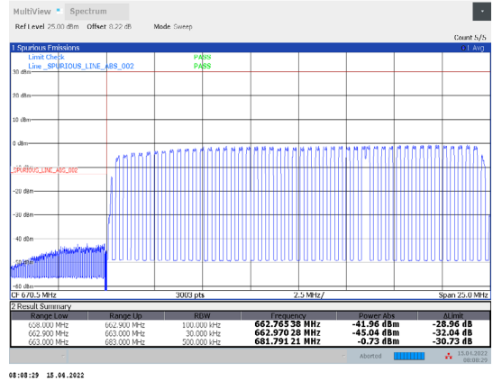
1-N71-PC3-15-20-L-27-CP-16QAM-Outer_Full-106@0-Ant1-PASS-see graph
