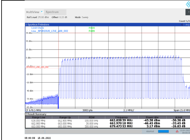
1-N71-PC3-15-20-L-4-DFT-PI/2BPSK-Outer_Full-100@0-Ant1-PASS-see graph
