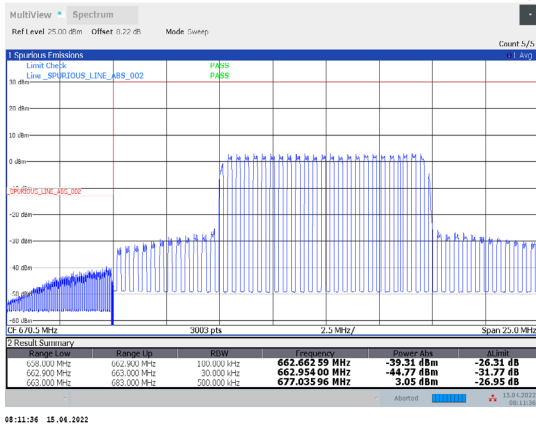
1-N71-PC3-15-20-L-36-CP-256QAM-Inner_Full-53@26-Ant1-PASS-see graph
