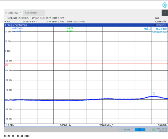
1-N71-PC3-15-20-L-3-CP-QPSK-Outter_Full-106@0-100 0-3000-Ant1--46.23--13-PASS
