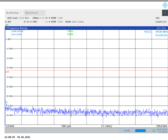
1-N71-PC3-15-15-M-3-CP-QPSK-Outer_Full-79@0-0.00 9-0.15-Ant1--69.58--33-PASS
