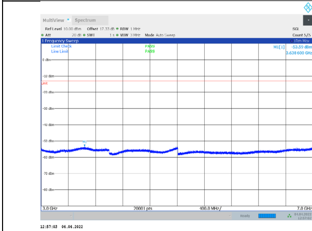
1-N71-PC3-15-20-L-3-CP-QPSK-Outter_Full-106@0-30 00-7000-Ant1--53.59--13-PASS
