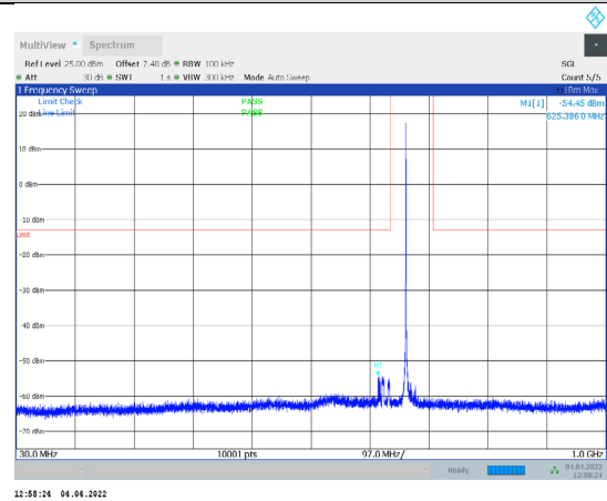
1-N71-PC3-15-20-M-1-CP-QPSK-Edge_1RB_Left-1@0- 30-1000-Ant1--54.45--13-PASS
