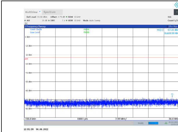
1-N71-PC3-15-15-H-2-CP-QPSK-Edge_1RB_Right-1@ 78.0.15-30-Ant1--67.16--23-PASS
