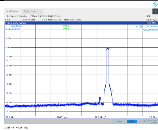
1-N71-PC3-15-15-M-3-CP-QPSK-Outer_Full-79@0-30-1 000-Ant1--51.06--13-PASS
