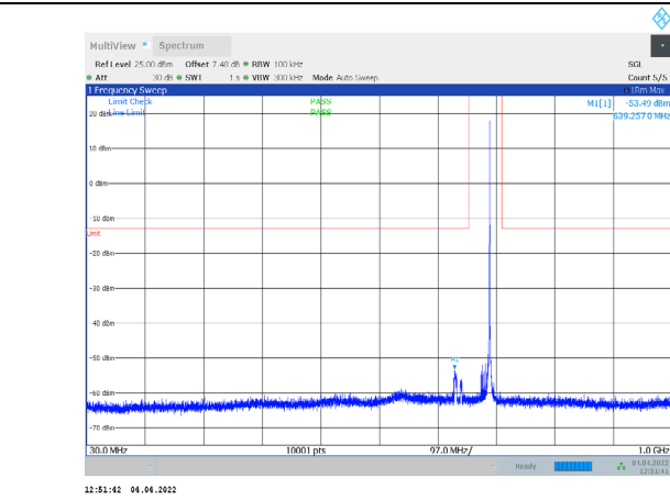
1-N71-PC3-15-15-H-2-CP-QPSK-Edge_1RB_Right-1@ 78.30-1000-Ant1--53.49--13-PASS
