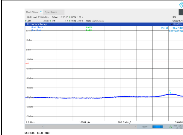
1-N71-PC3-15-15-M-3-CP-QPSK-Outer_Full-79@0-10 00-3000-Ant1--46.27--13-PASS
