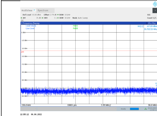
1-N71-PC3-15-20-M-1-CP-QPSK-Edge_1RB_Left-1@ 0-0.15-30-Ant1--67.39--23-PASS
