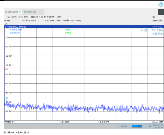
1-N71-PC3-15-20-M-1-CP-QPSK-Edge_1RB_Left-1@0- 0.009-0.15-Ant1--69.12--33-PASS
