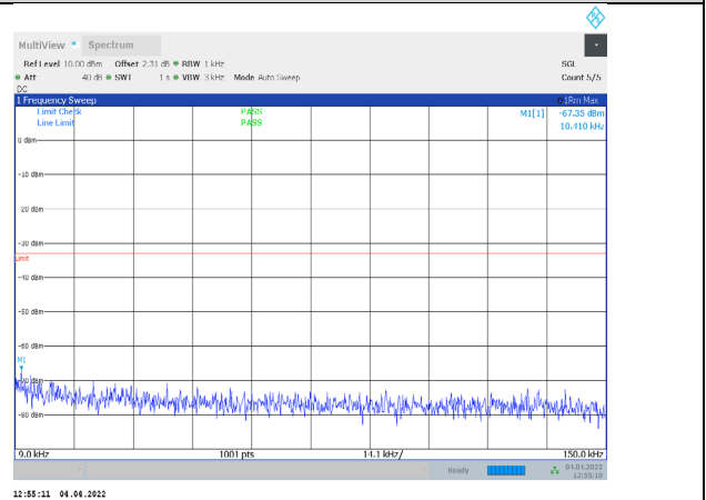
1-N71-PC3-15-20-L-2-CP-QPSK-Edge_1RB_Right-1@1 05-0.009-0.15-Ant1--67.35--33-PASS
