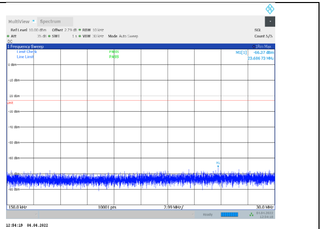
1-N71-PC3-15-20-L-1-CP-QPSK-Edge_1RB_Left-1@0-0 .15-30-Ant1--66.37--23-PASS
