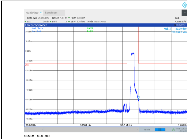
1-N71-PC3-15-20-L-3-CP-QPSK-Outter_Full-106@0-30 -1000-Ant1--50.39--13-PASS
