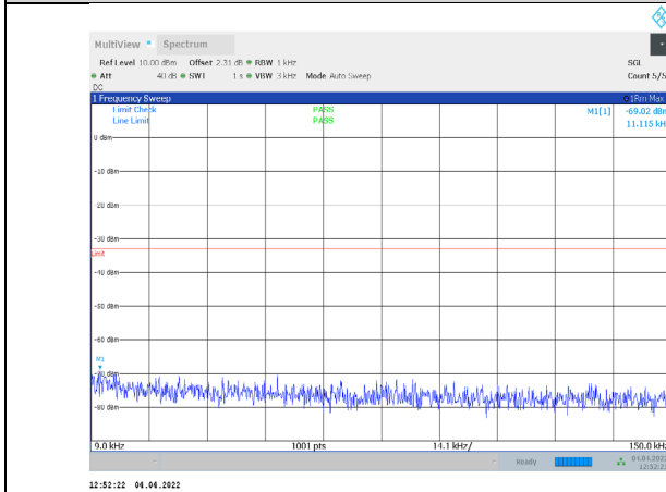
1-N71-PC3-15-15-H-3-CP-QPSK-Outer_Full-79@0.0 09.0.15-Ant1--69.02--33-PASS
