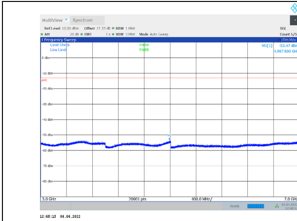
1-N71-PC3-15-15-M-2-CP-QPSK-Edge_1RB_Right-1@ 78-3000-7000-Ant1--53.47--13-PASS
