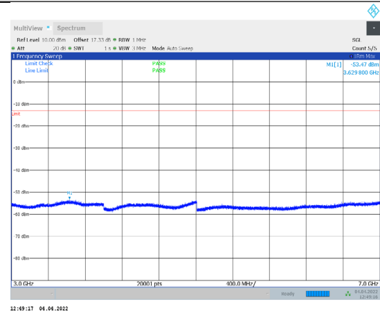
1-N71-PC3-15-15-M-3-CP-QPSK-Outer_Full-79@0-300 0-7000-Ant1--53.47--13-PASS
