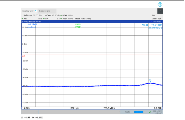
1-N71-PC3-15-20-H-3-CP-QPSK-Outet_Full-106@0-10 00-3000-Ant1--46.14--13-PASS
