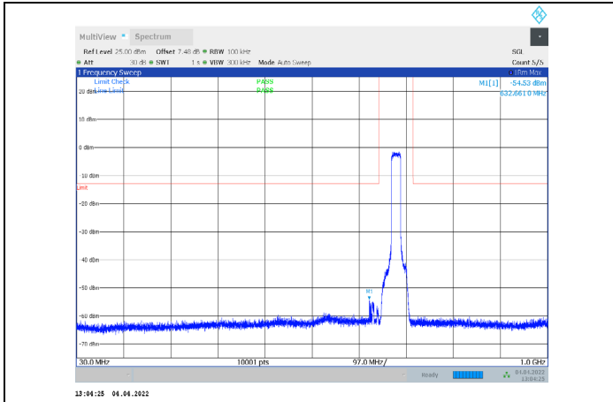
1-N71-PC3-15-20-H-3-CP-QPSK-Outet_Full-106@0-30 -1000-Ant1--54.53--13-PASS
