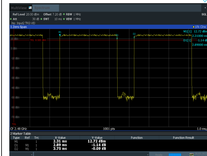
3DH5_Ant1_2480
