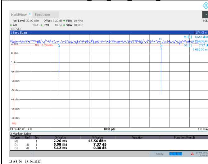
11AX20SISO_Ant1_2437_106Tone_RU53
